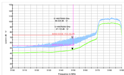
802.11n HT20-Channel 36: Peak + Average
