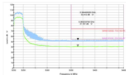
802.11n HT20-Channel 48: Peak + Average
