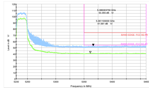
802.11a-Channel 48: Peak + Average
