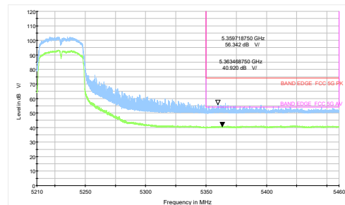
802.11n HT40-Channel 46: Peak + Average
