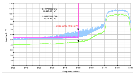
802.11a-Channel 36: Peak + Average
