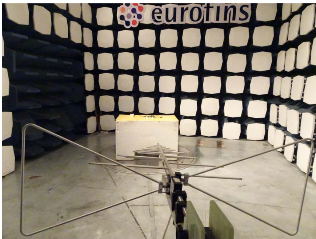
30MHz-1GHz
