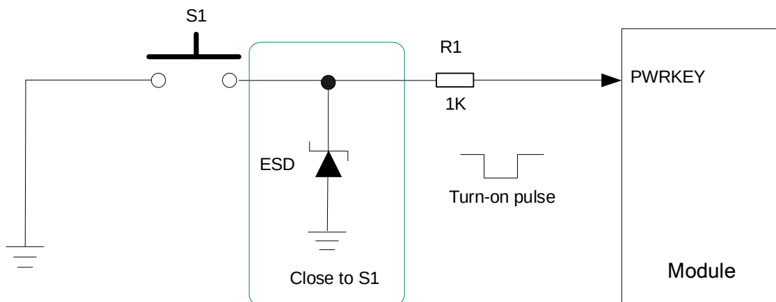
Figure 10: Reference Design of Turn-On with Keystroke
