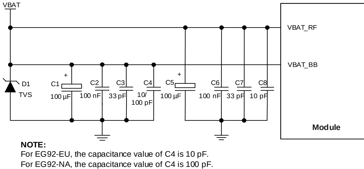
Figure 8: Reference Design of Power Supply
