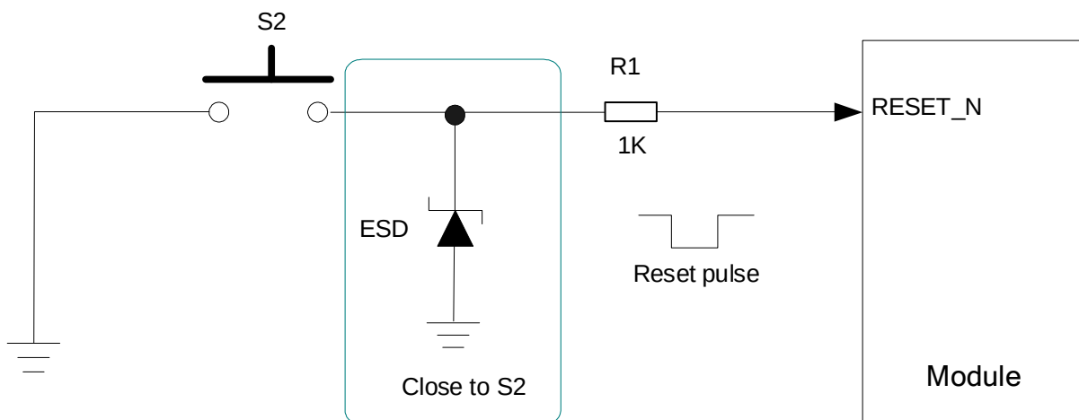
Figure 14: Reference Design of Reset with Button
