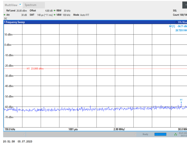
Band II-9262-0.15~30MHz
