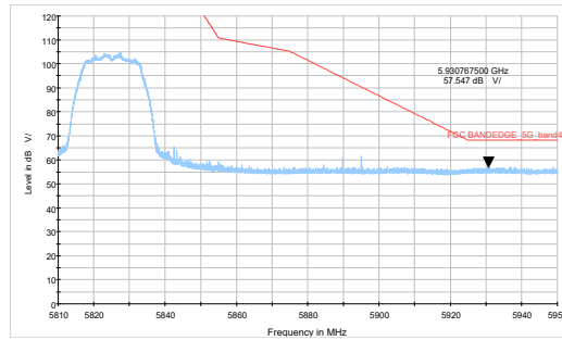
802.11ac VHT20-Channel 165: Peak
