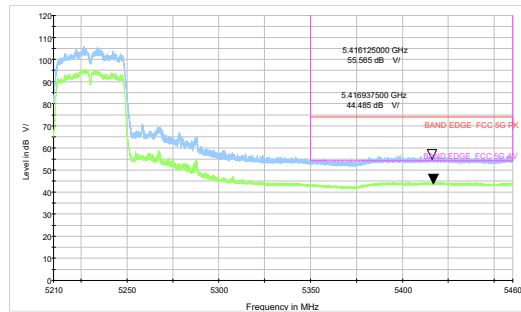
802.11ac VHT40-Channel 46: Peak + Average
