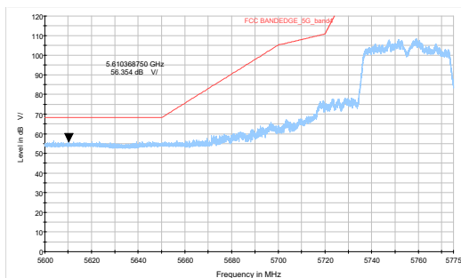
802.11ac VHT40-Channel 151: Peak
