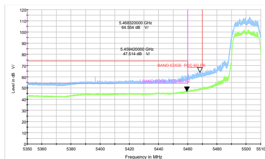
802.11ac VHT20 -Channel 100: Peak + Average
