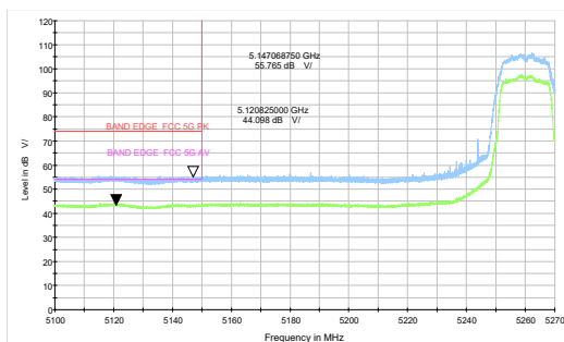
802.11a-Channel 52: Peak + Average
