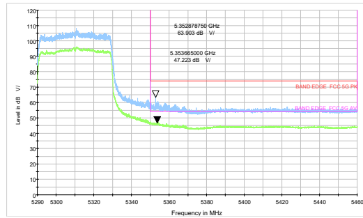
802.11ax HE40-Channel 62: Peak + Average
