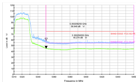
802.11a-Channel 64: Peak + Average
