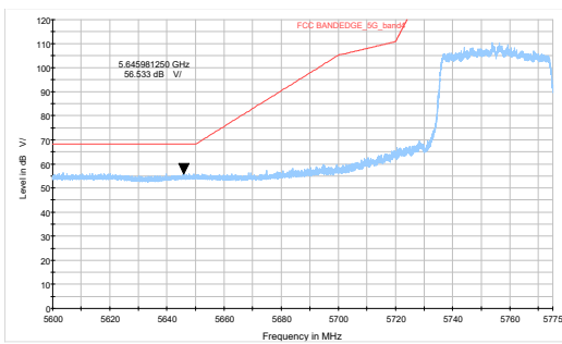
802.11ax HE80- Channel 155: Peak
