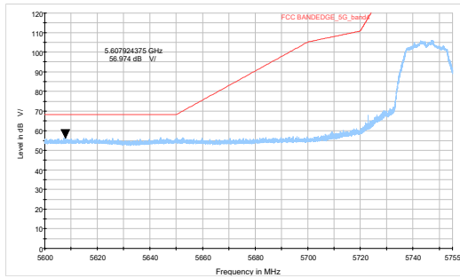
802.11ac VHT20-Channel 149: Peak
