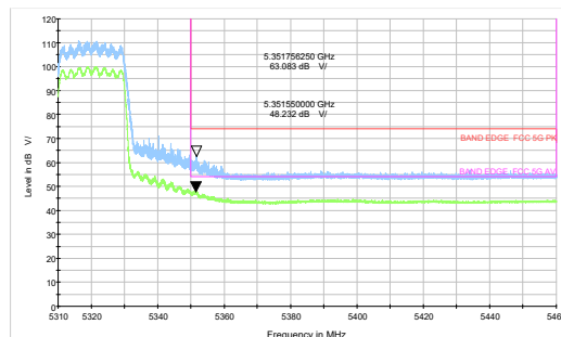
802.11ax HE20 -Channel 64: Peak + Average
