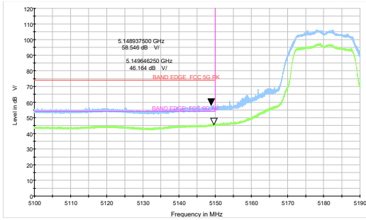
802.11ac VHT20 -Channel 36: Peak + Average
