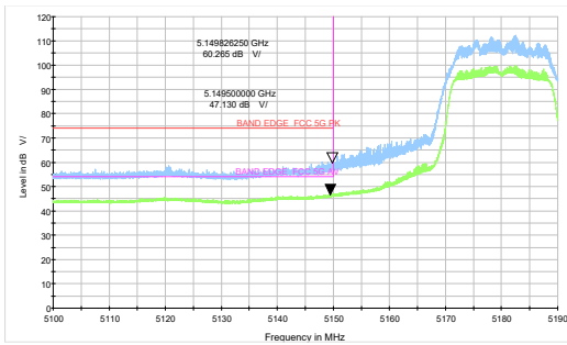
802.11ac VHT40-Channel 38: Peak + Average
