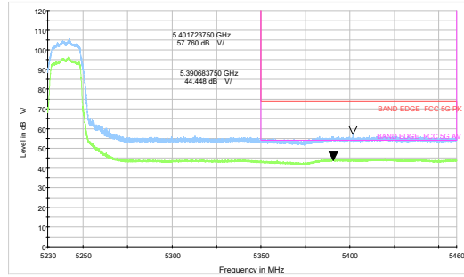
802.11ac VHT20 -Channel 48: Peak + Average
