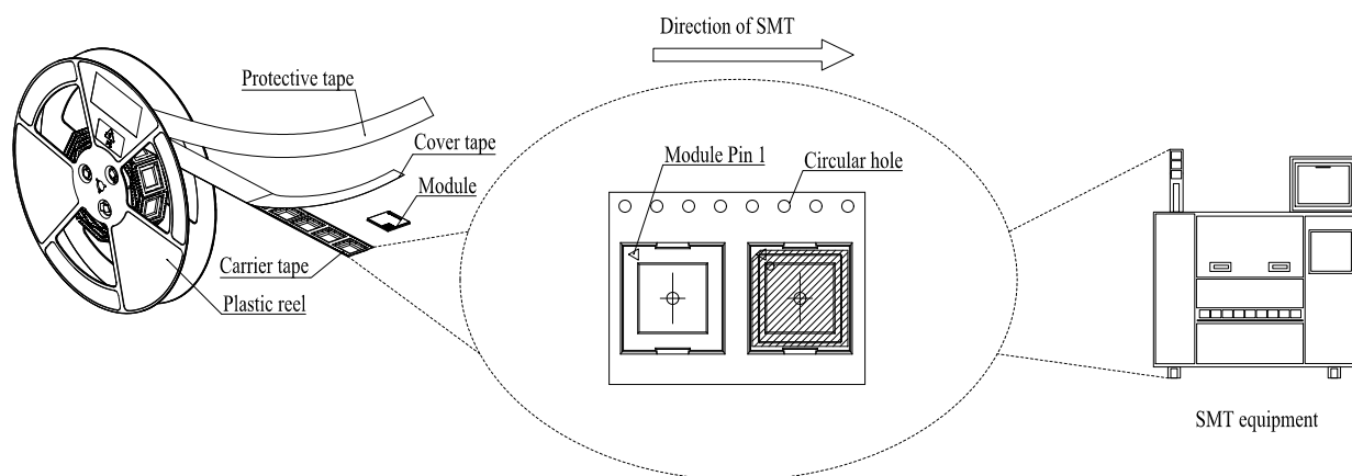
Figure 23: Mounting Direction
