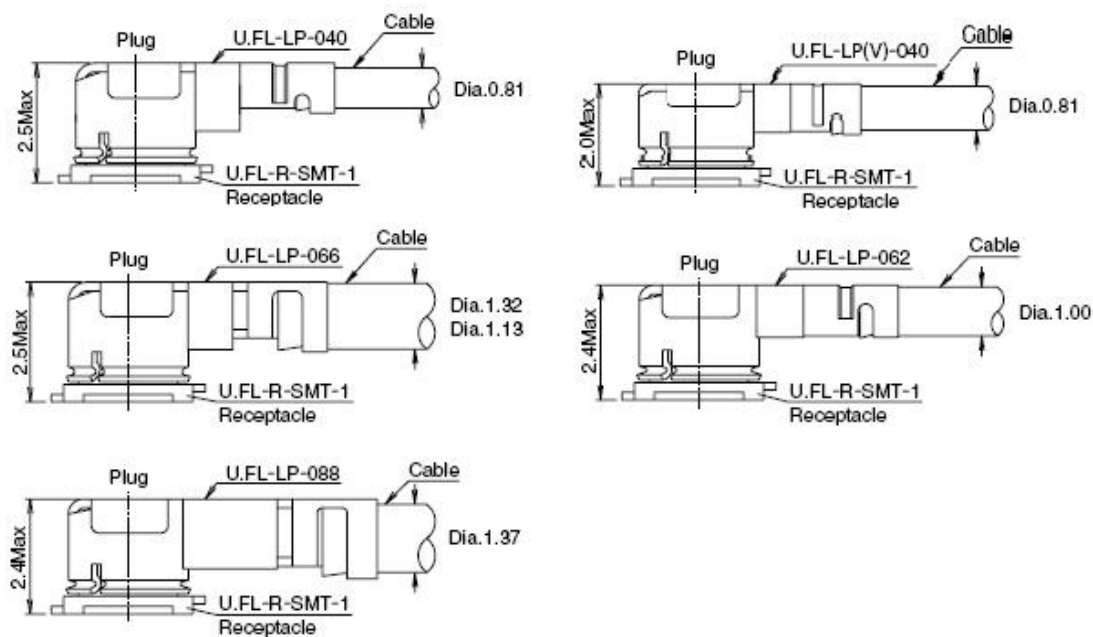
Figure 15: Space Factor of Mated Connectors (Unit: mm)
