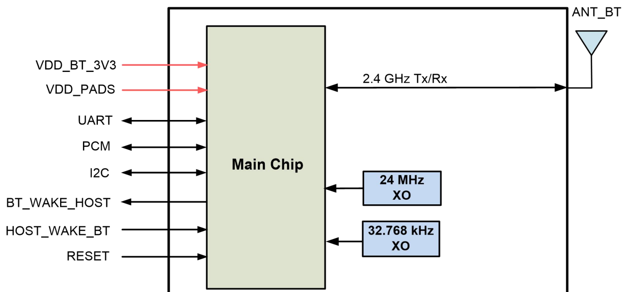
Figure 1: Functional Diagram
