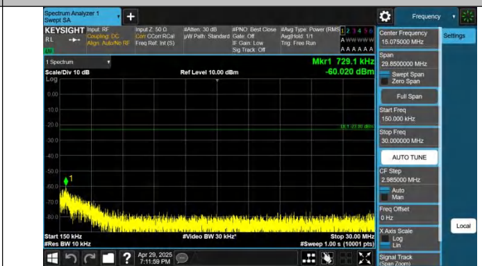
Band5-1.4MHz-QPSK-20643-1RB#0-0.15~30-PASS
