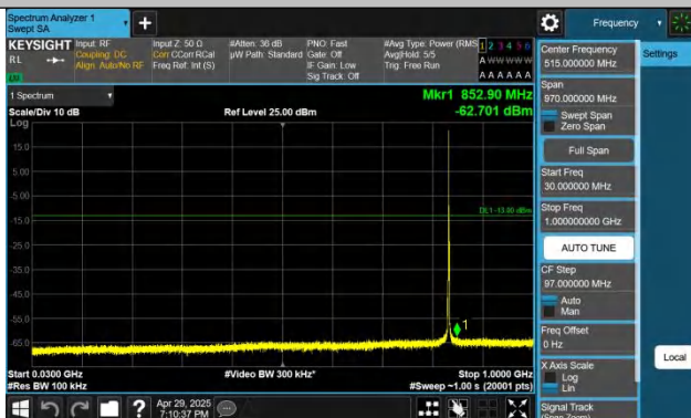
Band5-1.4MHz-QPSK-20525-1RB#0-30~1000-PASS
