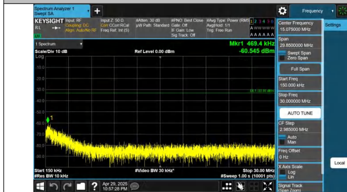
Band66-5MHz-QPSK-132322-1RB#24-0.15~30-PASS
