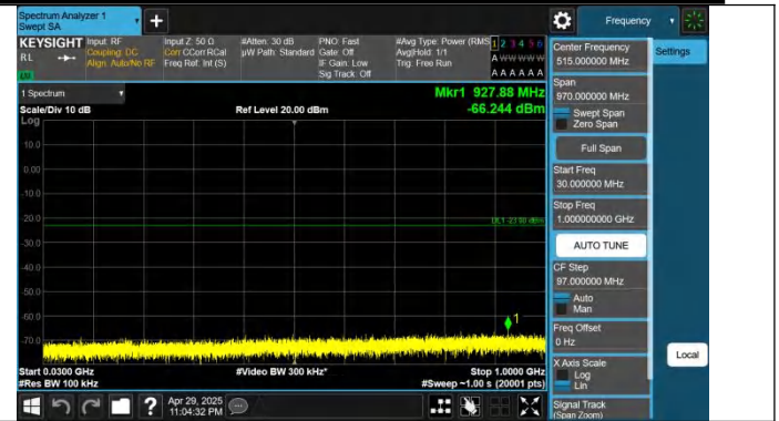
Band66-10MHz-QPSK-132022-1RB#49-30~1000-PASS
