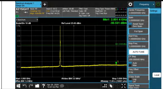
Band66-5MHz-QPSK-132322-1RB#0-1000~3000-PASS
