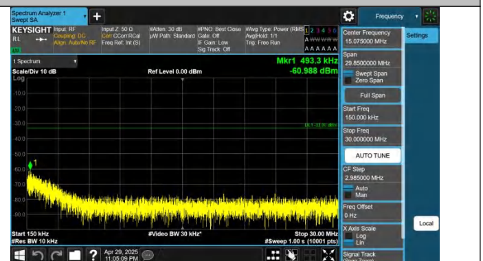
Band66-10MHz-QPSK-132322-1RB#0-0.15~30-PASS
