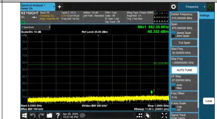
Band66-5MHz-QPSK-132322-1RB#24-30~1000-PASS
