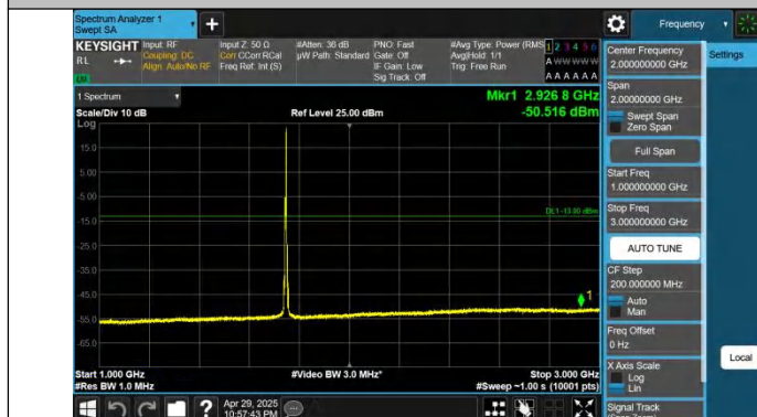
Band66-5MHz-QPSK-132322-1RB#24-1000~3000-PASS
