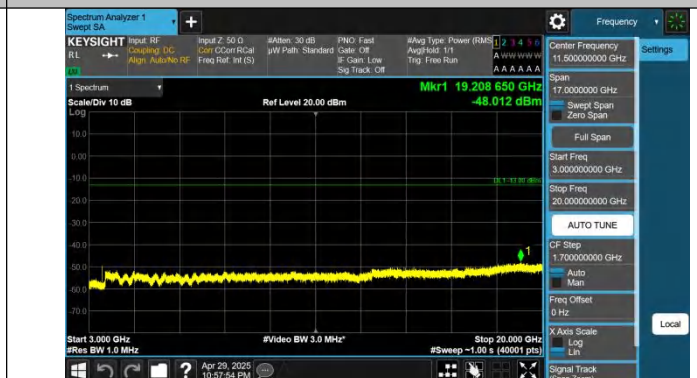
Band66-5MHz-QPSK-132322-1RB#24-3000~20000-PASS
