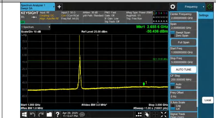
Band66-15MHz-QPSK-132322-1RB#0-1000~3000-PASS
