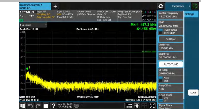
Band66-5MHz-QPSK-131997-1RB#0-0.15~30-PASS
