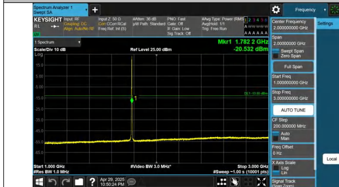
Band66-3MHz-QPSK-132657-1RB#14-1000~3000-PASS
