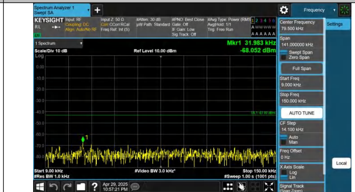
Band66-5MHz-QPSK-132322-1RB#24-0.009~0.15-PASS
