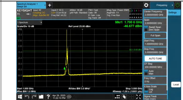
Band66-20MHz-QPSK-132322-1RB#0-1000~3000-PASS
