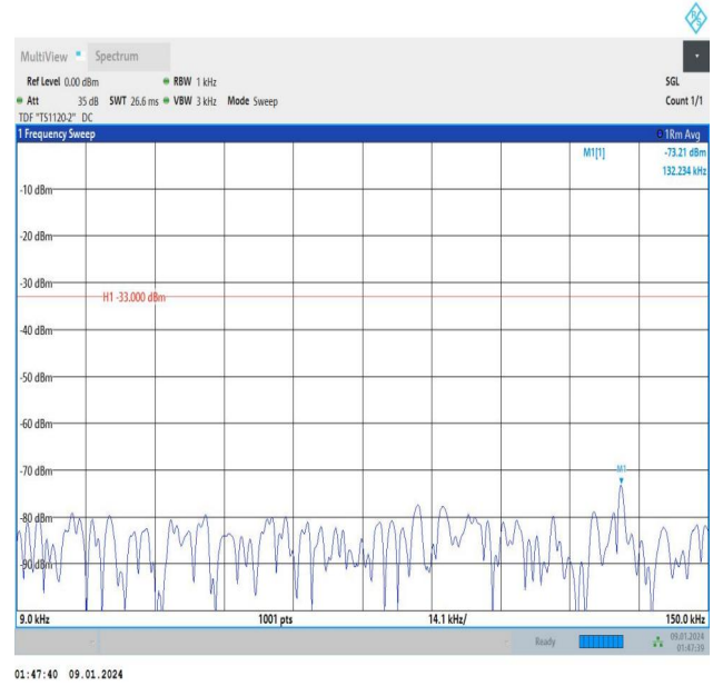
Band12_1.4MHz_16QAM_23095_1RB#5_0.009~0.15_0.009~0.15
