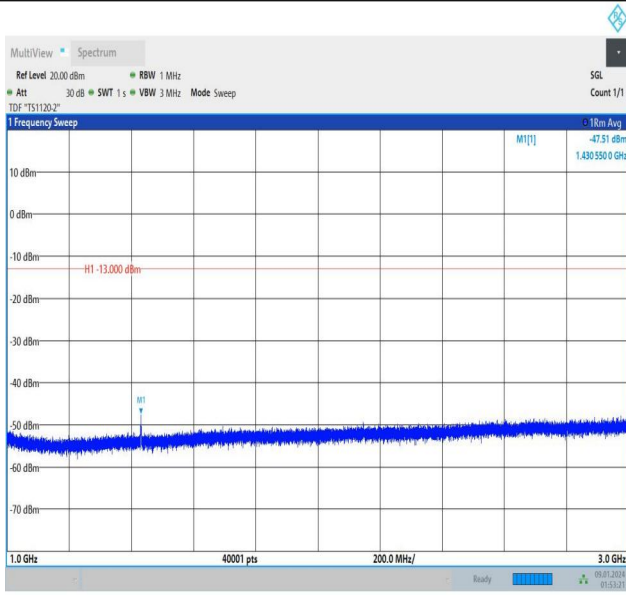
Band12_1.4MHz_16QAM_23173_6RB#0_1000~3000_1000~3000
