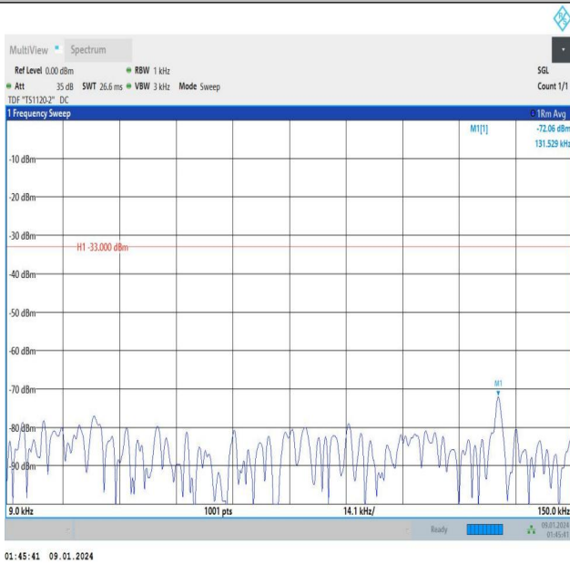
Band12_1.4MHz_QPSK_23095_1RB#0_0.009~0.15_0.009~0.15
