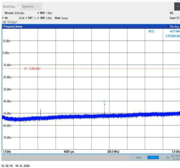
Band12_1.4MHz_16QAM_23173_1RB#5_1000~3000_1000~3000
