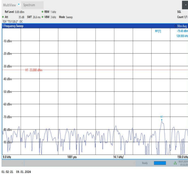
Band12_1.4MHz_QPSK_23173_6RB#0_0.009~0.15_0.009~0.15
