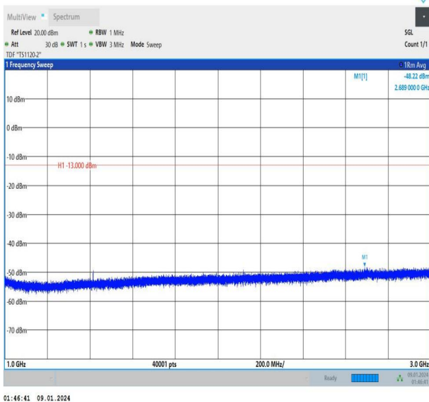
Band12_1.4MHz_16QAM_23095_1RB#0_1000~3000_1000~3000
