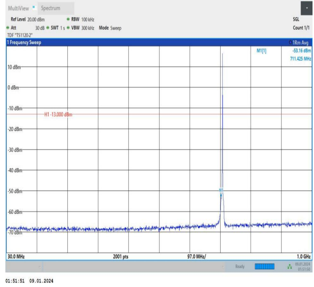
Band12_1.4MHz_16QAM_23173_1RB#5_30~1000_30~1000
