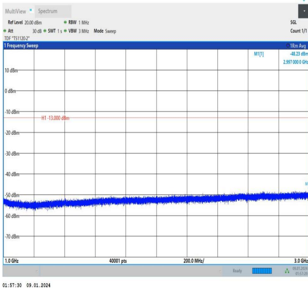
Band12_3MHz_16QAM_23025_15RB#0_1000~3000_1000~3000
