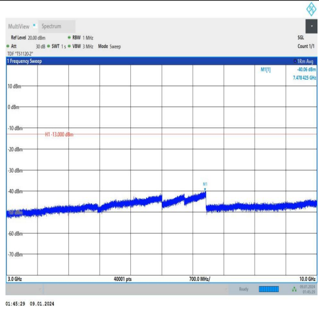
Band12_1.4MHz_16QAM_23017_6RB#0_3000~10000_3000~10000
