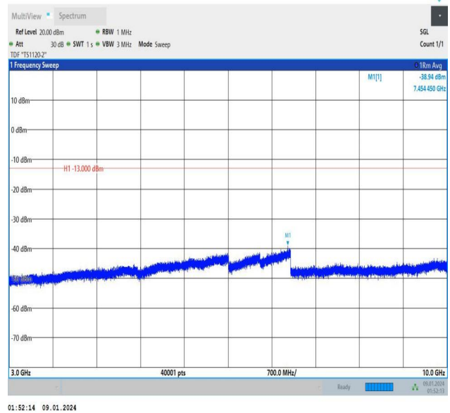
Band12_1.4MHz_16QAM_23173_1RB#5_3000~10000_3000~10000
