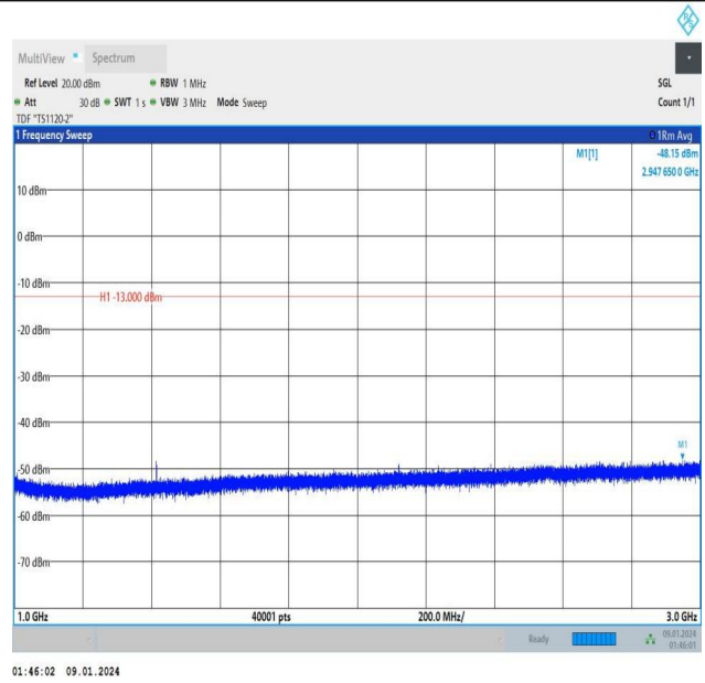
Band12_1.4MHz_QPSK_23095_1RB#0_1000~3000_1000~3000
