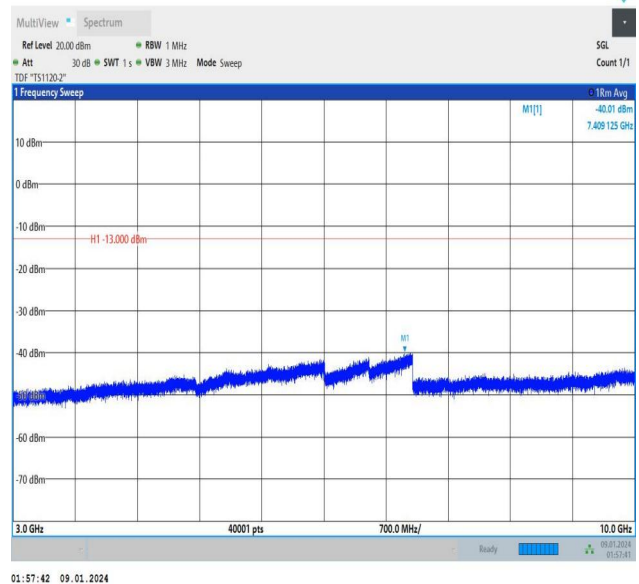
Band12_3MHz_16QAM_23025_15RB#0_3000~10000_3000~10000
