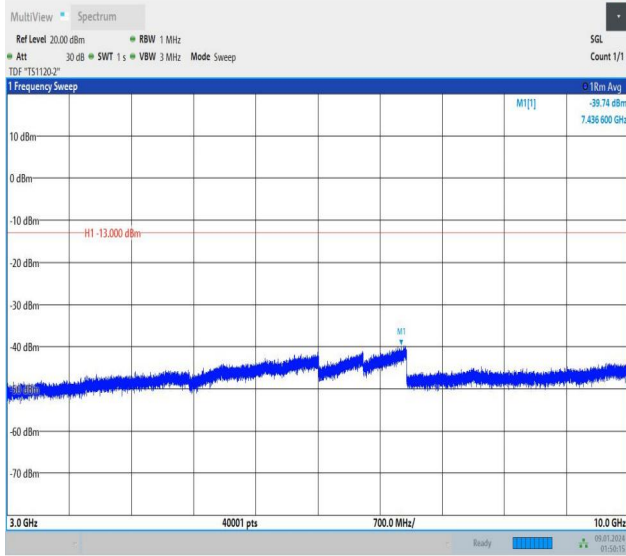
Band12_1.4MHz_QPSK_23173_1RB#0_3000~10000_3000~10000
