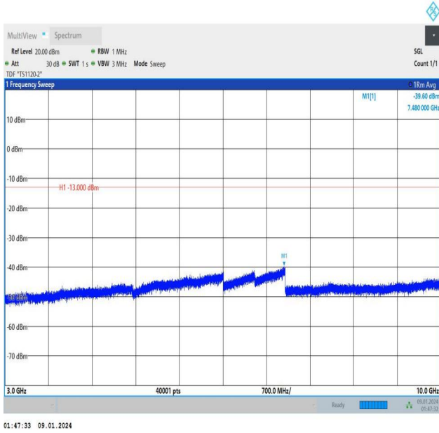
Band12_1.4MHz_QPSK_23095_1RB#5_3000~10000_3000~10000
