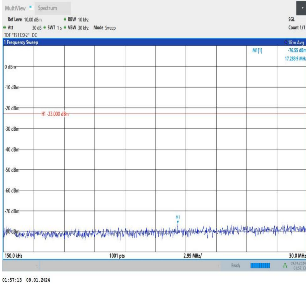
Band12_3MHz_16QAM_23025_15RB#0_0.15~30_0.15~30
