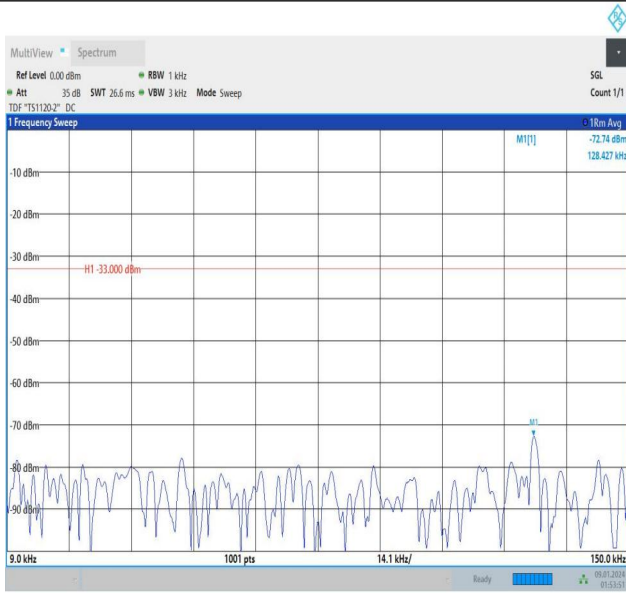
Band12_1.4MHz_16QAM_23173_6RB#0_1000~3000_1000~3000
