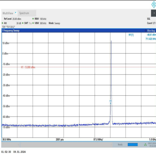
Band12_1.4MHz_QPSK_23173_6RB#0_30~1000_30~1000
