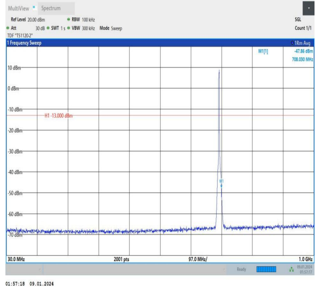
Band12_3MHz_16QAM_23025_15RB#0_30~1000_30~1000
