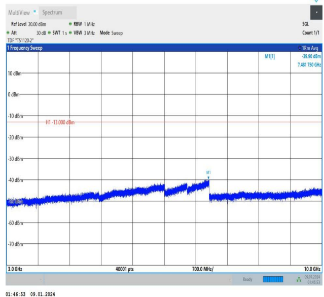
Band12_1.4MHz_16QAM_23095_1RB#0_3000~10000_3000~10000
