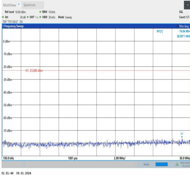
Band12_1.4MHz_16QAM_23173_1RB#5_0.15~30_0.15~30
