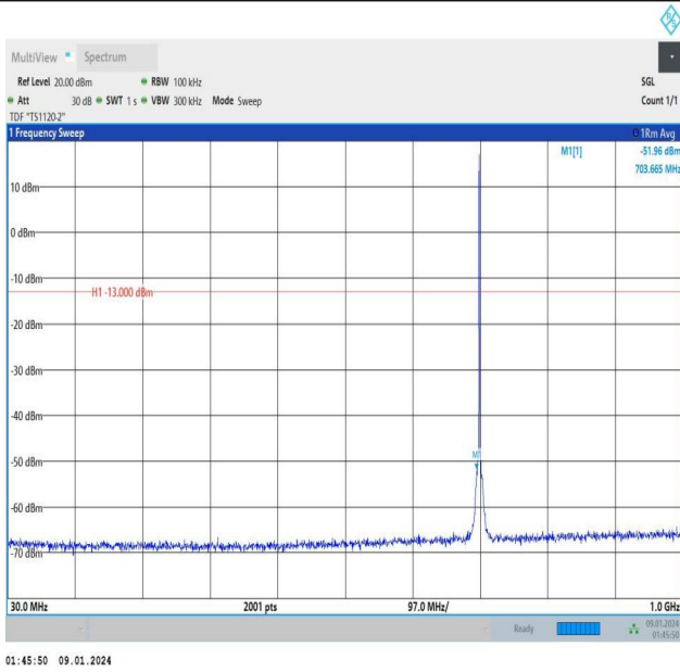
Band12_1.4MHz_QPSK_23095_1RB#0_30~1000_30~1000
