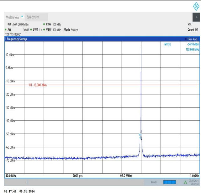
Band12_1.4MHz_16QAM_23095_1RB#5_30~1000_30~1000
