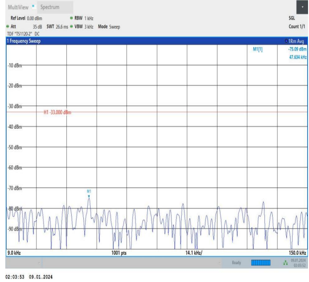
Band12_3MHz_16QAM_23165_1RB#14_0.009~0.15_0.009~0.15
