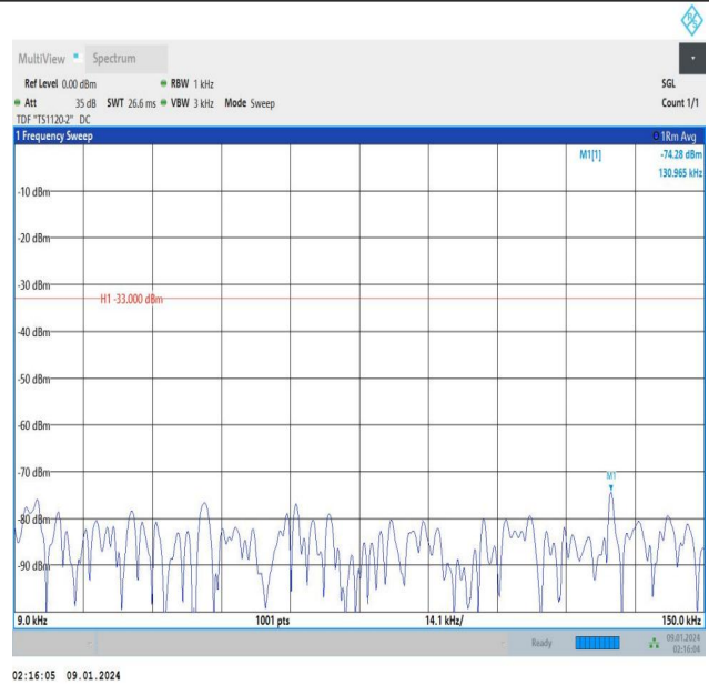
Band12_5MHz_16QAM_23155_1RB#24_0.009~0.15_0.009~0.15 15
