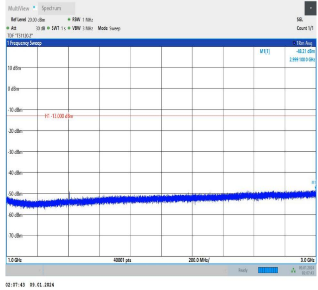
Band12_5MHz_QPSK_23035_1RB#24_1000~3000_1000~300 0
