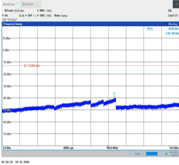
Band12_5MHz_QPSK_23035_25RB#0_3000~10000_3000~10000
