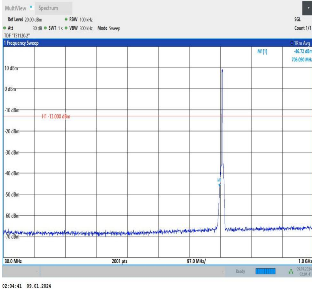
Band12_3MHz_QPSK_23165_15RB#0_30~1000_30~1000
