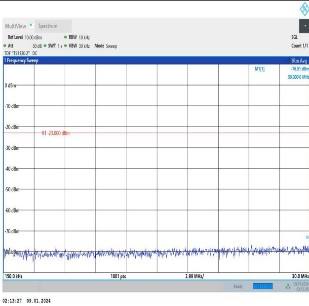
Band12_5MHz_16QAM_23095_25RB#0_0.15~30_0.15~30
