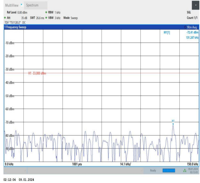
Band12_5MHz_16QAM_23095_1RB#24_0.009~0.15_0.009~0.15
