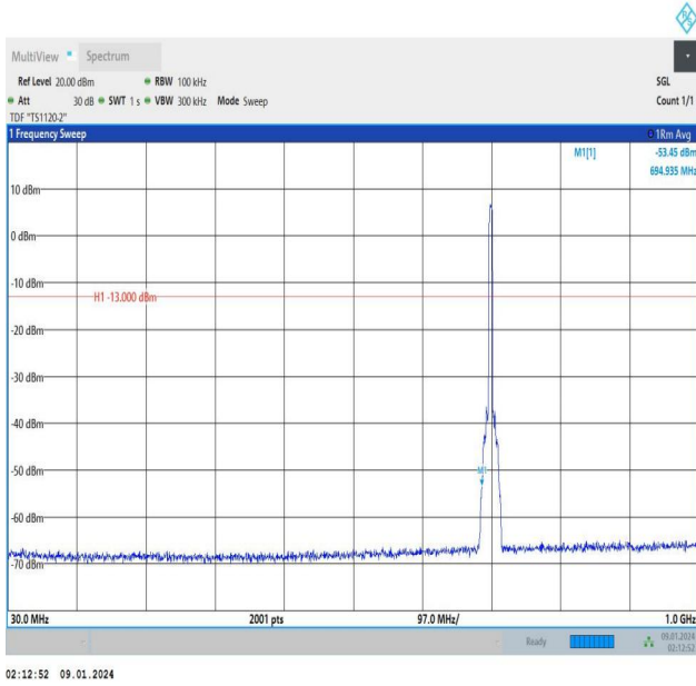
Band12_5MHz_QPSK_23095_25RB#0_30~1000_30~1000
