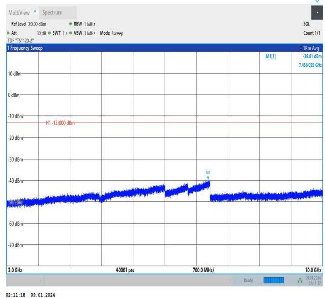
Band12_5MHz_16QAM_23095_1RB#0_3000~10000_3000~10
