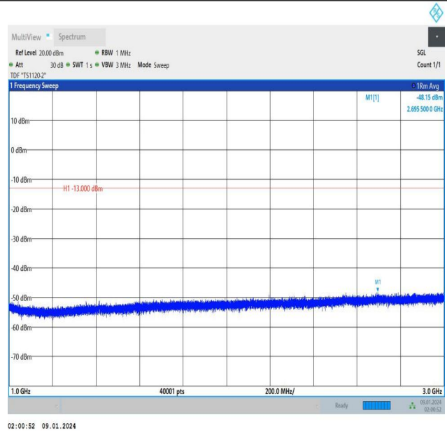
Band12_3MHz_QPSK_23095_15RB#0_1000~3000_1000~300
