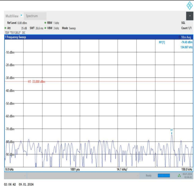
Band12_5MHz_16QAM_23035_1RB#0_0.009~0.15_0.009~0.155
