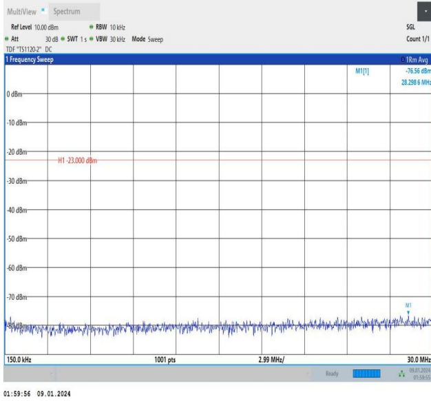
Band12_3MHz_16QAM_23095_1RB#14_0.15~30_0.15~30
