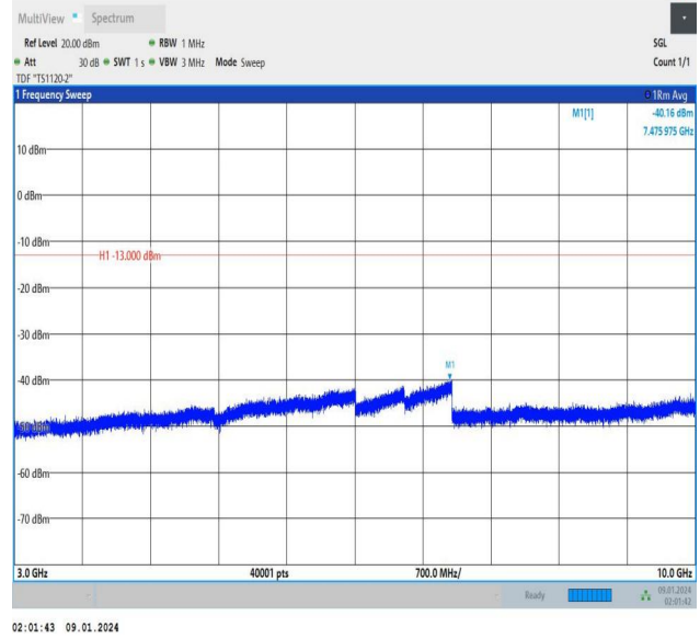
Band12_3MHz_16QAM_23095_15RB#0_3000~10000_3000~10000
