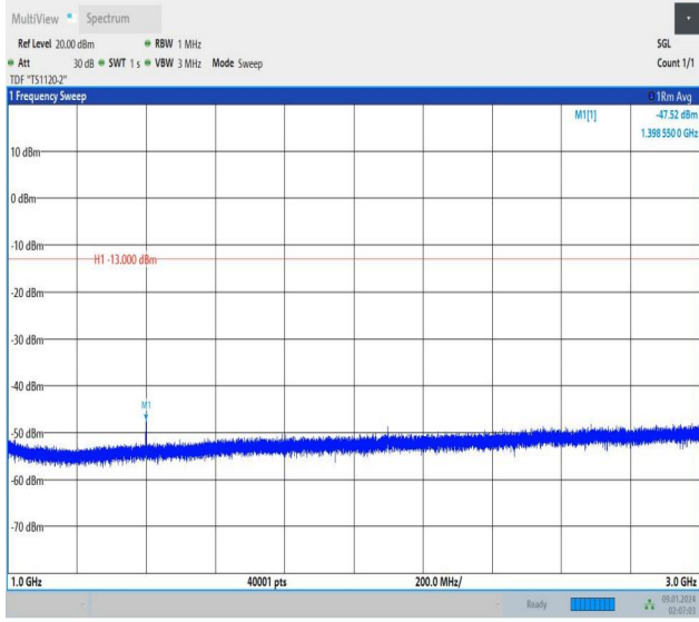
Band12_5MHz_16QAM_23035_1RB#0_1000~3000_1000~30
