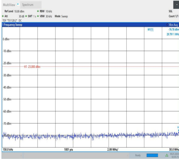
Band12_3MHz_16QAM_23165_15RB#0_0.15~30_0.15~30
