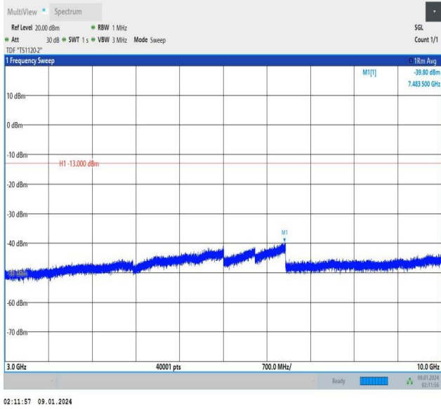
Band12_5MHz_QPSK_23095_1RB#24_3000~10000_3000~10000
