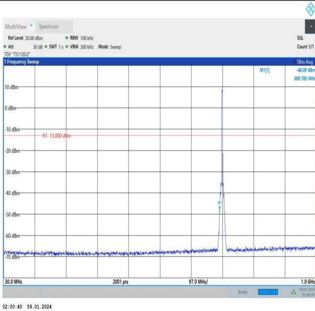
Band12_3MHz_QPSK_23095_15RB#0_30~1000_30~1000
