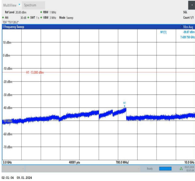
Band12_3MHz_QPSK_23095_15RB#0_3000~10000_3000~10000
