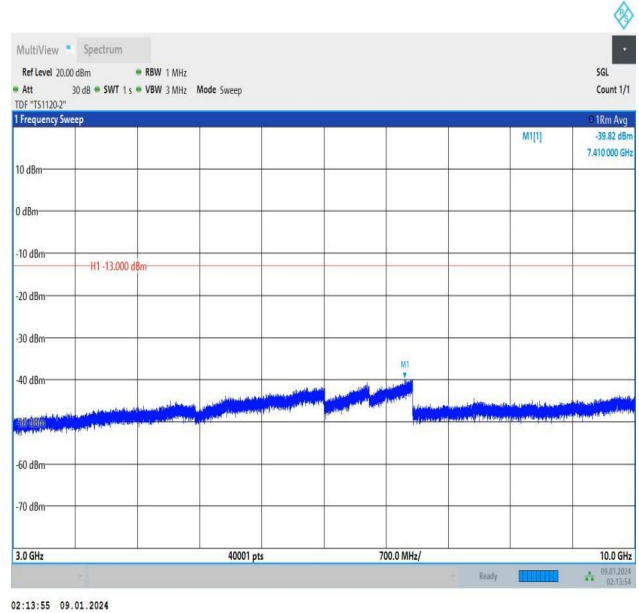
Band12_5MHz_16QAM_23095_25RB#0_3000~10000_3000~10000
