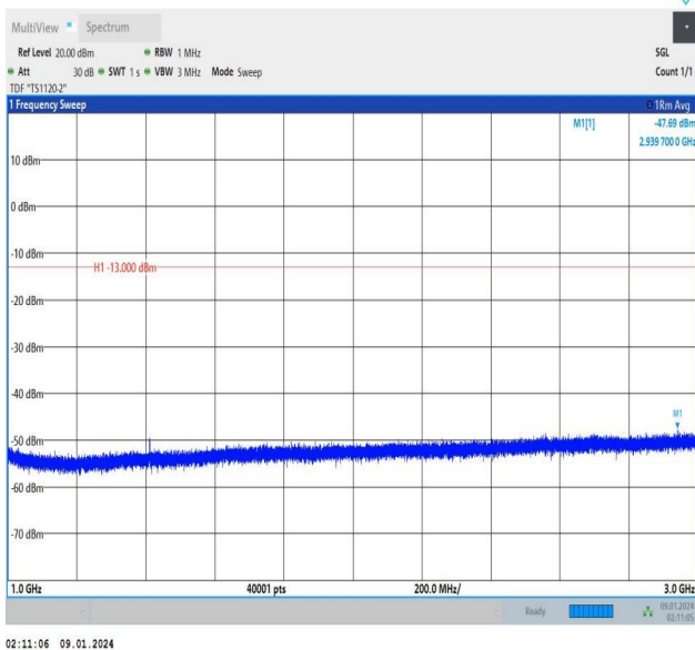
Band12_5MHz_16QAM_23095_1RB#0_1000~3000_1000~30
