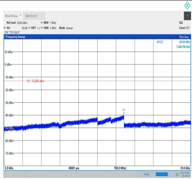
Band12_3MHz_16QAM_23165_1RB#14_3000~10000_3000~10000
