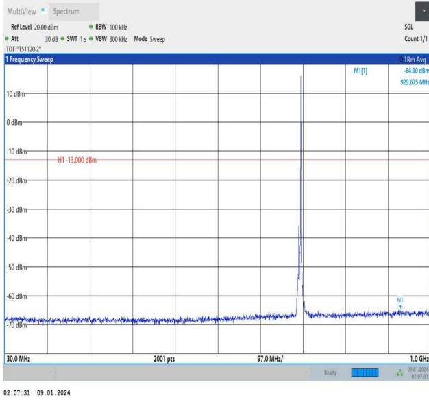
Band12_5MHz_QPSK_23035_1RB#24_30~1000_30~1000
