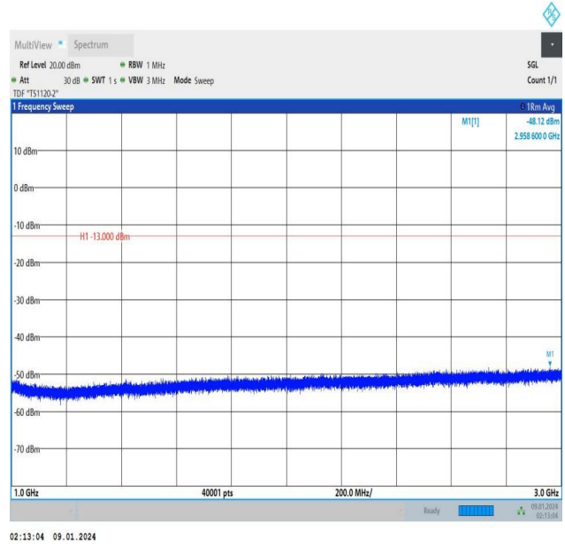
Band12_5MHz_QPSK_23095_25RB#0_1000~3000_1000~300 0
