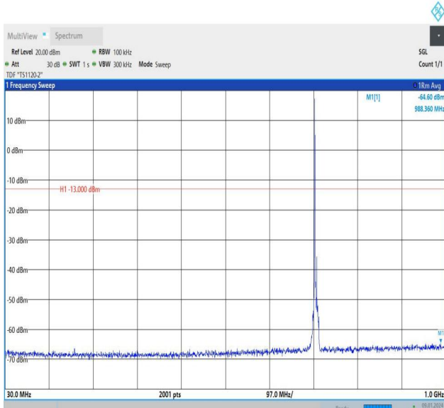
Band12_5MHz_QPSK_23155_1RB#0_30~1000_30~1000
