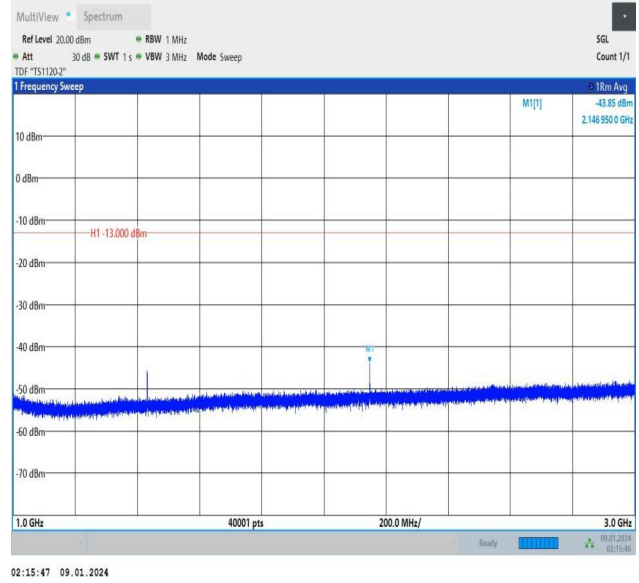
Band12_5MHz_QPSK_23155_1RB#24_1000~3000_1000~300 0
