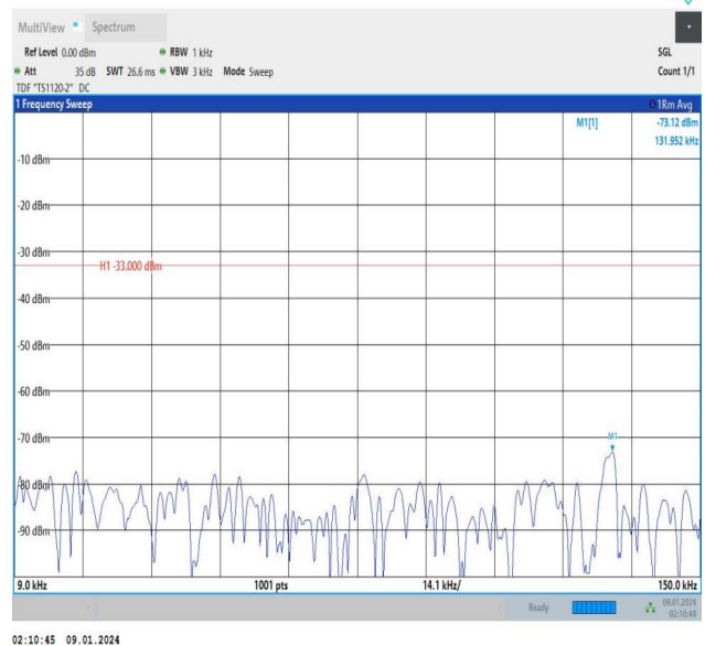
Band12_5MHz_16QAM_23095_1RB#0_0.009~0.15_0.009~0.15
