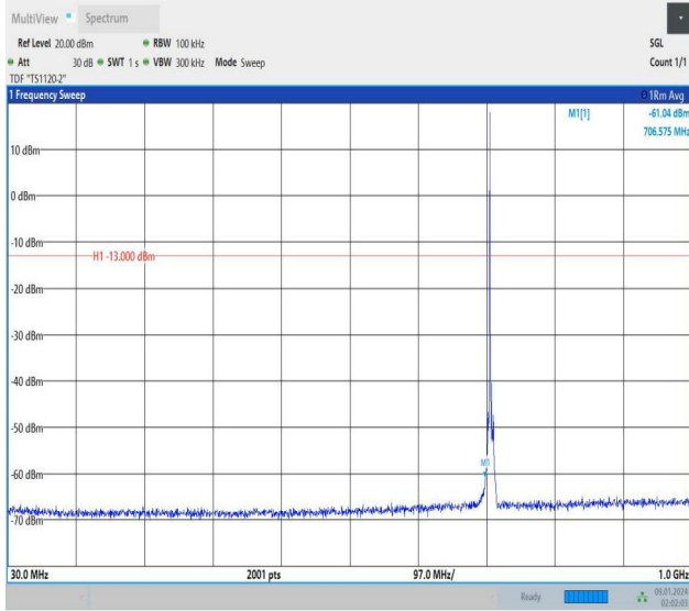
Band12_3MHz_QPSK_23165_1RB#0_30~1000_30~1000
