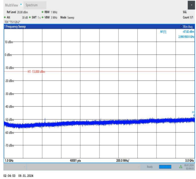
Band12_3MHz_QPSK_23165_15RB#0_1000~3000_1000~300 0
