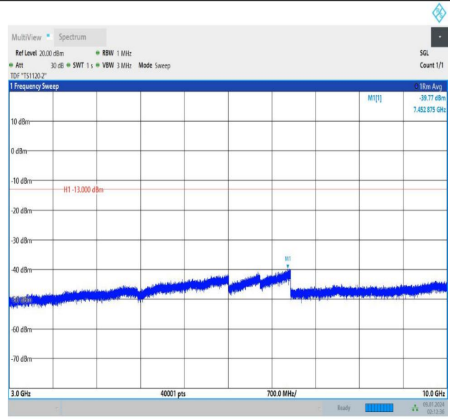
Band12_5MHz_16QAM_23095_1RB#24_3000~10000_3000~10000
