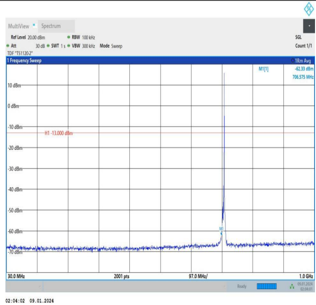
Band12_3MHz_16QAM_23165_1RB#14_30~1000_30~1000
