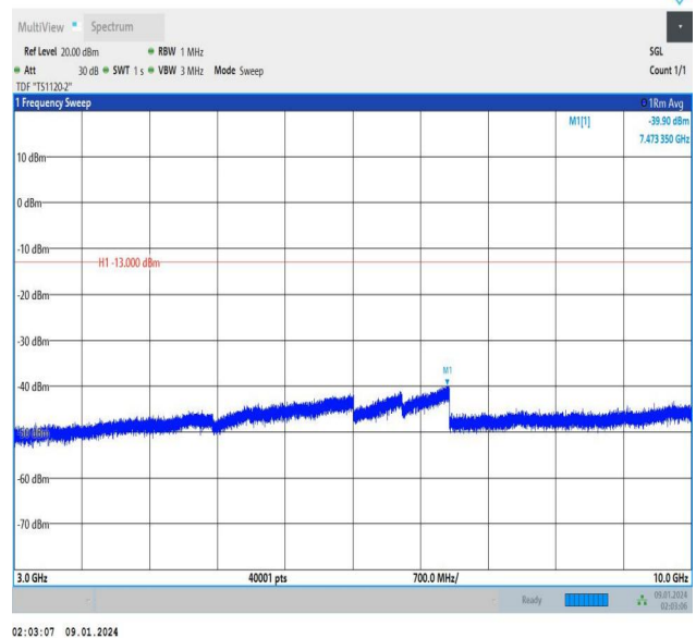
Band12_3MHz_16QAM_23165_1RB#0_3000~10000_3000~10
