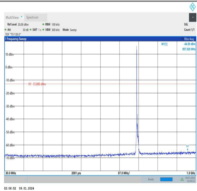
Band12_5MHz_16QAM_23035_1RB#0_30~1000_30~1000
