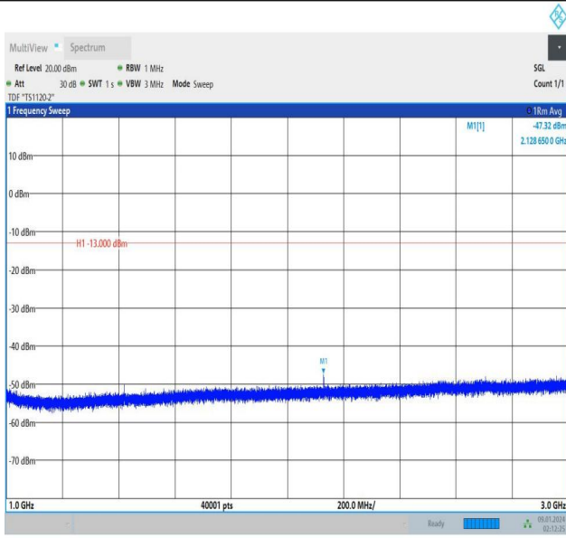
Band12_5MHz_16QAM_23095_1RB#24_1000~3000_1000~3000
