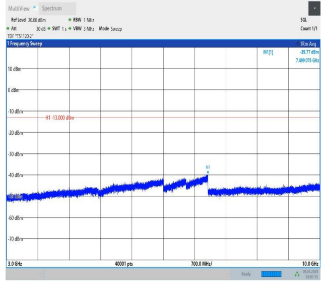
Band12_5MHz_16QAM_23035_1RB#0_3000~10000_3000~10
