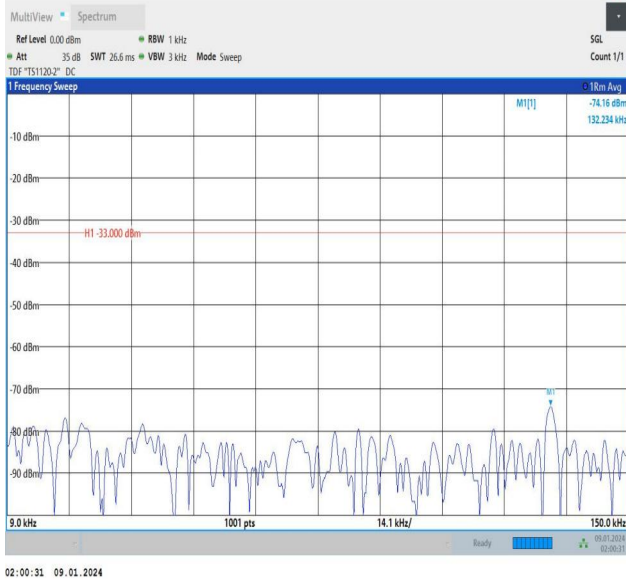
Band12_3MHz_QPSK_23095_15RB#0_0.009~0.15_0.009~0.
