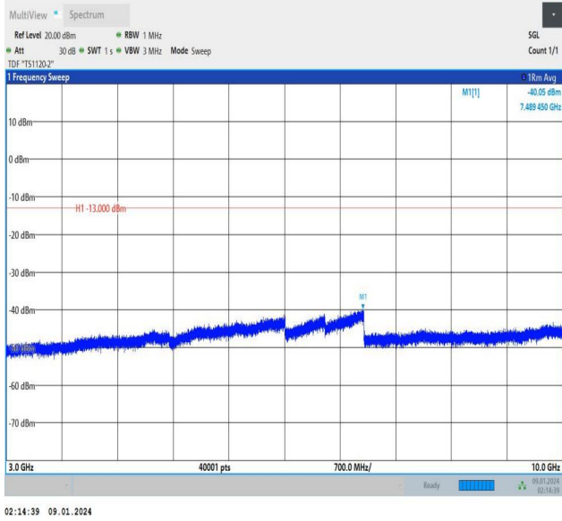
Band12_5MHz_QPSK_23155_1RB#0_3000~10000_3000~10000
