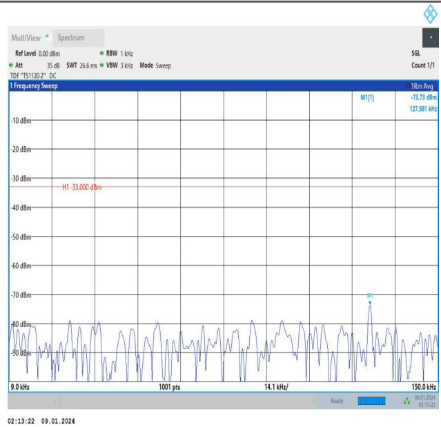
Band12_5MHz_16QAM_23095_25RB#0_0.009~0.15_0.009~0. 15
