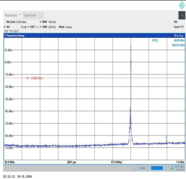
Band12_5MHz_16QAM_23095_1RB#24_30~1000_30~1000
