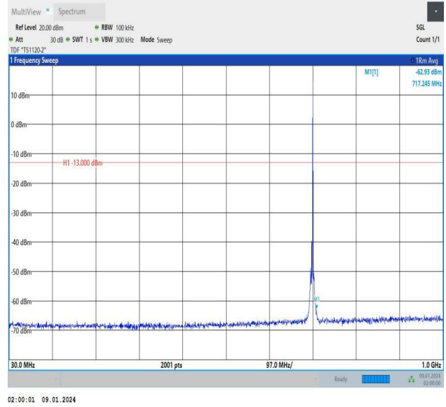
Band12_3MHz_16QAM_23095_1RB#14_30~1000_30~1000
