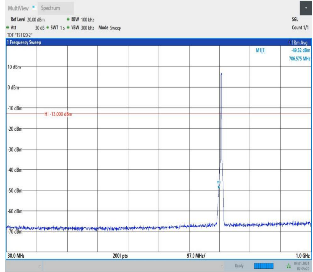
Band12_3MHz_16QAM_23165_15RB#0_30~1000_30~1000
