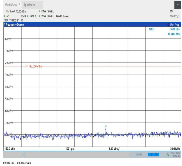
Band12_3MHz_QPSK_23095_15RB#0_0.15~30_0.15~30
