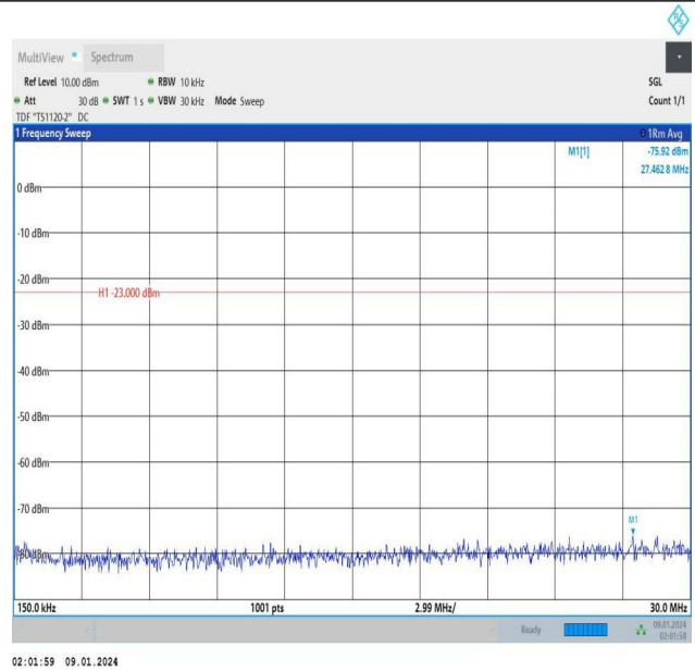
Band12_3MHz_QPSK_23165_1RB#0_0.15~30_0.15~30
