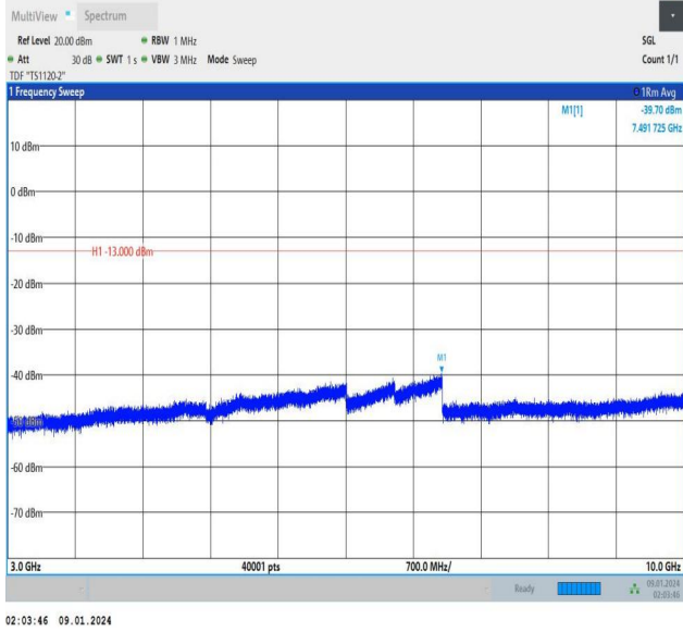
Band12_3MHz_QPSK_23165_1RB#14_3000~10000_3000~10000
