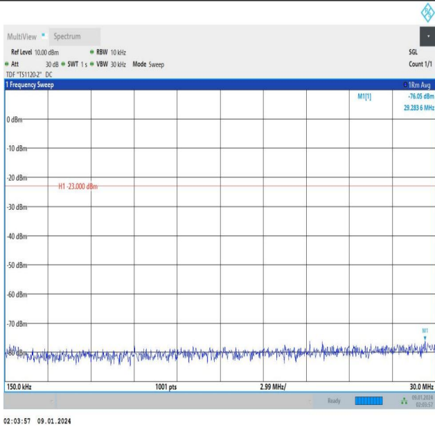
Band12_3MHz_16QAM_23165_1RB#14_0.15~30_0.15~30
