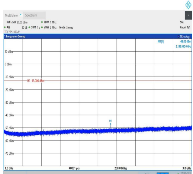
Band12_5MHz_QPSK_23155_1RB#0_1000~3000_1000~3000
