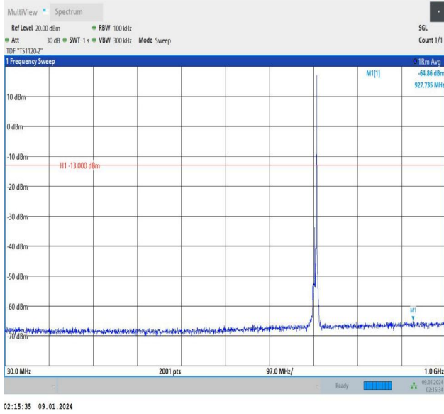
Band12_5MHz_QPSK_23155_1RB#24_30~1000_30~1000
