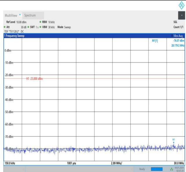
Band12_5MHz_QPSK_23035_1RB#24_0.15~30_0.15~30
