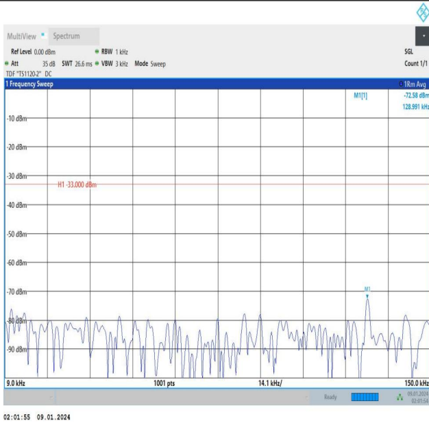
Band12_3MHz_QPSK_23165_1RB#0_0.009~0.15_0.009~0.15
