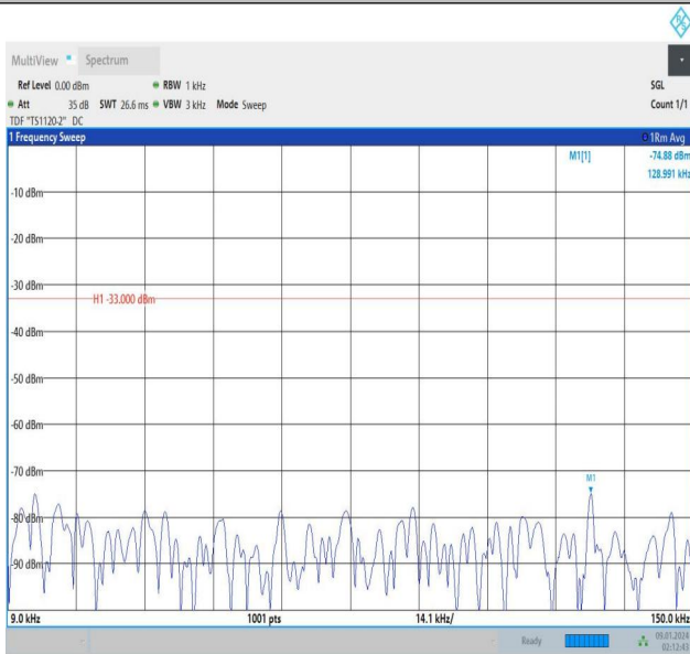
Band12_5MHz_16QAM_23095_1RB#24_1000~3000_1000~3000
