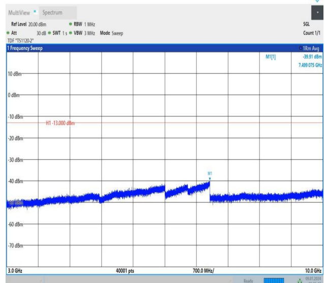
Band12_3MHz_16QAM_23165_15RB#0_3000~10000_3000~10000
