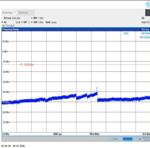
Band12_5MHz_QPSK_23035_1RB#0_3000~10000_3000~10000
