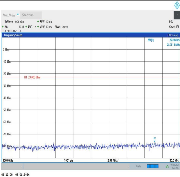
Band12_5MHz_16QAM_23095_1RB#24_0.15~30_0.15~30
