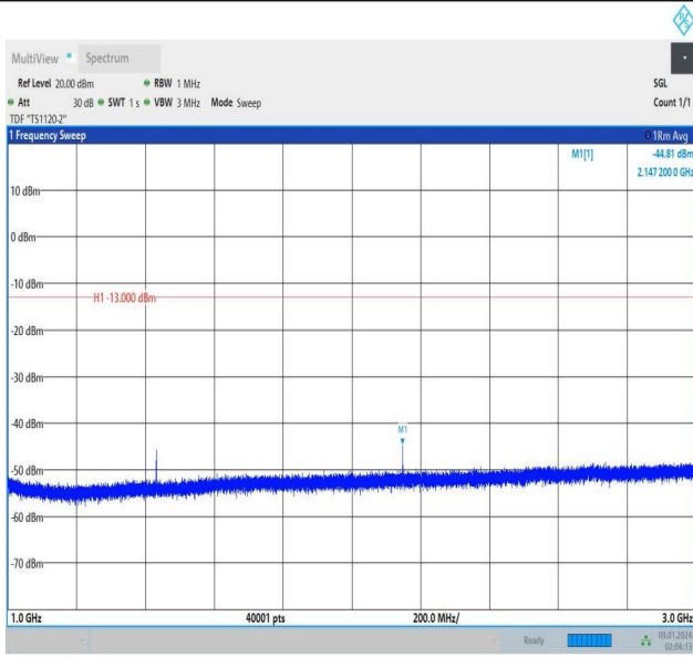
Band12_3MHz_16QAM_23165_1RB#14_1000~3000_1000~3000
