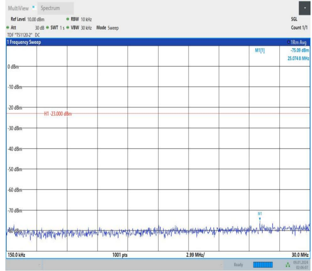
Band12_5MHz_QPSK_23035_1RB#0_0.15~30_0.15~30
