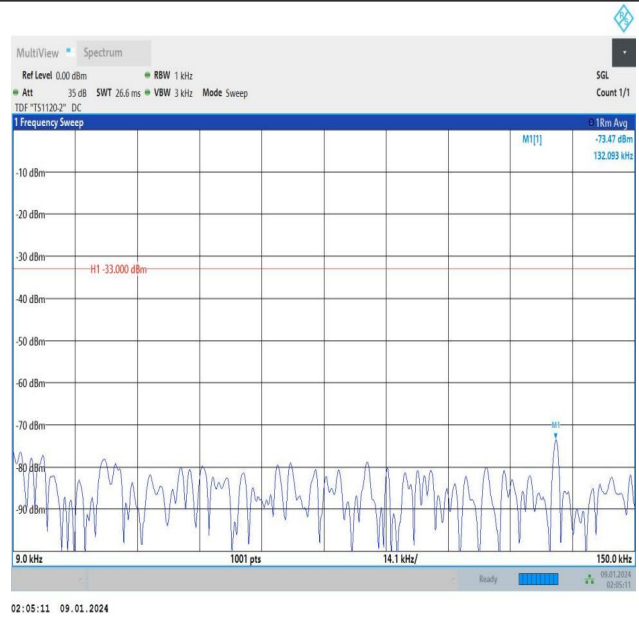
Band12_3MHz_16QAM_23165_15RB#0_0.009~0.15_0.009~0. 15
