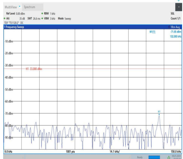
Band12_3MHz_16QAM_23165_1RB#0_0.009~0.15_0.009~0.1
