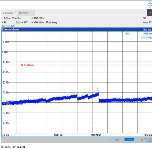
Band12_3MHz_QPSK_23165_15RB#0_3000~10000_3000~1 0000
