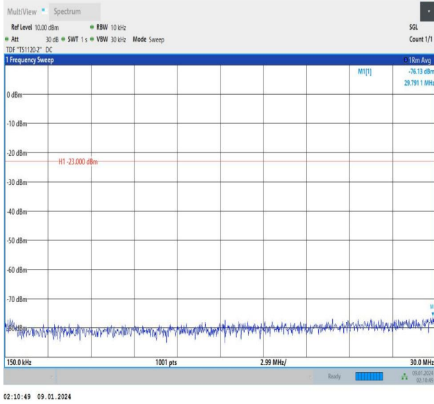
Band12_5MHz_16QAM_23095_1RB#0_0.15~30_0.15~30
