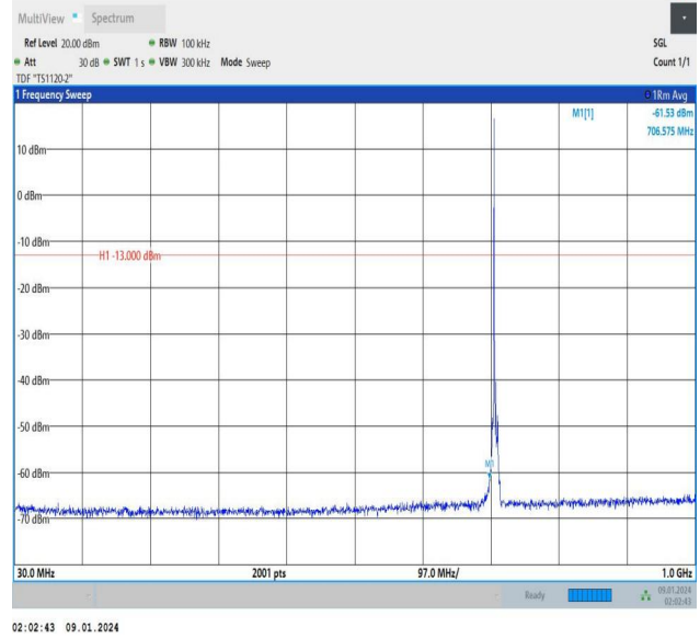
Band12_3MHz_16QAM_23165_1RB#0_30~1000_30~1000
