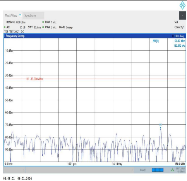
Band12_5MHz_16QAM_23035_1RB#24_0.009~0.15_0.009~0.15 15
