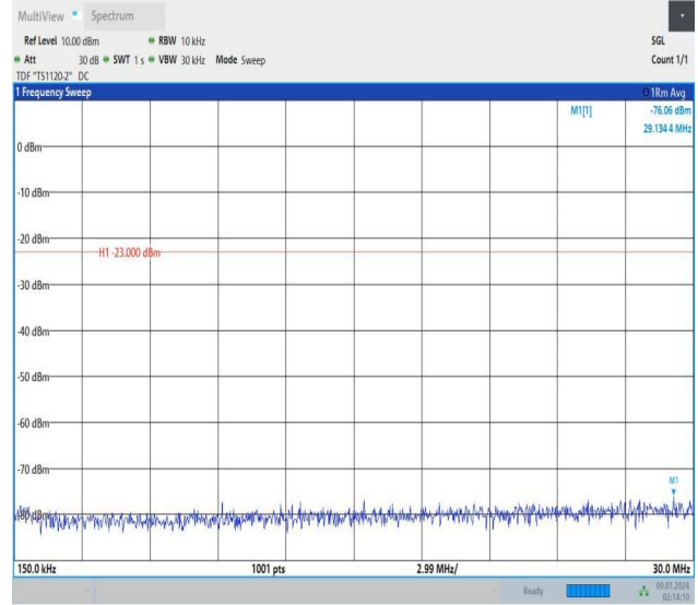
Band12_5MHz_QPSK_23155_1RB#0_0.15~30_0.15~30
