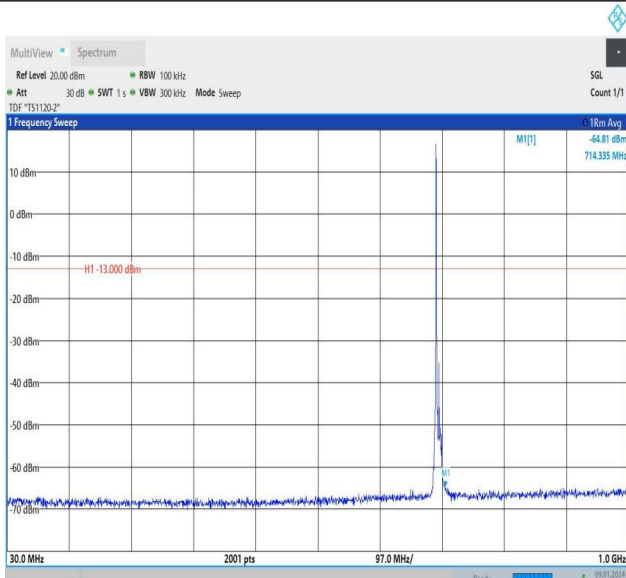
Band12_5MHz_QPSK_23035_1RB#0_30~1000_30~1000
