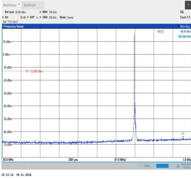
Band12_5MHz_QPSK_23095_1RB#0_30~1000_30~1000
