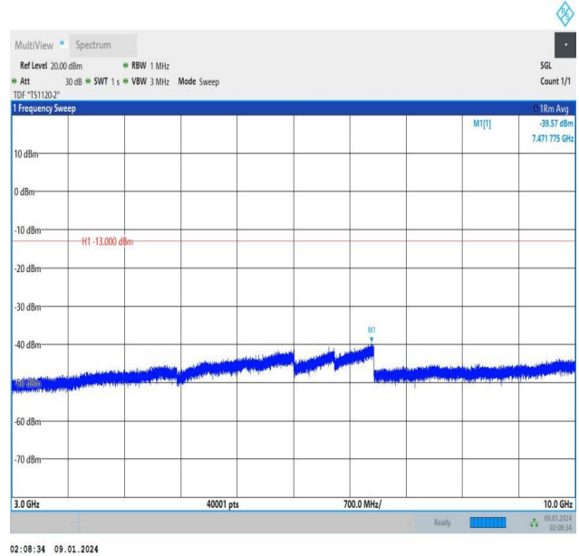
Band12_5MHz_16QAM_23035_1RB#24_3000~10000_3000~10000
