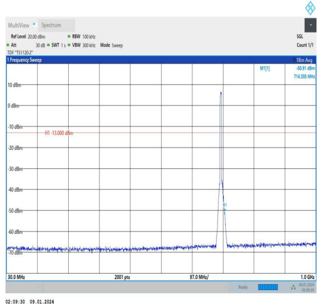
Band12_5MHz_16QAM_23035_25RB#0_30~1000_30~1000
