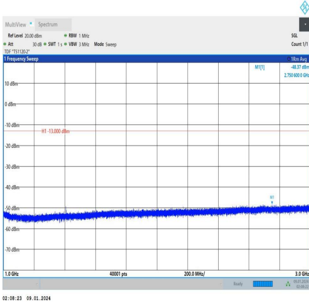
Band12_5MHz_16QAM_23035_1RB#24_1000~3000_1000~3000
