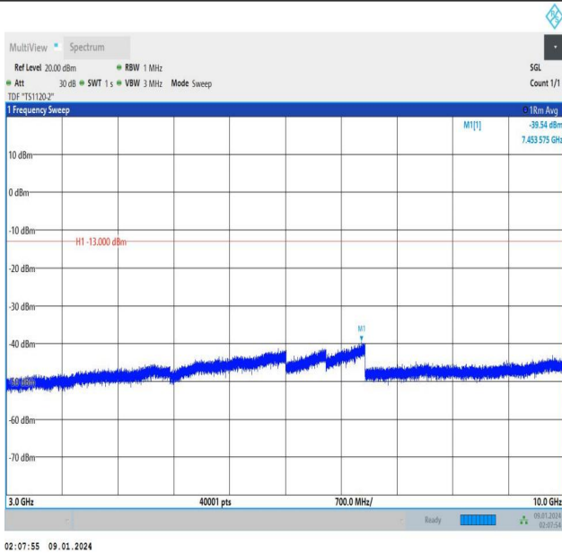
Band12_5MHz_QPSK_23035_1RB#24_3000~10000_3000~1 0000
