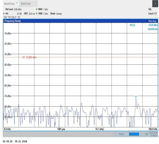
Band12_5MHz_16QAM_23035_25RB#0_0.009~0.15_0.009~0.15
