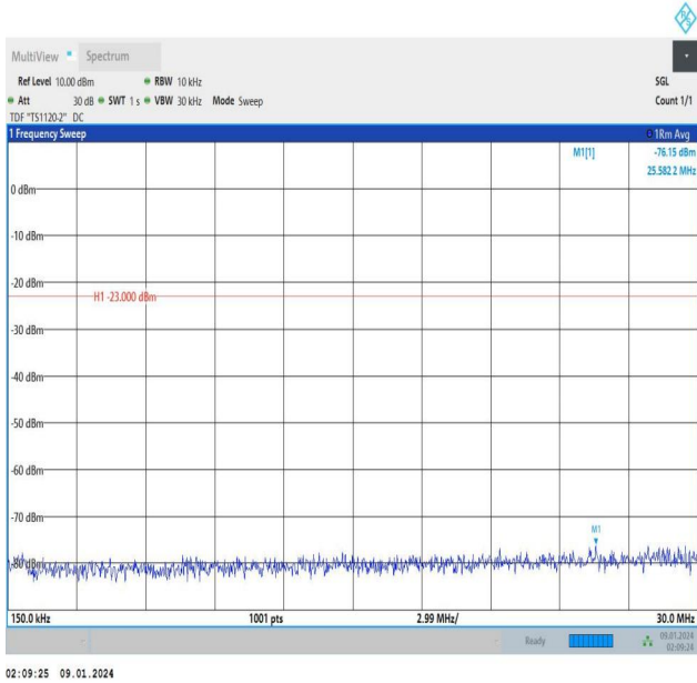
Band12_5MHz_16QAM_23035_25RB#0_0.15~30_0.15~30
