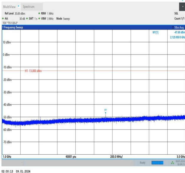
Band12_3MHz_16QAM_23095_1RB#14_1000~3000_1000~3000
