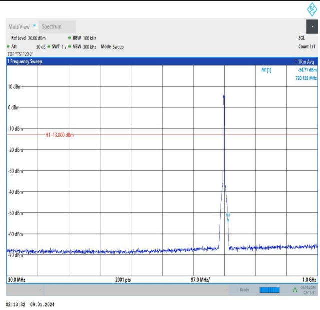
Band12_5MHz_16QAM_23095_25RB#0_30~1000_30~1000
