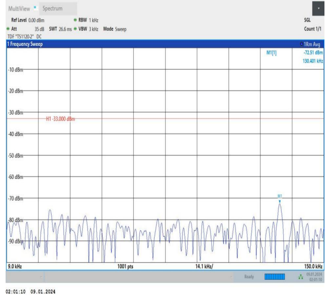
Band12_3MHz_16QAM_23095_15RB#0_0.009~0.15_0.009~0.15
