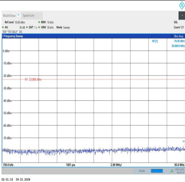
Band12_3MHz_16QAM_23095_15RB#0_0.15~30_0.15~30
