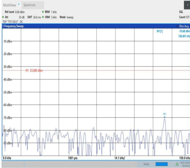
Band12_5MHz_QPSK_23035_1RB#0_0.009~0.15_0.009~0.1
