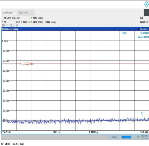
Band12_5MHz_16QAM_23155_1RB#0_0.15~30_0.15~30
