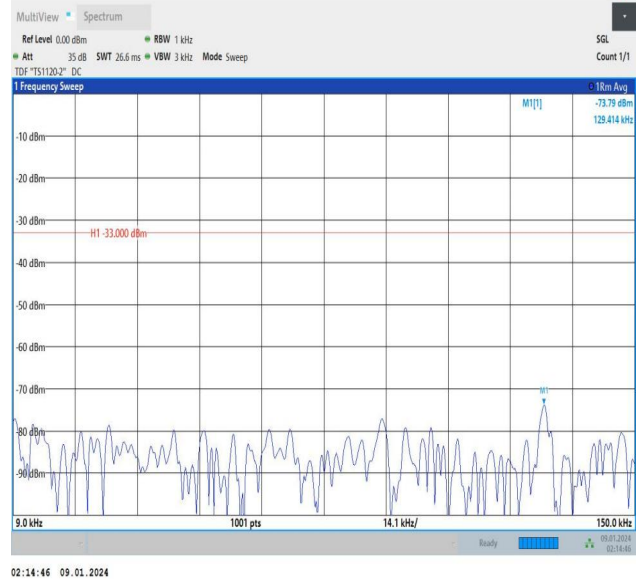
Band12_5MHz_16QAM_23155_1RB#0_0.009~0.15_0.009~0.15
