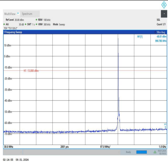
Band12_5MHz_16QAM_23155_1RB#0_30~1000_30~1000
