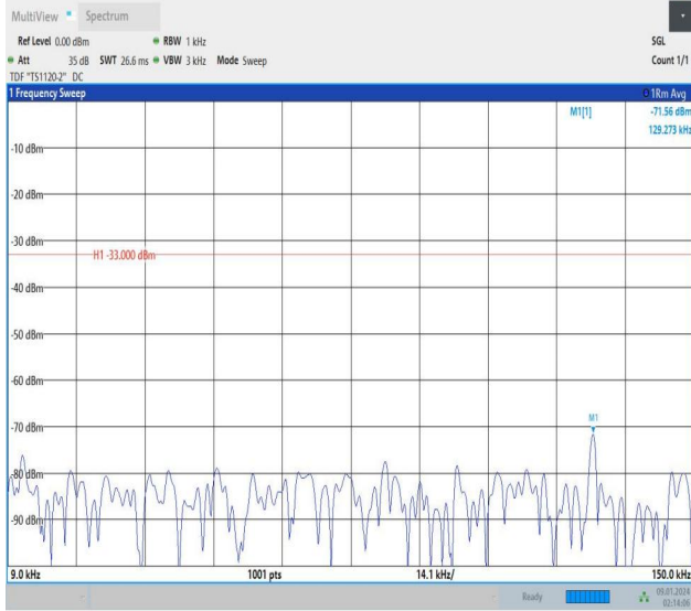
Band12_5MHz_QPSK_23155_1RB#0_0.009~0.15_0.009~0.1
