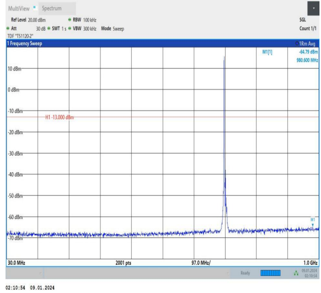
Band12_5MHz_16QAM_23095_1RB#0_30~1000_30~1000
