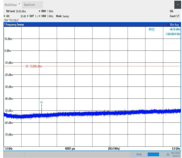
Band12_3MHz_QPSK_23165_1RB#0_1000~3000_1000~3000
