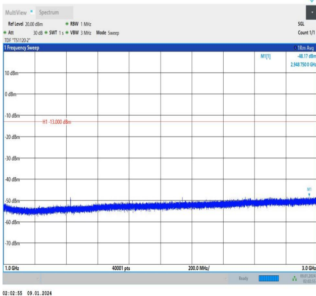
Band12_3MHz_16QAM_23165_1RB#0_1000~3000_1000~30
