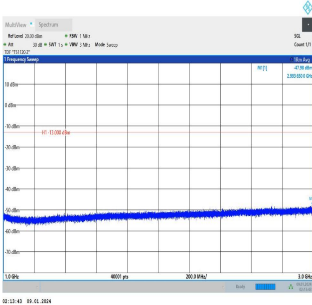
Band12_5MHz_16QAM_23095_25RB#0_1000~3000_1000~3000
