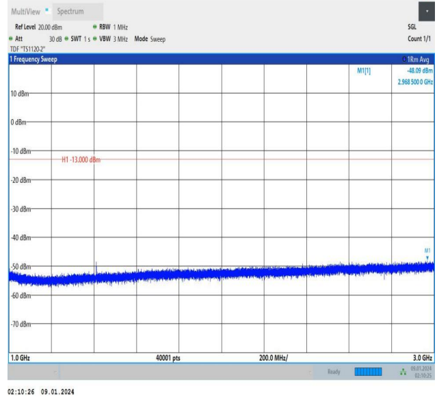
Band12_5MHz_QPSK_23095_1RB#0_1000~3000_1000~3000
