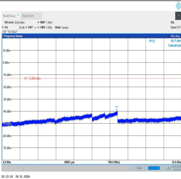
Band12_5MHz_QPSK_23095_25RB#0_3000~10000_3000~1 0000
