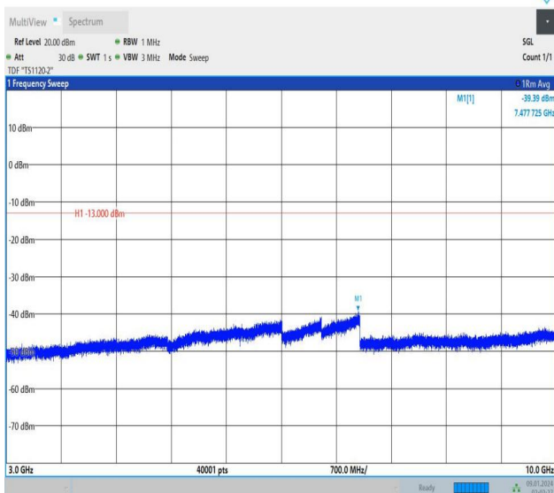
Band12_3MHz_QPSK_23165_1RB#0_3000~10000_3000~10000
