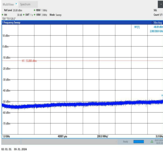
Band12_3MHz_16QAM_23095_15RB#0_1000~3000_1000~3000
