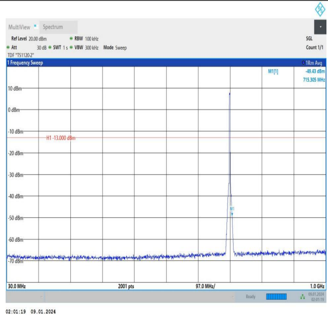
Band12_3MHz_16QAM_23095_15RB#0_30~1000_30~1000
