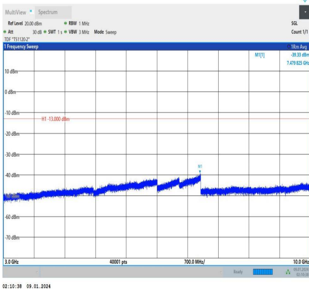
Band12_5MHz_QPSK_23095_1RB#0_3000~10000_3000~10000
