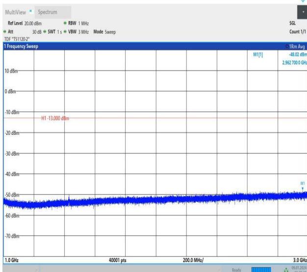
Band12_3MHz_16QAM_23165_15RB#0_1000~3000_1000~3000
