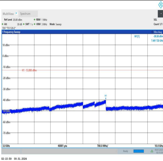
Band12_5MHz_QPSK_23155_1RB#24_3000~10000_3000~1 0000
