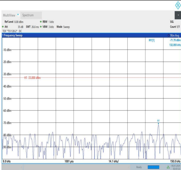
Band12_5MHz_QPSK_23035_1RB#24_0.009~0.15_0.009~0.
