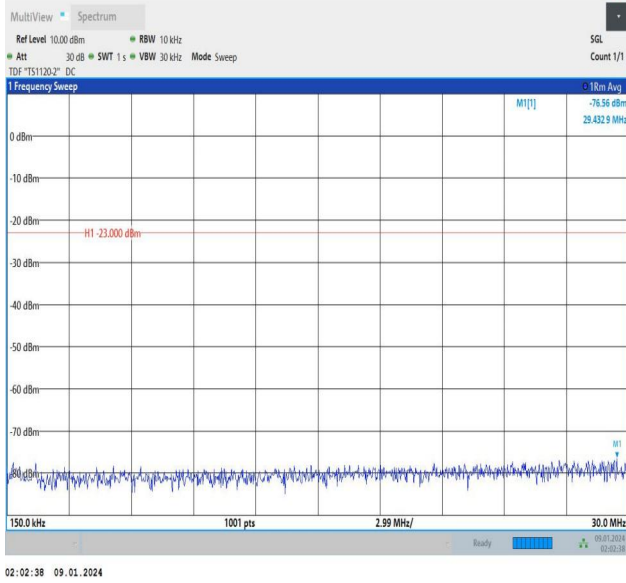
Band12_3MHz_16QAM_23165_1RB#0_0.15~30_0.15~30
