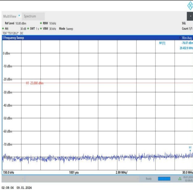
Band12_5MHz_16QAM_23035_1RB#24_0.15~30_0.15~30
