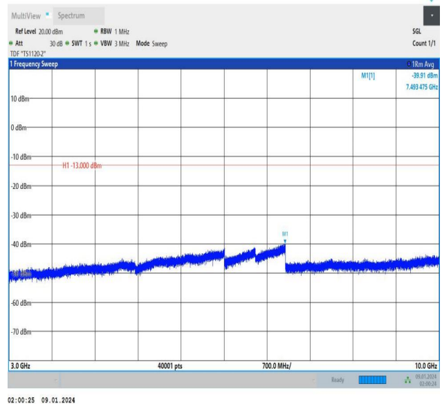
Band12_3MHz_16QAM_23095_1RB#14_3000~10000_3000~10000
