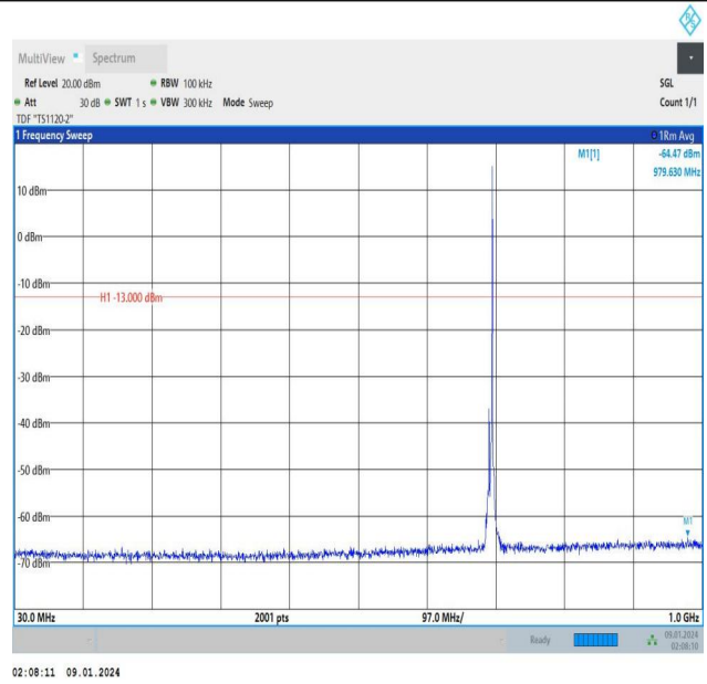
Band12_5MHz_16QAM_23035_1RB#24_30~1000_30~1000
