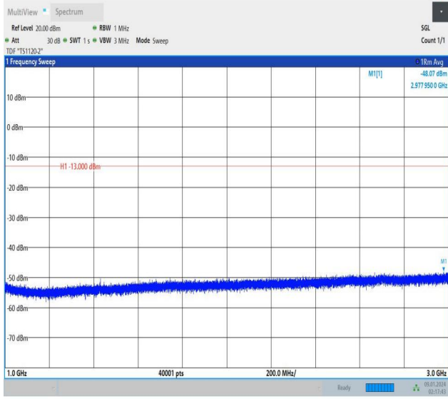
Band12_5MHz_16QAM_23155_25RB#0_1000~3000_1000~3000
