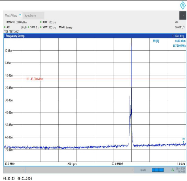
Band12_10MHz_16QAM_23060_1RB#49_30~1000_30~1000
