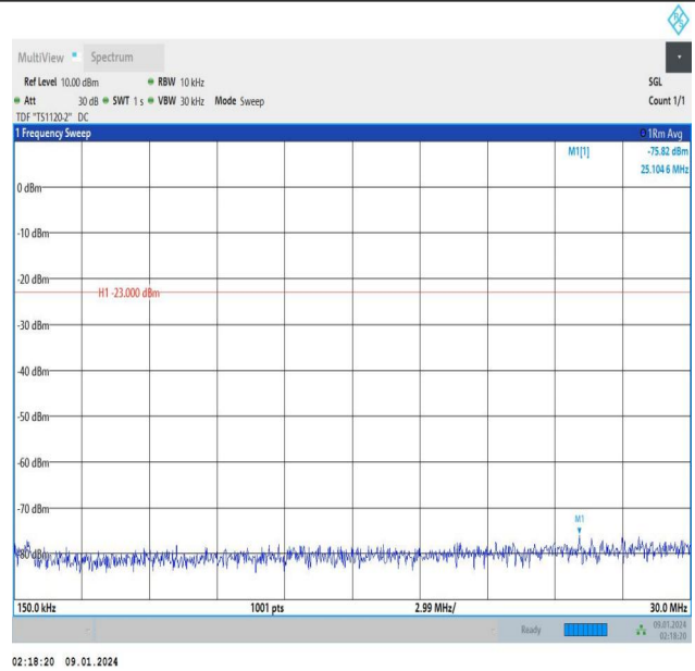
Band12_10MHz_QPSK_23060_1RB#0_0.15~30_0.15~30
