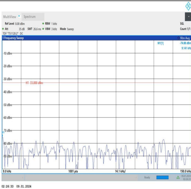
Band12_10MHz_QPSK_23060_50RB#0_0.009~0.15_0.009~0.15
