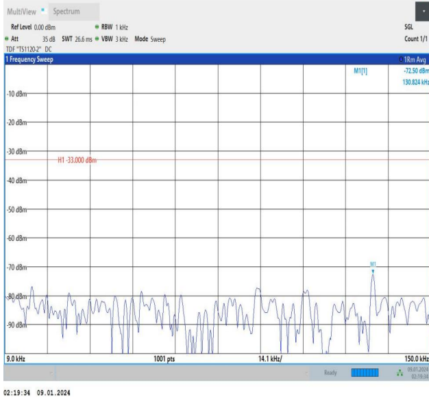
Band12_10MHz_QPSK_23060_1RB#49_0.009~0.15_0.009~0.15
