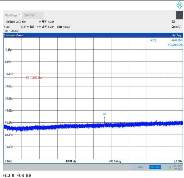
Band12_10MHz_QPSK_23060_1RB#49_1000~3000_1000~3000
