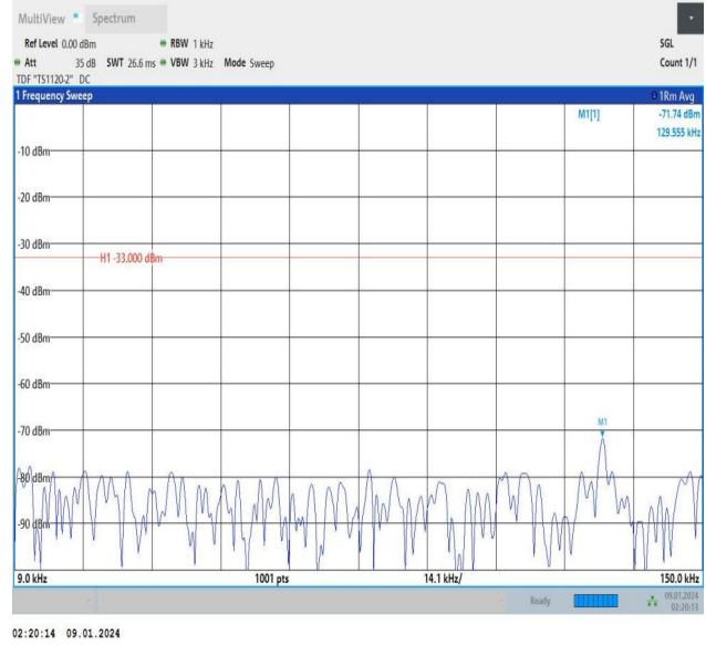
Band12_10MHz_16QAM_23060_1RB#49_0.009~0.15_0.009~0.15
