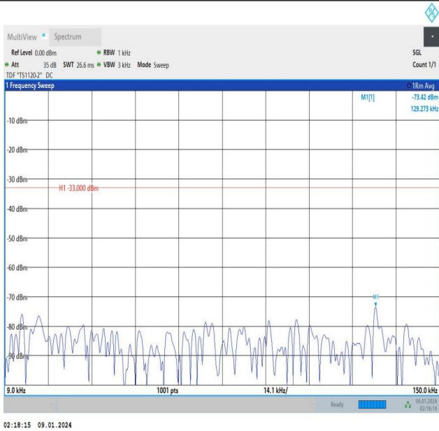
Band12_10MHz_QPSK_23060_1RB#0_0.009~0.15_0.009~0.15
