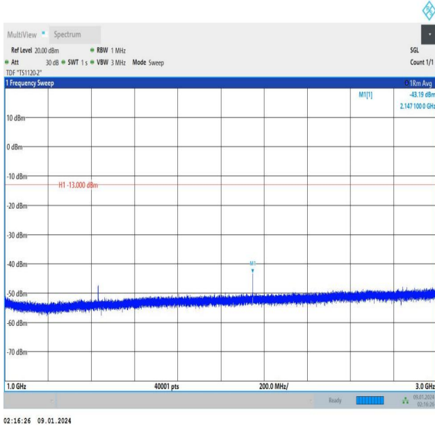
Band12_5MHz_16QAM_23155_1RB#24_1000~3000_1000~3000
