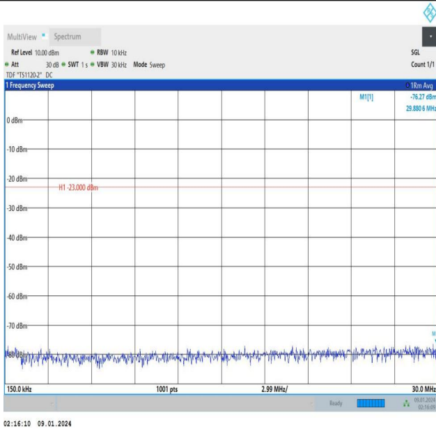
Band12_5MHz_16QAM_23155_1RB#24_0.15~30_0.15~30
