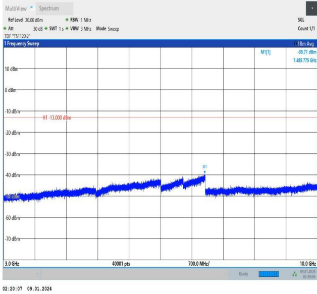
Band12_10MHz_QPSK_23060_1RB#49_3000~10000_3000~10000
