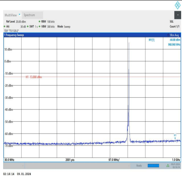
Band12_5MHz_16QAM_23155_1RB#24_30~1000_30~1000
