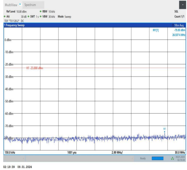
Band12_10MHz_QPSK_23060_1RB#49_0.15~30_0.15~30
