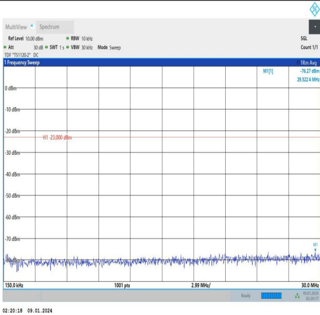
Band12_10MHz_16QAM_23060_1RB#49_0.15~30_0.15~30
