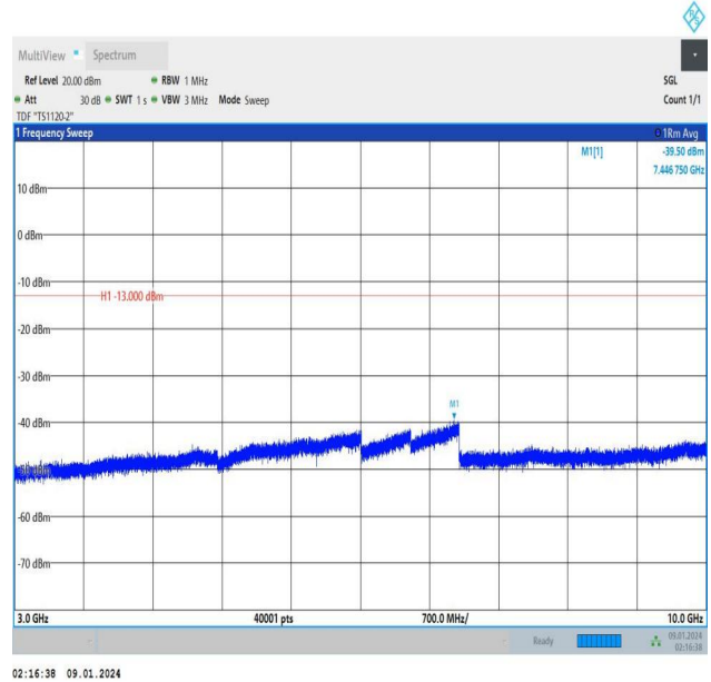
Band12_5MHz_16QAM_23155_1RB#24_3000~10000_3000~10000
