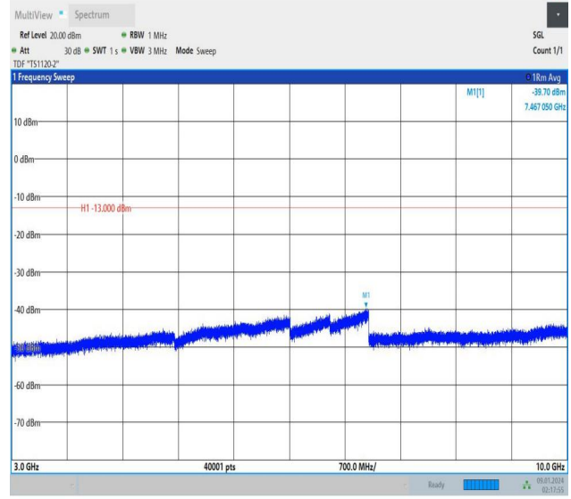
Band12_5MHz_16QAM_23155_25RB#0_3000~10000_3000~10000
