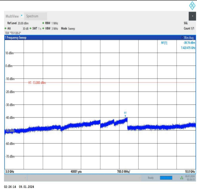
Band12_10MHz_16QAM_23130_1RB#49_3000~10000_3000~10000
