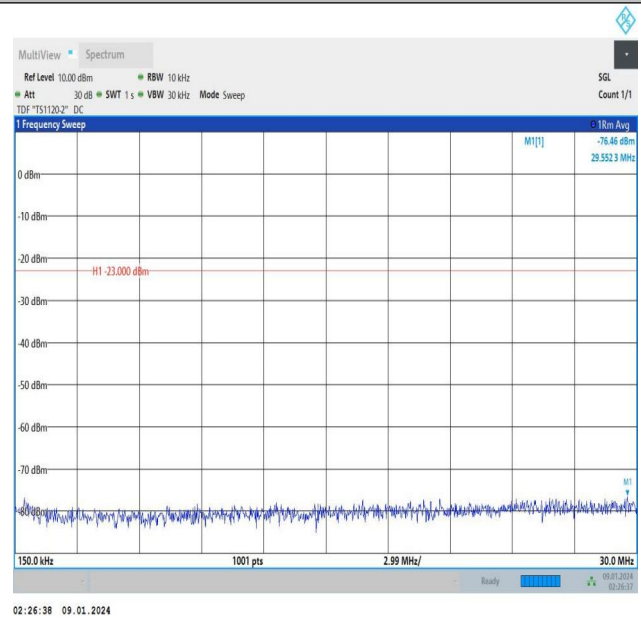
Band12_10MHz_QPSK_23060_50RB#0_0.15~30_0.15~30
