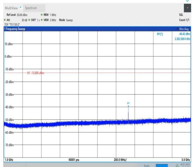
Band13_5MHz_QPSK_23205_1RB#0_1000~3000_1000~3000
