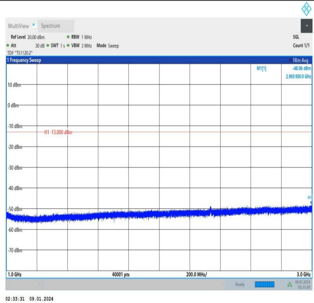
Band13_5MHz_QPSK_23205_25RB#0_1000~3000_1000~300
