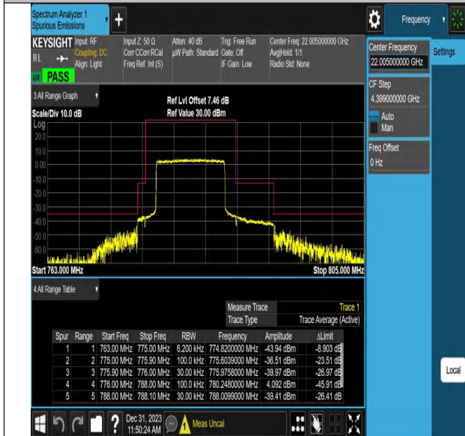
Band13_10MHz_QPSK_23230_50RB#0
