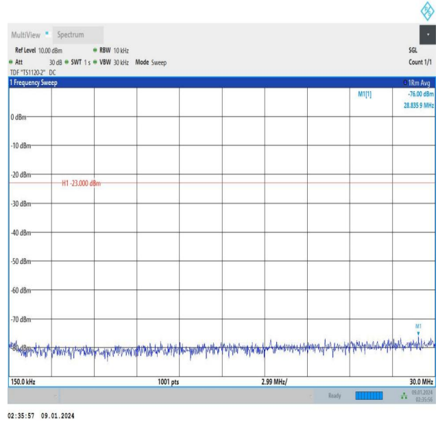
Band13_5MHz_QPSK_23230_1RB#24_0.15~30_0.15~30
