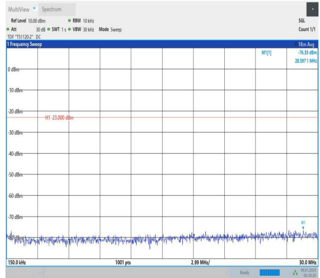
Band13_5MHz_QPSK_23205_1RB#0_0.15~30_0.15~30
