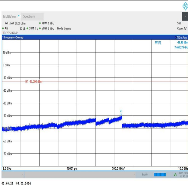
Band13_5MHz_QPSK_23255_1RB#24_3000~10000_3000~1
