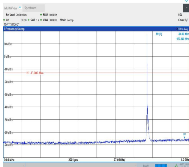
Band13_5MHz_QPSK_23205_1RB#0_30~1000_30~1000
