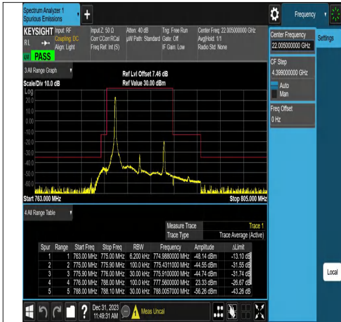
Band13_10MHz_QPSK_23230_1RB#0
