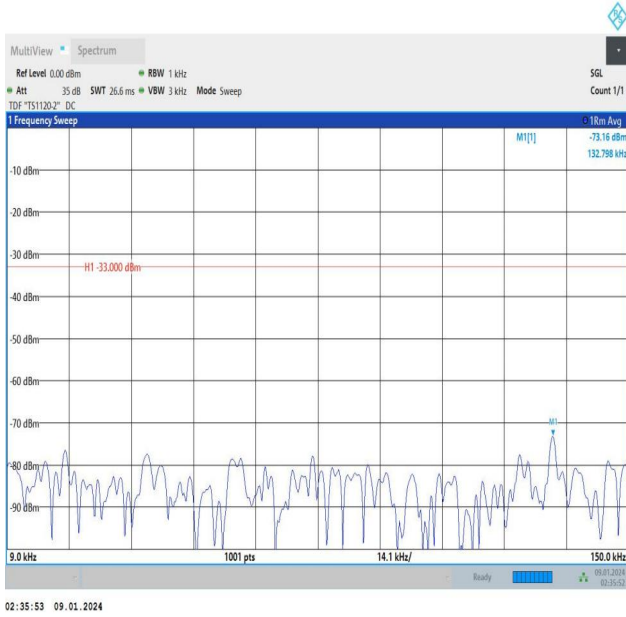
Band13_5MHz_QPSK_23230_1RB#24_0.009~0.15_0.009~0.
