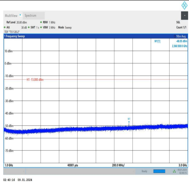
Band13_5MHz_QPSK_23255_1RB#24_1000~3000_1000~300
