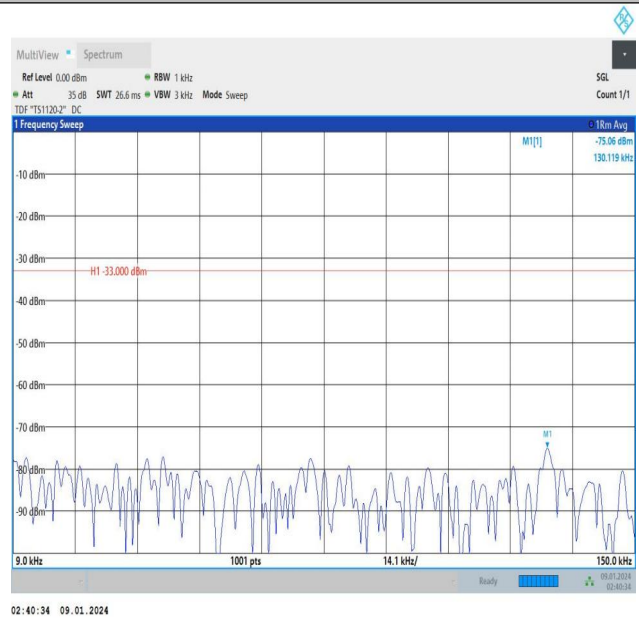
Band13_5MHz_16QAM_23255_1RB#24_0.009~0.15_0.009~0.
