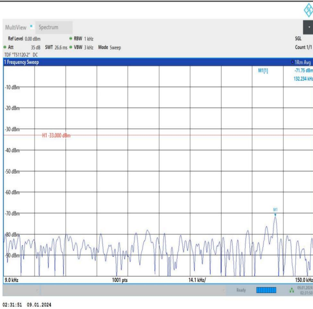
Band13_5MHz_QPSK_23205_1RB#24_0.009~0.15_0.009~0.15
