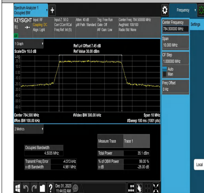
Band13-5MHz-QPSK-23255-25RB#0-PASS
