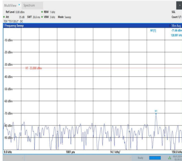
Band13_5MHz_QPSK_23205_1RB#0_0.009~0.15_0.009~0.15
