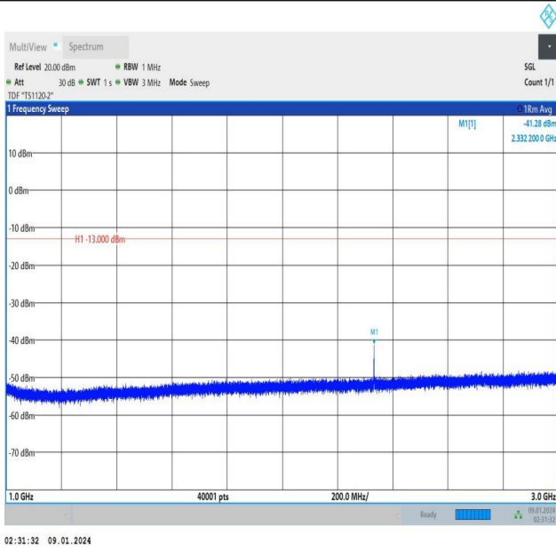
Band13_5MHz_16QAM_23205_1RB#0_1000~3000_1000~3000
