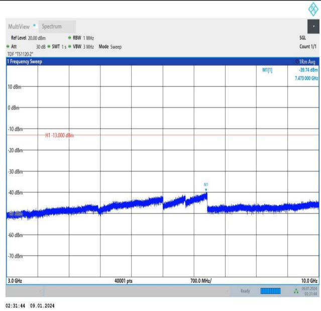
Band13_5MHz_16QAM_23205_1RB#0_3000~10000_3000~10000
