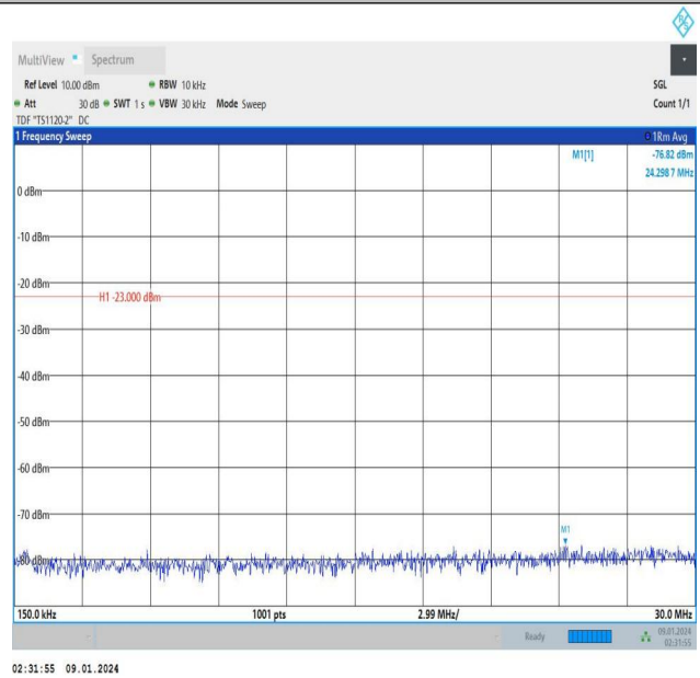
Band13_5MHz_QPSK_23205_1RB#24_0.15~30_0.15~30
