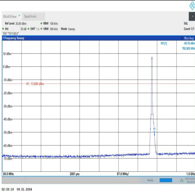
Band13_5MHz_QPSK_23205_25RB#0_30~1000_30~1000
