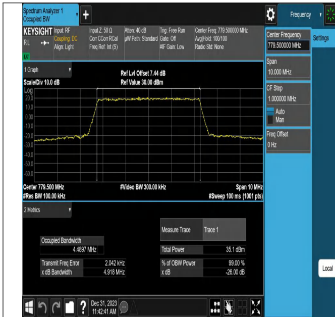
Band13-5MHz-QPSK-23205-25RB#0-PASS
