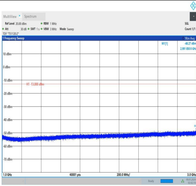
Band13_5MHz_16QAM_23255_25RB#0_1000~3000_1000~3000
