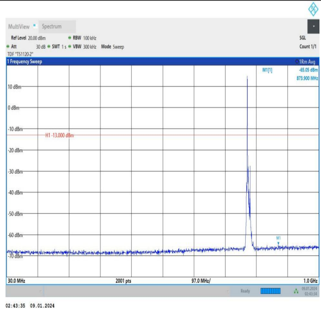
Band13_10MHz_16QAM_23230_1RB#0_30~1000_30~1000
