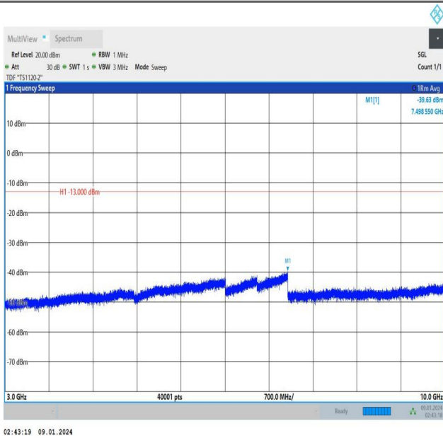
Band13_10MHz_QPSK_23230_1RB#0_3000~10000_3000~1 0000
