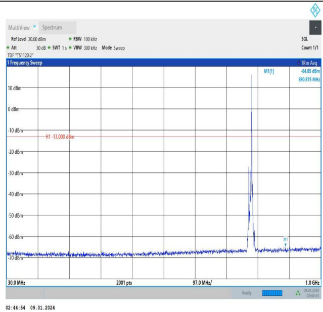
Band13_10MHz_16QAM_23230_1RB#49_30~1000_30~1000
