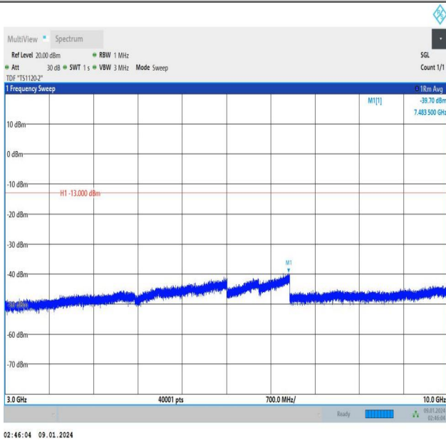
Band13_10MHz_QPSK_23230_50RB#0_3000~10000_3000~10000
