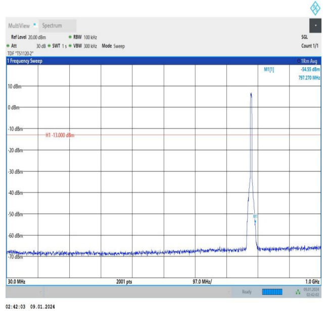
Band13_5MHz_16QAM_23255_25RB#0_30~1000_30~1000
