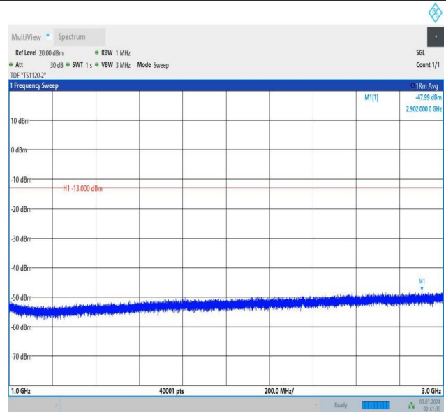
Band13_5MHz_QPSK_23255_25RB#0_1000~3000_1000~300
