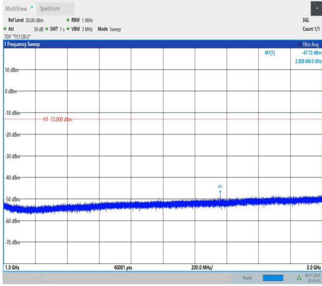
Band13_10MHz_16QAM_23230_1RB#49_1000~3000_1000~3000
