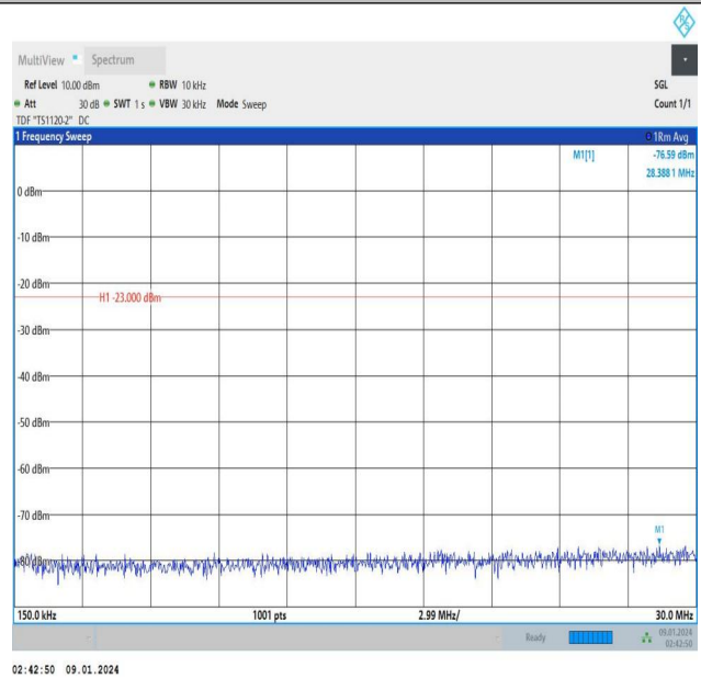
Band13_10MHz_QPSK_23230_1RB#0_0.15~30_0.15~30
