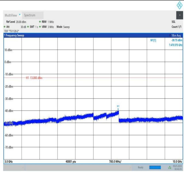
Band13_5MHz_16QAM_23255_25RB#0_3000~10000_3000~10000
