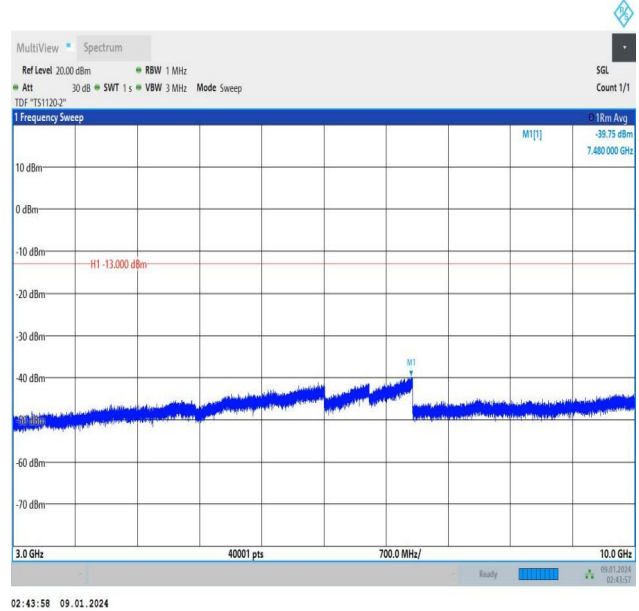
Band13_10MHz_16QAM_23230_1RB#0_3000~10000_3000~10000
