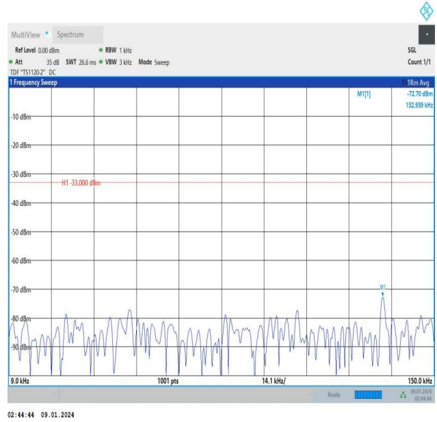
Band13_10MHz_16QAM_23230_1RB#49_0.009~0.15_0.009~0.15
