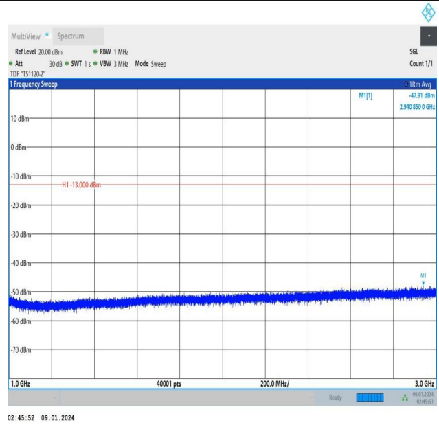
Band13_10MHz_QPSK_23230_50RB#0_1000~3000_1000~3000 00
