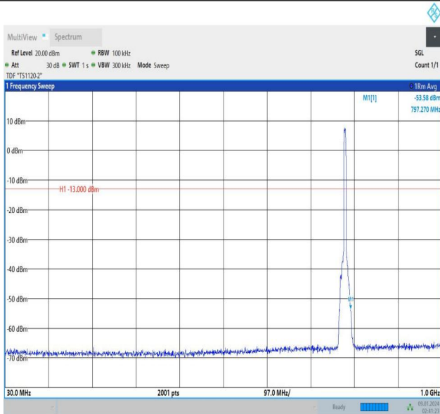
Band13_5MHz_QPSK_23255_25RB#0_30~1000_30~1000
