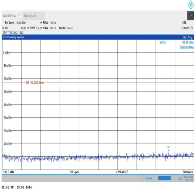
Band13_5MHz_16QAM_23255_25RB#0_0.15~30_0.15~30
