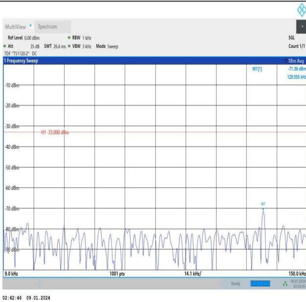
Band13_10MHz_QPSK_23230_1RB#0_0.009~0.15_0.009~0.15
