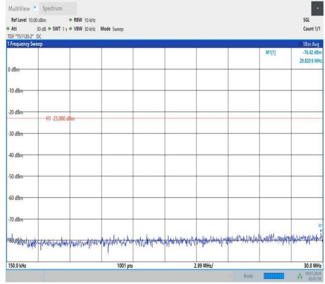
Band13_5MHz_QPSK_23255_25RB#0_0.15~30_0.15~30
