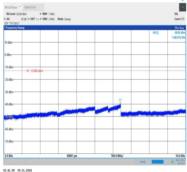
Band13_5MHz_16QAM_23255_1RB#24_3000~10000_3000~10000
