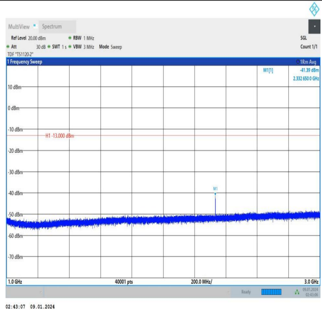
Band13_10MHz_QPSK_23230_1RB#0_1000~3000_1000~300 0
