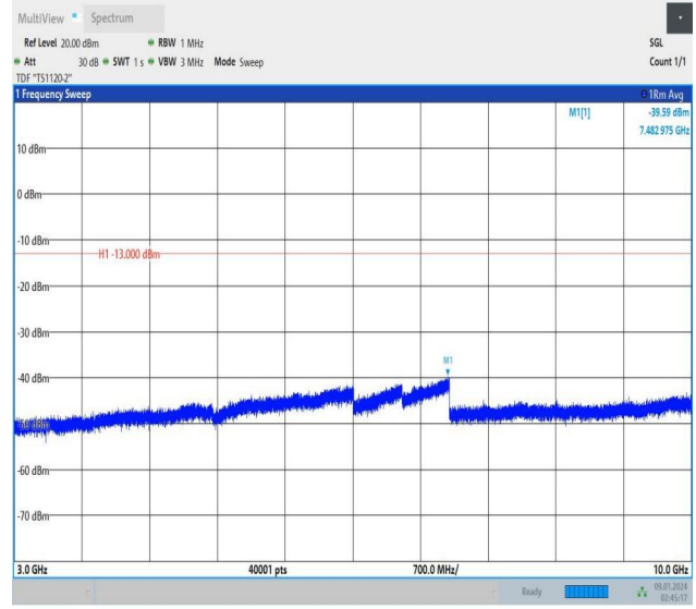
Band13_10MHz_16QAM_23230_1RB#49_3000~10000_3000~10000
