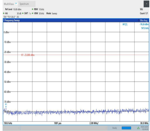
Band13_10MHz_QPSK_23230_1RB#49_0.15~30_0.15~30
