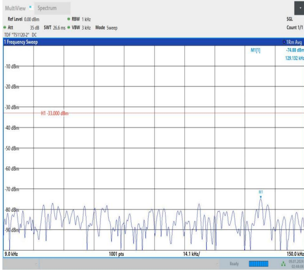
Band13_10MHz_QPSK_23230_1RB#49_0.009~0.15_0.009~0.15
