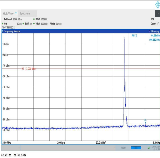
Band13_10MHz_QPSK_23230_1RB#0_30~1000_30~1000
