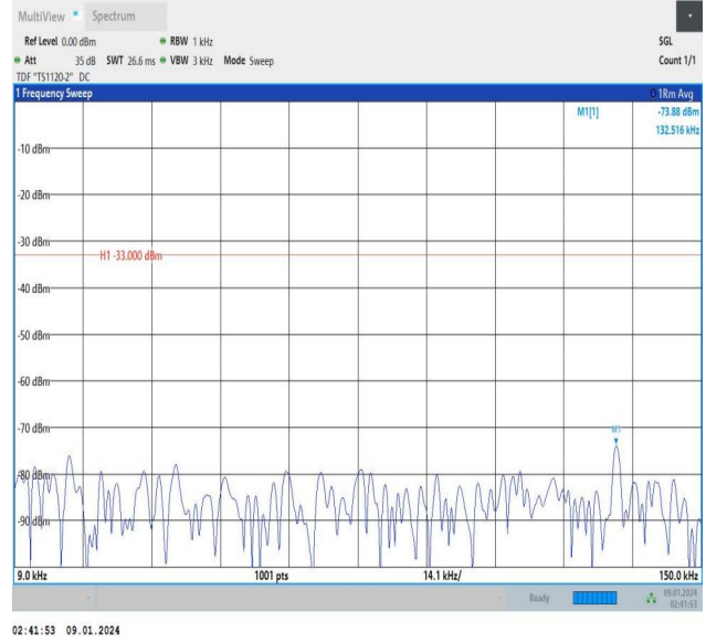
Band13_5MHz_16QAM_23255_25RB#0_0.009~0.15_0.009~0.15
