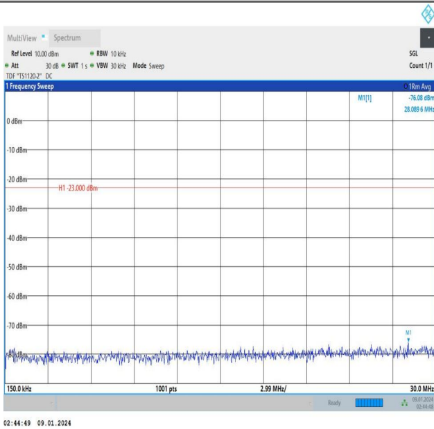
Band13_10MHz_16QAM_23230_1RB#49_0.15~30_0.15~30
