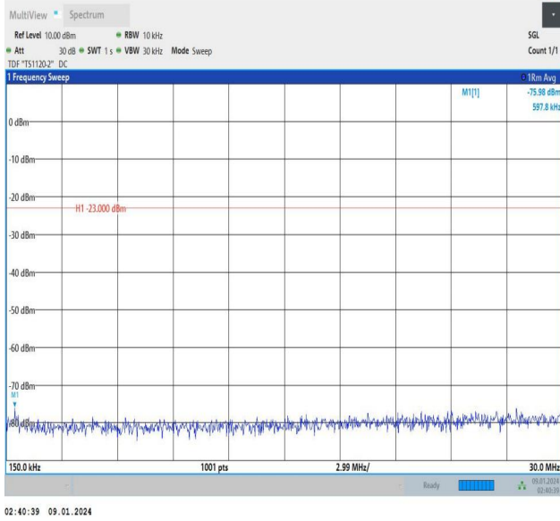
Band13_5MHz_16QAM_23255_1RB#24_0.15~30_0.15~30
