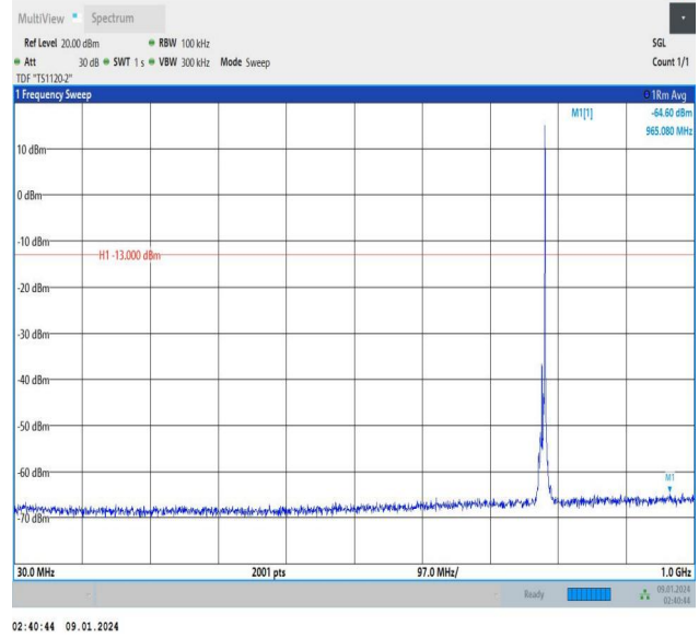
Band13_5MHz_16QAM_23255_1RB#24_30~1000_30~1000
