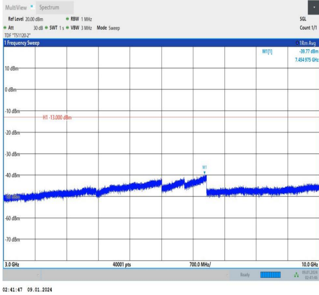
Band13_5MHz_QPSK_23255_25RB#0_3000~10000_3000~10000
