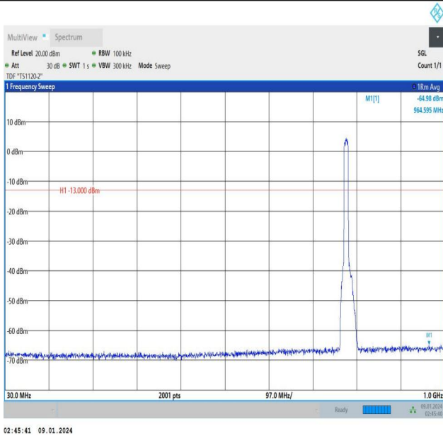
Band13_10MHz_QPSK_23230_50RB#0_30~1000_30~1000
