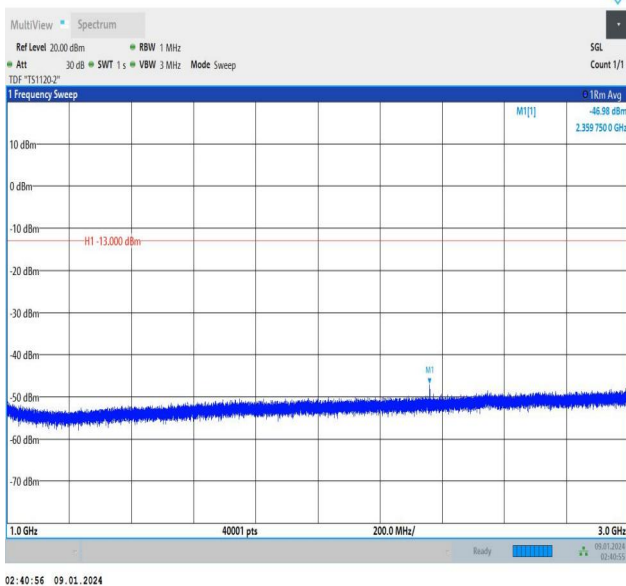
Band13_5MHz_16QAM_23255_1RB#24_1000~3000_1000~3000
