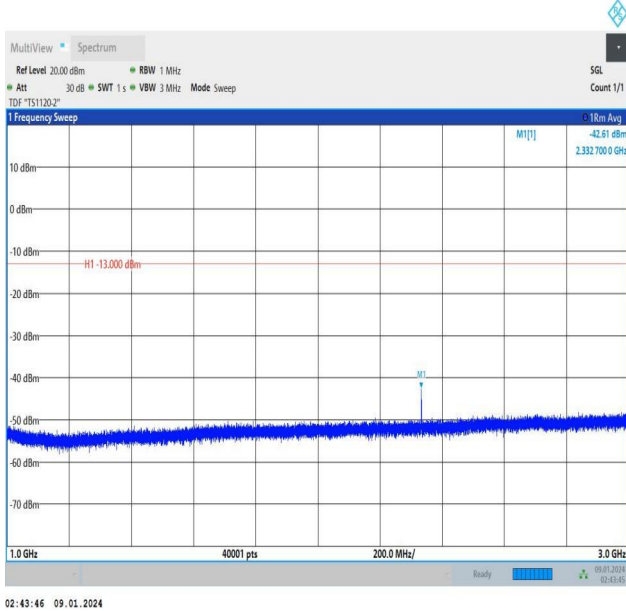
Band13_10MHz_16QAM_23230_1RB#0_1000~3000_1000~3000
