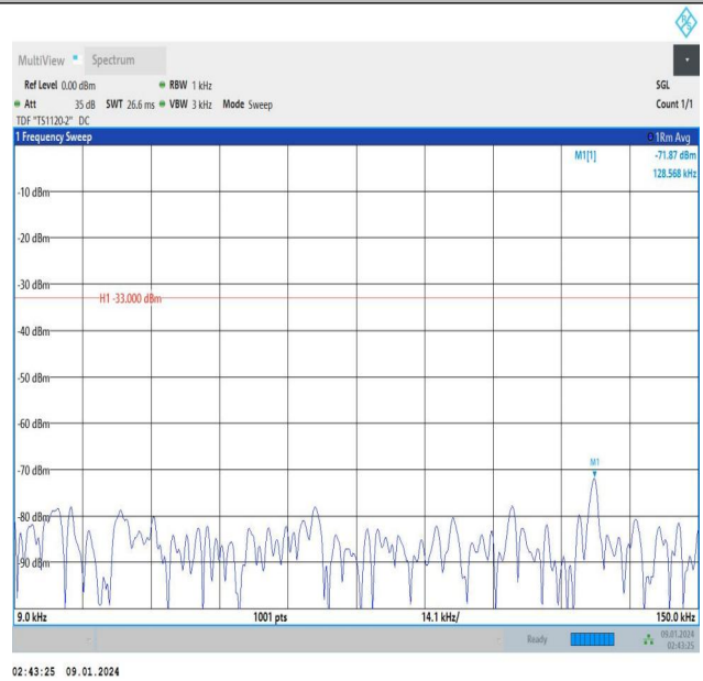
Band13_10MHz_16QAM_23230_1RB#0_0.009~0.15_0.009~0. 15
