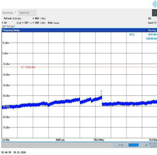
Band13_10MHz_QPSK_23230_1RB#49_3000~10000_3000~10000
