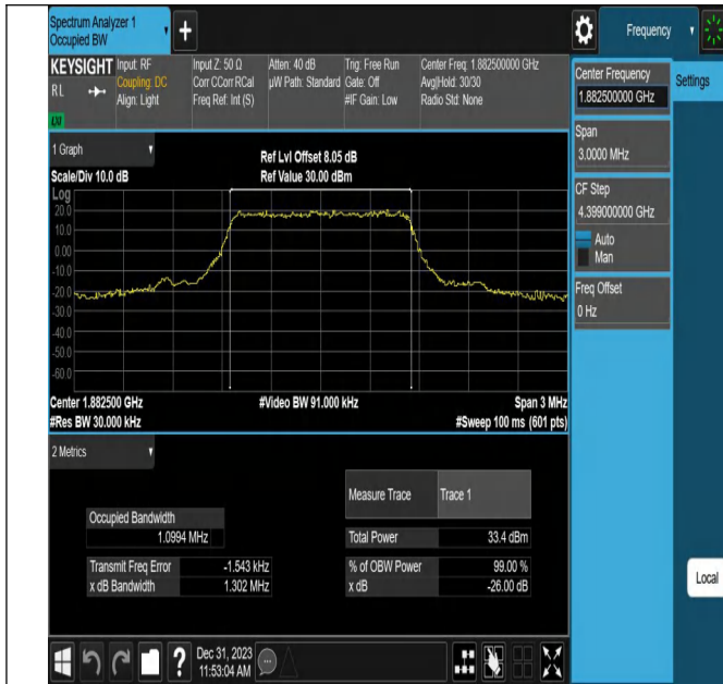
Band25-1.4MHz-16QAM-26365-6RB#0-PASS
