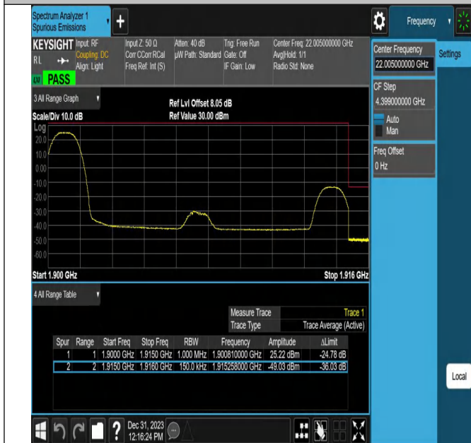
Band25_15MHz_16QAM_26615_1RB#0
