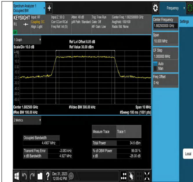
Band25-5MHz-16QAM-26365-25RB#0-PASS
