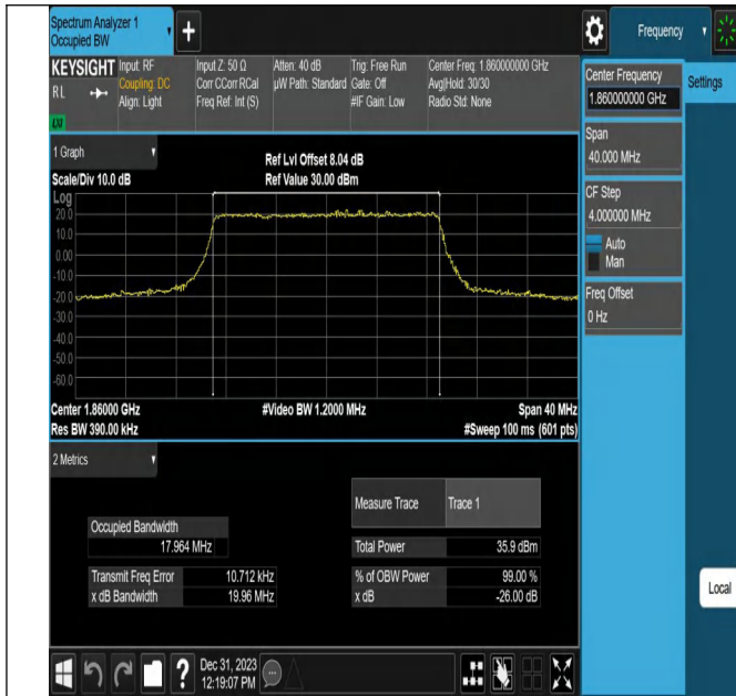
Band25-20MHz-QPSK-26140-100RB#0-PASS
