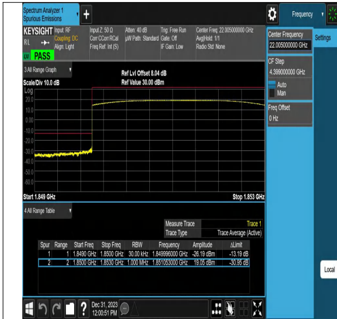
Band25_3MHz_16QAM_26055_15RB#0
