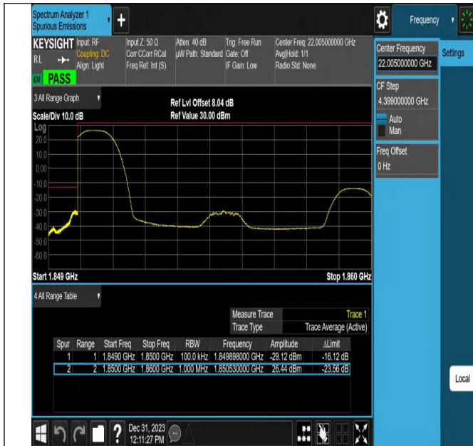
Band25_10MHz_QPSK_26090_1RB#0
