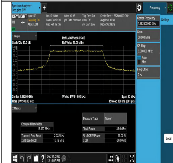
Band25-15MHz-QPSK-26365-75RB#0-PASS
