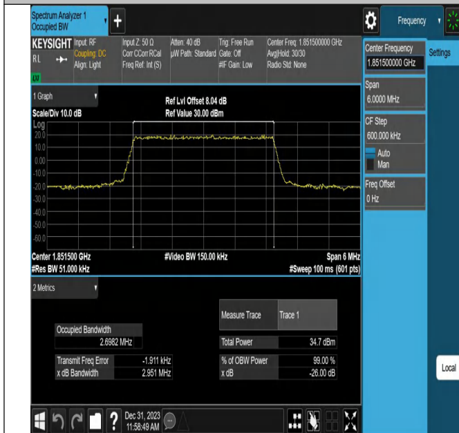
Band25-3MHz-QPSK-26055-15RB#0-PASS
