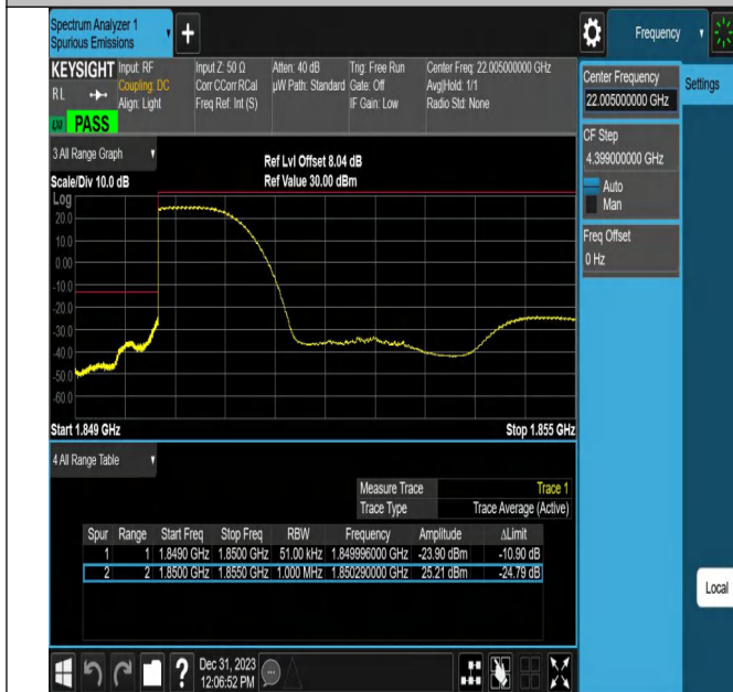
Band25_5MHz_16QAM_26065_1RB#0
