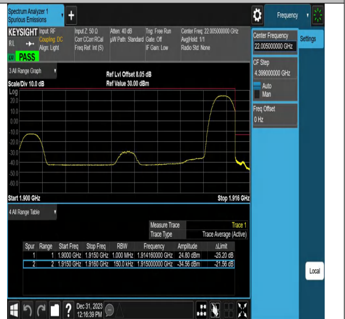
Band25_15MHz_16QAM_26615_1RB#74
