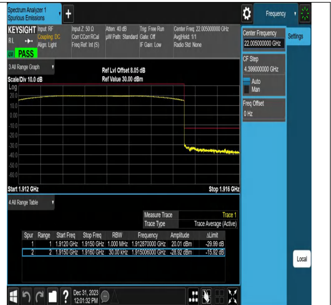
Band25_3MHz_QPSK_26675_15RB#0
