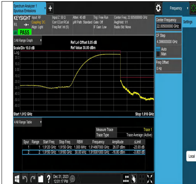
Band25_3MHz_QPSK_26675_1RB#14
