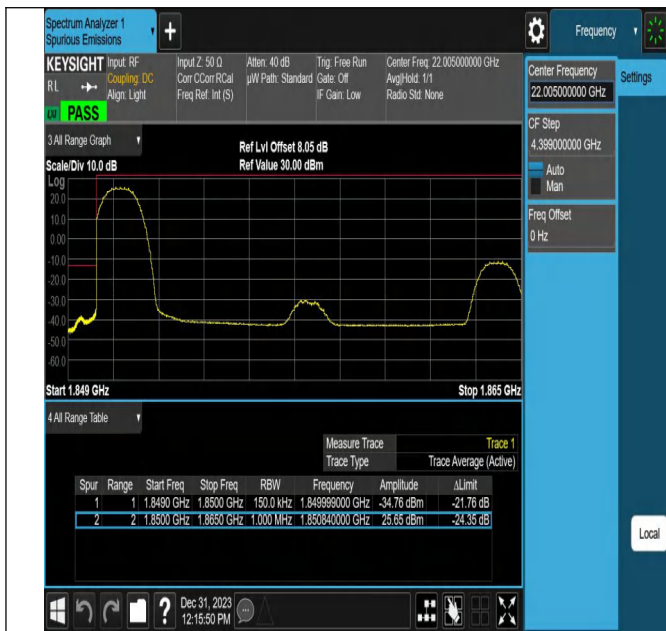
Band25_15MHz_16QAM_26115_1RB#0
