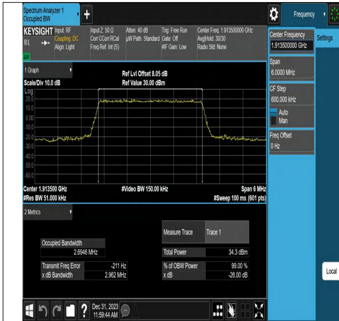
Band25-3MHz-QPSK-26675-15RB#0-PASS
