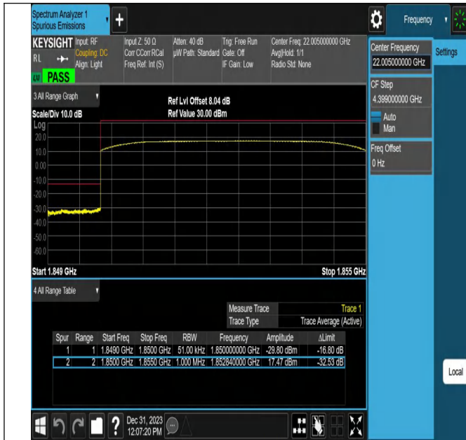
Band25_5MHz_16QAM_26065_25RB#0
