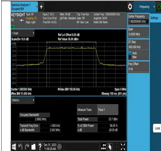
Band25-3MHz-16QAM-26365-15RB#0-PASS
