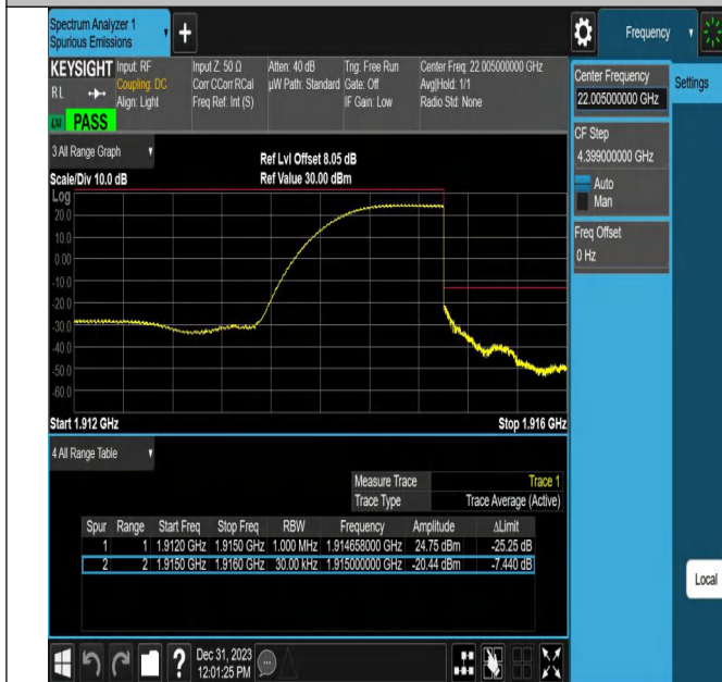
Band25_3MHz_16QAM_26675_1RB#14
