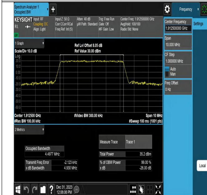
Band25-5MHz-QPSK-26665-25RB#0-PASS
