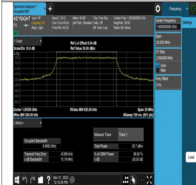
Band25-10MHz-QPSK-26090-50RB#0-PASS
