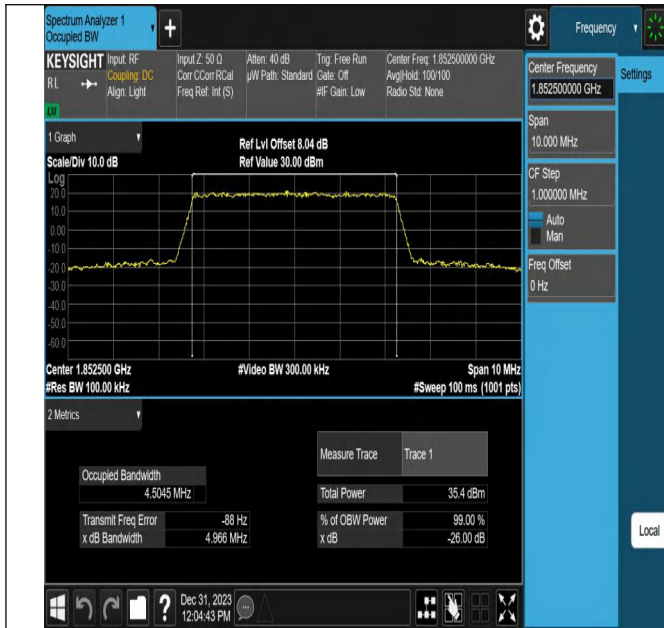
Band25-5MHz-QPSK-26065-25RB#0-PASS
