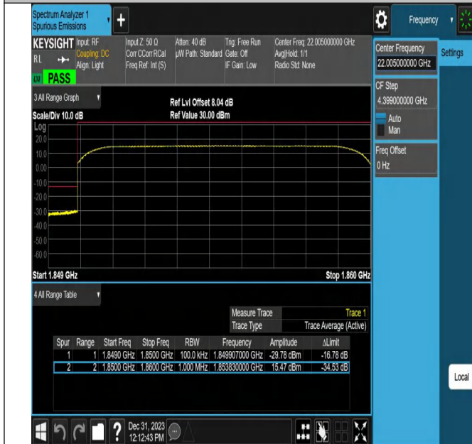
Band25_10MHz_QPSK_26090_50RB#0
