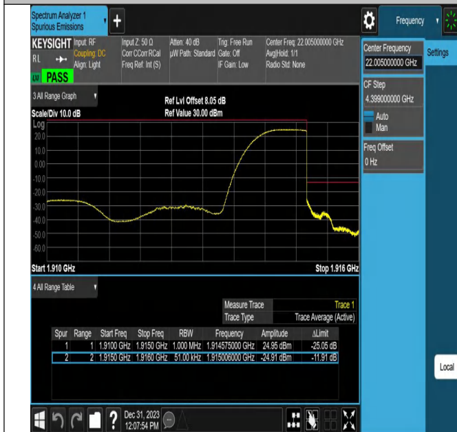
Band25_5MHz_16QAM_26665_1RB#24
