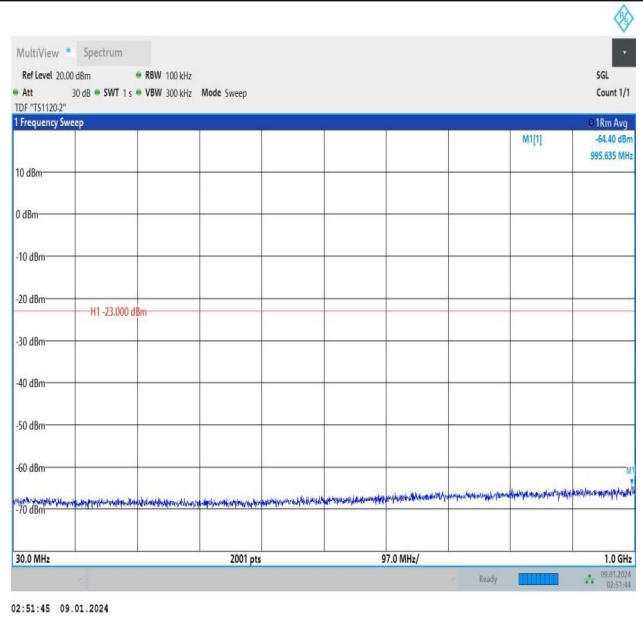
Band25_1.4MHz_16QAM_26365_1RB#0_30~1000_30~1000
