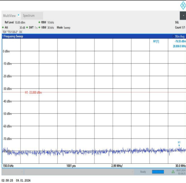
Band25_1.4MHz_16QAM_26683_6RB#0_0.15~30_0.15~30
