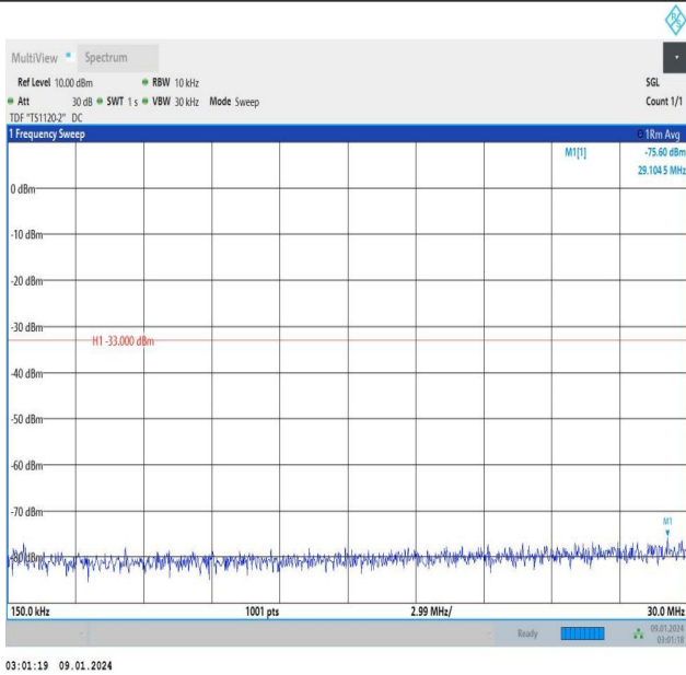
Band25_3MHz_16QAM_26055_1RB#14_0.15~30_0.15~30
