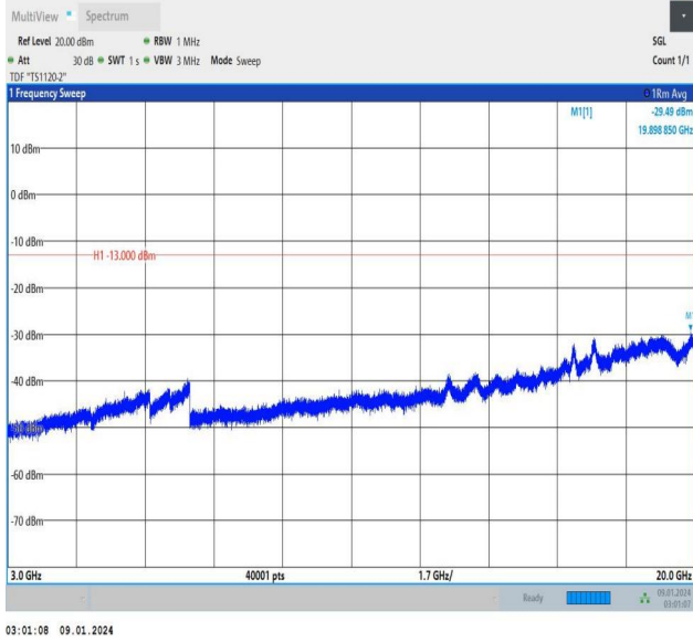
Band25_3MHz_QPSK_26055_1RB#14_3000~20000_3000~20000
