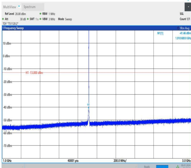
Band25_1.4MHz_16QAM_26683_1RB#5_1000~3000_1000~3000
