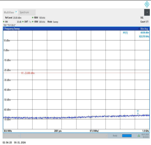
Band25_1.4MHz_16QAM_26365_6RB#0_30~1000_30~1000
