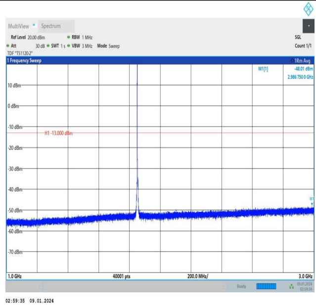
Band25_3MHz_QPSK_26055_1RB#0_1000~3000_1000~300
