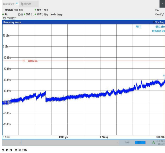
Band25_1.4MHz_QPSK_26047_1RB#0_3000~20000_3000~20000
