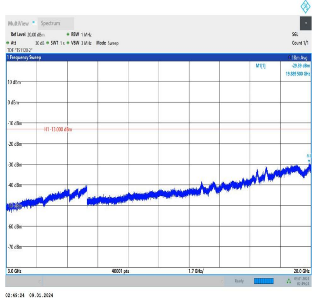
Band25_1.4MHz_16QAM_26047_1RB#5_3000~20000_3000~20000
