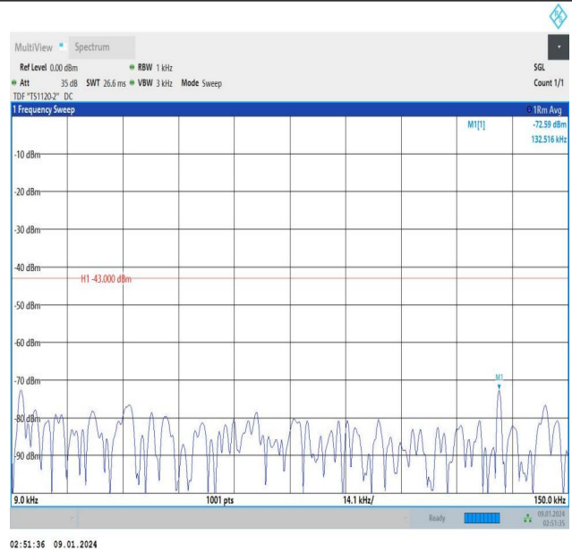
Band25_1.4MHz_16QAM_26365_1RB#0_0.009~0.15_0.009~0.15
