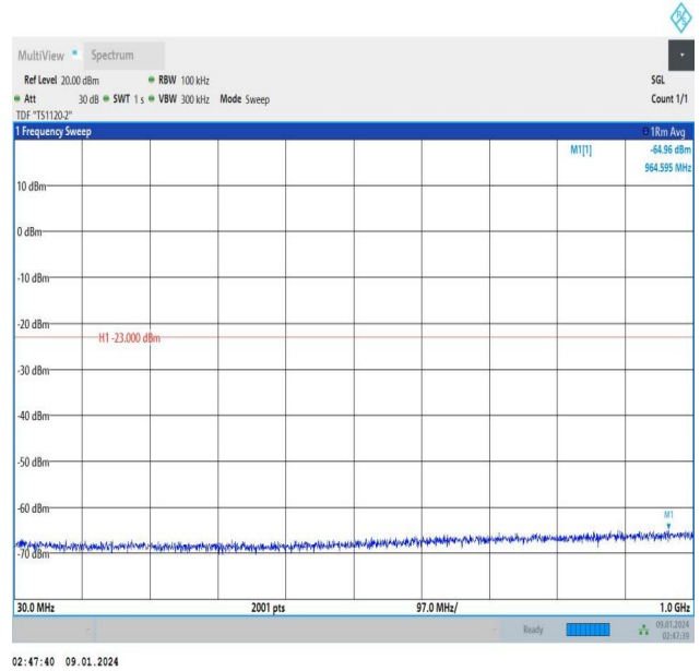
Band25_1.4MHz_16QAM_26047_1RB#0_30~1000_30~1000
