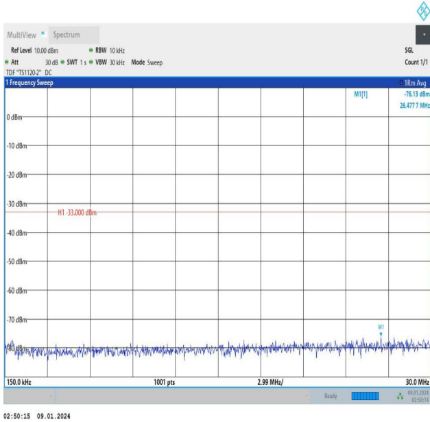
Band25_1.4MHz_16QAM_26047_6RB#0_0.15~30_0.15~30
