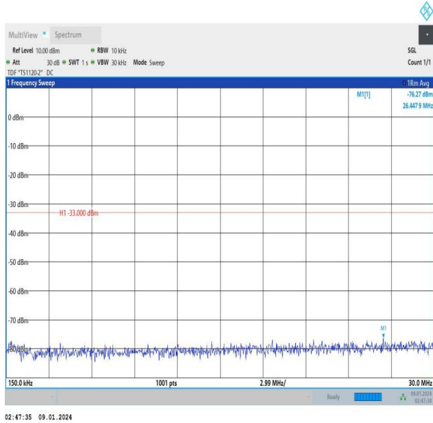
Band25_1.4MHz_16QAM_26047_1RB#0_0.15~30_0.15~30
