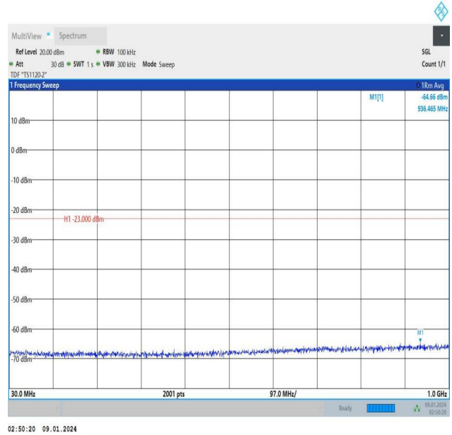
Band25_1.4MHz_16QAM_26047_6RB#0_30~1000_30~1000
