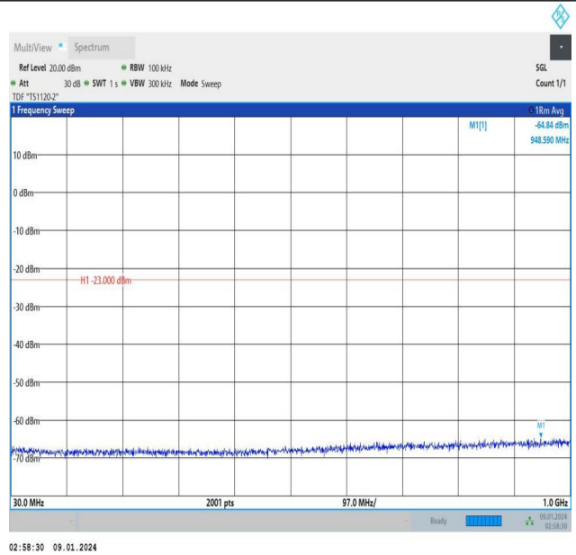
Band25_1.4MHz_16QAM_26683_6RB#0_30~1000_30~1000
