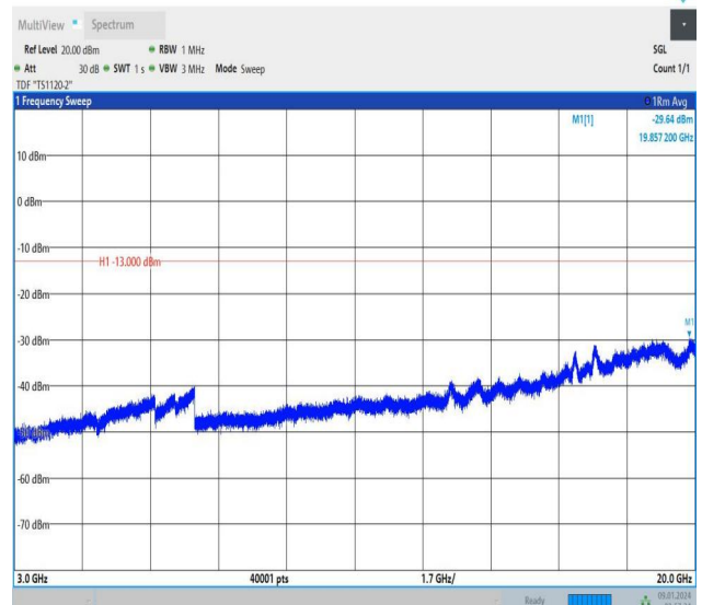
Band25_1.4MHz_16QAM_26683_1RB#5_3000~20000_3000~20000
