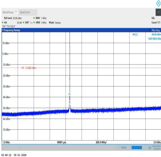
Band25_1.4MHz_16QAM_26047_1RB#5_1000~3000_1000~3000
