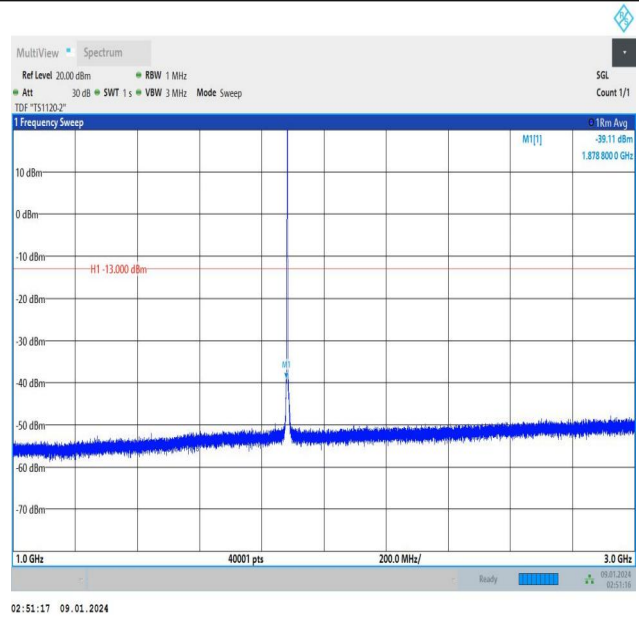
Band25_1.4MHz_QPSK_26365_1RB#0_1000~3000_1000~3000 00
