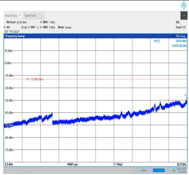
Band25_1.4MHz_16QAM_26683_6RB#0_3000~20000_3000~20000
