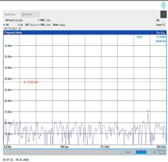
Band25_1.4MHz_16QAM_26683_1RB#5_0.009~0.15_0.009~0.15
