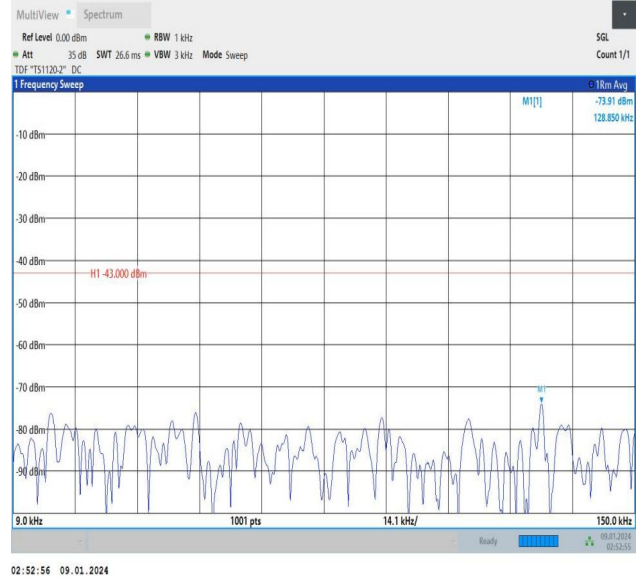
Band25_1.4MHz_16QAM_26365_1RB#5_0.009~0.15_0.009~0.15
