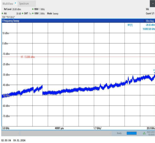
Band25_1.4MHz_QPSK_26047_6RB#0_3000~20000_3000~20000
