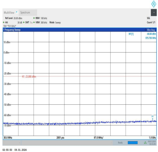
Band25_1.4MHz_16QAM_26683_1RB#0_30~1000_30~1000
