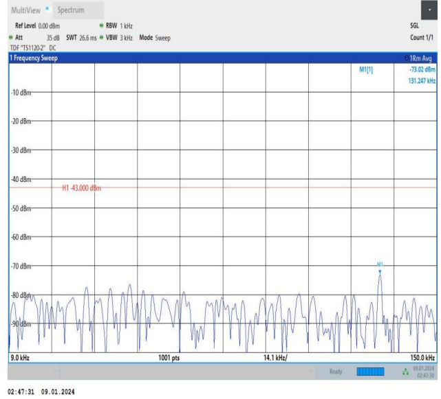
Band25_1.4MHz_16QAM_26047_1RB#0_0.009~0.15_0.009~0.15
