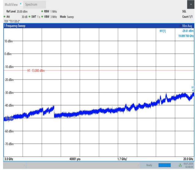
Band25_1.4MHz_16QAM_26047_1RB#0_3000~20000_3000~20000
