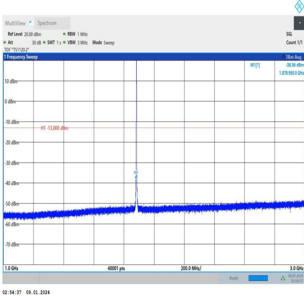
Band25_1.4MHz_16QAM_26365_6RB#0_1000~3000_1000~3000
