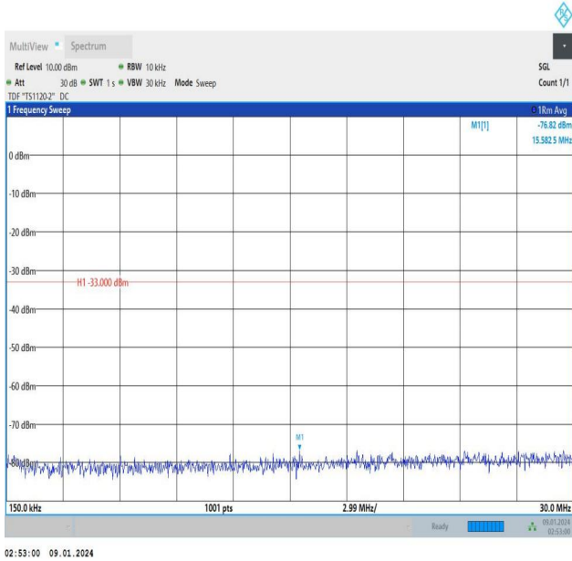
Band25_1.4MHz_16QAM_26365_1RB#5_0.15~30_0.15~30
