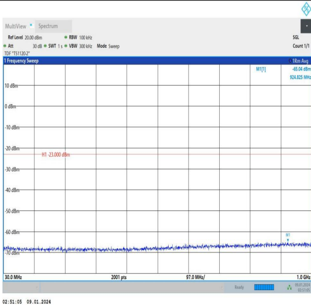
Band25_1.4MHz_QPSK_26365_1RB#0_30~1000_30~1000
