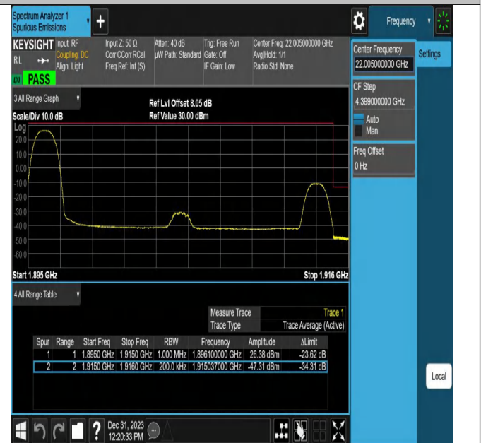
Band25_20MHz_QPSK_26590_1RB#0
