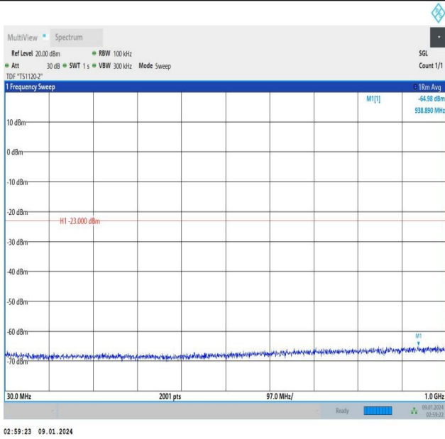
Band25_3MHz_QPSK_26055_1RB#0_30~1000_30~1000
