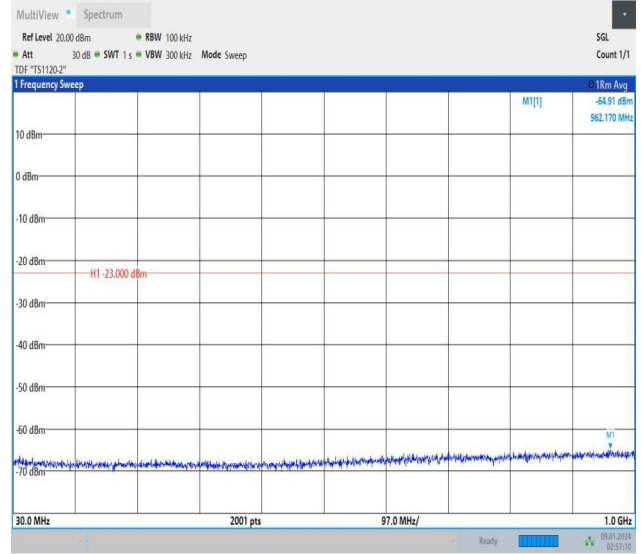
Band25_1.4MHz_16QAM_26683_1RB#5_30~1000_30~1000
