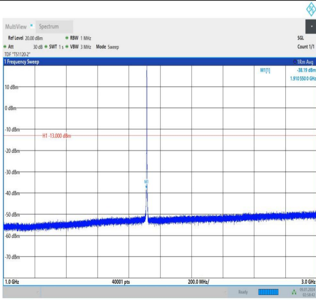
Band25_1.4MHz_16QAM_26683_6RB#0_1000~3000_1000~3000
