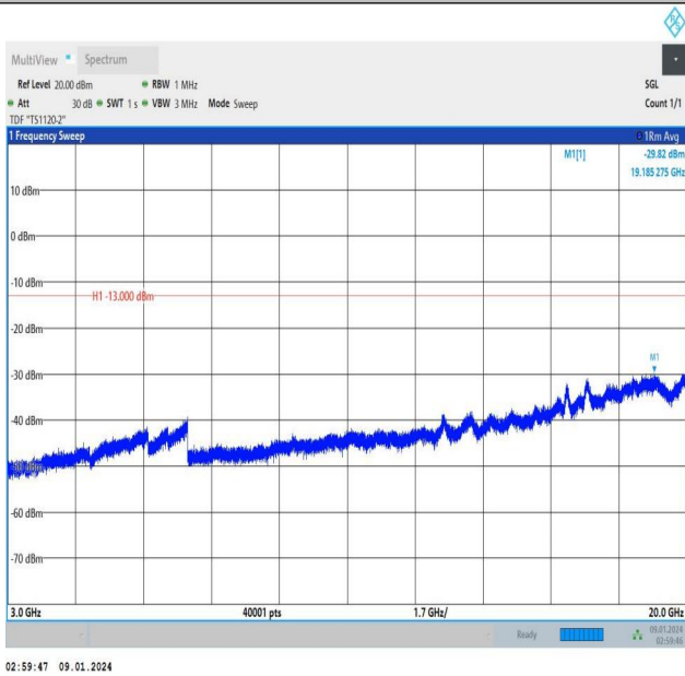
Band25_3MHz_QPSK_26055_1RB#0_3000~20000_3000~20
