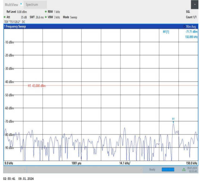
Band25_1.4MHz_16QAM_26683_1RB#0_0.009~0.15_0.009~0.15
