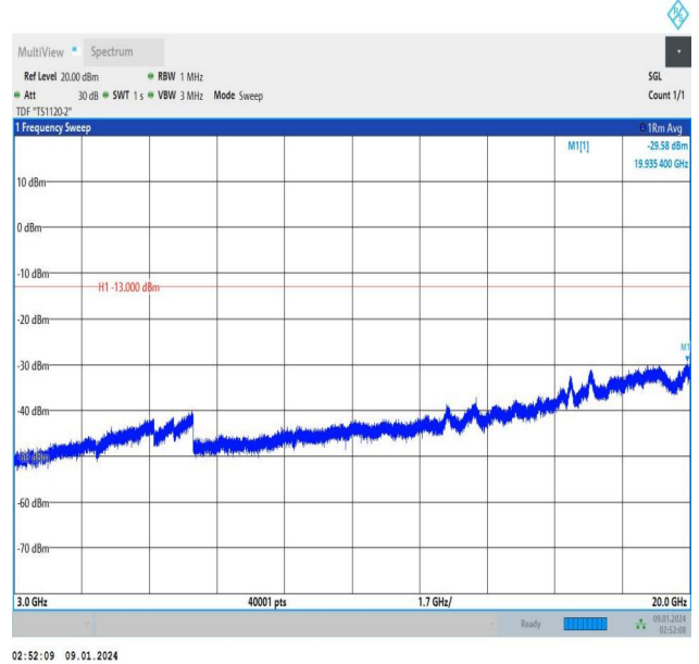
Band25_1.4MHz_16QAM_26365_1RB#0_3000~20000_3000~20000
