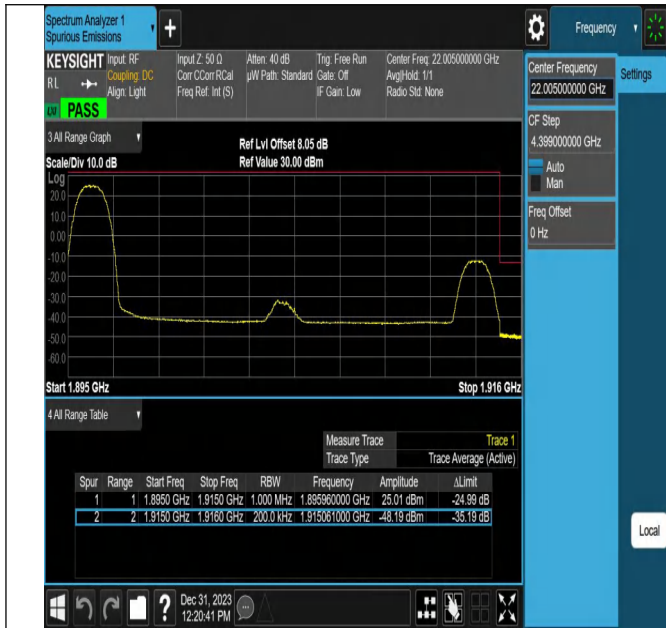
Band25_20MHz_16QAM_26590_1RB#0
