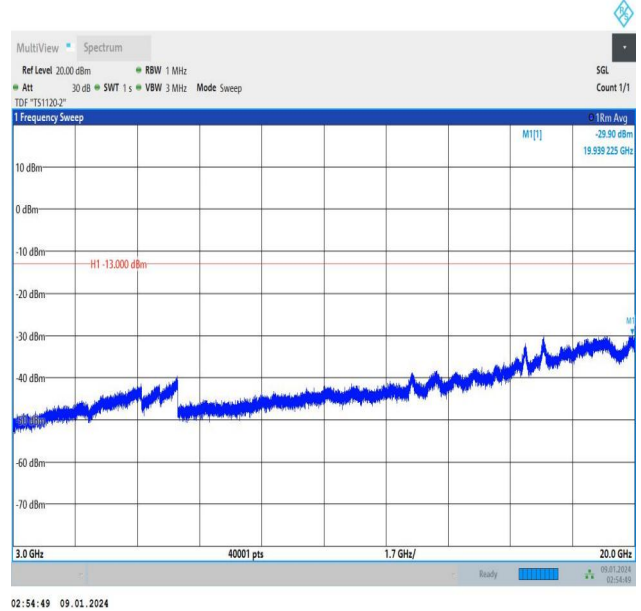
Band25_1.4MHz_16QAM_26365_6RB#0_3000~20000_3000~20000
