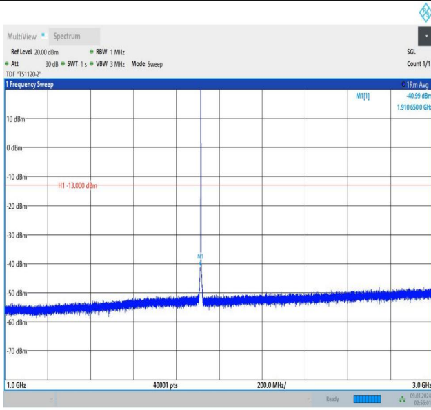
Band25_1.4MHz_16QAM_26683_1RB#0_1000~3000_1000~3000
