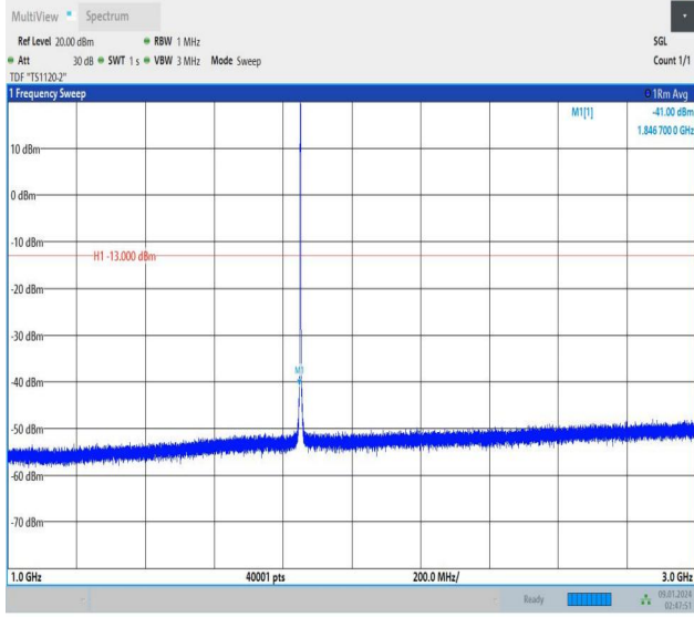
Band25_1.4MHz_16QAM_26047_1RB#0_1000~3000_1000~3000
