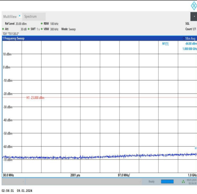
Band25_1.4MHz_QPSK_26683_1RB#5_30~1000_30~1000
