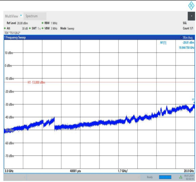
Band25_1.4MHz_16QAM_26683_1RB#0_3000~20000_3000~20000
