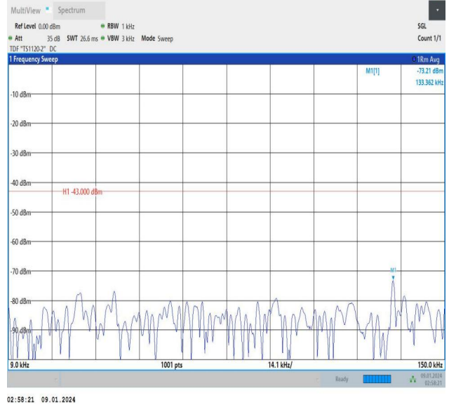
Band25_1.4MHz_16QAM_26683_6RB#0_0.009~0.15_0.009~0.15
