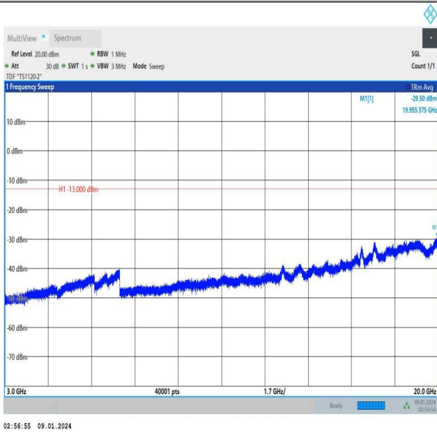
Band25_1.4MHz_QPSK_26683_1RB#5_3000~20000_3000~20000 0000
