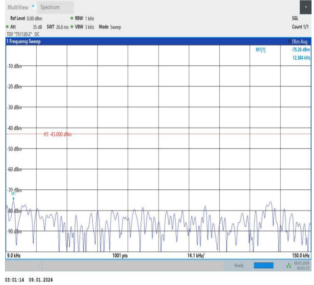
Band25_3MHz_16QAM_26055_1RB#14_0.009~0.15_0.009~0.15
