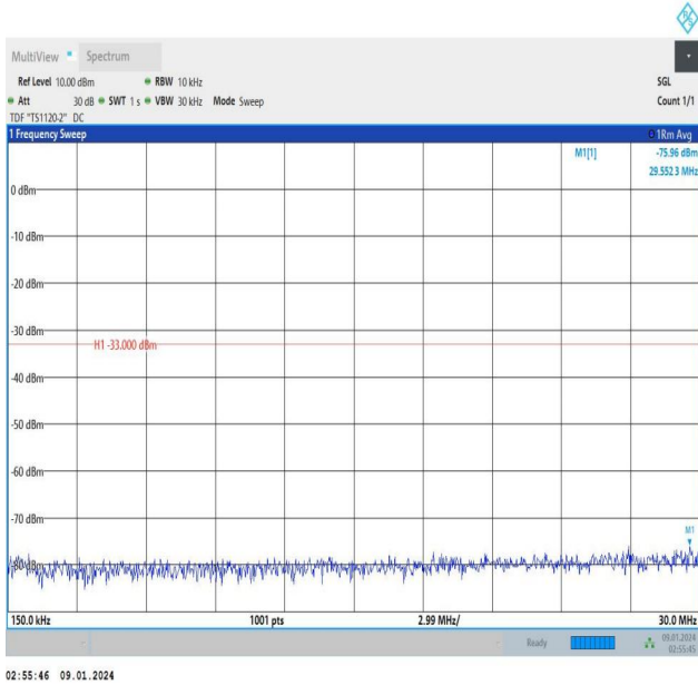
Band25_1.4MHz_16QAM_26683_1RB#0_0.15~30_0.15~30
