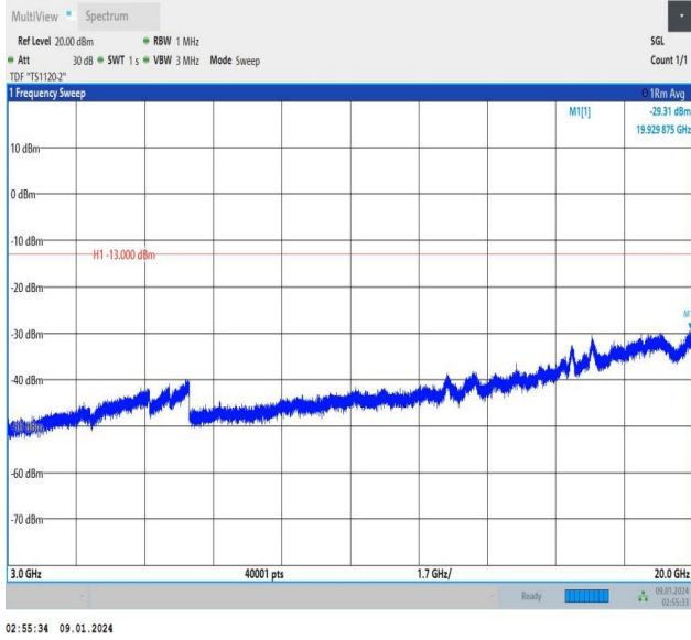
Band25_1.4MHz_QPSK_26683_1RB#0_3000~20000_3000~20000
