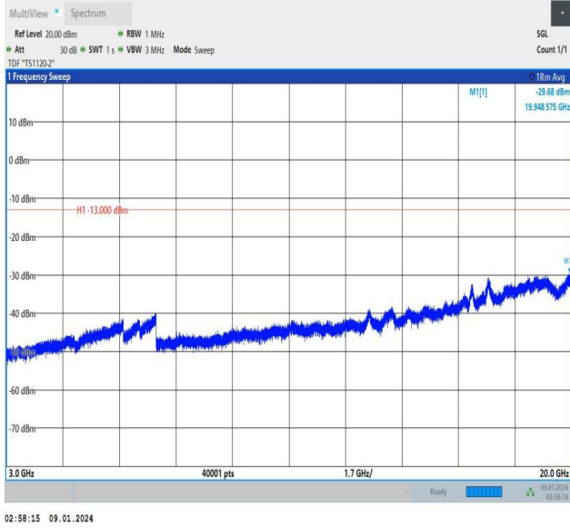
Band25_1.4MHz_QPSK_26683_6RB#0_3000~20000_3000~20000
