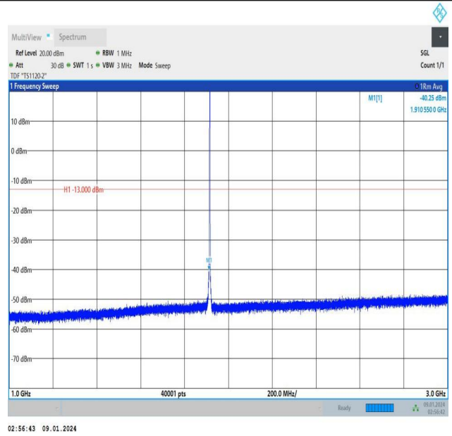
Band25_1.4MHz_QPSK_26683_1RB#5_1000~3000_1000~3000 00
