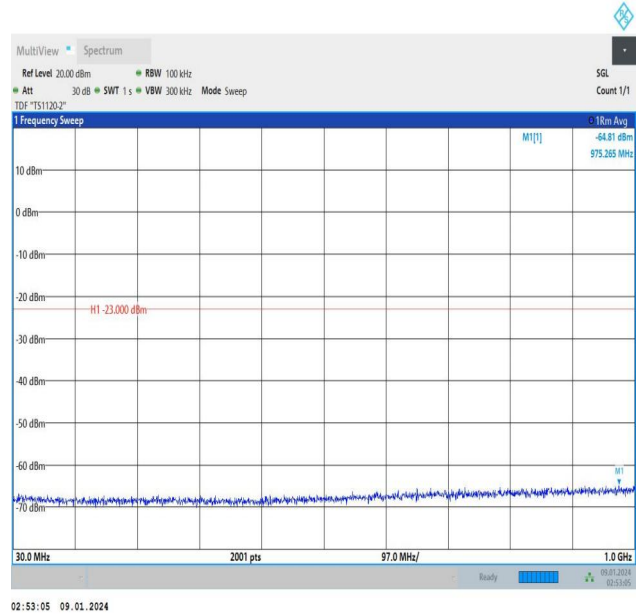
Band25_1.4MHz_16QAM_26365_1RB#5_30~1000_30~1000
