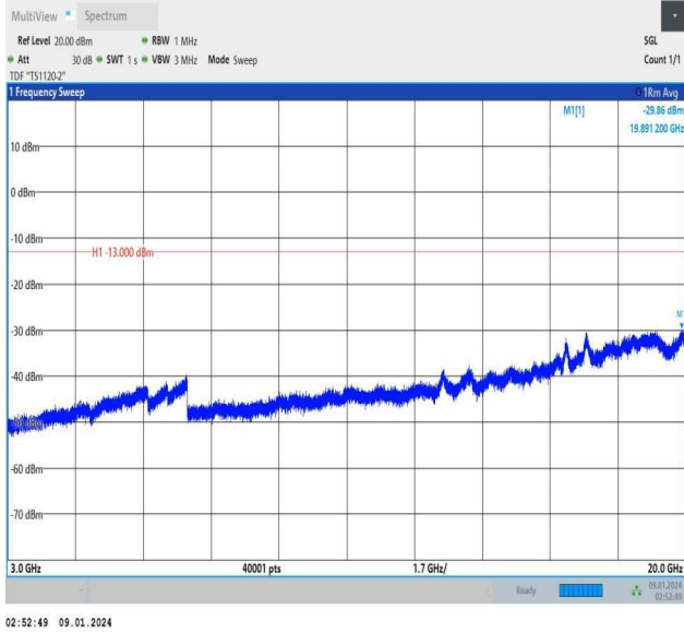
Band25_1.4MHz_QPSK_26365_1RB#5_3000~20000_3000~20000
