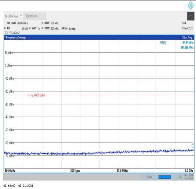
Band25_1.4MHz_16QAM_26047_1RB#5_30~1000_30~1000
