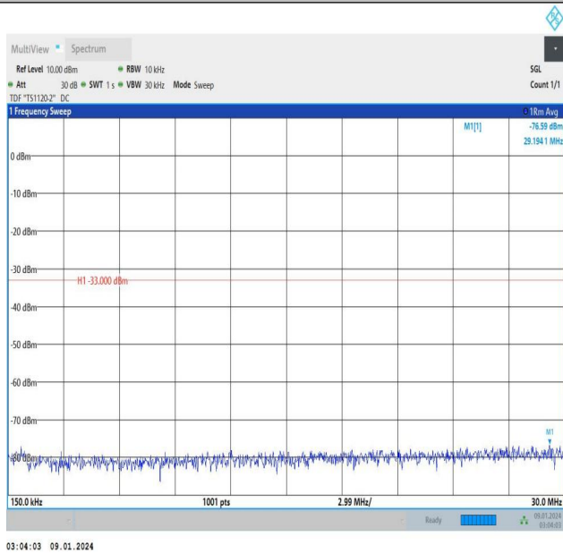
Band25_3MHz_16QAM_26365_1RB#0_0.15~30_0.15~30
