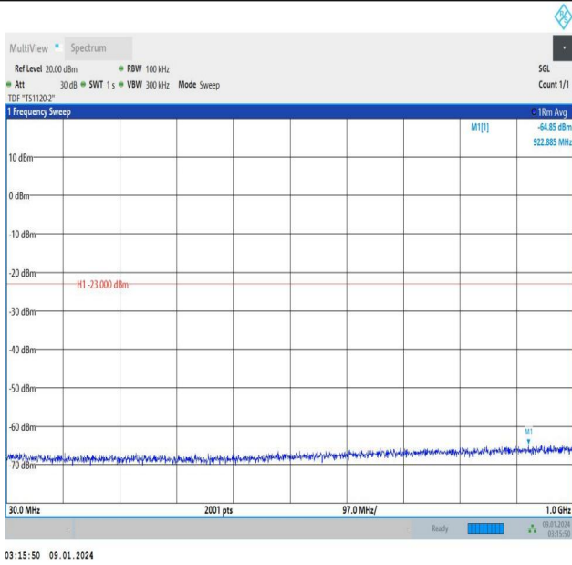
Band25_5MHz_QPSK_26365_1RB#0_30~1000_30~1000
