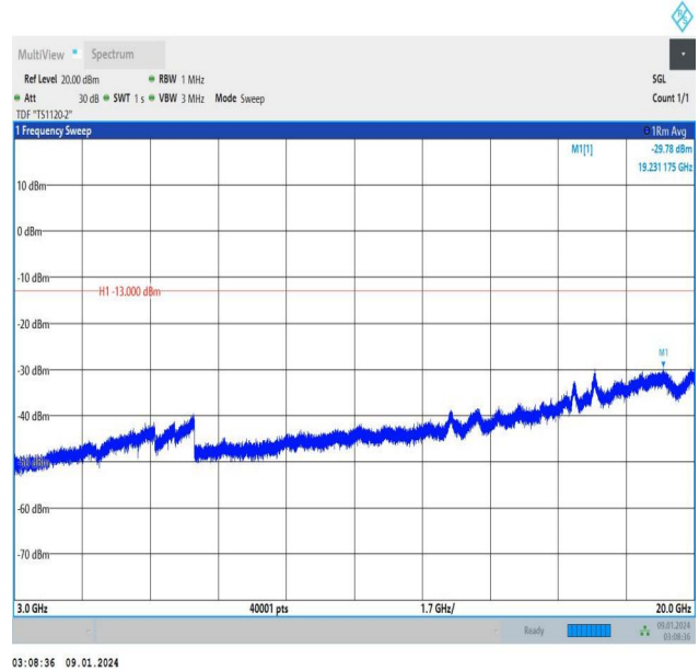
Band25_3MHz_16QAM_26675_1RB#0_3000~20000_3000~20000
