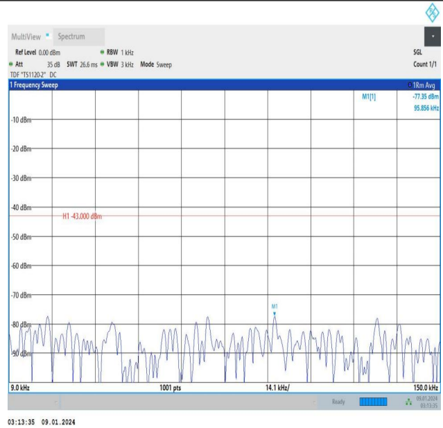
Band25_5MHz_16QAM_26065_1RB#24_0.009~0.15_0.009~0 .15
