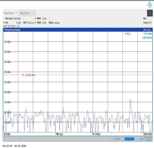
Band25_5MHz_16QAM_26365_25RB#0_0.009~0.15_0.009~0 .15
