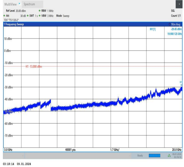
Band25_5MHz_16QAM_26365_1RB#24_3000~20000_3000~20000
