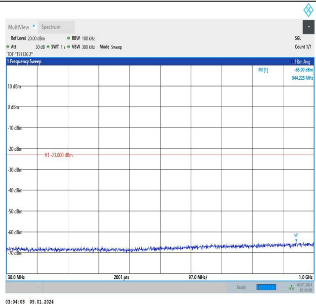
Band25_3MHz_16QAM_26365_1RB#0_30~1000_30~1000
