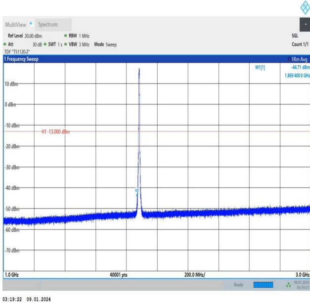
Band25_5MHz_16QAM_26365_25RB#0_1000~3000_1000~3000
