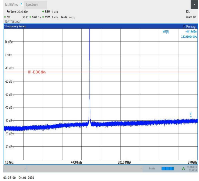
Band25_3MHz_QPSK_26365_1RB#14_1000~3000_1000~30 00
