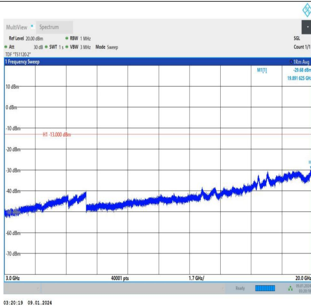
Band25_5MHz_QPSK_26665_1RB#0_3000~20000_3000~20000
