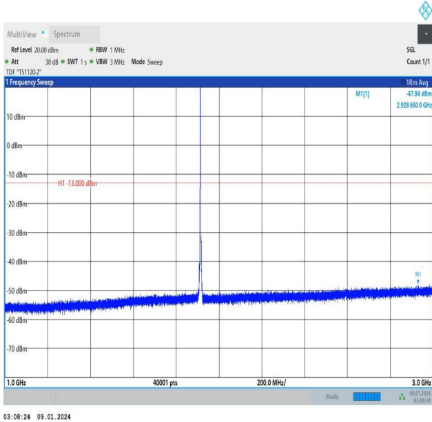
Band25_3MHz_16QAM_26675_1RB#0_1000~3000_1000~3000
