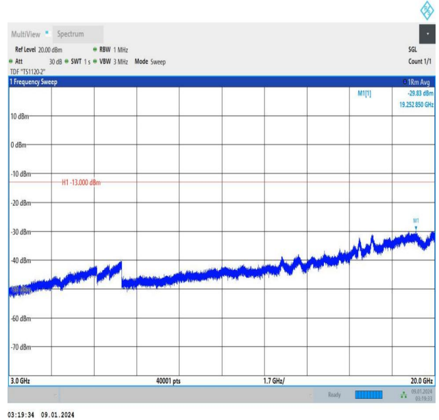
Band25_5MHz_16QAM_26365_25RB#0_3000~20000_3000~20000
