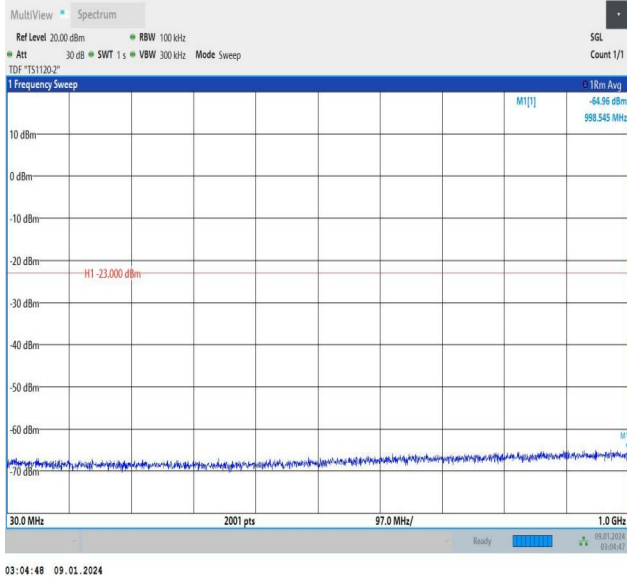
Band25_3MHz_QPSK_26365_1RB#14_30~1000_30~1000
