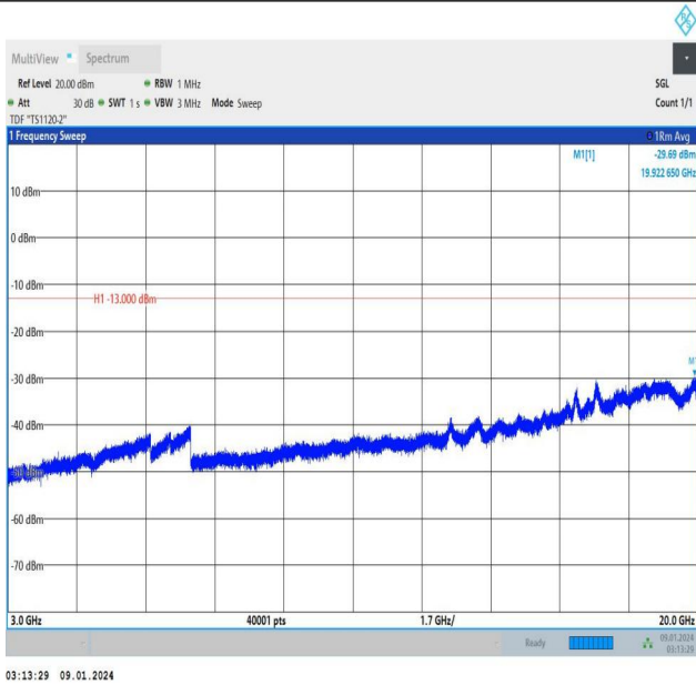
Band25_5MHz_QPSK_26065_1RB#24_3000~20000_3000~2 0000
