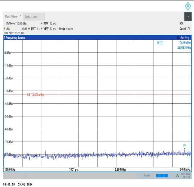
Band25_3MHz_QPSK_26055_15RB#0_0.15~30_0.15~30
