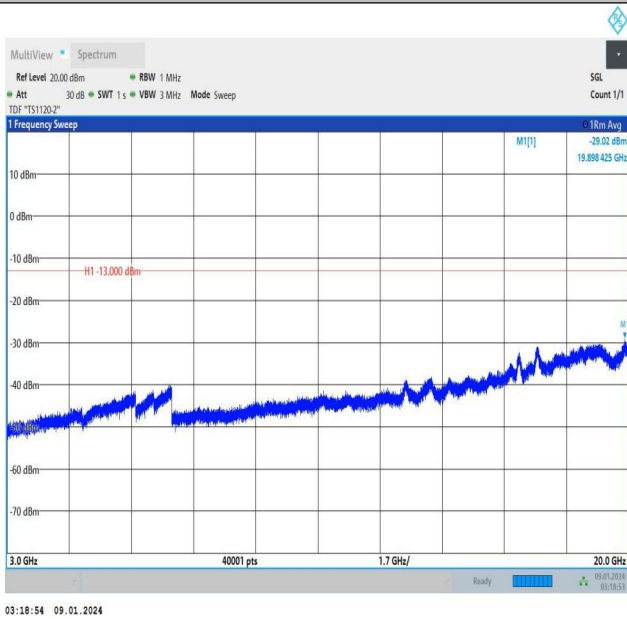
Band25_5MHz_QPSK_26365_25RB#0_3000~20000_3000~2 0000
