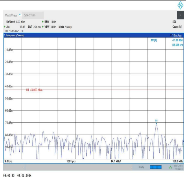
Band25_3MHz_16QAM_26055_15RB#0_0.009~0.15_0.009~0.15
