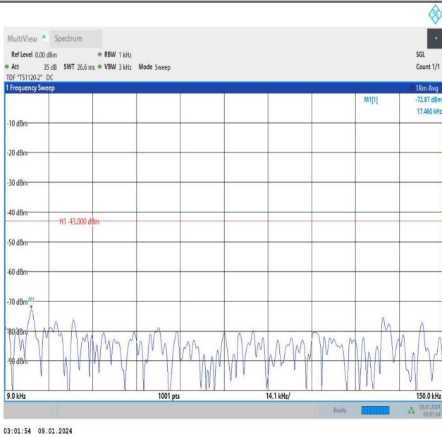
Band25_3MHz_QPSK_26055_15RB#0_0.009~0.15_0.009~0.15
