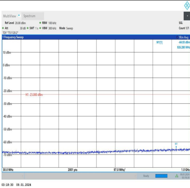
Band25_5MHz_QPSK_26365_25RB#0_30~1000_30~1000
