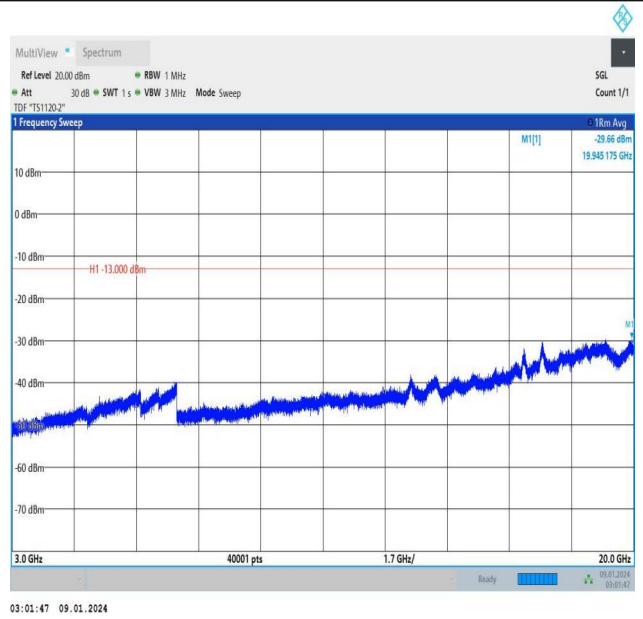
Band25_3MHz_16QAM_26055_1RB#14_3000~20000_3000~20000
