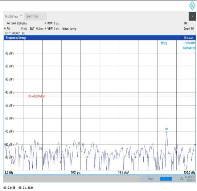
Band25_3MHz_16QAM_26365_1RB#0_0.009~0.15_0.009~0.15
