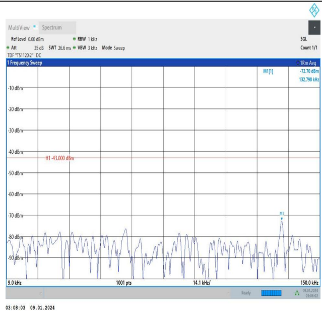
Band25_3MHz_16QAM_26675_1RB#0_0.009~0.15_0.009~0.15 15
