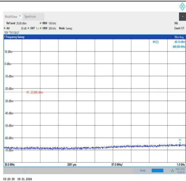
Band25_5MHz_16QAM_26665_1RB#0_30~1000_30~1000
