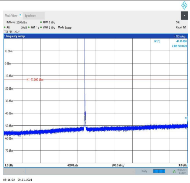
Band25_5MHz_QPSK_26365_1RB#0_1000~3000_1000~300
