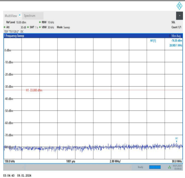
Band25_3MHz_QPSK_26365_1RB#14_0.15~30_0.15~30
