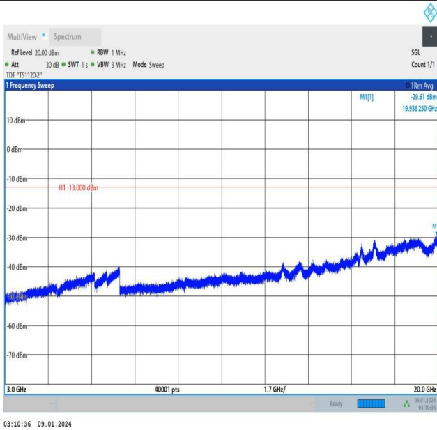
Band25_3MHz_QPSK_26675_15RB#0_3000~20000_3000~20000
