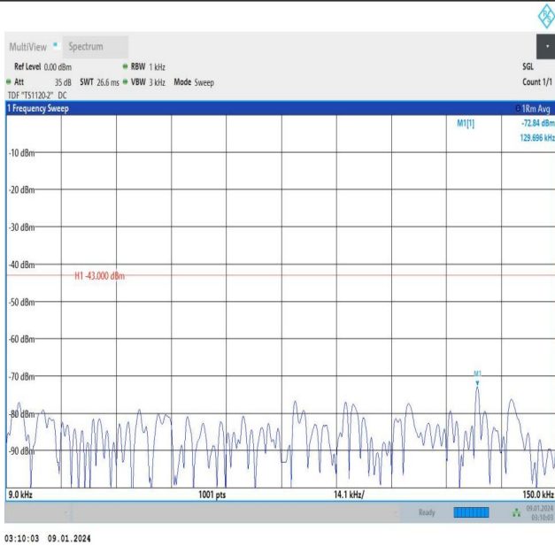
Band25_3MHz_QPSK_26675_15RB#0_0.009~0.15_0.009~0.15
