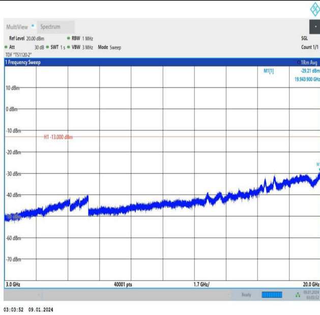
Band25_3MHz_QPSK_26365_1RB#0_3000~20000_3000~20000
