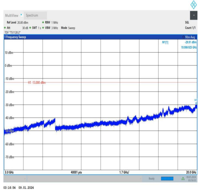
Band25_5MHz_16QAM_26365_1RB#0_3000~20000_3000~2 0000
