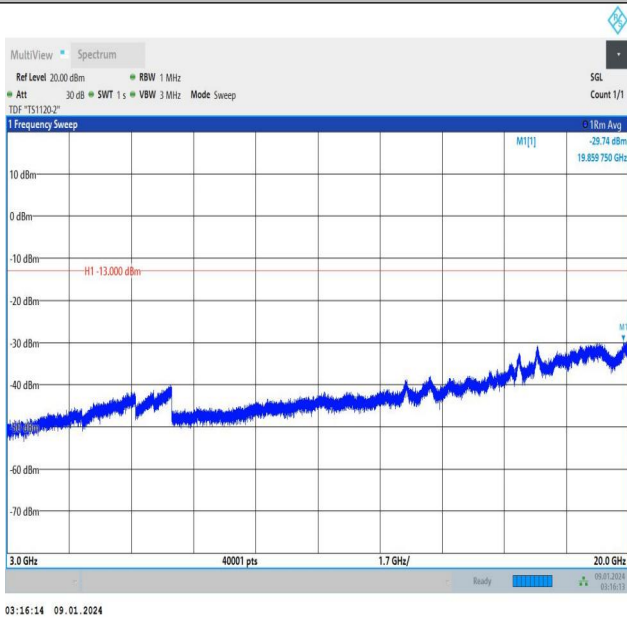
Band25_5MHz_QPSK_26365_1RB#0_3000~20000_3000~20
