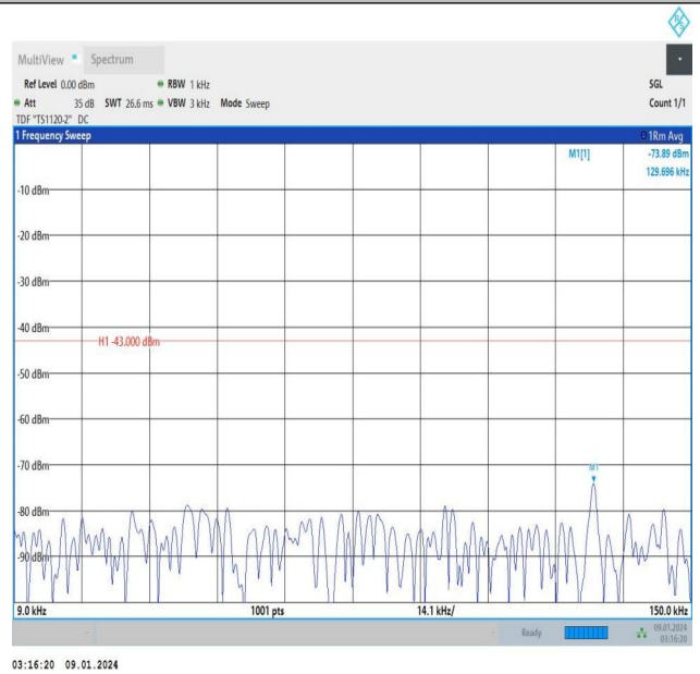
Band25_5MHz_16QAM_26365_1RB#0_0.009~0.15_0.009~0.
