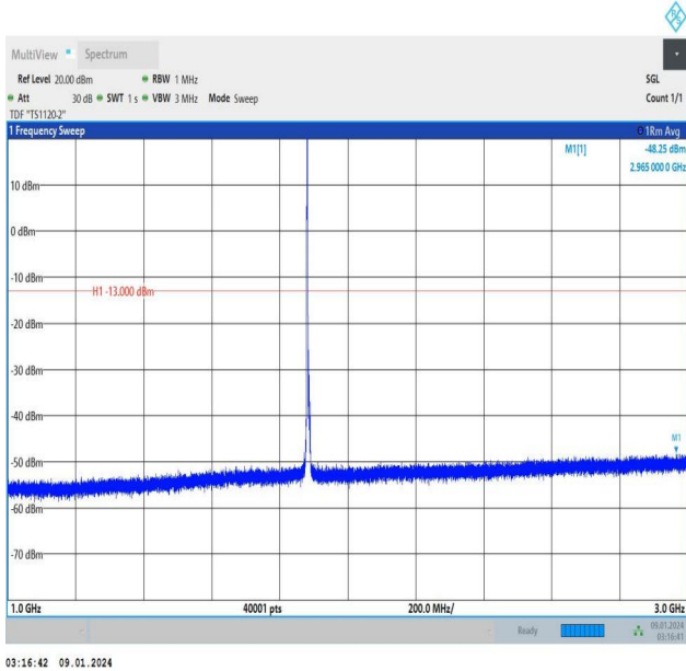
Band25_5MHz_16QAM_26365_1RB#0_1000~3000_1000~30 00
