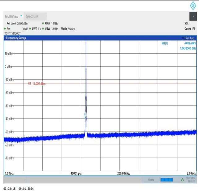
Band25_3MHz_QPSK_26055_15RB#0_1000~3000_1000~3000
