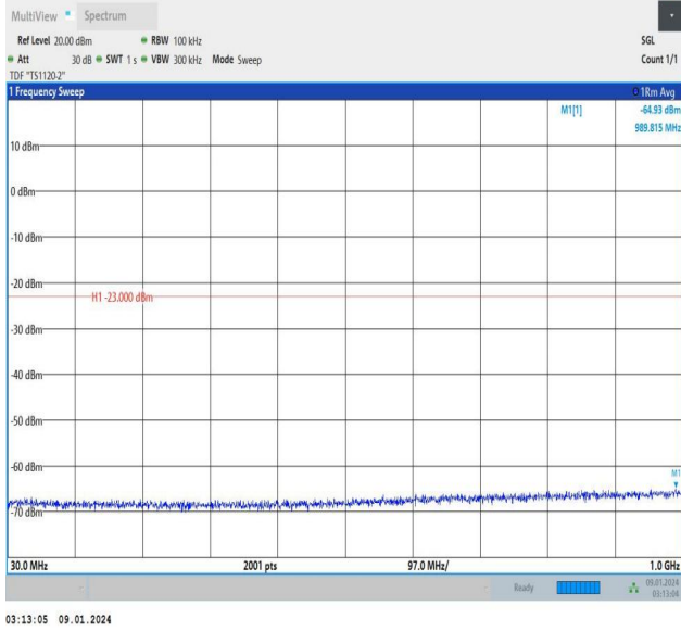
Band25_5MHz_QPSK_26065_1RB#24_30~1000_30~1000
