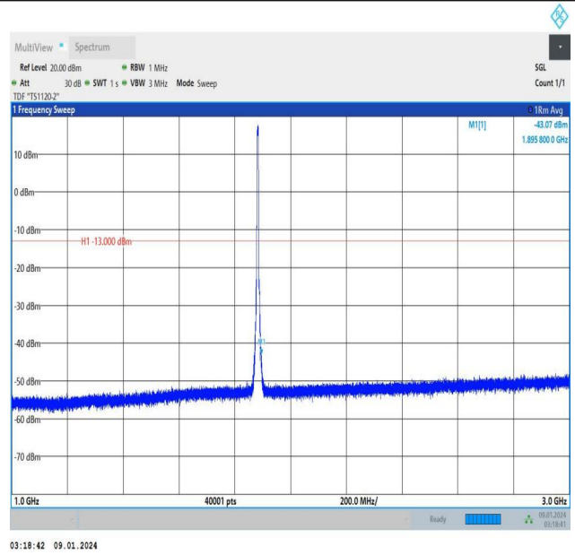
Band25_5MHz_QPSK_26365_25RB#0_1000~3000_1000~30 00
