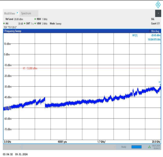
Band25_3MHz_16QAM_26365_1RB#0_3000~20000_3000~2 0000
