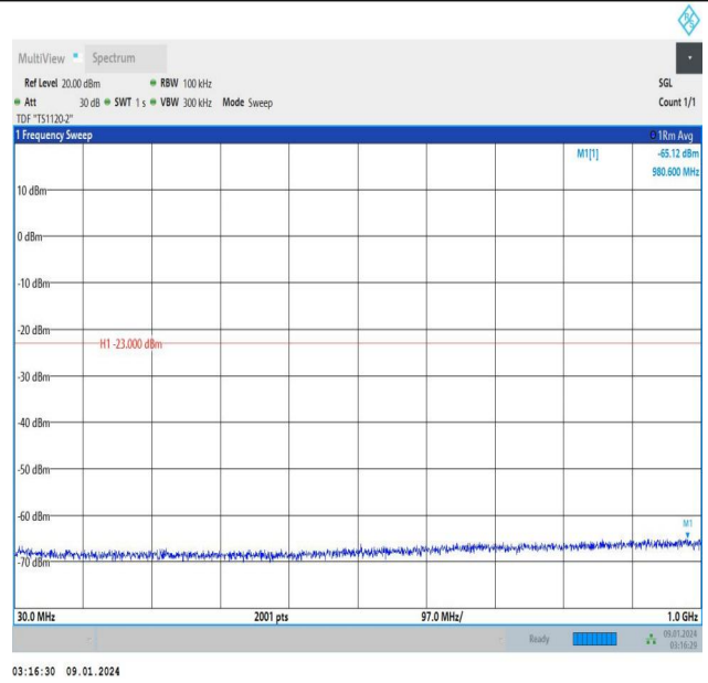
Band25_5MHz_16QAM_26365_1RB#0_30~1000_30~1000
