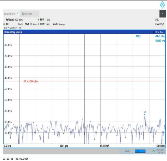
Band25_3MHz_16QAM_26675_15RB#0_0.009~0.15_0.009~0.15
