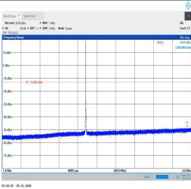
Band25_3MHz_16QAM_26365_1RB#0_1000~3000_1000~30 00
