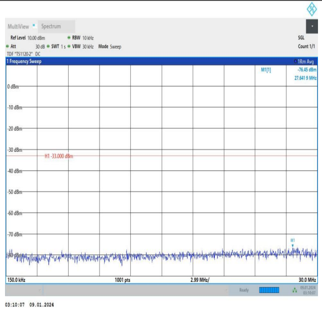
Band25_3MHz_QPSK_26675_15RB#0_0.15~30_0.15~30
