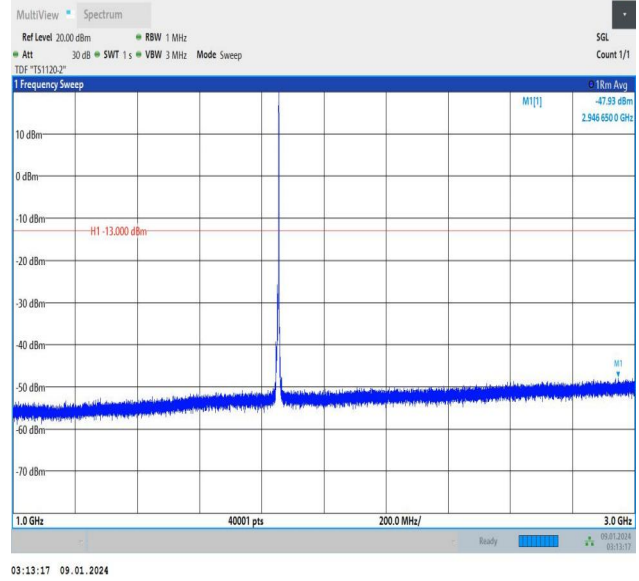
Band25_5MHz_QPSK_26065_1RB#24_1000~3000_1000~30 00
