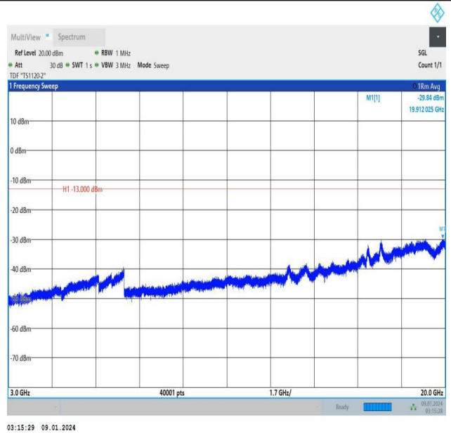
Band25_5MHz_16QAM_26065_25RB#0_3000~20000_3000~20000
