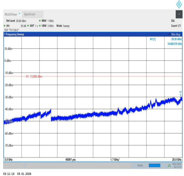
Band25_3MHz_16QAM_26675_15RB#0_3000~20000_3000~20000
