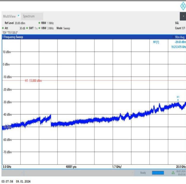
Band25_3MHz_QPSK_26675_1RB#0_3000~20000_3000~20000 000
