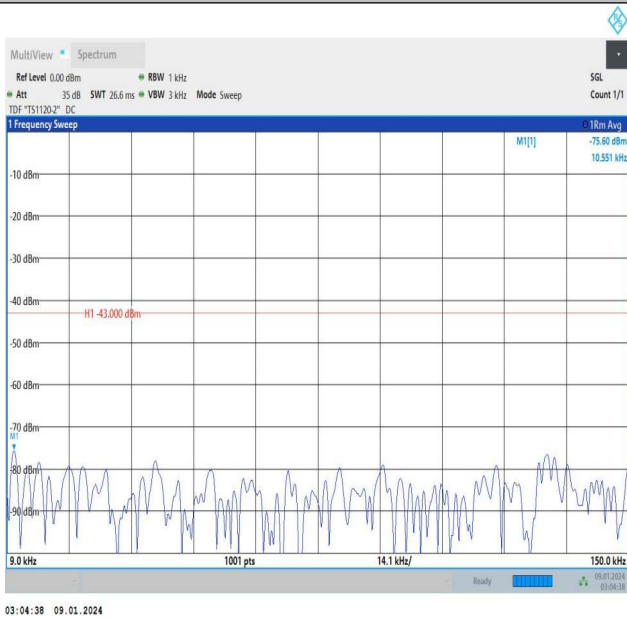
Band25_3MHz_QPSK_26365_1RB#14_0.009~0.15_0.009~0. 15
