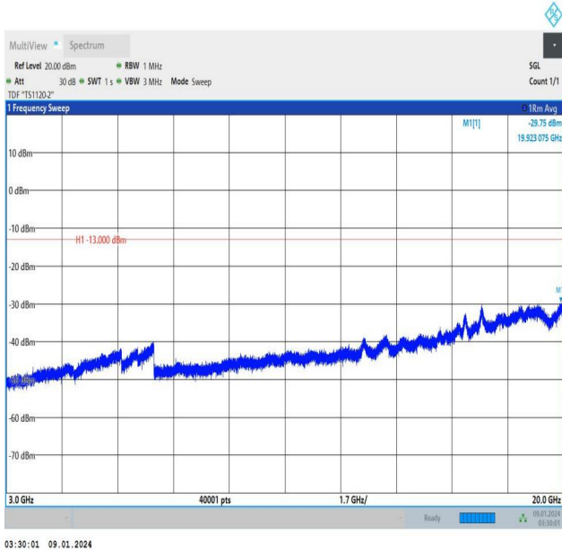
Band25_10MHz_QPSK_26640_1RB#0_3000~20000_3000~20000
