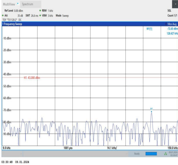
Band25_10MHz_QPSK_26640_1RB#49_0.009~0.15_0.009~0.15
