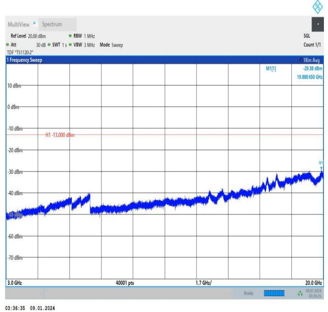
Band25_15MHz_QPSK_26115_1RB#74_3000~20000_3000~2 0000
