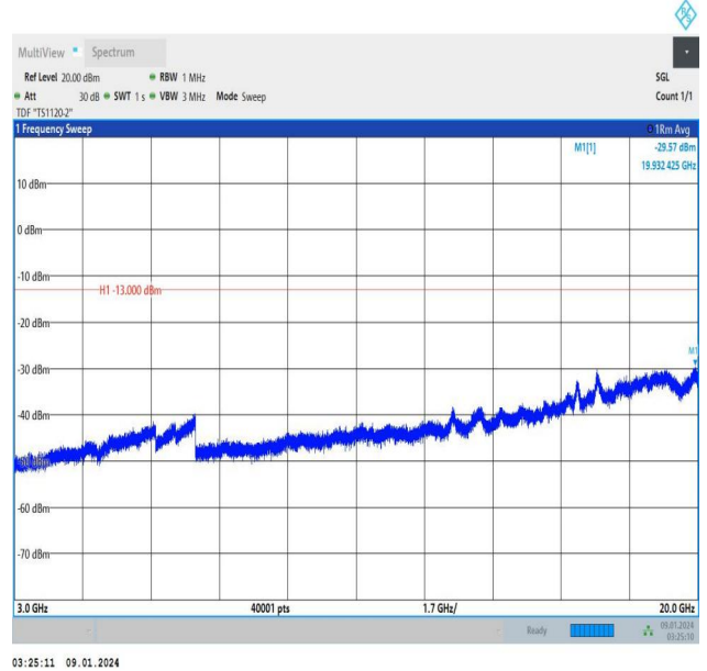
Band25_10MHz_16QAM_26090_1RB#0_3000~20000_3000~20000
