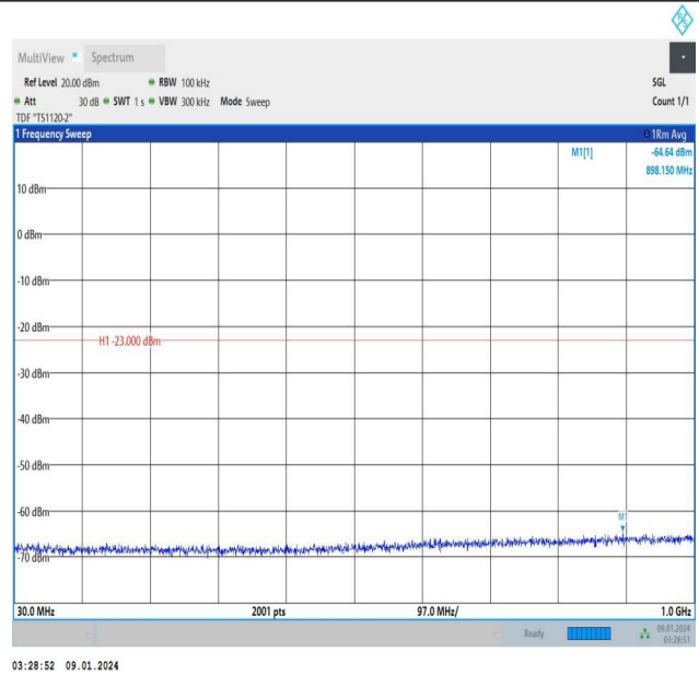
Band25_10MHz_16QAM_26365_1RB#49_30~1000_30~1000
