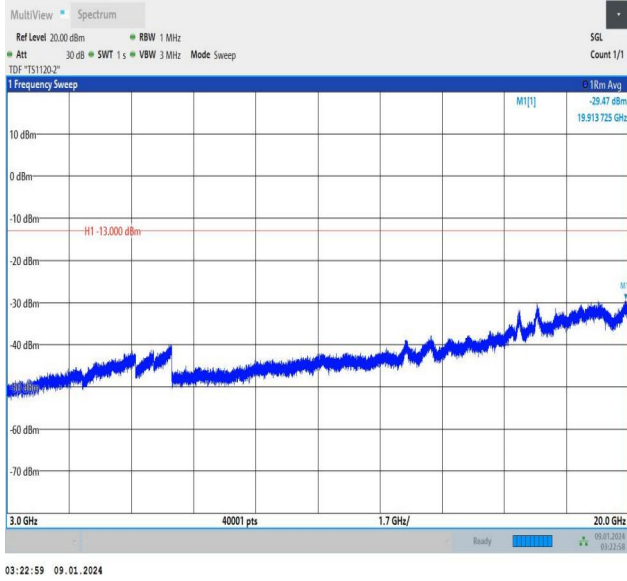
Band25_5MHz_QPSK_26665_25RB#0_3000~20000_3000~20000
