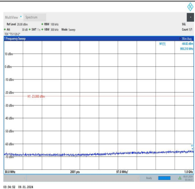
Band25_15MHz_QPSK_26115_1RB#0_30~1000_30~1000
