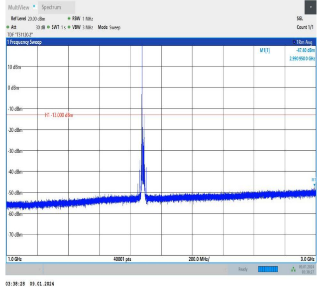
Band25_15MHz_16QAM_26365_1RB#0_1000~3000_1000~3000
