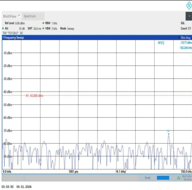
Band25_10MHz_QPSK_26640_50RB#0_0.009~0.15_0.009~0.15
