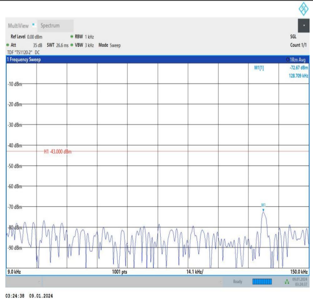
Band25_10MHz_16QAM_26090_1RB#0_0.009~0.15_0.009~0.15
