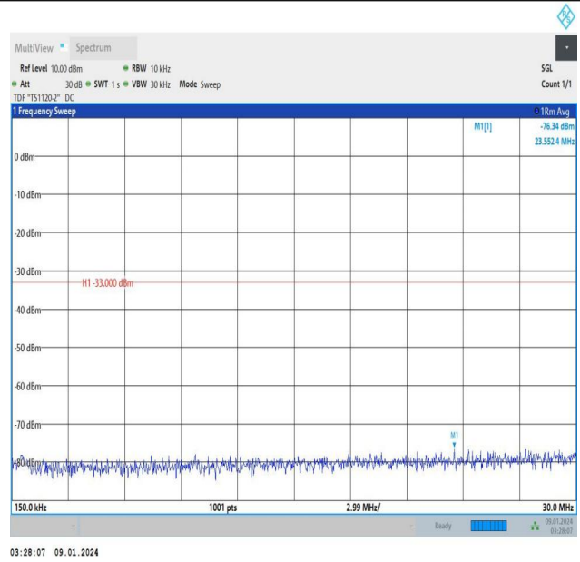
Band25_10MHz_QPSK_26365_1RB#49_0.15~30_0.15~30
