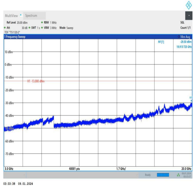
Band25_10MHz_QPSK_26365_50RB#0_3000~20000_3000~20000
