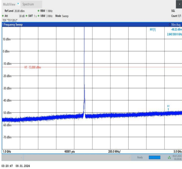
Band25_5MHz_16QAM_26665_1RB#0_1000~3000_1000~30 00
