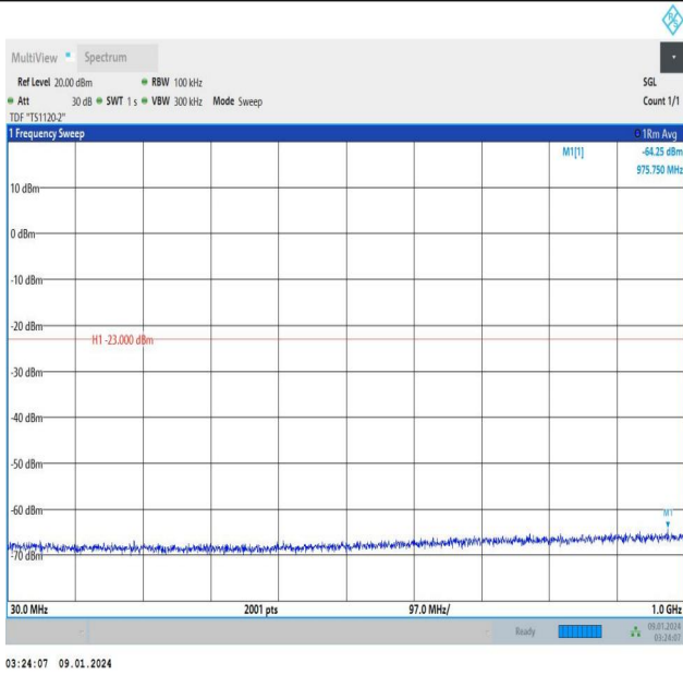
Band25_10MHz_QPSK_26090_1RB#0_30~1000_30~1000
