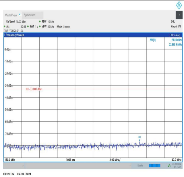
Band25_10MHz_QPSK_26090_1RB#49_0.15~30_0.15~30
