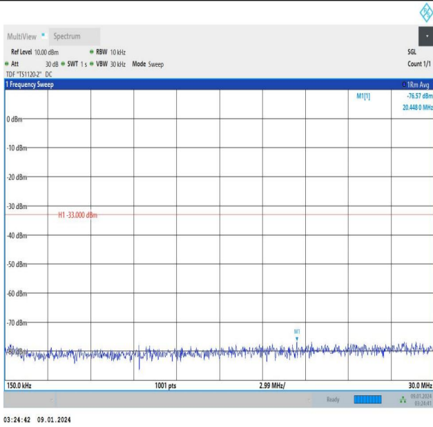
Band25_10MHz_16QAM_26090_1RB#0_0.15~30_0.15~30
