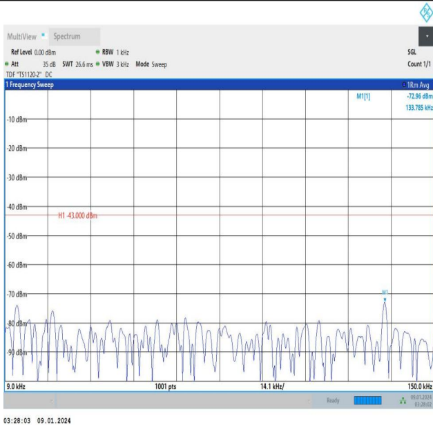
Band25_10MHz_QPSK_26365_1RB#49_0.009~0.15_0.009~0.15
