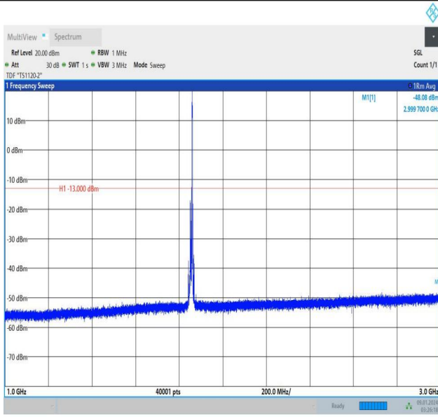
Band25_10MHz_16QAM_26090_1RB#49_1000~3000_1000~3000
