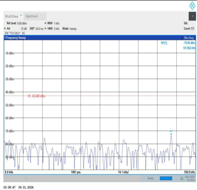
Band25_15MHz_QPSK_26365_1RB#74_0.009~0.15_0.009~0.15
