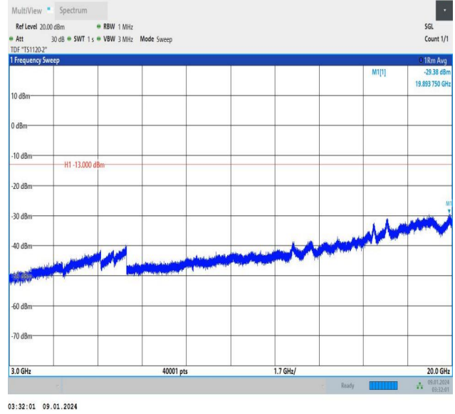
Band25_10MHz_16QAM_26640_1RB#49_3000~20000_3000~20000
