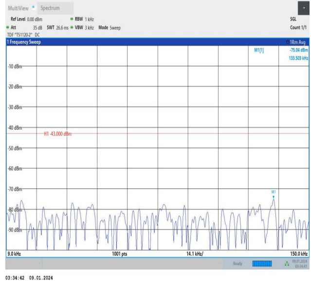
Band25_15MHz_QPSK_26115_1RB#0_0.009~0.15_0.009~0.1
