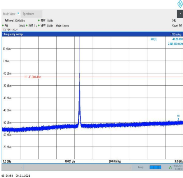
Band25_10MHz_16QAM_26090_1RB#0_1000~3000_1000~3000
