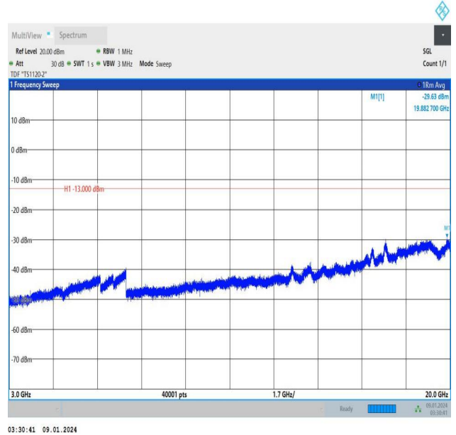
Band25_10MHz_16QAM_26640_1RB#0_3000~20000_3000~20000
