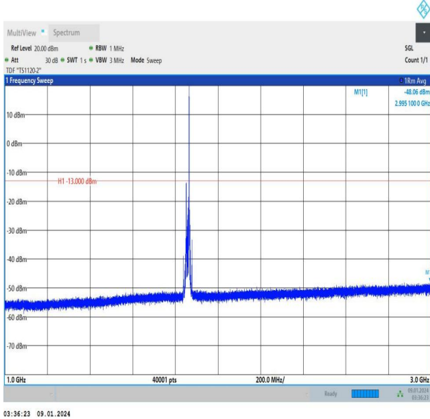
Band25_15MHz_QPSK_26115_1RB#74_1000~3000_1000~30 00
