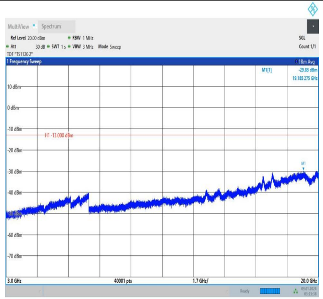
Band25_5MHz_16QAM_26665_25RB#0_3000~20000_3000~20000
