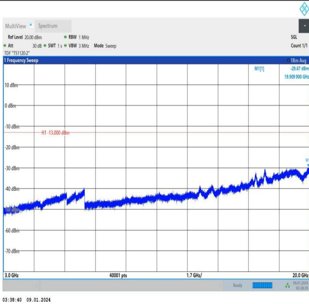
Band25_15MHz_16QAM_26365_1RB#0_3000~20000_3000~20000
