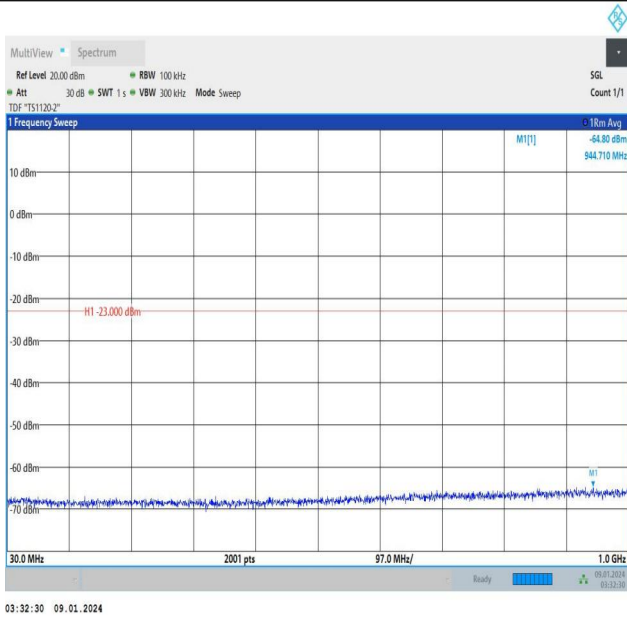
Band25_10MHz_QPSK_26090_50RB#0_30~1000_30~1000
