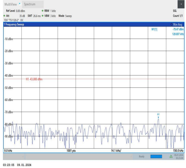
Band25_5MHz_16QAM_26665_25RB#0_0.009~0.15_0.009~0.15
