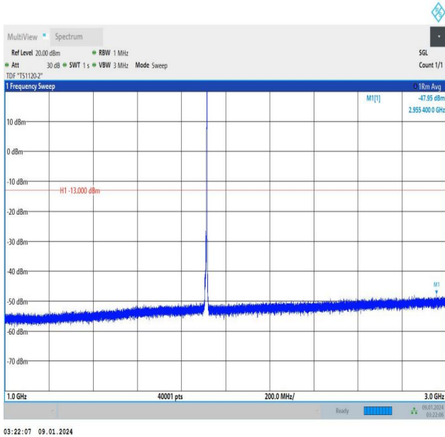
Band25_5MHz_16QAM_26665_1RB#24_1000~3000_1000~3000
