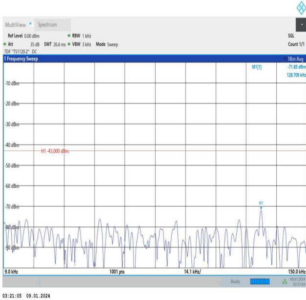
Band25_5MHz_QPSK_26665_1RB#24_0.009~0.15_0.009~0. 15
