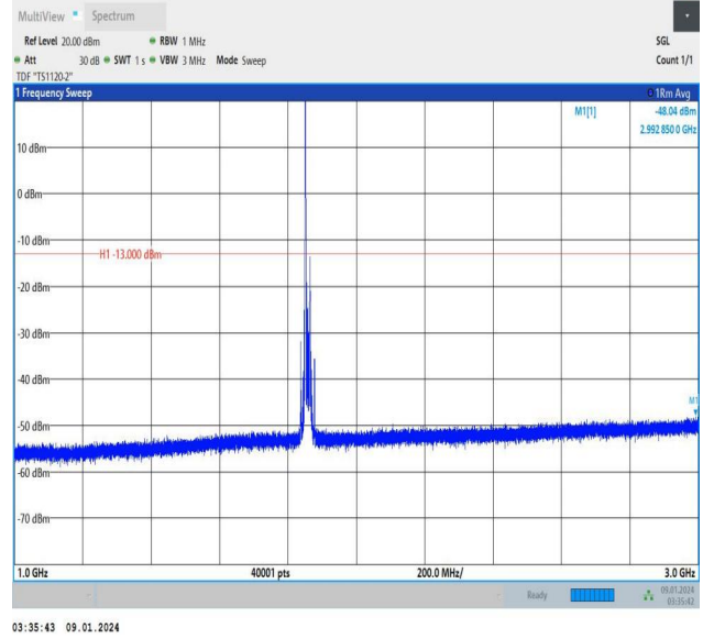
Band25_15MHz_16QAM_26115_1RB#0_1000~3000_1000~3000
