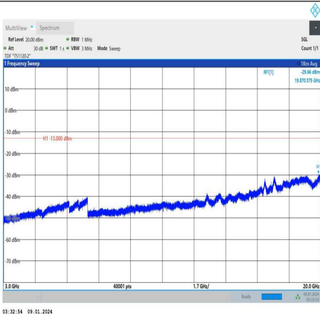
Band25_10MHz_QPSK_26090_50RB#0_3000~20000_3000~20000
