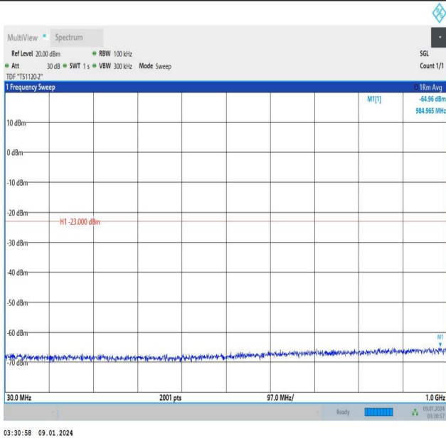
Band25_10MHz_QPSK_26640_1RB#49_30~1000_30~1000
