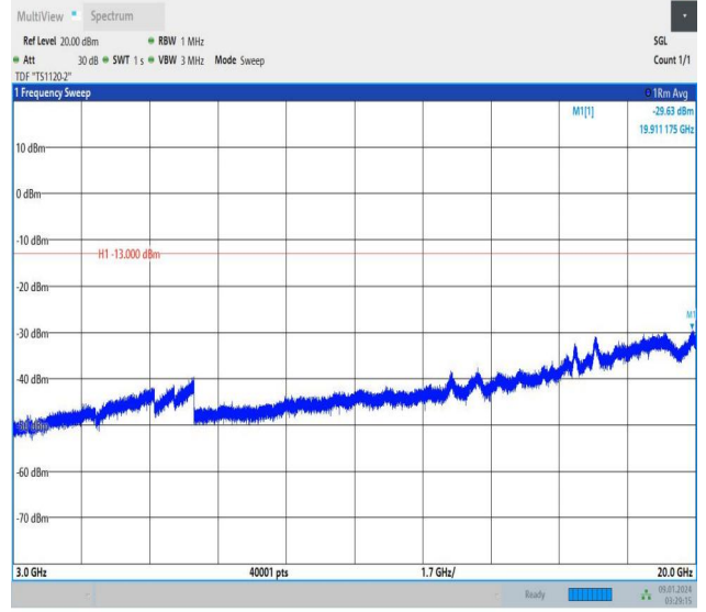
Band25_10MHz_16QAM_26365_1RB#49_3000~20000_3000~20000
