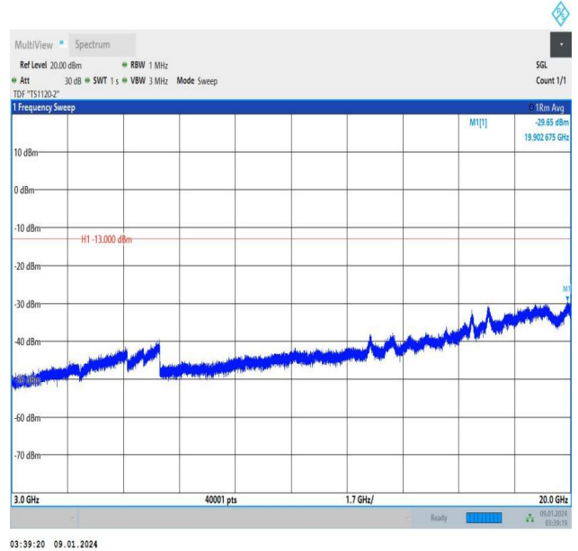
Band25_15MHz_QPSK_26365_1RB#74_3000~20000_3000~20000
