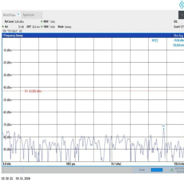
Band25_10MHz_QPSK_26090_50RB#0_0.009~0.15_0.009~0.15
