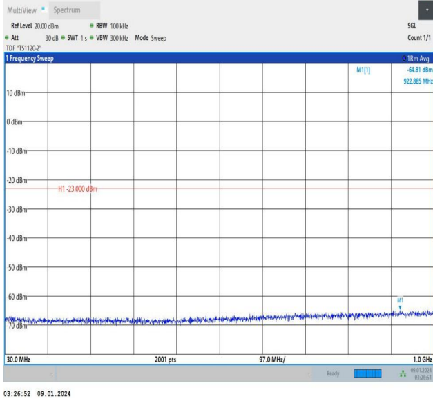
Band25_10MHz_QPSK_26365_1RB#0_30~1000_30~1000
