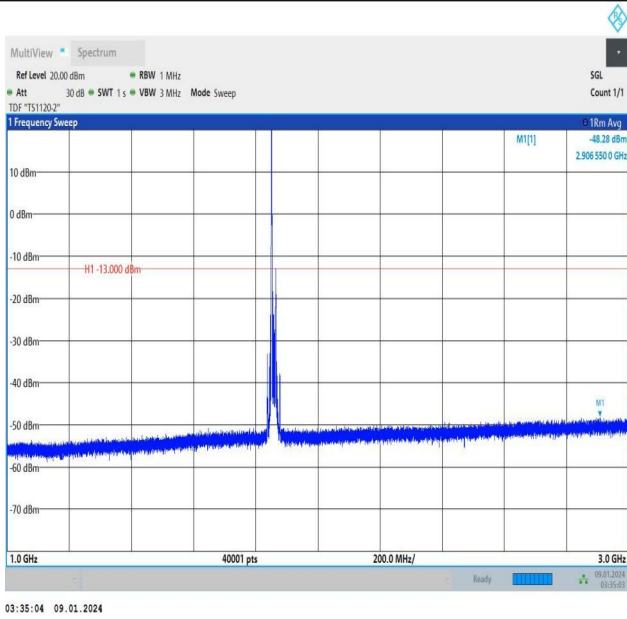
Band25_15MHz_QPSK_26115_1RB#0_1000~3000_1000~300 0
