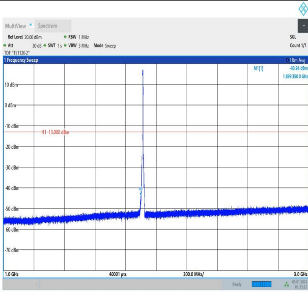
Band25_5MHz_16QAM_26665_25RB#0_1000~3000_1000~3000
