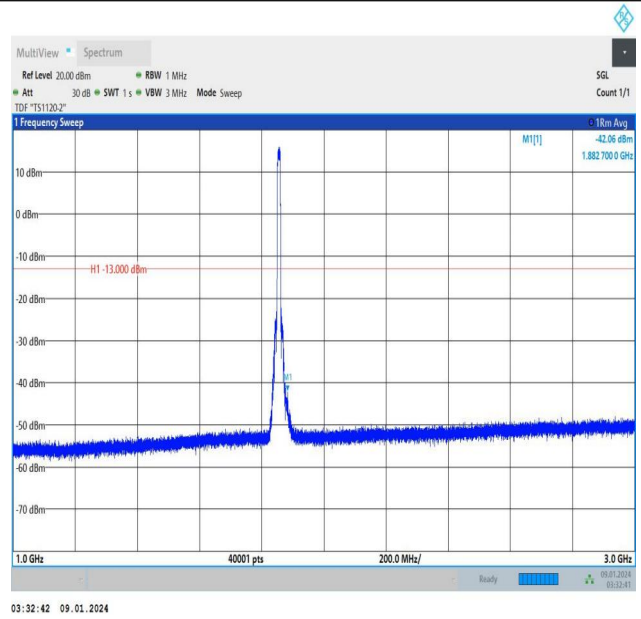
Band25_10MHz_QPSK_26090_50RB#0_1000~3000_1000~3000
