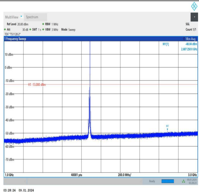
Band25_10MHz_QPSK_26365_1RB#49_1000~3000_1000~3000
