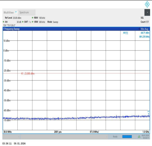
Band25_15MHz_QPSK_26115_1RB#74_30~1000_30~1000
