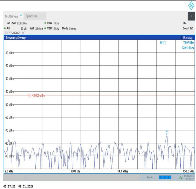
Band25_10MHz_16QAM_26365_1RB#0_0.009~0.15_0.009~0.15
