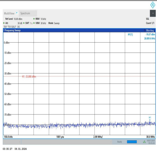
Band25_15MHz_16QAM_26115_1RB#0_0.15~30_0.15~30 0.15
