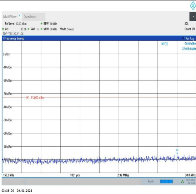
Band25_15MHz_QPSK_26115_1RB#74_0.15~30_0.15~30
