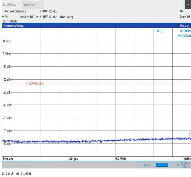
Band25_5MHz_QPSK_26665_1RB#24_30~1000_30~1000
