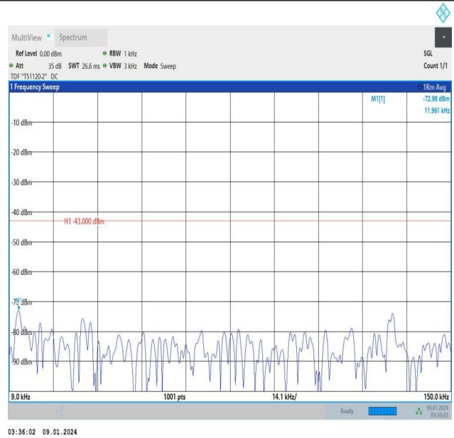
Band25_15MHz_QPSK_26115_1RB#74_0.009~0.15_0.009~0.15
