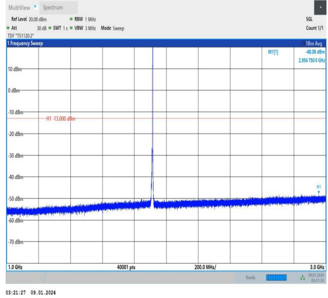
Band25_5MHz_QPSK_26665_1RB#24_1000~3000_1000~30 00
