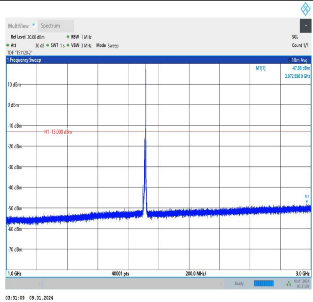
Band25_10MHz_QPSK_26640_1RB#49_1000~3000_1000~3000
