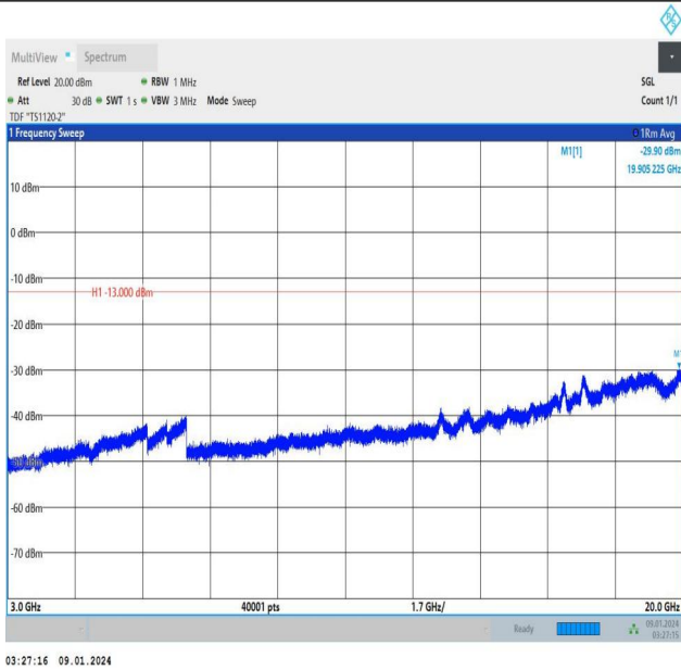
Band25_10MHz_QPSK_26365_1RB#0_3000~20000_3000~20000
