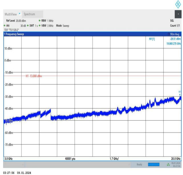
Band25_10MHz_16QAM_26365_1RB#0_3000~20000_3000~20000
