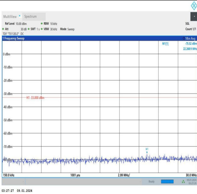
Band25_10MHz_16QAM_26365_1RB#0_0.15~30_0.15~30
