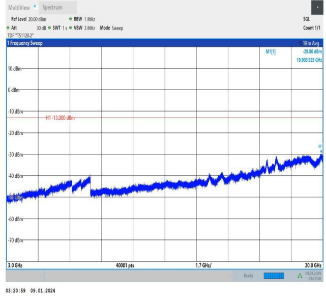
Band25_5MHz_16QAM_26665_1RB#0_3000~20000_3000~2 0000
