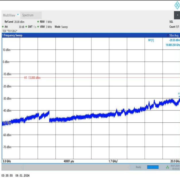
Band25_15MHz_16QAM_26115_1RB#0_3000~20000_3000~20000
