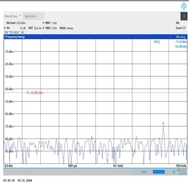
Band25_10MHz_QPSK_26365_50RB#0_0.009~0.15_0.009~0.15
