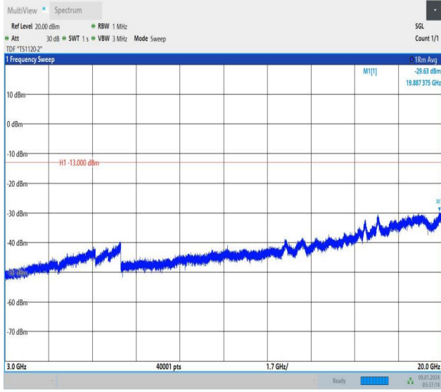
Band25_15MHz_16QAM_26115_1RB#74_3000~20000_3000~20000
