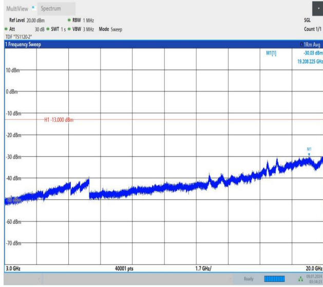
Band25_10MHz_QPSK_26640_50RB#0_3000~20000_3000~20000
