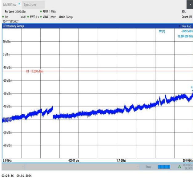
Band25_10MHz_QPSK_26365_1RB#49_3000~20000_3000~20000
