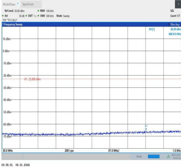
Band25_15MHz_16QAM_26115_1RB#0_30~1000_30~1000
