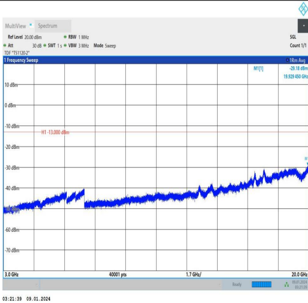
Band25_5MHz_QPSK_26665_1RB#24_3000~20000_3000~2 0000
