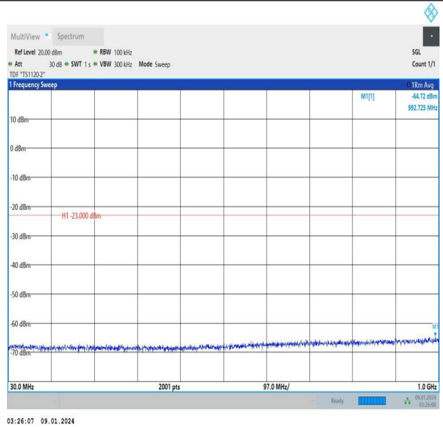
Band25_10MHz_16QAM_26090_1RB#49_30~1000_30~1000
