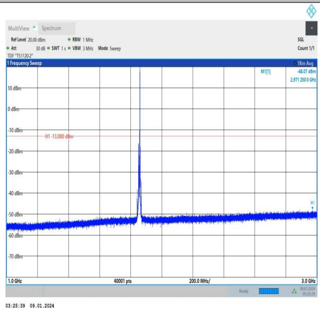
Band25_10MHz_QPSK_26090_1RB#49_1000~3000_1000~3000
