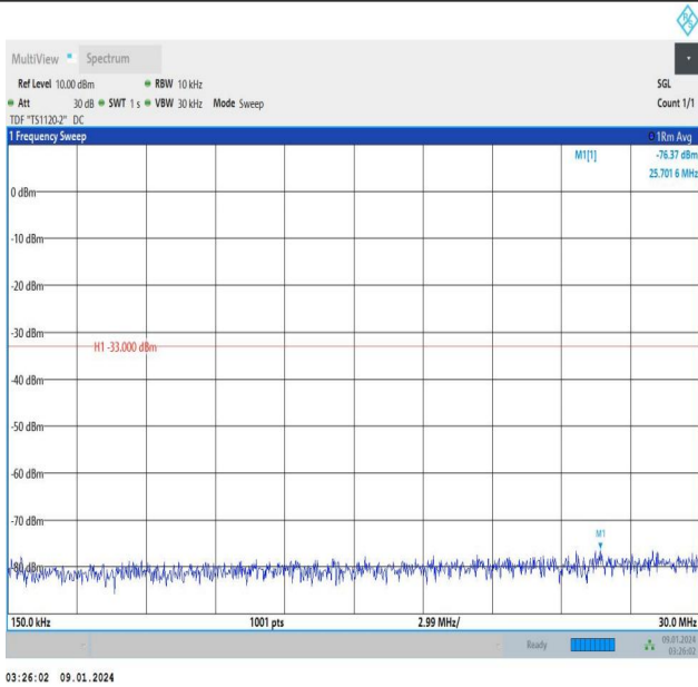
Band25_10MHz_16QAM_26090_1RB#49_0.15~30_0.15~30
