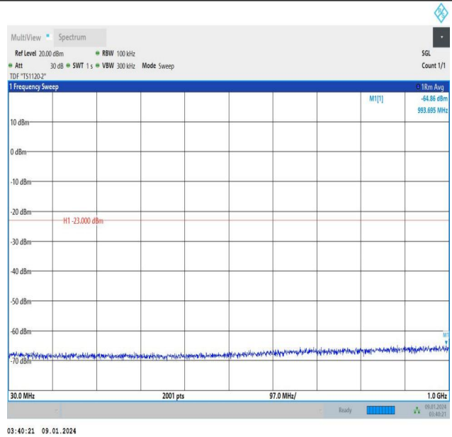
Band25_15MHz_QPSK_26615_1RB#0_30~1000_30~1000
