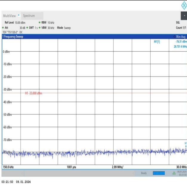
Band25_5MHz_16QAM_26665_1RB#24_0.15~30_0.15~30
