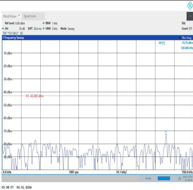
Band25_15MHz_16QAM_26365_1RB#0_0.009~0.15_0.009~0 .15
