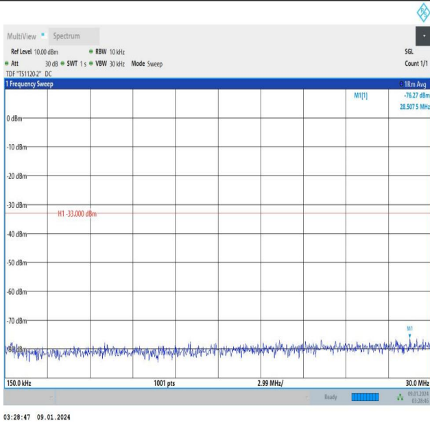
Band25_10MHz_16QAM_26365_1RB#49_0.15~30_0.15~30
