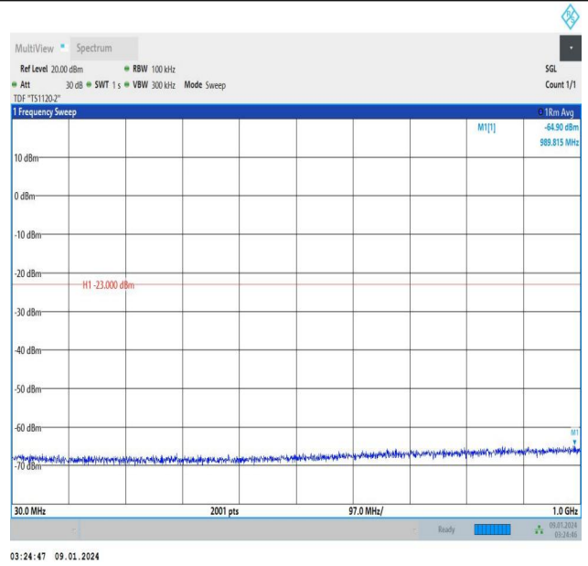
Band25_10MHz_16QAM_26090_1RB#0_30~1000_30~1000
