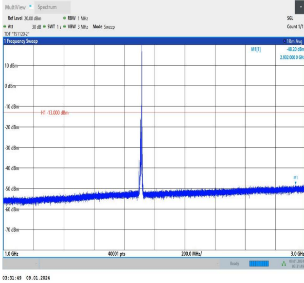
Band25_10MHz_16QAM_26640_1RB#49_1000~3000_1000~3000
