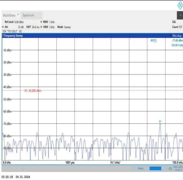
Band25_10MHz_QPSK_26090_1RB#49_0.009~0.15_0.009~0.15
