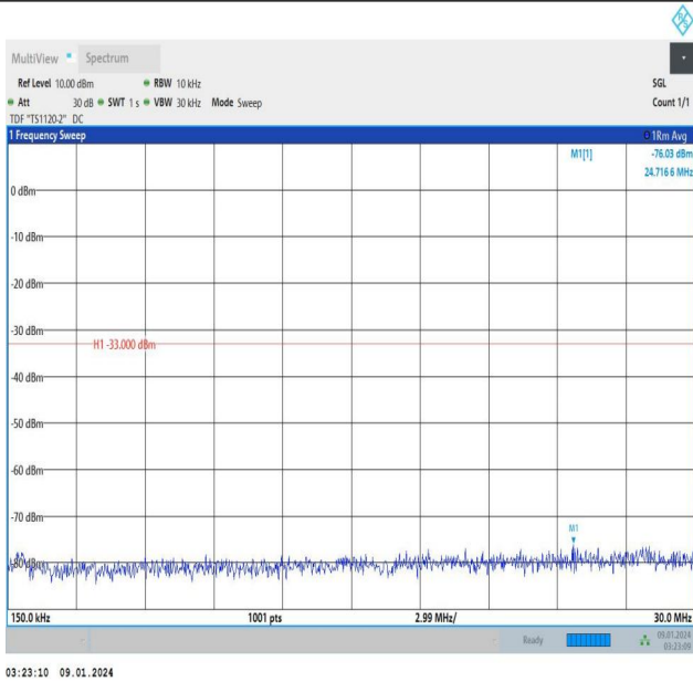
Band25_5MHz_16QAM_26665_25RB#0_0.15~30_0.15~30
