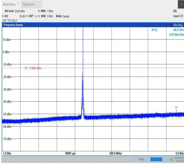
Band25_10MHz_16QAM_26365_1RB#49_1000~3000_1000~3000
