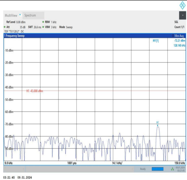
Band25_5MHz_16QAM_26665_1RB#24_0.009~0.15_0.009~0 .15
