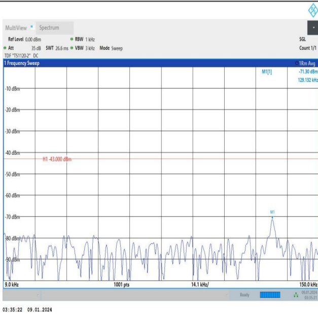
Band25_15MHz_16QAM_26115_1RB#0_0.009~0.15_0.009~0.15 .15
