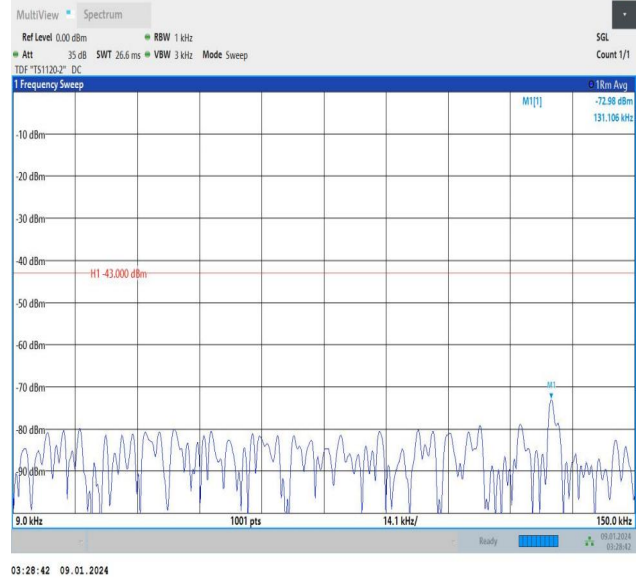
Band25_10MHz_16QAM_26365_1RB#49_0.009~0.15_0.009~0.15
