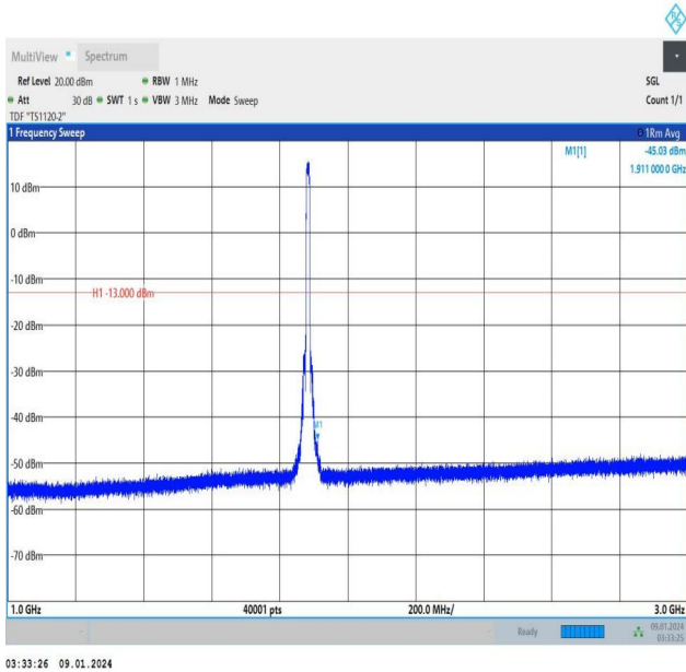
Band25_10MHz_QPSK_26365_50RB#0_1000~3000_1000~3000
