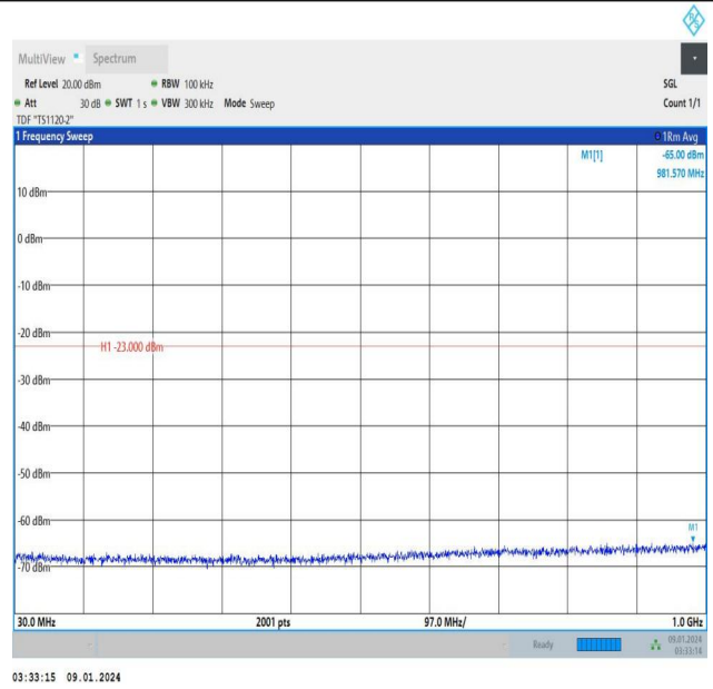
Band25_10MHz_QPSK_26365_50RB#0_30~1000_30~1000
