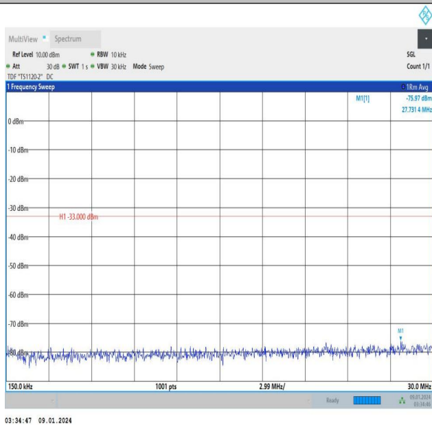
Band25_15MHz_QPSK_26115_1RB#0_0.15~30_0.15~30
