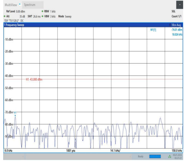
Band25_10MHz_16QAM_26640_1RB#49_0.009~0.15_0.009~ 0.15
