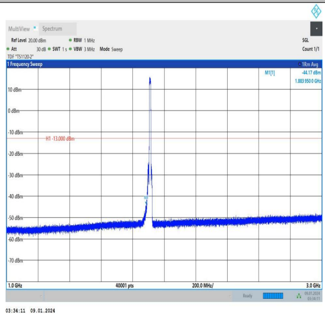
Band25_10MHz_QPSK_26640_50RB#0_1000~3000_1000~3000
