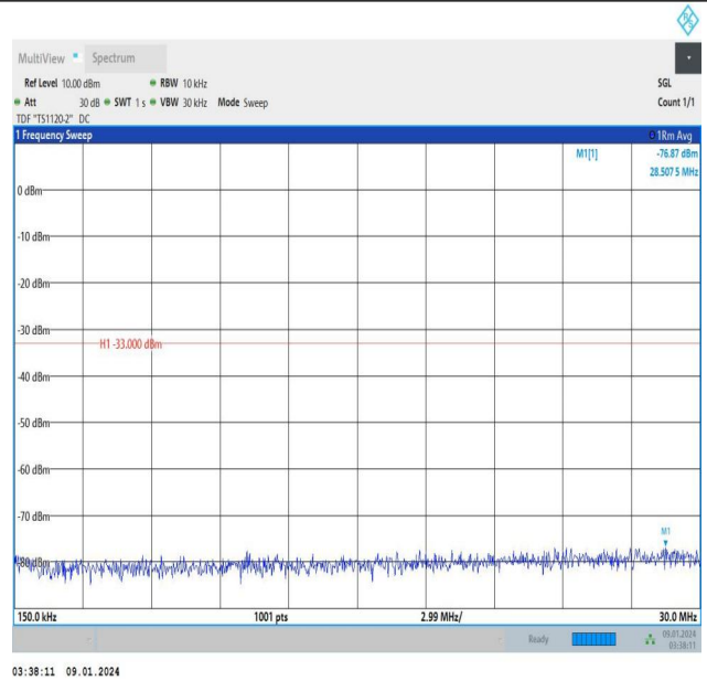
Band25_15MHz_16QAM_26365_1RB#0_0.15~30_0.15~30
