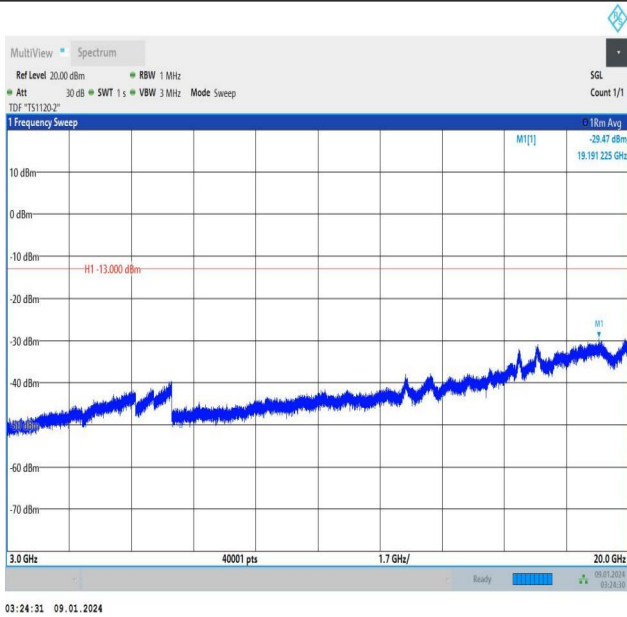
Band25_10MHz_QPSK_26090_1RB#0_3000~20000_3000~20000
