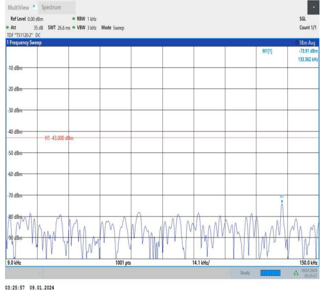
Band25_10MHz_16QAM_26090_1RB#49_0.009~0.15_0.009~0.15
