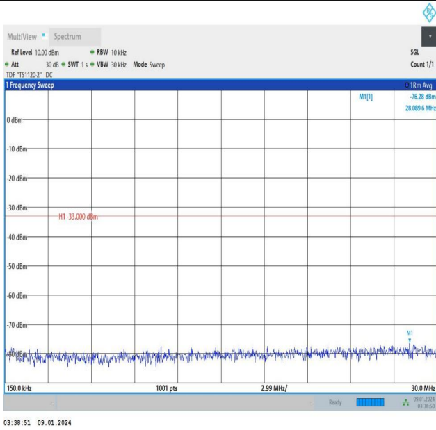
Band25_15MHz_QPSK_26365_1RB#74_0.15~30_0.15~30
