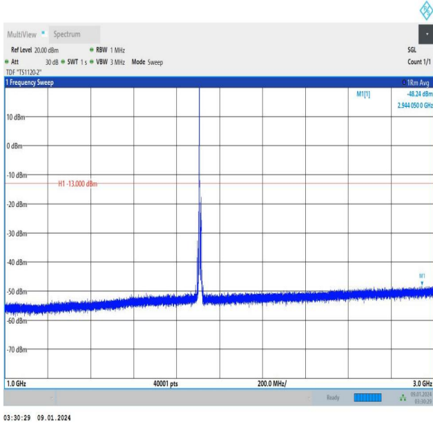
Band25_10MHz_16QAM_26640_1RB#0_1000~3000_1000~3000
