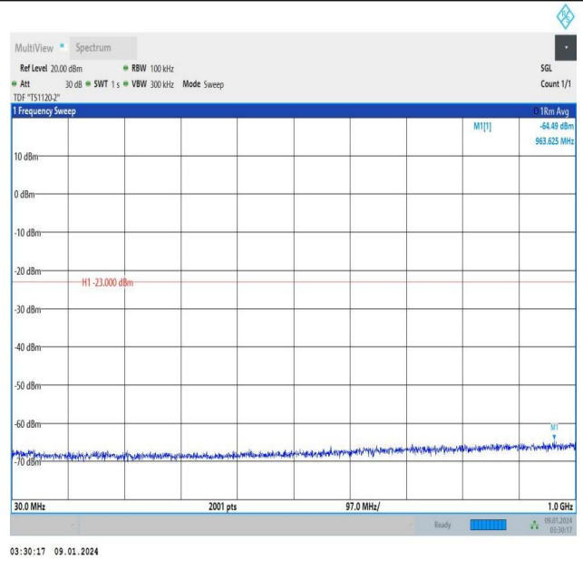
Band25_10MHz_16QAM_26640_1RB#0_30~1000_30~1000
