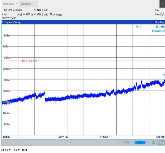
Band25_10MHz_QPSK_26090_1RB#49_3000~20000_3000~20000
