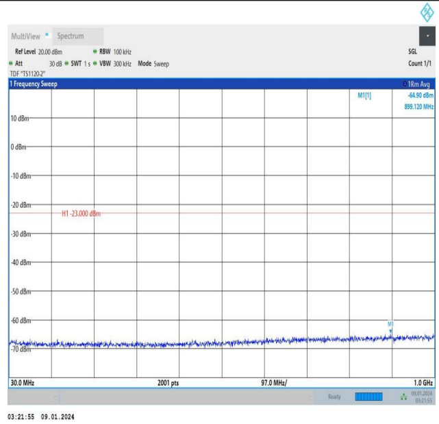
Band25_5MHz_16QAM_26665_1RB#24_30~1000_30~1000
