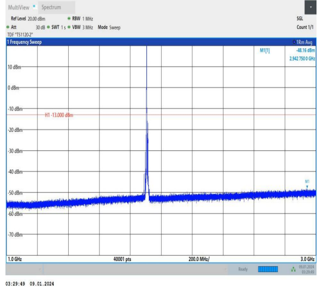
Band25_10MHz_QPSK_26640_1RB#0_1000~3000_1000~3000
