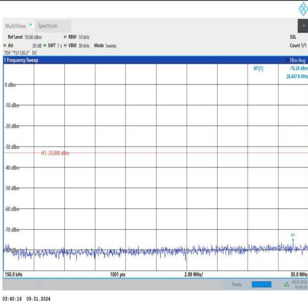
Band25_15MHz_QPSK_26615_1RB#0_0.15~30_0.15~30
