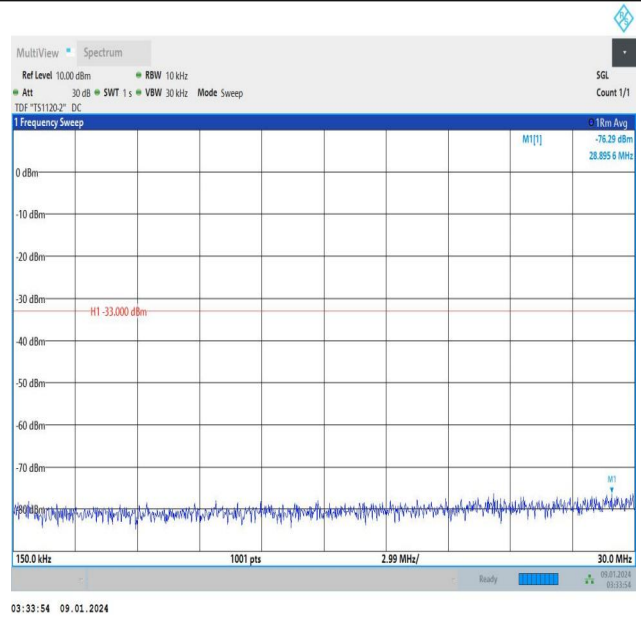
Band25_10MHz_QPSK_26640_50RB#0_0.15~30_0.15~30
