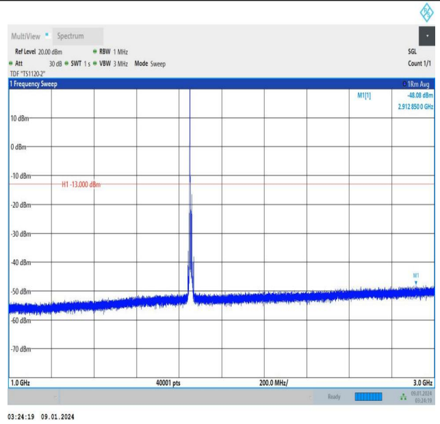
Band25_10MHz_QPSK_26090_1RB#0_1000~3000_1000~3000
