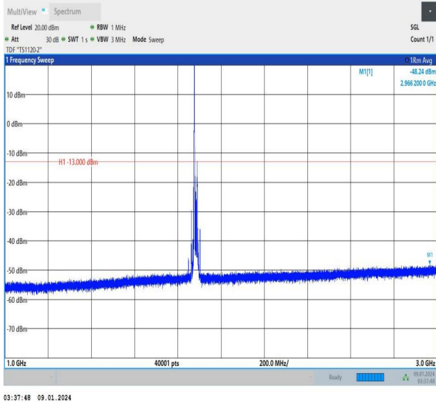
Band25_15MHz_QPSK_26365_1RB#0_1000~3000_1000~30 00
