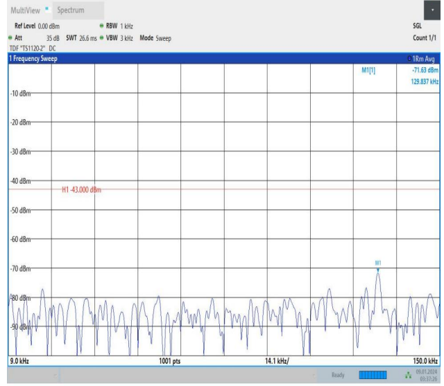
Band25_15MHz_QPSK_26365_1RB#0_0.009~0.15_0.009~0.15
