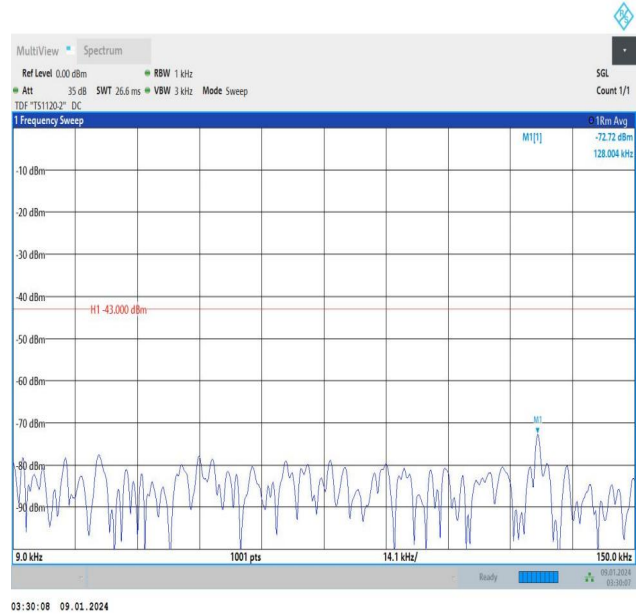
Band25_10MHz_16QAM_26640_1RB#0_0.009~0.15_0.009~0.15
