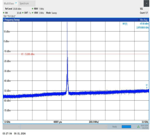
Band25_10MHz_QPSK_26365_1RB#0_1000~3000_1000~3000
