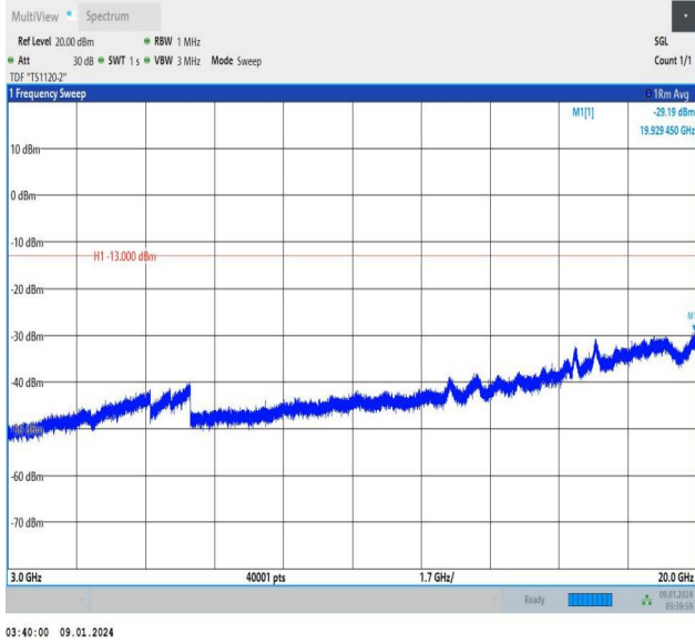
Band25_15MHz_16QAM_26365_1RB#74_3000~20000_3000~20000
