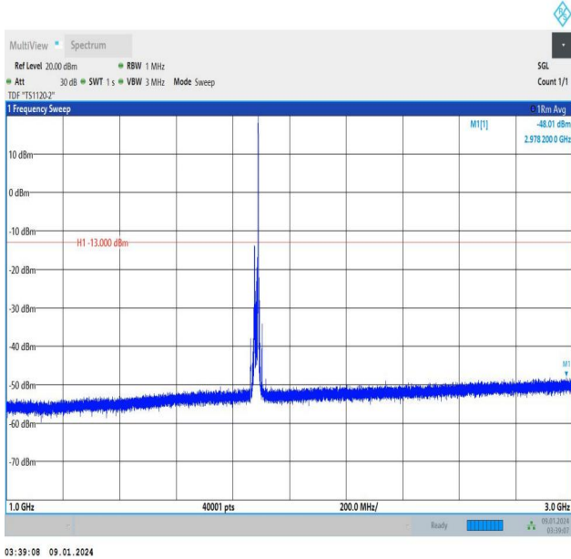
Band25_15MHz_QPSK_26365_1RB#74_1000~3000_1000~3000
