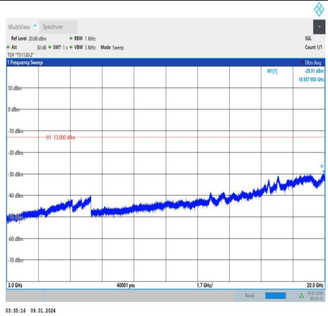
Band25_15MHz_QPSK_26115_1RB#0_3000~20000_3000~20000 000
