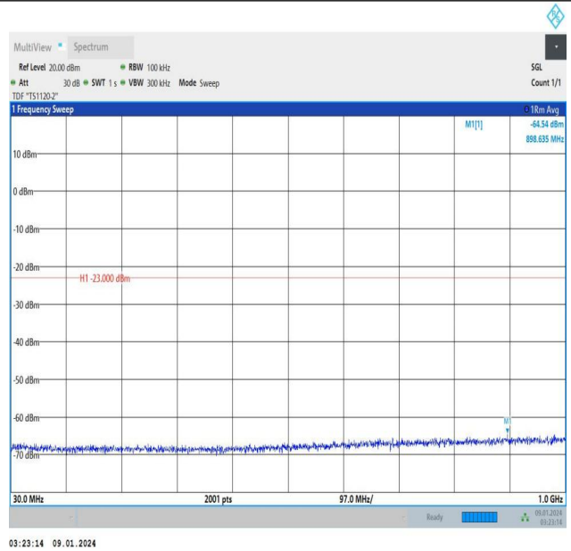
Band25_5MHz_16QAM_26665_25RB#0_30~1000_30~1000
