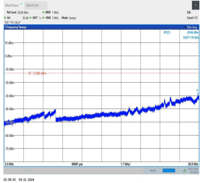
Band25_15MHz_QPSK_26365_1RB#0_3000~20000_3000~2 0000
