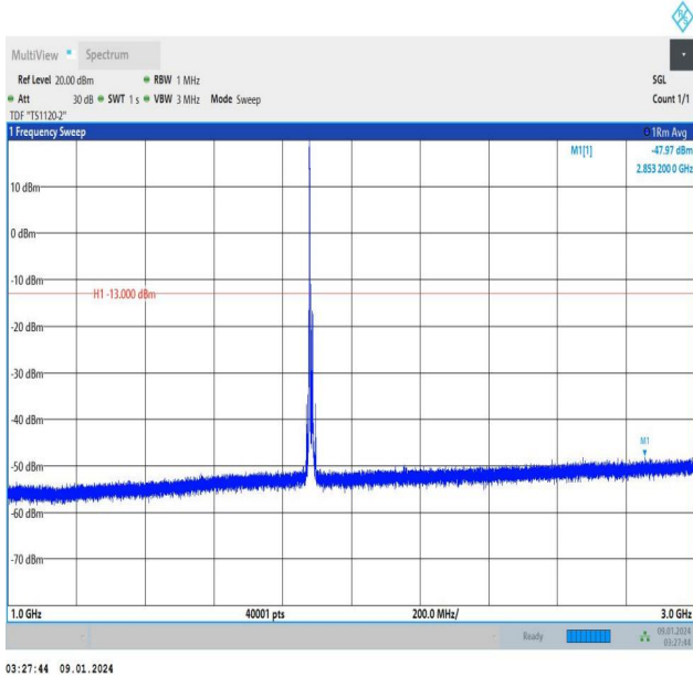
Band25_10MHz_16QAM_26365_1RB#0_1000~3000_1000~3000
