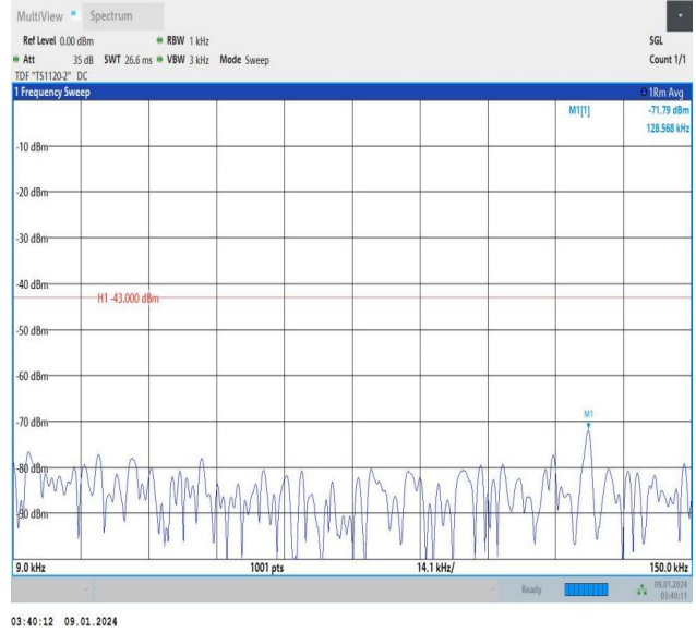
Band25_15MHz_QPSK_26615_1RB#0_0.009~0.15_0.009~0.15
