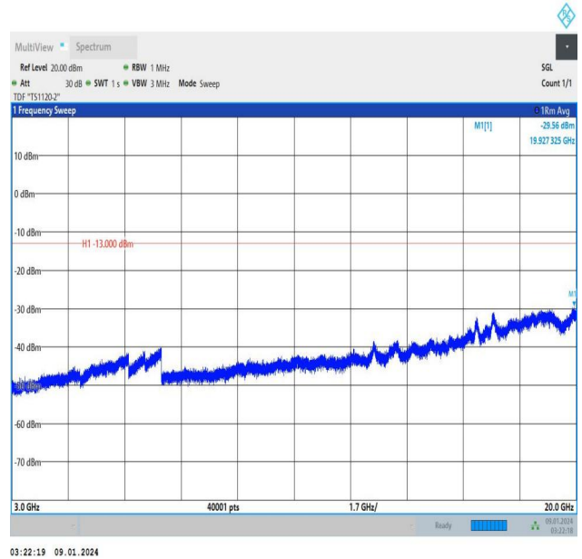
Band25_5MHz_16QAM_26665_1RB#24_3000~20000_3000~20000
