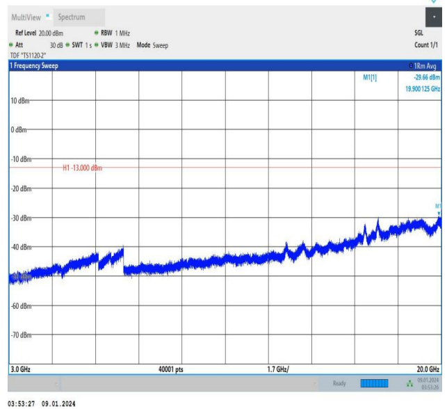
Band25_20MHz_16QAM_26590_1RB#99_3000~20000_3000~20000
