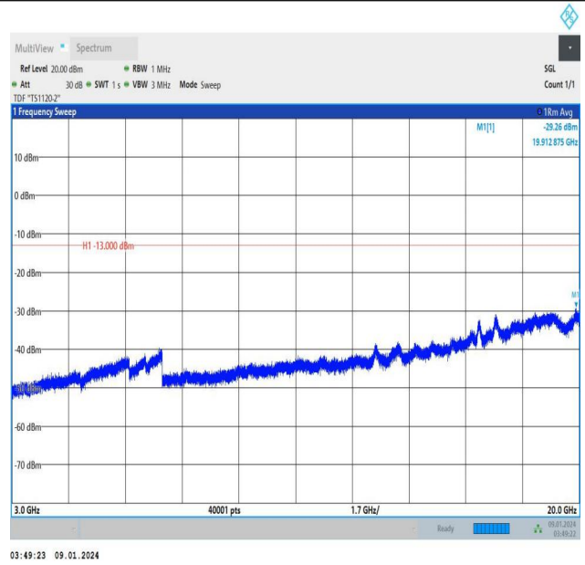
Band25_20MHz_16QAM_26365_1RB#0_3000~20000_3000~20000
