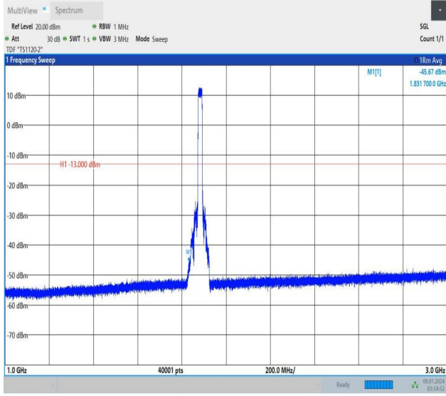
Band25_20MHz_QPSK_26365_100RB#0_1000~3000_1000~3000
