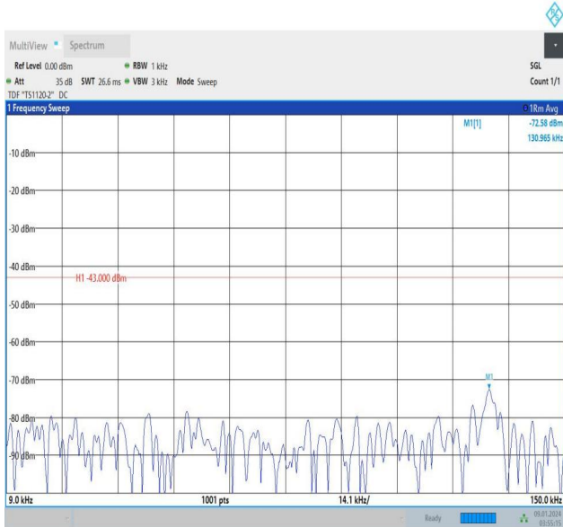
Band25_20MHz_QPSK_26365_100RB#0_1000~3000_1000~3000
