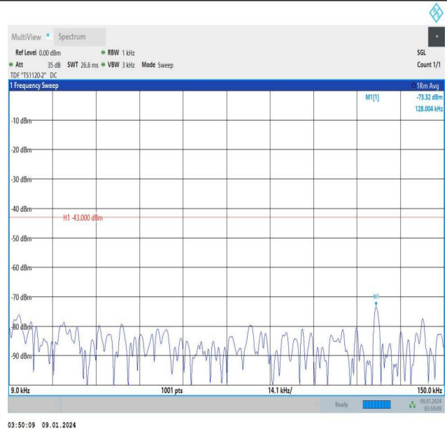
Band25_20MHz_16QAM_26365_1RB#99_0.009~0.15_0.009~0.15
