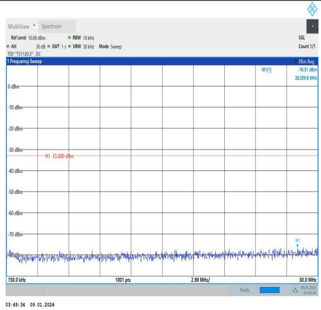
Band25_20MHz_QPSK_26365_1RB#99_0.15~30_0.15~30
