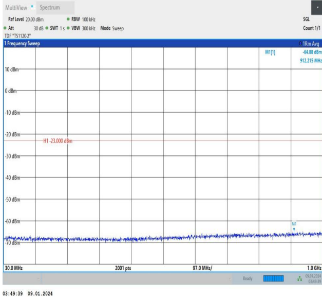
Band25_20MHz_QPSK_26365_1RB#99_30~1000_30~1000
