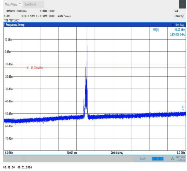
Band25_20MHz_QPSK_26590_1RB#99_1000~3000_1000~3000
