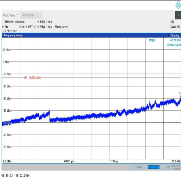
Band25_20MHz_QPSK_26365_1RB#99_3000~20000_3000~20000
