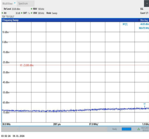
Band25_20MHz_QPSK_26590_1RB#99_30~1000_30~1000
