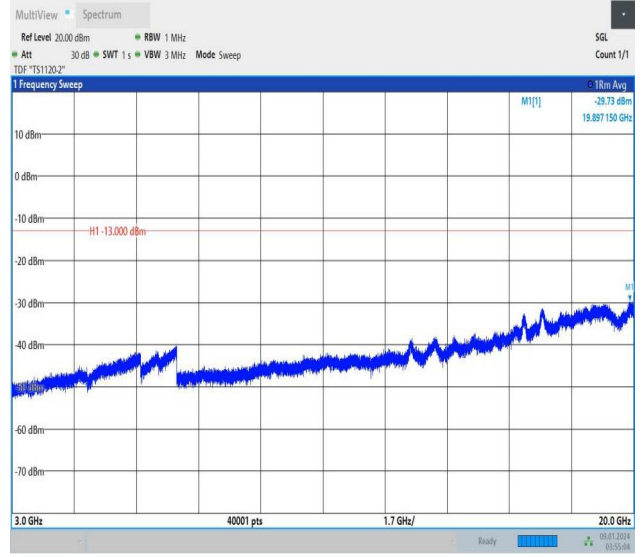
Band25_20MHz_QPSK_26365_100RB#0_3000~20000_3000~20000
