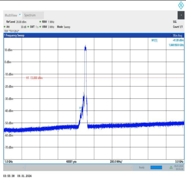
Band25_20MHz_QPSK_26590_100RB#0_1000~3000_1000~3000
