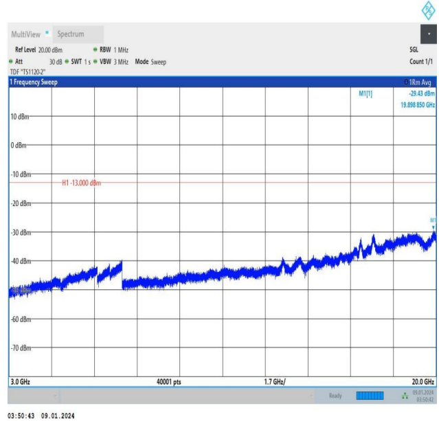
Band25_20MHz_16QAM_26365_1RB#99_3000~20000_3000~20000
