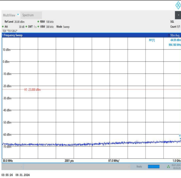
Band25_20MHz_QPSK_26590_100RB#0_30~1000_30~1000
