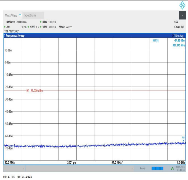
Band25_20MHz_16QAM_26140_1RB#99_30~1000_30~1000
