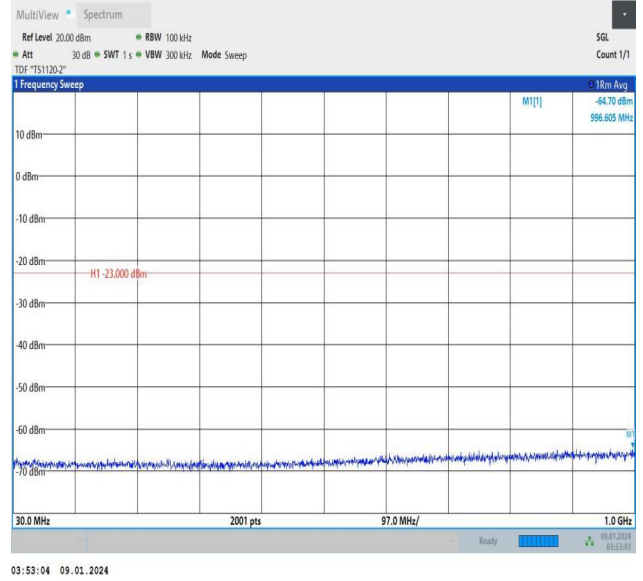
Band25_20MHz_16QAM_26590_1RB#99_30~1000_30~1000
