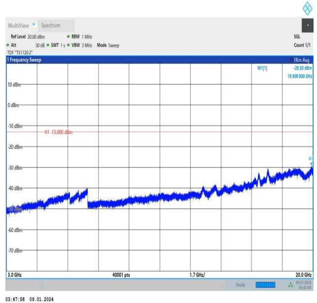
Band25_20MHz_16QAM_26140_1RB#99_3000~20000_3000~20000
