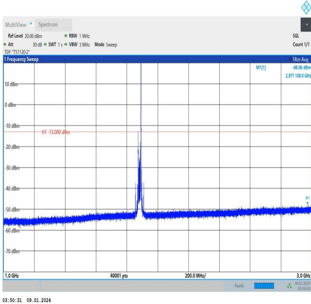
Band25_20MHz_16QAM_26365_1RB#99_1000~3000_1000~3000
