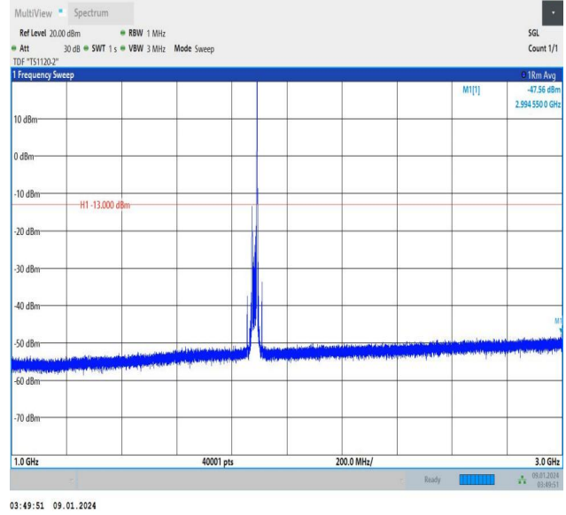
Band25_20MHz_QPSK_26365_1RB#99_1000~3000_1000~3000
