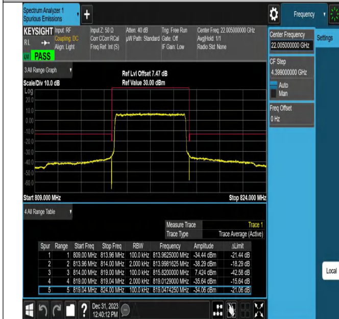
Band26_5MHz_QPSK_26715_25RB#0
