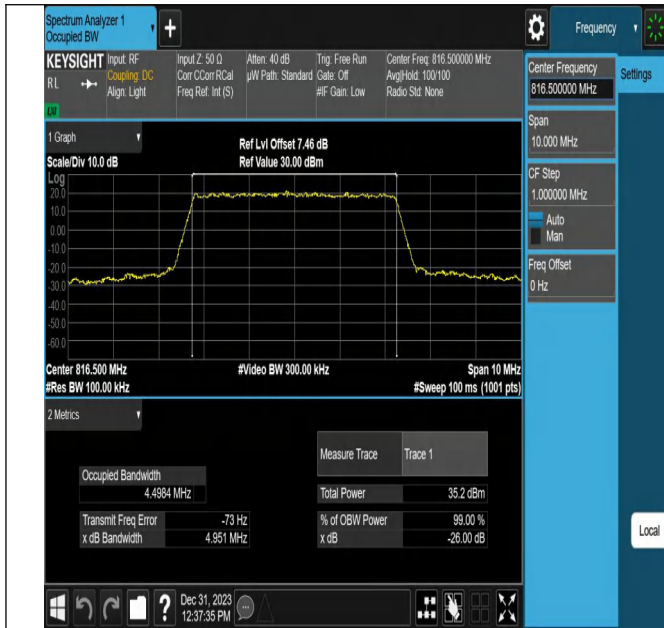
26(814-824)-5MHz-QPSK-26715-25RB#0-PASS
