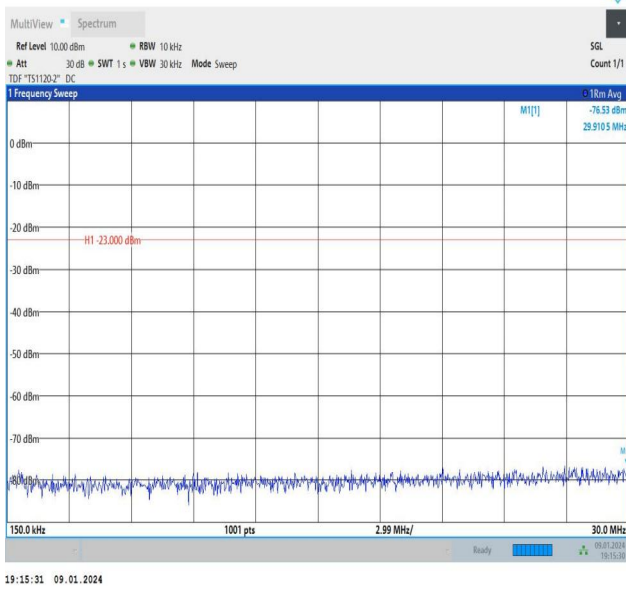
Band26_1.4MHz_16QAM_26697_1RB#5_0.15~30_0.15~30
