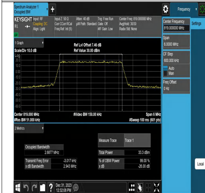
26(814-824)-3MHz-16QAM-26740-15RB#0-PASS
