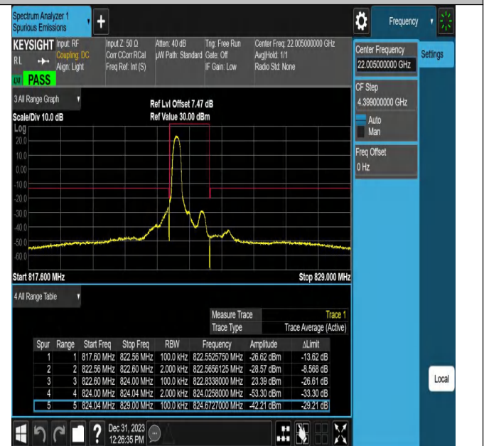
Band26_1.4MHz_QPSK_26783_1RB#0
