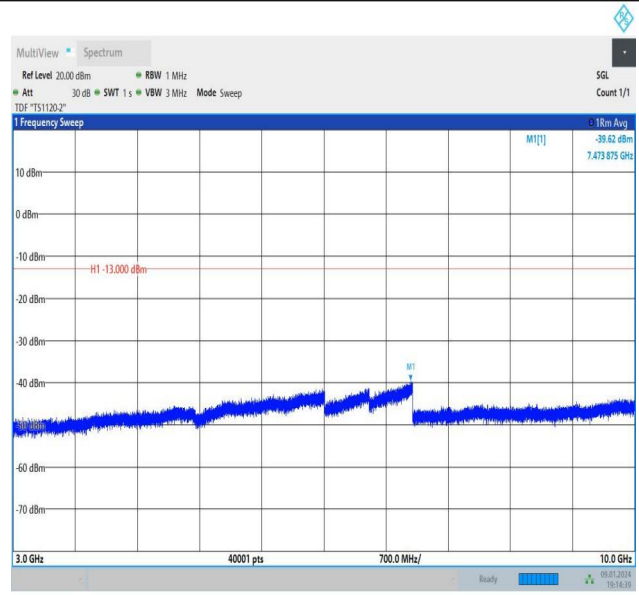
Band26_1.4MHz_16QAM_26697_1RB#0_3000~10000_3000~10000
