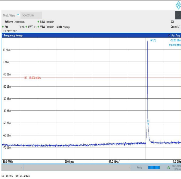
Band26_1.4MHz_QPSK_26697_1RB#5_30~1000_30~1000
