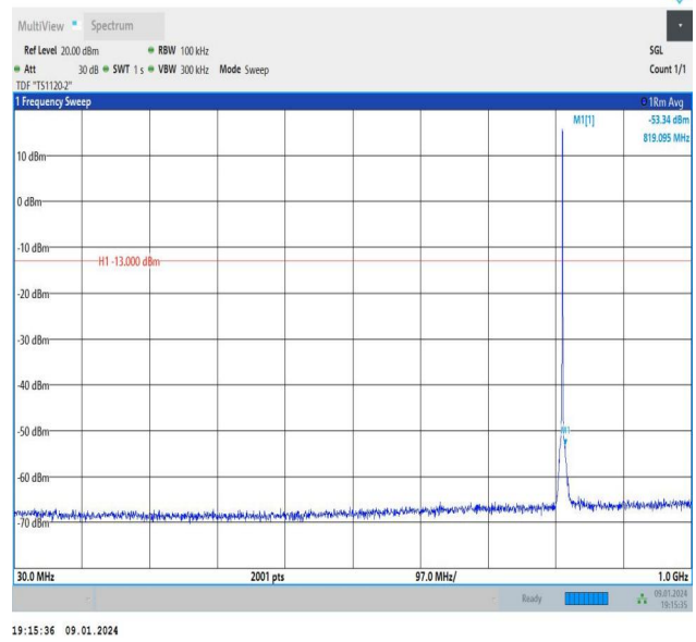
Band26_1.4MHz_16QAM_26697_1RB#5_30~1000_30~1000
