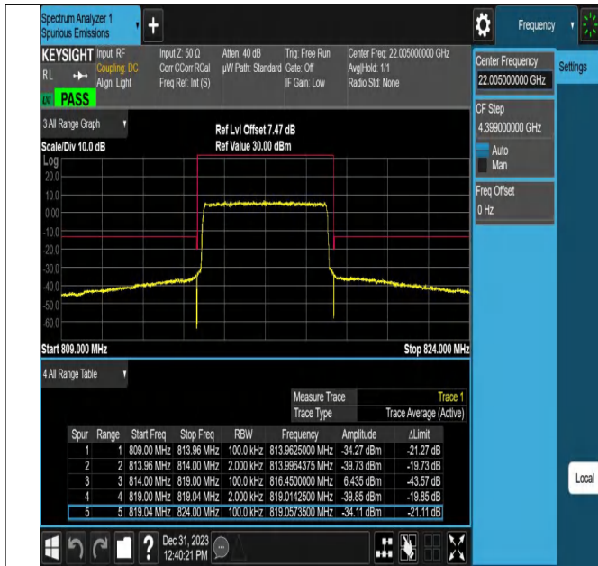
Band26_5MHz_16QAM_26715_25RB#0
