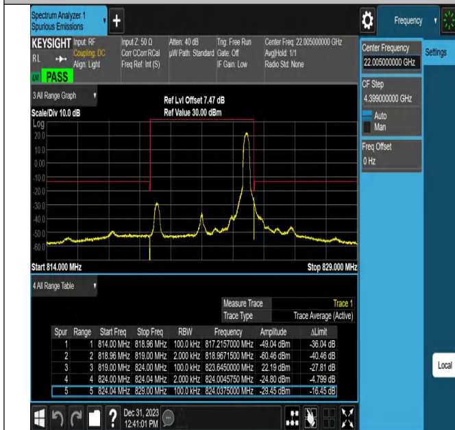
Band26_5MHz_16QAM_26765_1RB#24
