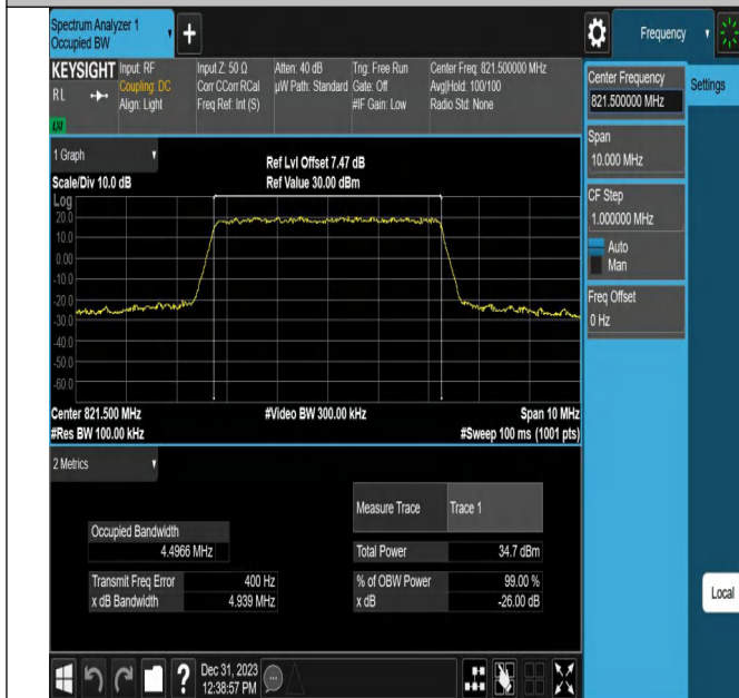
26(814-824)-5MHz-QPSK-26765-25RB#0-PASS
