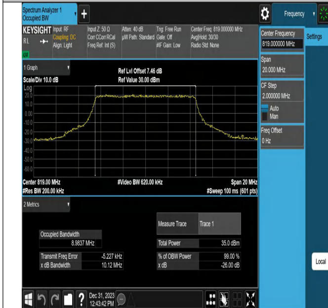
26(814-824)-10MHz-QPSK-26740-50RB#0-PASS
