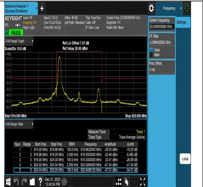
Band26_5MHz_QPSK_26765_1RB#0
