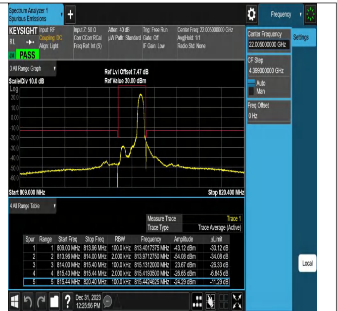
Band26_1.4MHz_QPSK_26697_1RB#5
