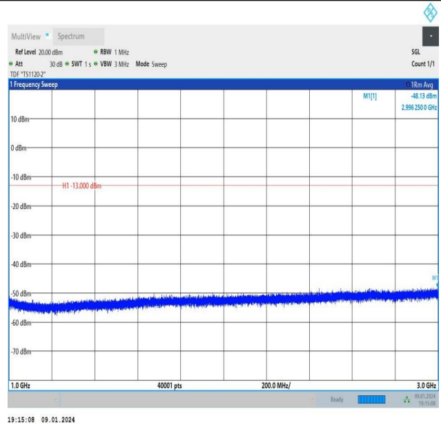
Band26_1.4MHz_QPSK_26697_1RB#5_1000~3000_1000~3000
