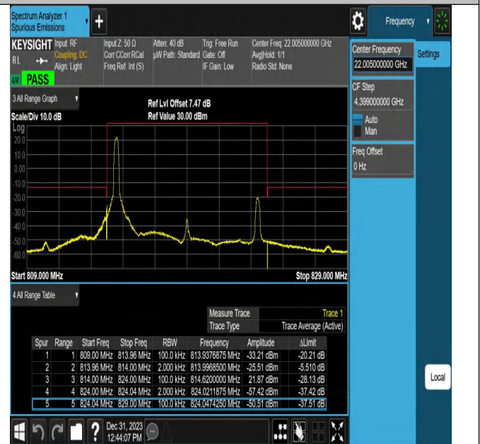
Band26_10MHz_16QAM_26740_1RB#0
