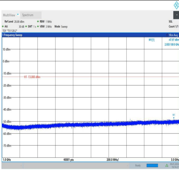
Band26_1.4MHz_16QAM_26697_1RB#0_1000~3000_1000~3000
