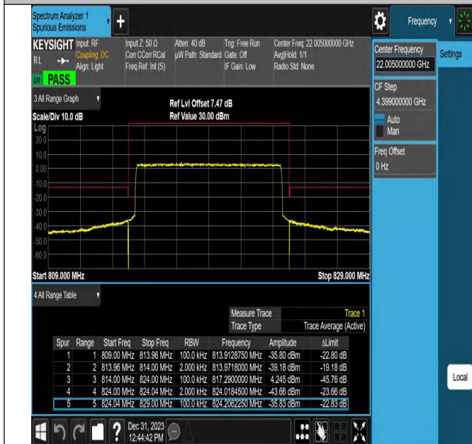
Band26_10MHz_QPSK_26740_50RB#0
