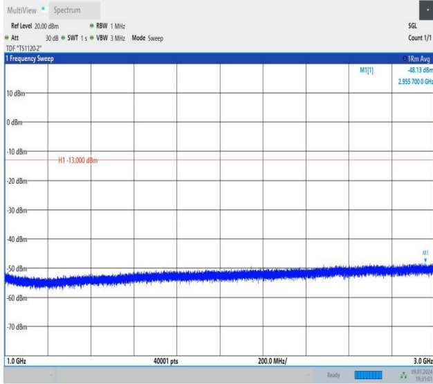
Band26_3MHz_16QAM_26740_1RB#0_1000~3000_1000~3000
