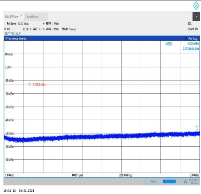
Band26_3MHz_QPSK_26740_1RB#14_1000~3000_1000~300 0
