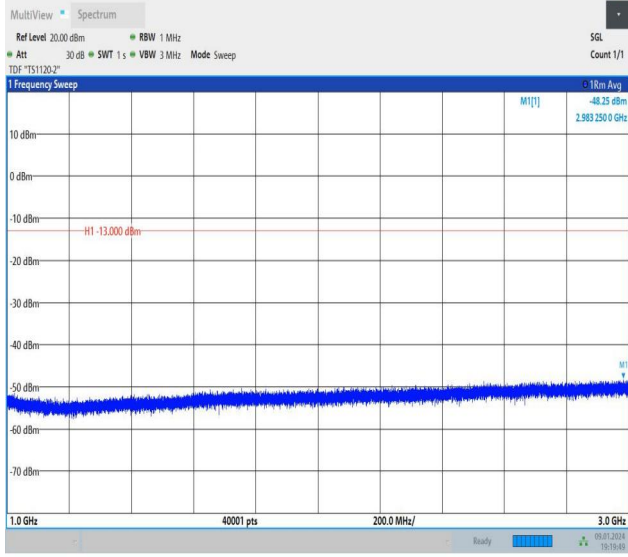
Band26_1.4MHz_16QAM_26740_1RB#5_1000~3000_1000~3000
