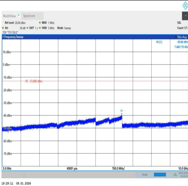
Band26_3MHz_QPSK_26705_15RB#0_3000~10000_3000~1 0000
