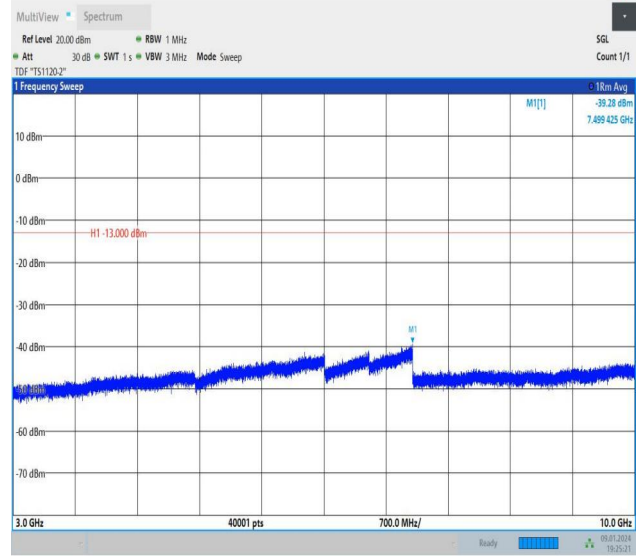
Band26_1.4MHz_16QAM_26783_6RB#0_3000~10000_3000~10000
