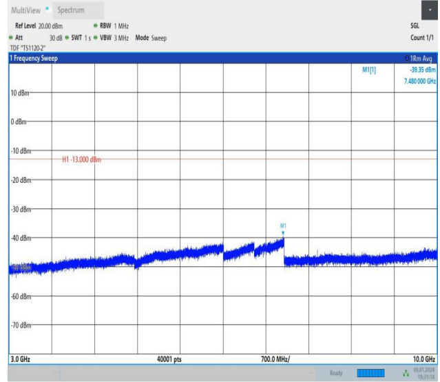
Band26_3MHz_16QAM_26740_1RB#0_3000~10000_3000~10000
