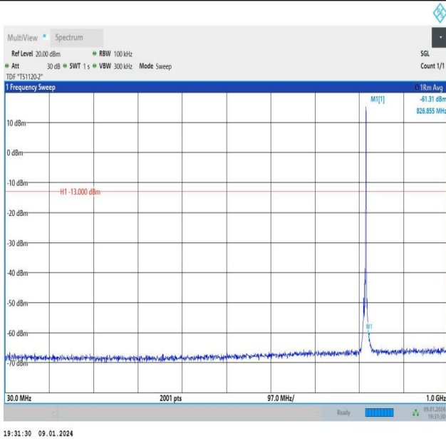
Band26_3MHz_QPSK_26740_1RB#14_30~1000_30~1000
