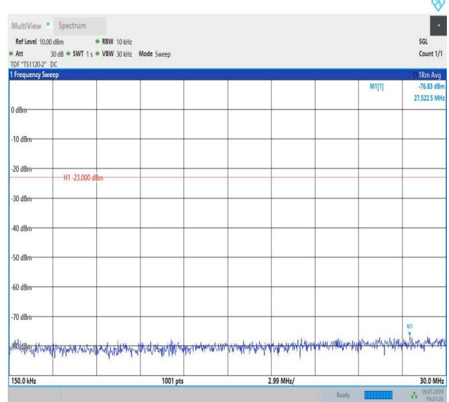
Band26_3MHz_QPSK_26740_1RB#14_0.15~30_0.15~30
