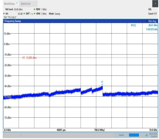
Band26_1.4MHz_16QAM_26740_1RB#5_3000~10000_3000~10000
