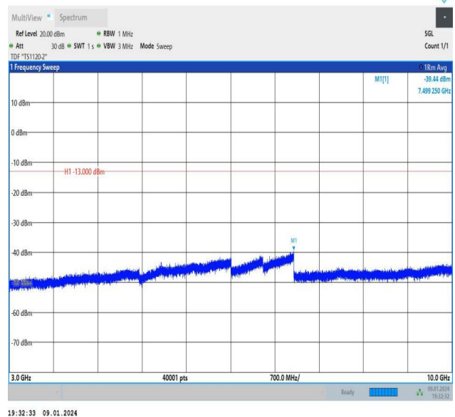
Band26_3MHz_16QAM_26740_1RB#14_3000~10000_3000~10000
