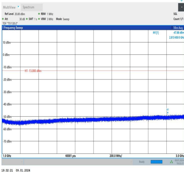
Band26_3MHz_16QAM_26740_1RB#14_1000~3000_1000~3000
