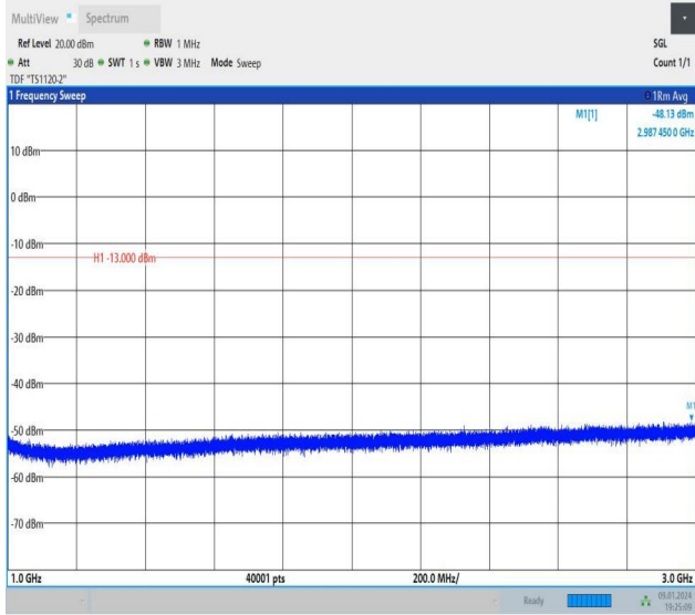
Band26_1.4MHz_16QAM_26783_6RB#0_1000~3000_1000~3000
