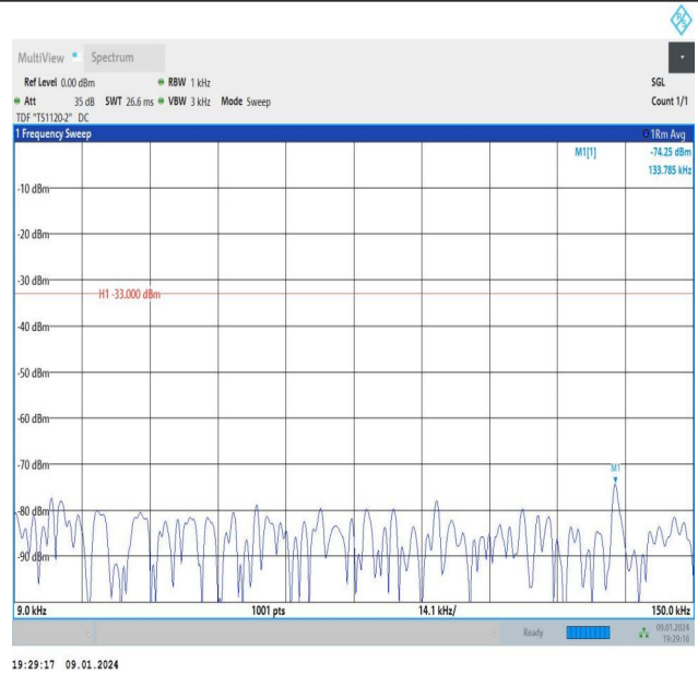
Band26_3MHz_16QAM_26705_15RB#0_0.009~0.15_0.009~0. 15
