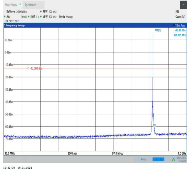
Band26_3MHz_16QAM_26740_1RB#14_30~1000_30~1000
