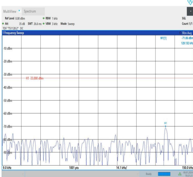
Band26_3MHz_QPSK_26740_1RB#14_0.009~0.15_0.009~0.15
