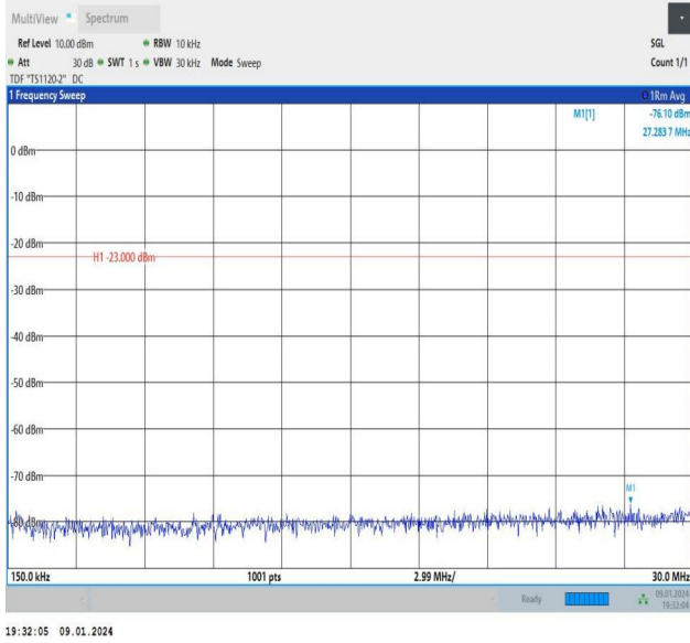
Band26_3MHz_16QAM_26740_1RB#14_0.15~30_0.15~30
