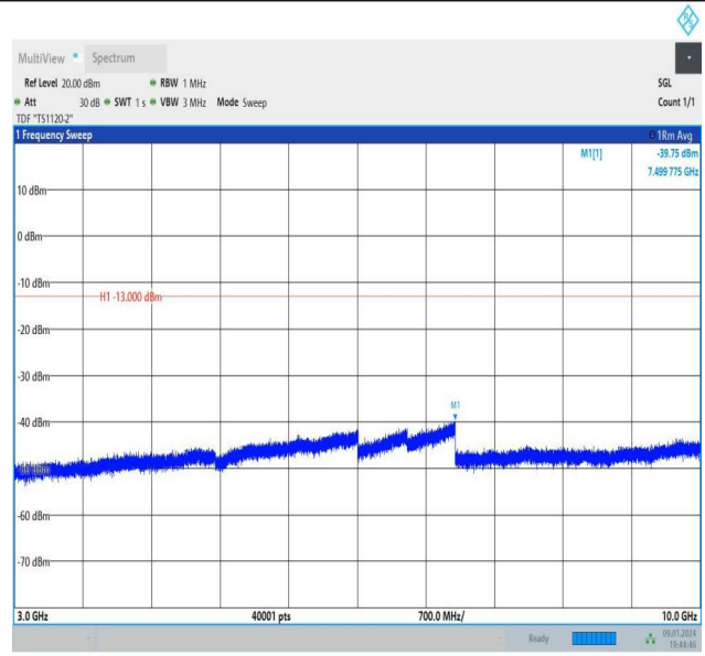
Band26_5MHz_16QAM_26740_1RB#24_3000~10000_3000~10000
