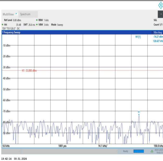
Band26_5MHz_QPSK_26740_1RB#0_0.009~0.15_0.009~0.15
