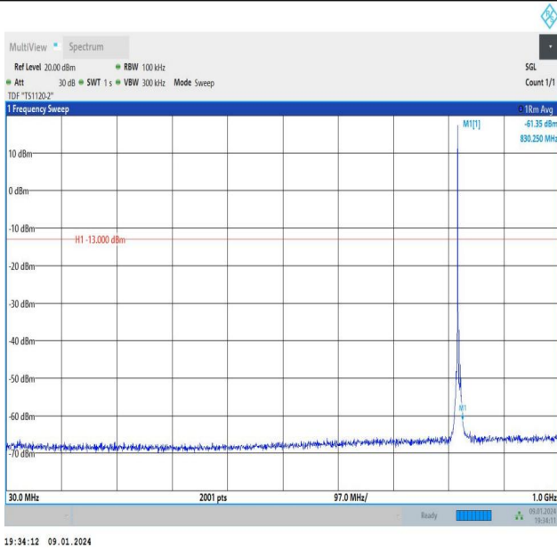
Band26_3MHz_QPSK_26775_1RB#0_30~1000_30~1000
