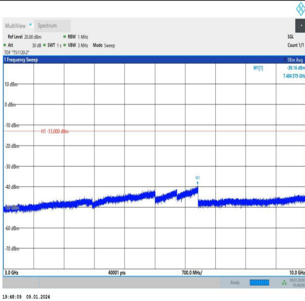
Band26_5MHz_QPSK_26765_1RB#24_3000~10000_3000~1 0000
