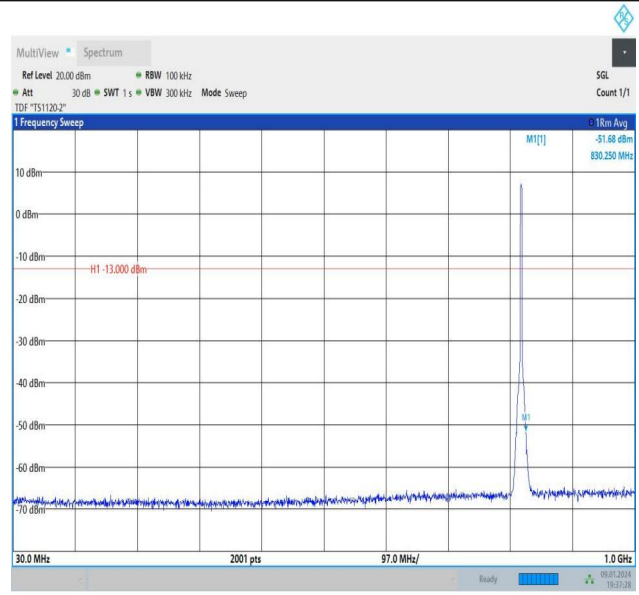
Band26_3MHz_16QAM_26775_15RB#0_30~1000_30~1000
