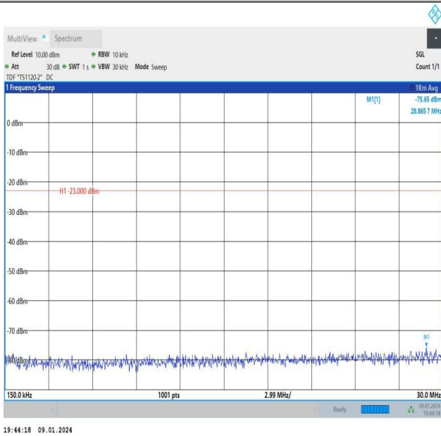
Band26_5MHz_16QAM_26740_1RB#24_0.15~30_0.15~30
