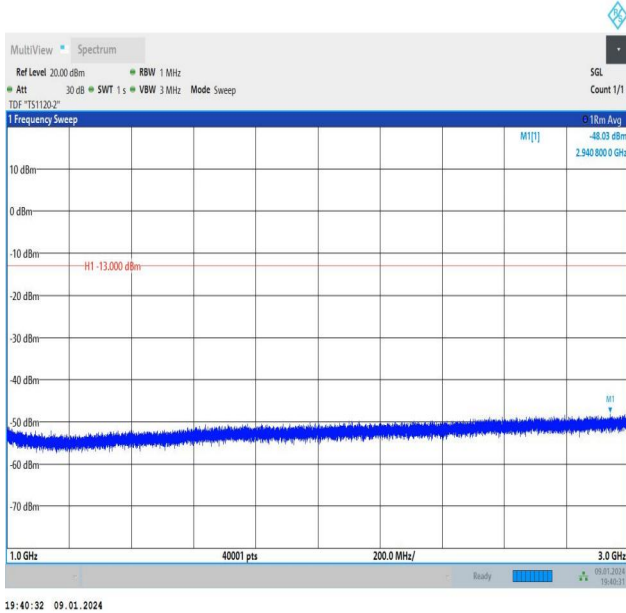
Band26_5MHz_16QAM_26715_1RB#24_1000~3000_1000~3000
