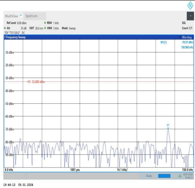
Band26_5MHz_16QAM_26740_1RB#24_0.009~0.15_0.009~0.15
