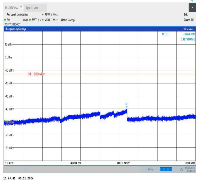
Band26_5MHz_16QAM_26765_1RB#24_3000~10000_3000~10000
