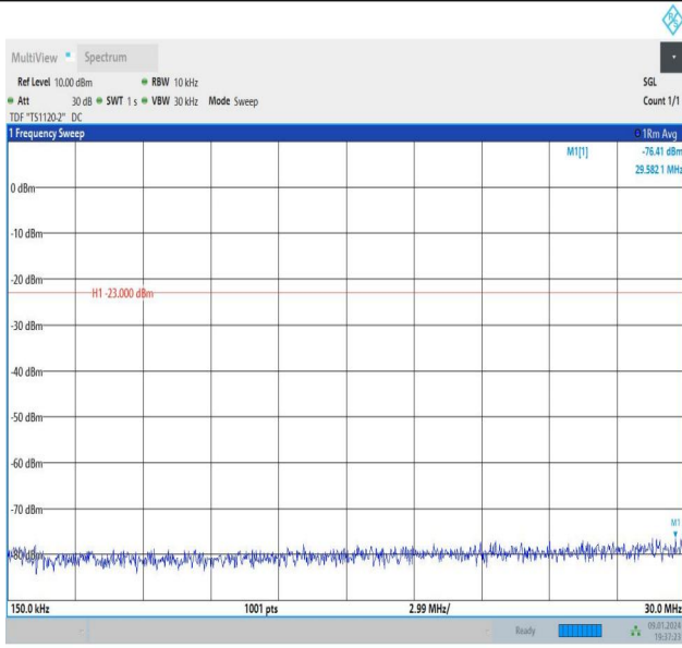
Band26_3MHz_16QAM_26775_15RB#0_0.15~30_0.15~30
