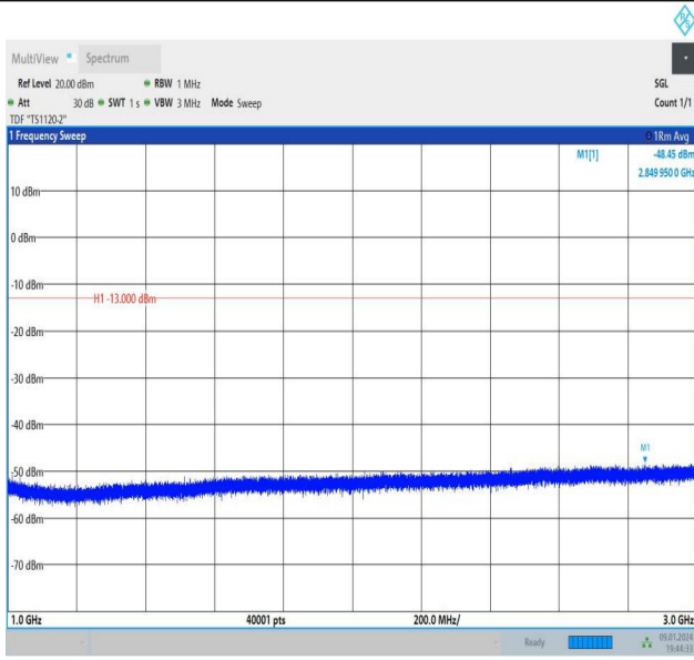
Band26_5MHz_16QAM_26740_1RB#24_1000~3000_1000~3000
