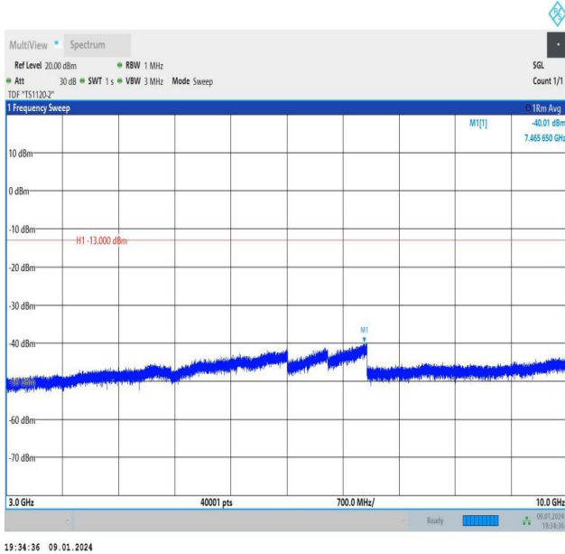
Band26_3MHz_QPSK_26775_1RB#0_3000~10000_3000~10000
