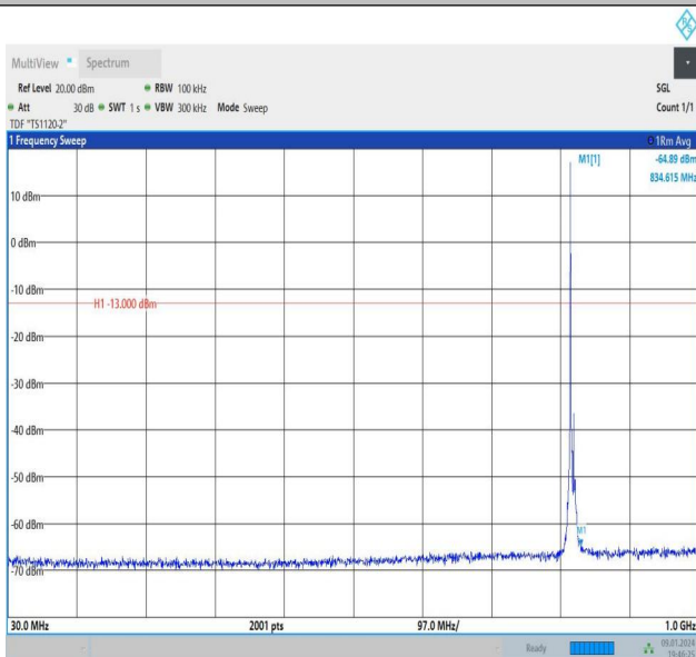
Band26_5MHz_QPSK_26765_1RB#0_30~1000_30~1000
