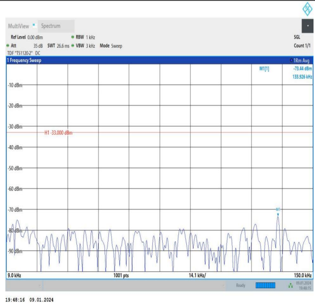
Band26_5MHz_16QAM_26765_1RB#24_0.009~0.15_0.009~0. 15
