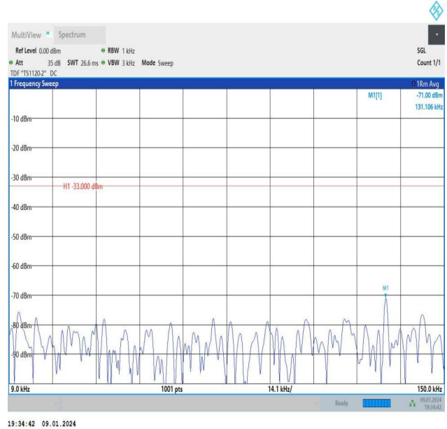
Band26_3MHz_16QAM_26775_1RB#0_0.009~0.15_0.009~0.1
