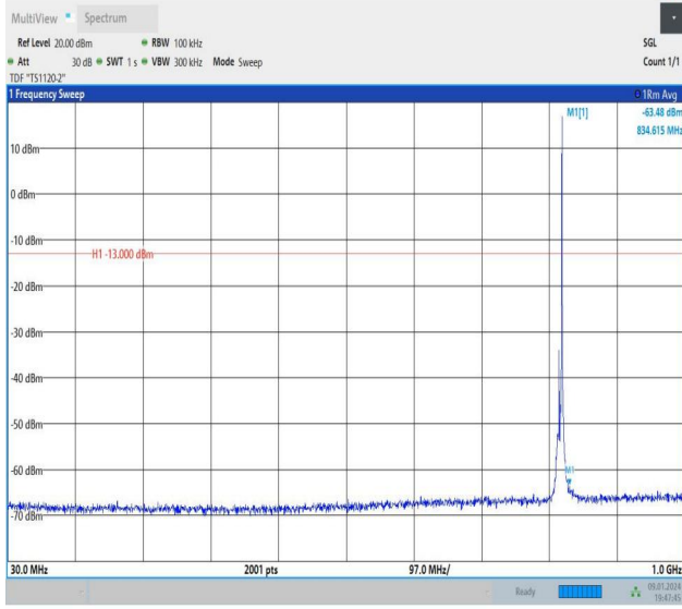
Band26_5MHz_QPSK_26765_1RB#24_30~1000_30~1000
