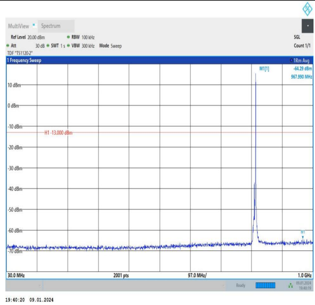
Band26_5MHz_16QAM_26715_1RB#24_30~1000_30~1000
