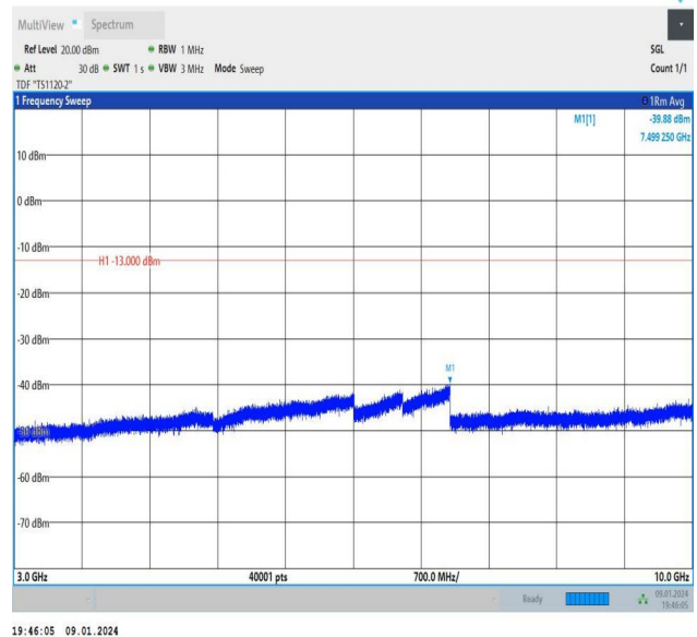
Band26_5MHz_16QAM_26740_25RB#0_3000~10000_3000~10000
