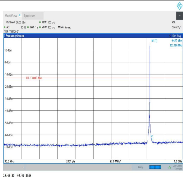
Band26_5MHz_16QAM_26740_1RB#24_30~1000_30~1000
