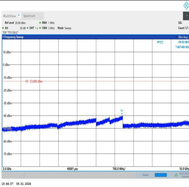
Band26_5MHz_QPSK_26740_1RB#24_3000~10000_3000~10000
