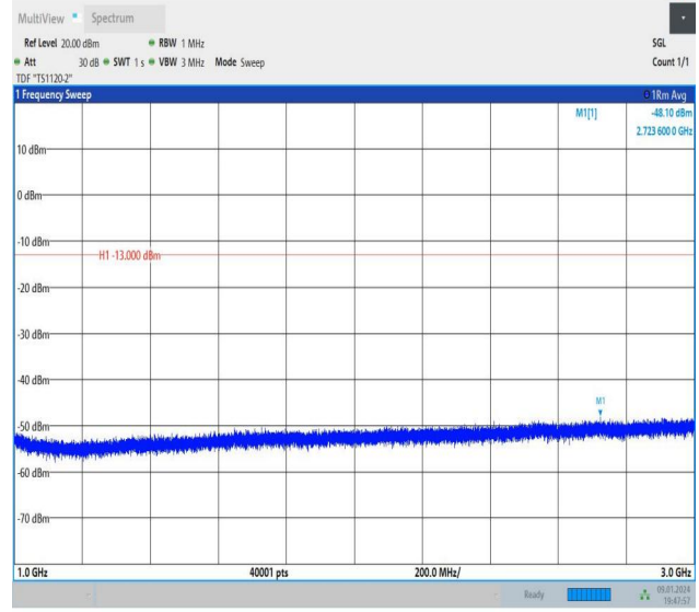
Band26_5MHz_QPSK_26765_1RB#24_1000~3000_1000~300 0
