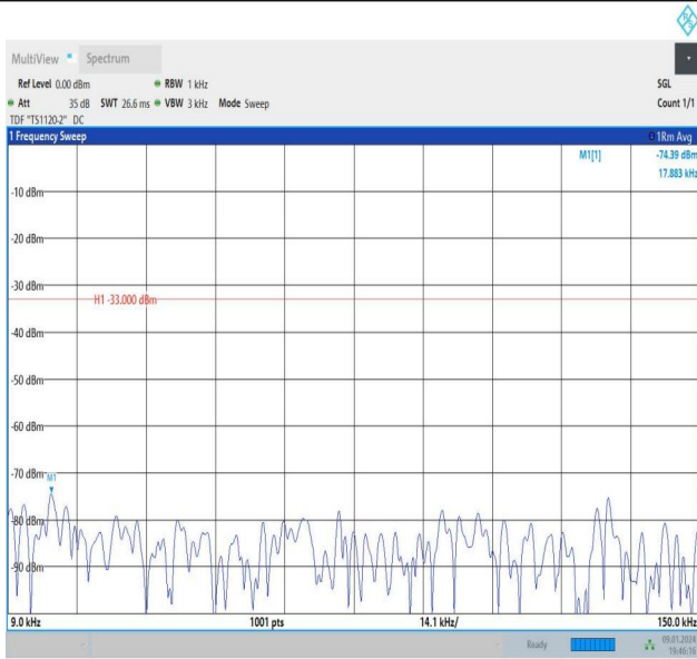
Band26_5MHz_QPSK_26765_1RB#0_0.009~0.15_0.009~0.1
