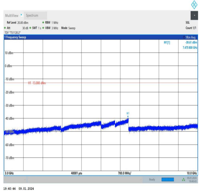
Band26_5MHz_16QAM_26715_1RB#24_3000~10000_3000~10000
