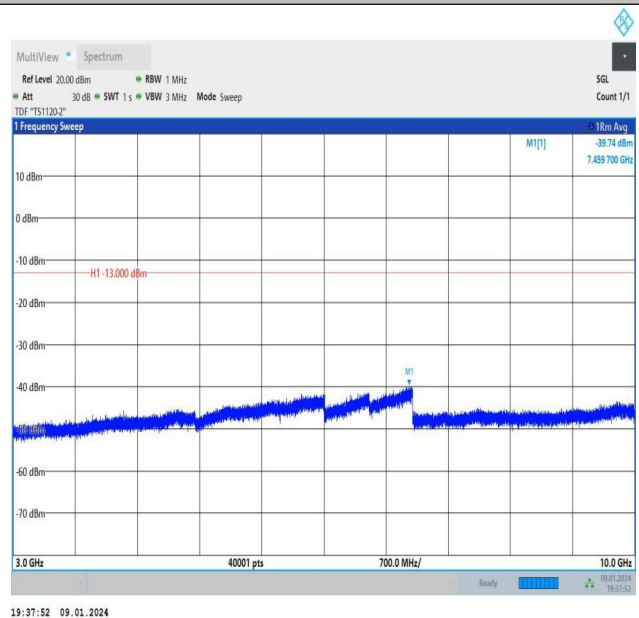
Band26_3MHz_16QAM_26775_15RB#0_3000~10000_3000~10000
