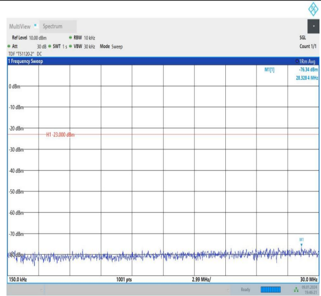
Band26_5MHz_QPSK_26765_1RB#0_0.15~30_0.15~30
