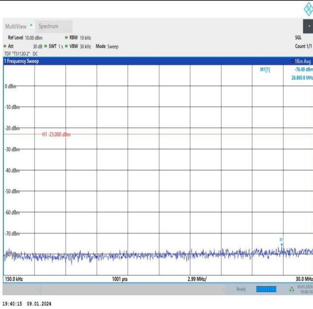
Band26_5MHz_16QAM_26715_1RB#24_0.15~30_0.15~30
