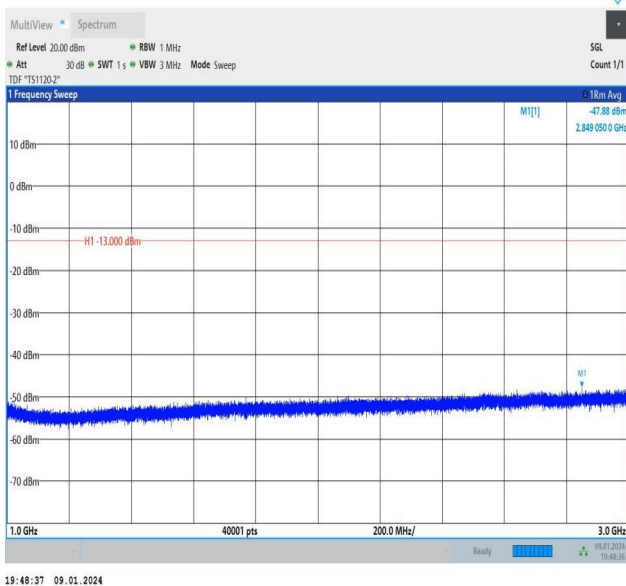
Band26_5MHz_16QAM_26765_1RB#24_1000~3000_1000~3000
