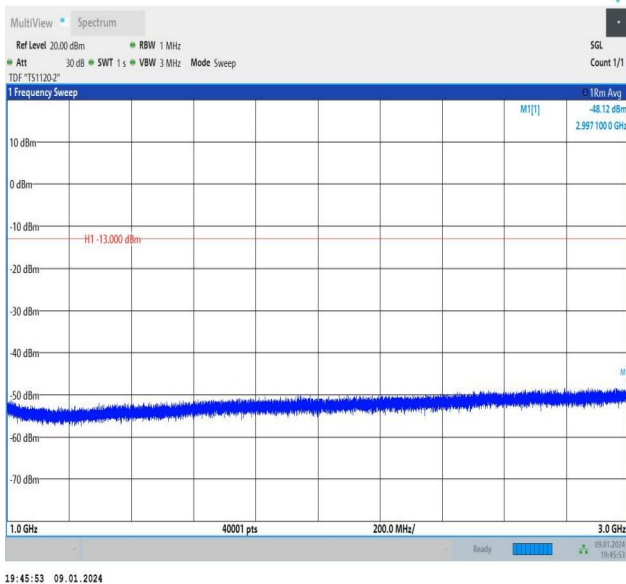
Band26_5MHz_16QAM_26740_25RB#0_1000~3000_1000~3000
