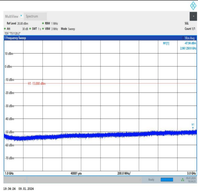
Band26_3MHz_QPSK_26775_1RB#0_1000~3000_1000~3000
