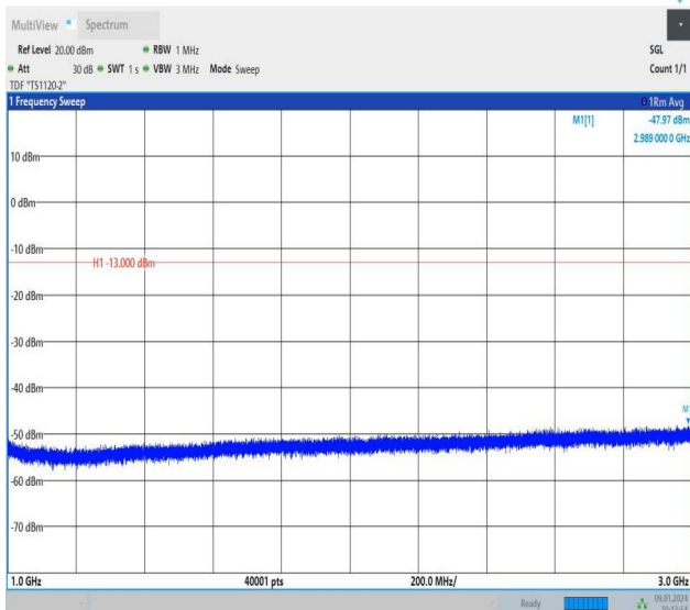
Band26_1.4MHz_16QAM_27033_1RB#5_1000~3000_1000~3000
