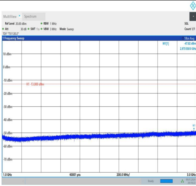
Band26_3MHz_16QAM_26805_1RB#14_1000~3000_1000~3000
