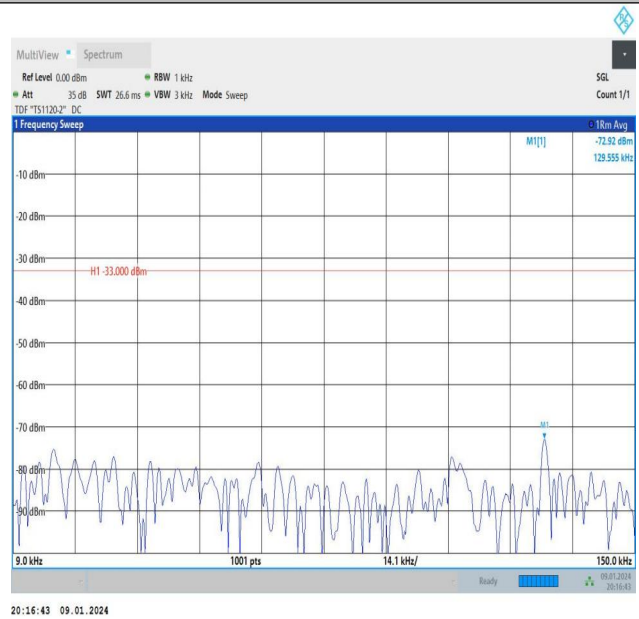
Band26_3MHz_16QAM_26805_1RB#0_0.009~0.15_0.009~0.
