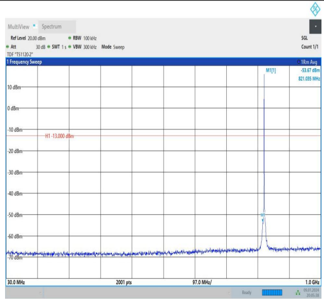
Band26_1.4MHz_16QAM_26797_1RB#5_30~1000_30~1000
