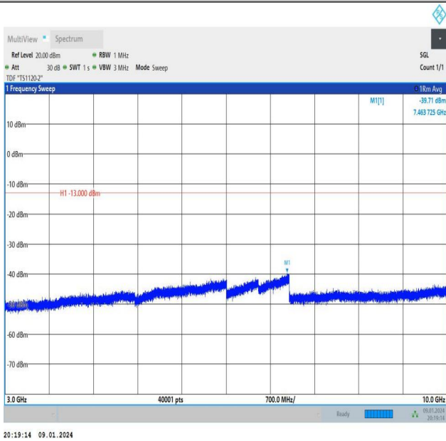
Band26_3MHz_QPSK_26805_15RB#0_3000~10000_3000~10000
