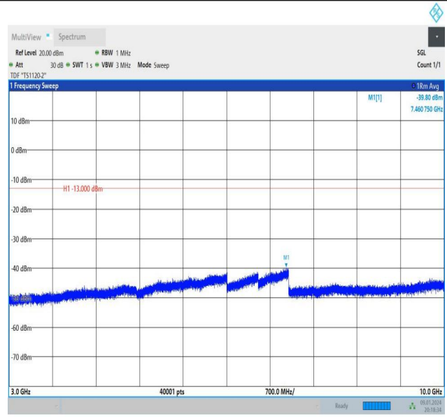
Band26_3MHz_16QAM_26805_1RB#14_3000~10000_3000~10000
