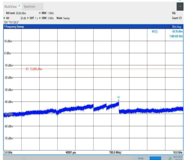
Band26_1.4MHz_16QAM_27033_1RB#5_3000~10000_3000~10000
