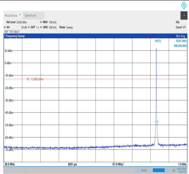
Band26_1.4MHz_16QAM_26915_6RB#0_30~1000_30~1000
