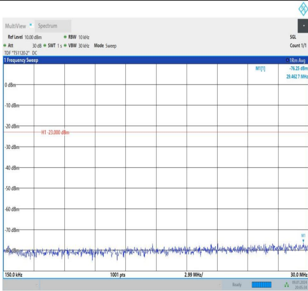
Band26_1.4MHz_16QAM_26797_1RB#5_0.15~30_0.15~30
