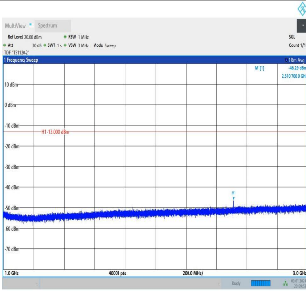
Band26_1.4MHz_16QAM_26915_1RB#5_1000~3000_1000~3000
