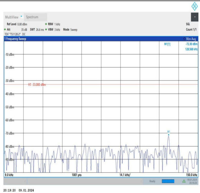
Band26_3MHz_16QAM_26805_15RB#0_0.009~0.15_0.009~0.15
