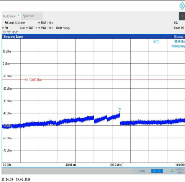
Band26_3MHz_QPSK_27025_1RB#0_3000~10000_3000~10000
