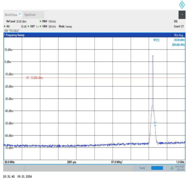
Band26_5MHz_16QAM_26815_25RB#0_30~1000_30~1000
