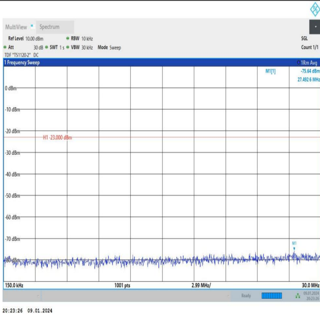
Band26_3MHz_16QAM_26915_15RB#0_0.15~30_0.15~30
