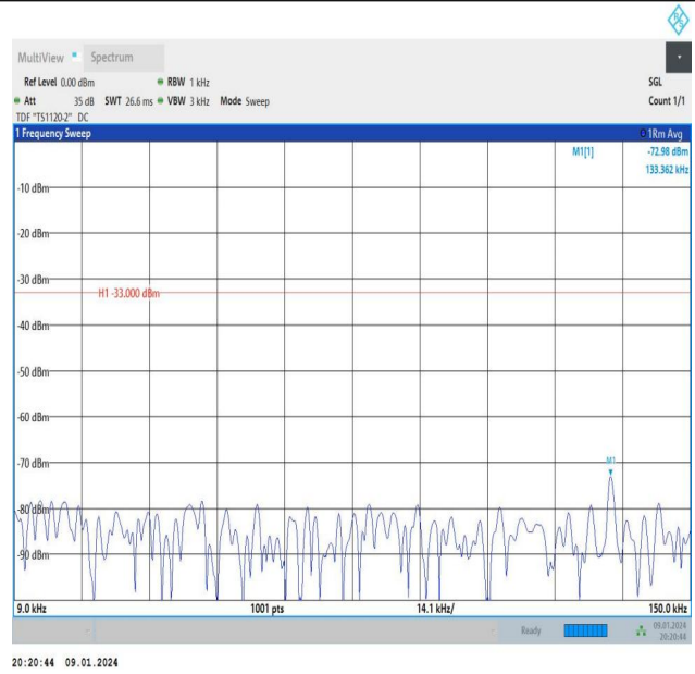
Band26_3MHz_16QAM_26915_1RB#0_0.009~0.15_0.009~0.15
