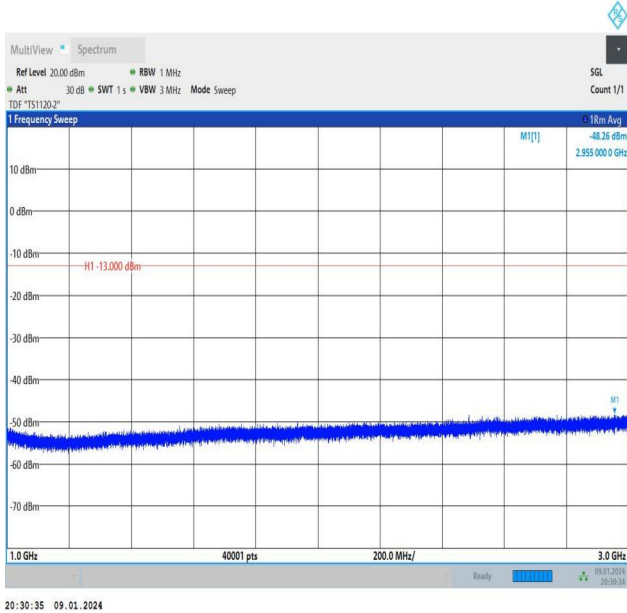
Band26_5MHz_16QAM_26815_1RB#24_1000~3000_1000~3000
