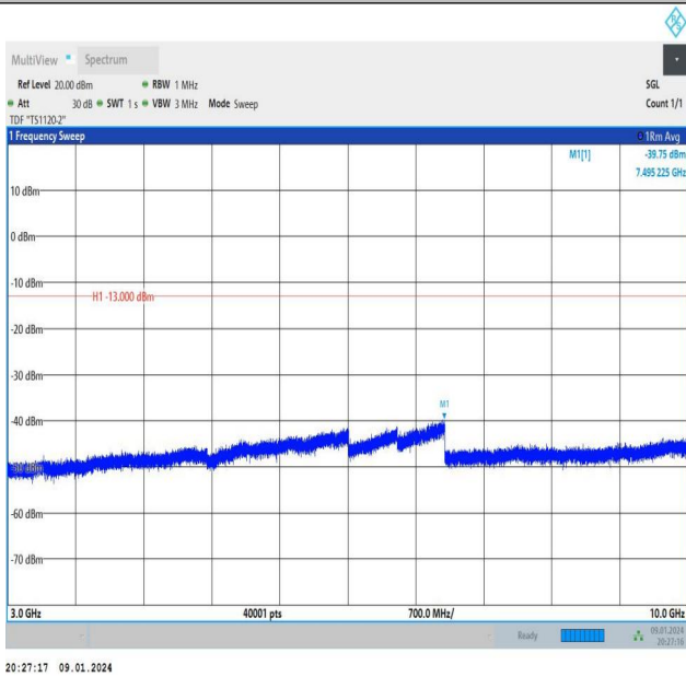
Band26_3MHz_QPSK_27025_15RB#0_3000~10000_3000~10000
