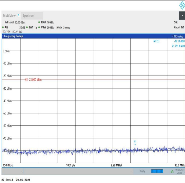
Band26_5MHz_16QAM_26815_1RB#24_0.15~30_0.15~30
