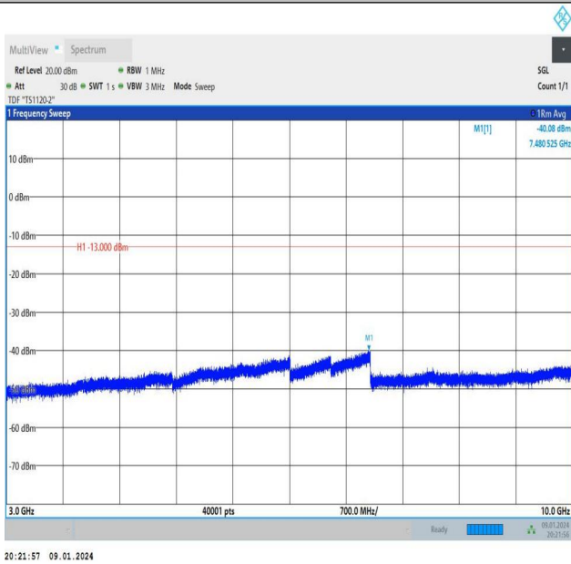
Band26_3MHz_QPSK_26915_1RB#14_3000~10000_3000~10000
