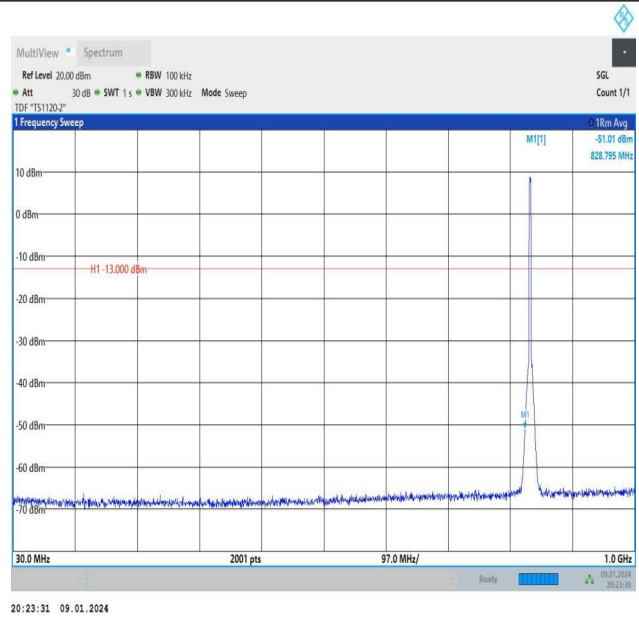
Band26_3MHz_16QAM_26915_15RB#0_30~1000_30~1000
