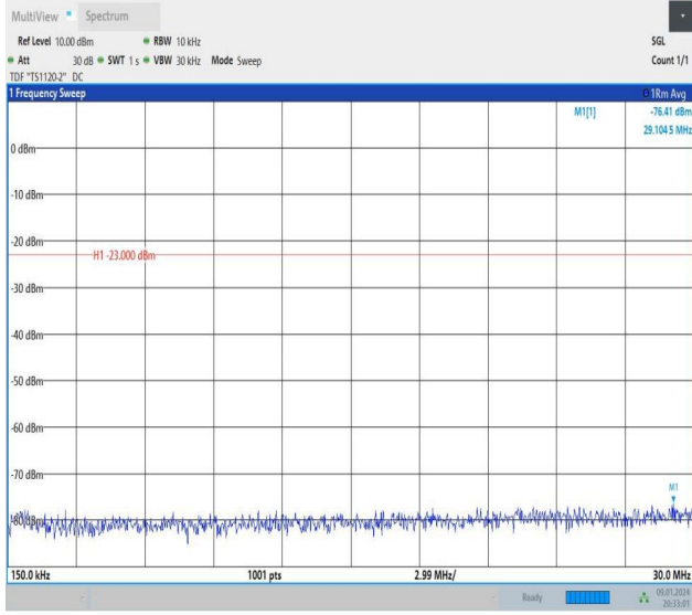
Band26_5MHz_16QAM_26915_1RB#0_0.15~30_0.15~30
