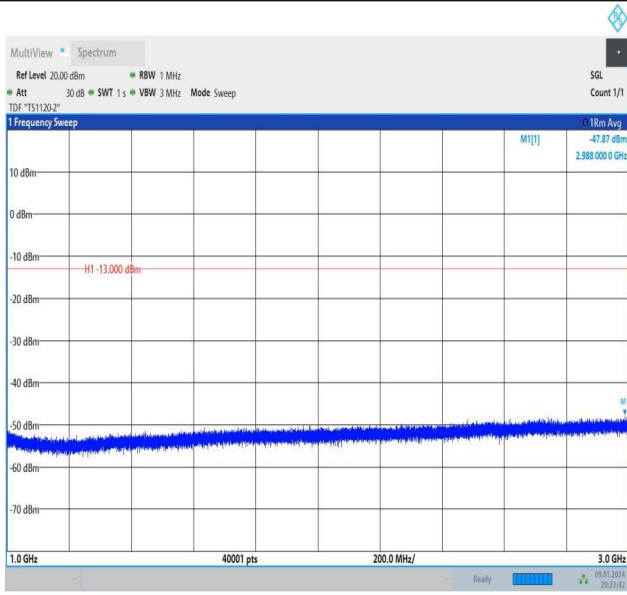
Band26_3MHz_16QAM_26915_15RB#0_1000~3000_1000~3000
