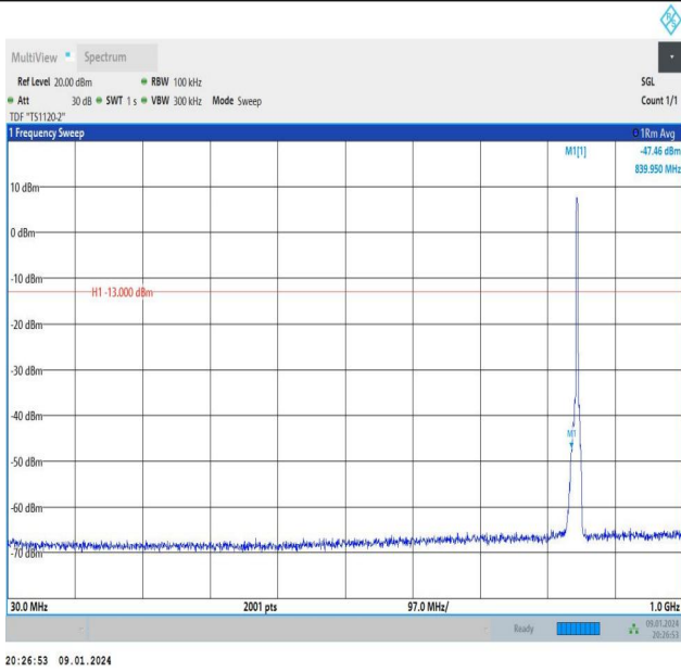
Band26_3MHz_QPSK_27025_15RB#0_30~1000_30~1000
