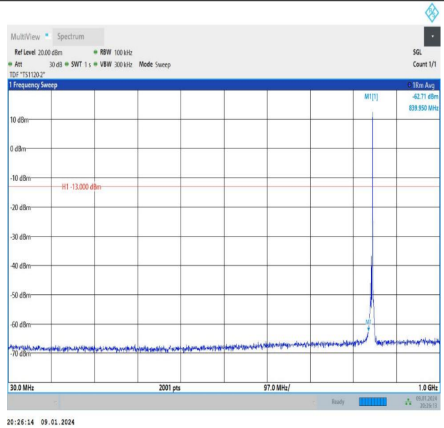
Band26_3MHz_16QAM_27025_1RB#14_30~1000_30~1000
