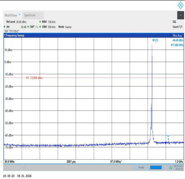
Band26_5MHz_16QAM_26815_1RB#24_30~1000_30~1000
