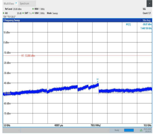
Band26_3MHz_16QAM_27025_1RB#14_3000~10000_3000~10000
