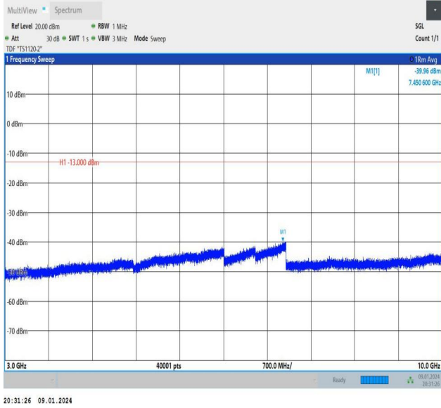
Band26_5MHz_QPSK_26815_25RB#0_3000~10000_3000~10000
