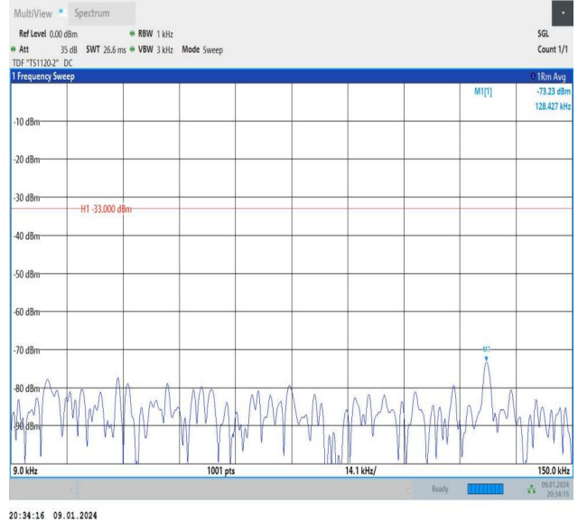
Band26_5MHz_16QAM_26915_1RB#24_0.009~0.15_0.009~0.15
