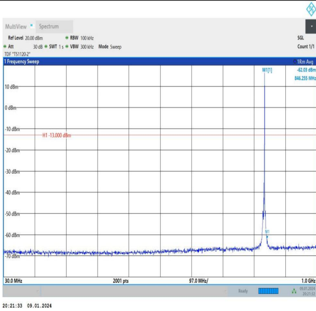
Band26_3MHz_QPSK_26915_1RB#14_30~1000_30~1000
