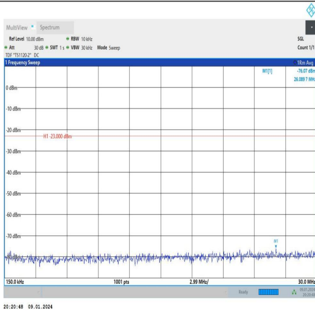
Band26_3MHz_16QAM_26915_1RB#0_0.15~30_0.15~30
