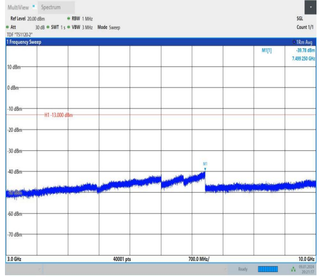
Band26_3MHz_16QAM_26915_1RB#0_3000~10000_3000~1 0000
