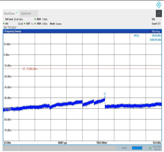
Band26_5MHz_16QAM_26815_25RB#0_3000~10000_3000~10000
