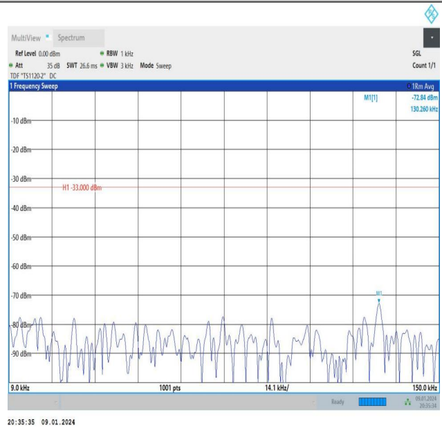
Band26_5MHz_16QAM_26915_25RB#0_0.009~0.15_0.009~0.15
