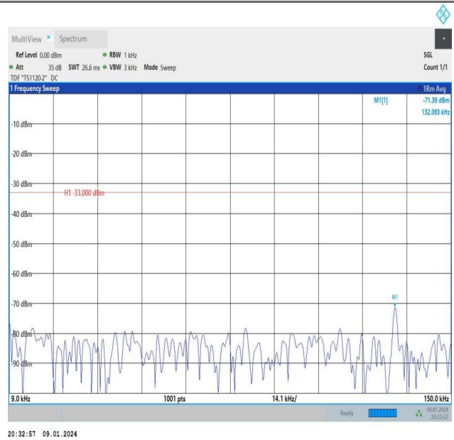
Band26_5MHz_16QAM_26915_1RB#0_0.009~0.15_0.009~0.15
