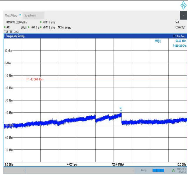
Band26_3MHz_16QAM_26915_15RB#0_3000~10000_3000~10000
