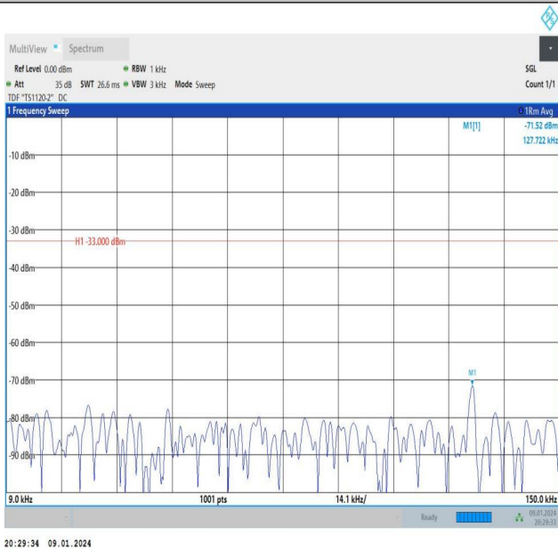
Band26_5MHz_QPSK_26815_1RB#24_0.009~0.15_0.009~0.15
