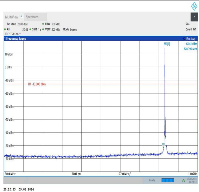
Band26_3MHz_16QAM_26915_1RB#0_30~1000_30~1000
