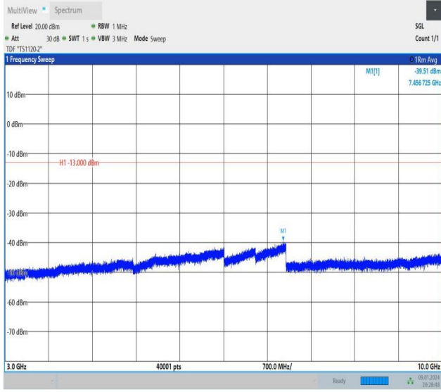
Band26_5MHz_QPSK_26815_1RB#0_3000~10000_3000~10000
