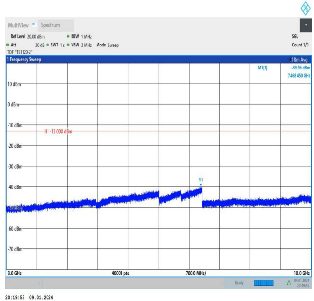
Band26_3MHz_16QAM_26805_15RB#0_3000~10000_3000~10000
