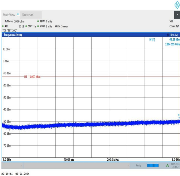
Band26_3MHz_16QAM_26805_15RB#0_1000~3000_1000~3000
