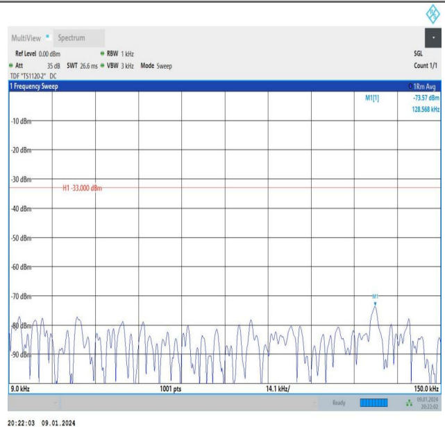
Band26_3MHz_16QAM_26915_1RB#14_0.009~0.15_0.009~0.15
