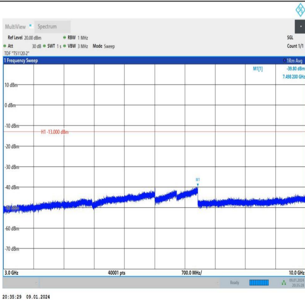
Band26_5MHz_QPSK_26915_25RB#0_3000~10000_3000~10000
