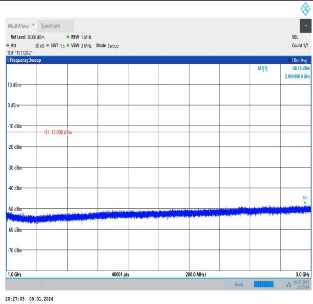
Band26_3MHz_QPSK_27025_15RB#0_1000~3000_1000~3000
