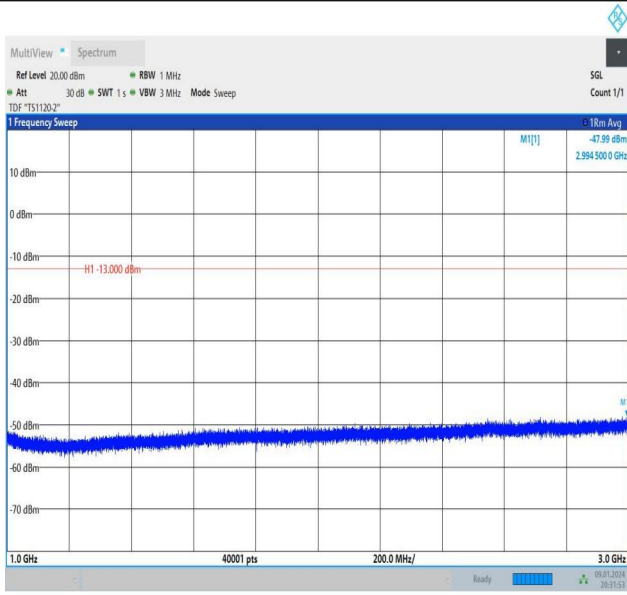
Band26_5MHz_16QAM_26815_25RB#0_1000~3000_1000~3000
