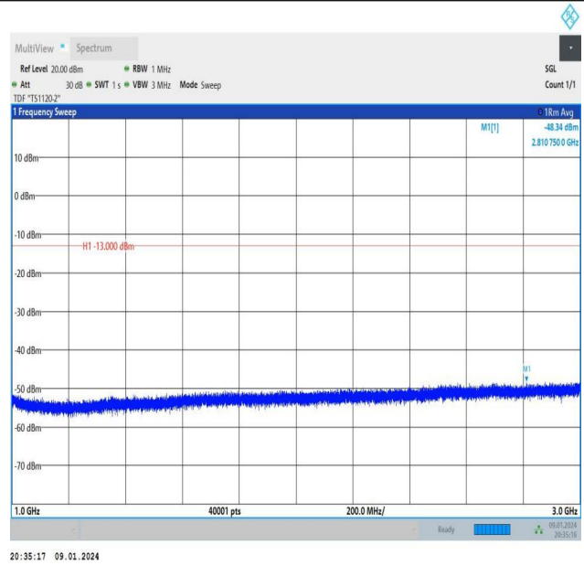
Band26_5MHz_QPSK_26915_25RB#0_1000~3000_1000~3000
