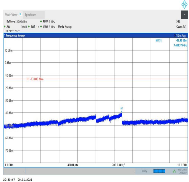
Band26_5MHz_16QAM_26815_1RB#24_3000~10000_3000~10000
