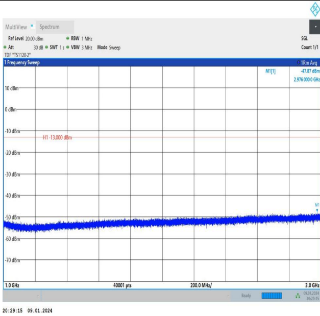
Band26_5MHz_16QAM_26815_1RB#0_1000~3000_1000~3000
