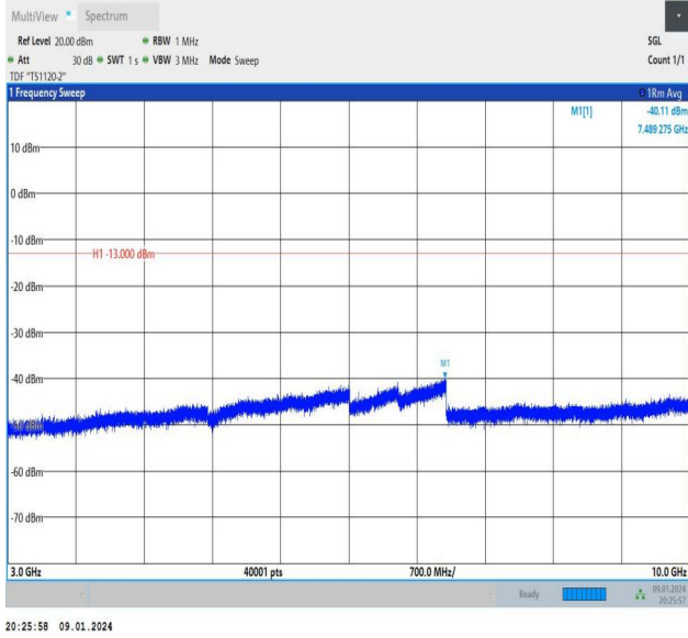
Band26_3MHz_QPSK_27025_1RB#14_3000~10000_3000~10000
