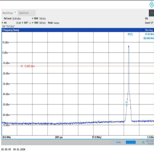
Band26_5MHz_QPSK_26915_25RB#0_30~1000_30~1000
