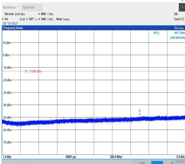
Band26_5MHz_16QAM_26915_1RB#0_1000~3000_1000~3000
