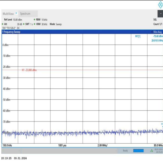
Band26_3MHz_16QAM_26805_15RB#0_0.15~30_0.15~30
