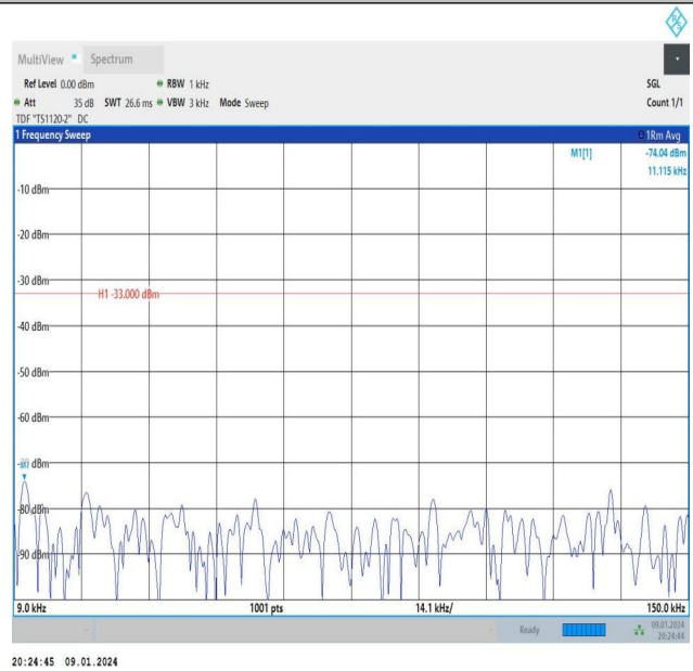
Band26_3MHz_16QAM_27025_1RB#0_0.009~0.15_0.009~0.15
