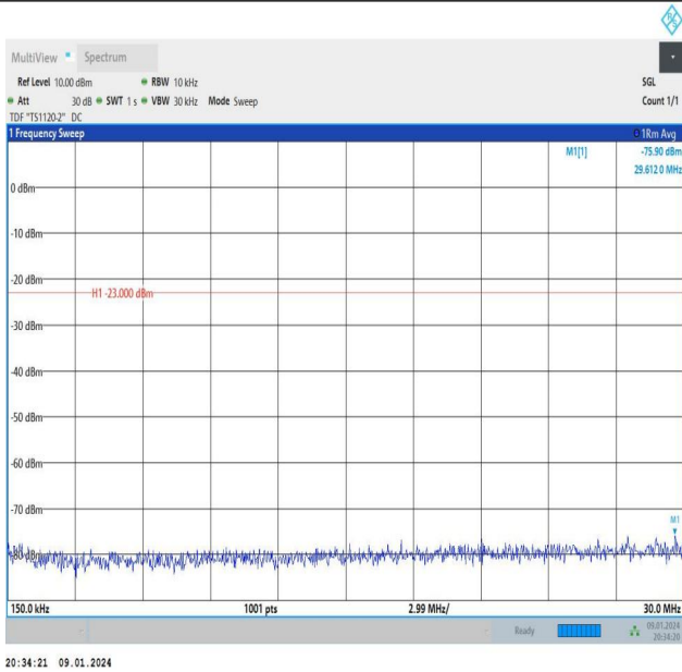
Band26_5MHz_16QAM_26915_1RB#24_0.15~30_0.15~30
