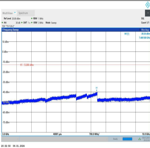
Band26_5MHz_QPSK_26915_1RB#0_3000~10000_3000~10000
