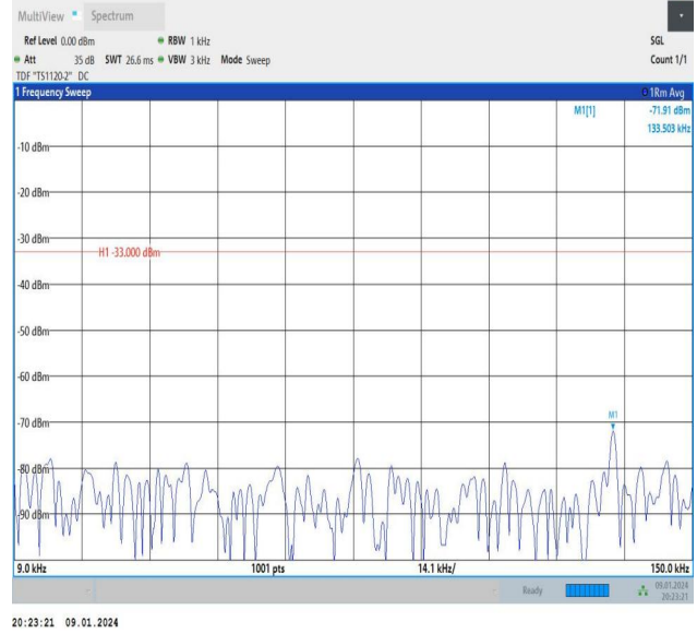
Band26_3MHz_16QAM_26915_15RB#0_0.009~0.15_0.009~0.15
