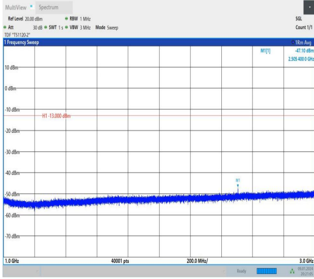
Band26_3MHz_16QAM_26915_1RB#0_1000~3000_1000~30 00
