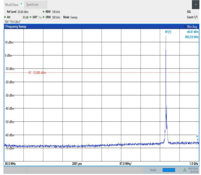
Band26_5MHz_16QAM_26915_1RB#0_30~1000_30~1000
