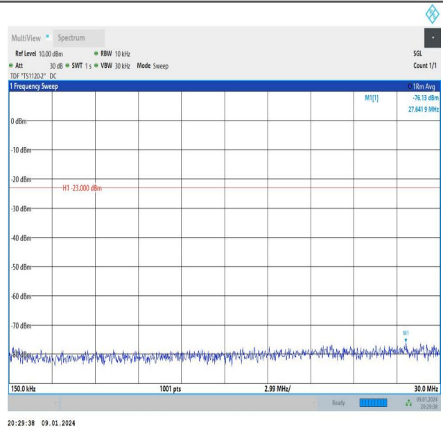
Band26_5MHz_QPSK_26815_1RB#24_0.15~30_0.15~30
