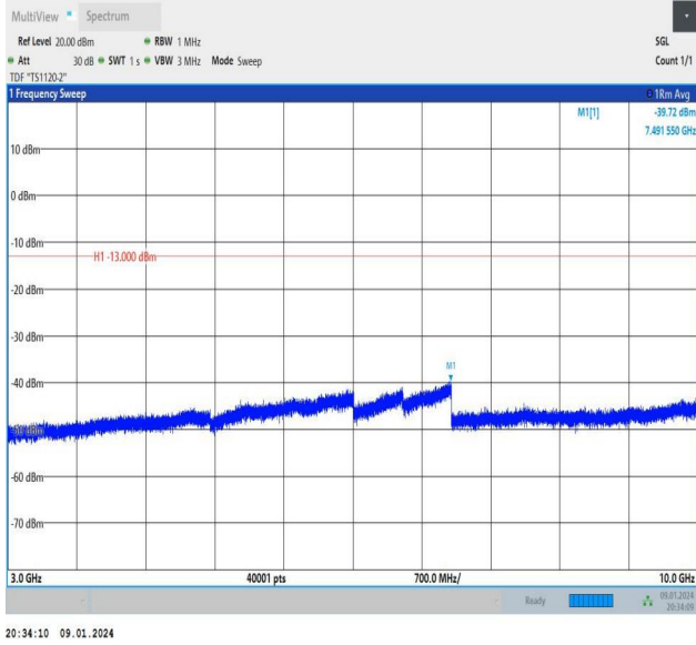
Band26_5MHz_QPSK_26915_1RB#24_3000~10000_3000~10000
