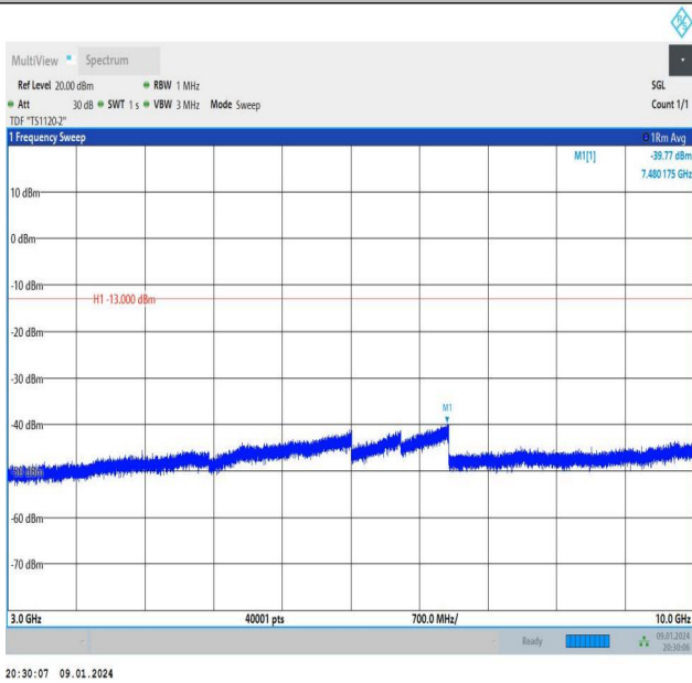
Band26_5MHz_QPSK_26815_1RB#24_3000~10000_3000~10000
