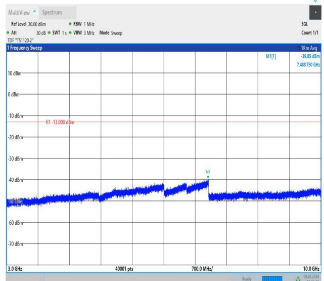
Band26_5MHz_16QAM_26915_1RB#0_3000~10000_3000~10000
