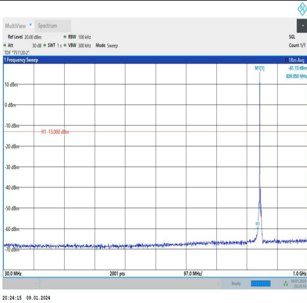
Band26_3MHz_QPSK_27025_1RB#0_30~1000_30~1000
