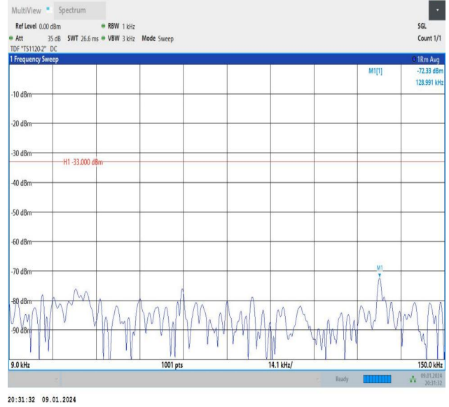
Band26_5MHz_16QAM_26815_25RB#0_0.009~0.15_0.009~0.15
