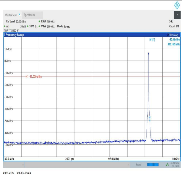
Band26_3MHz_16QAM_26805_15RB#0_30~1000_30~1000
