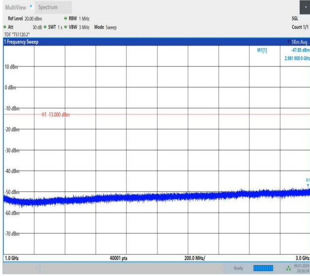
Band26_3MHz_16QAM_27025_1RB#14_1000~3000_1000~3000
