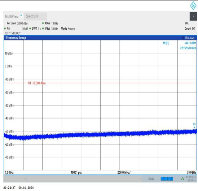
Band26_3MHz_QPSK_27025_1RB#0_1000~3000_1000~300
