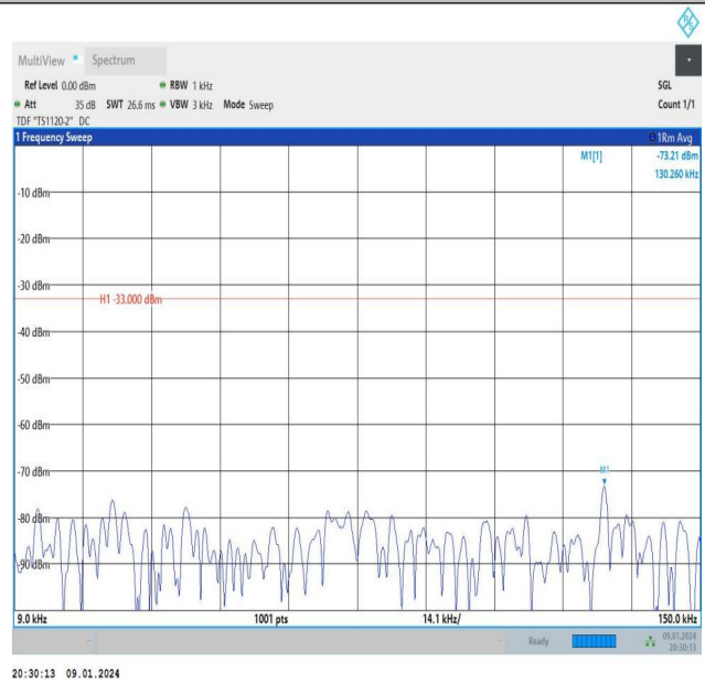
Band26_5MHz_16QAM_26815_1RB#24_0.009~0.15_0.009~0.15
