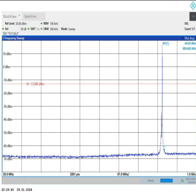
Band26_5MHz_QPSK_26815_1RB#24_30~1000_30~1000
