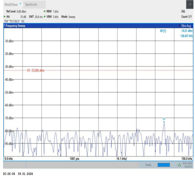
Band26_3MHz_16QAM_27025_1RB#14_0.009~0.15_0.009~0.15
