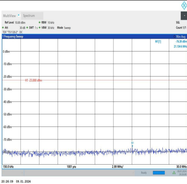
Band26_3MHz_16QAM_27025_1RB#14_0.15~30_0.15~30
