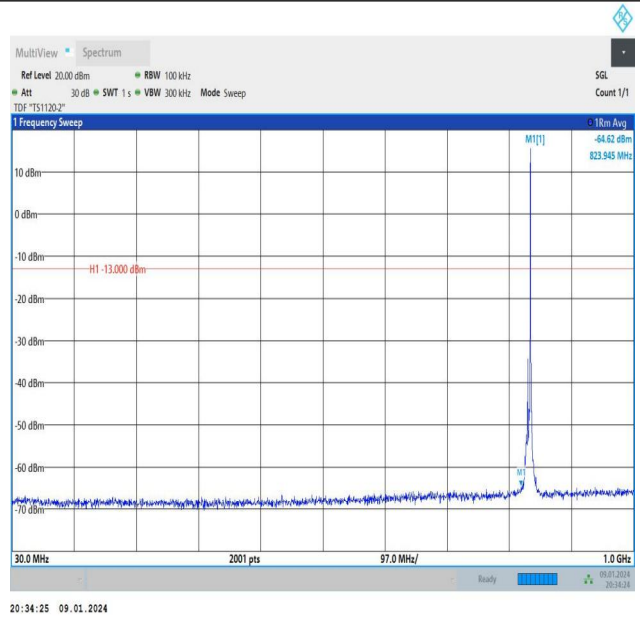
Band26_5MHz_16QAM_26915_1RB#24_30~1000_30~1000
