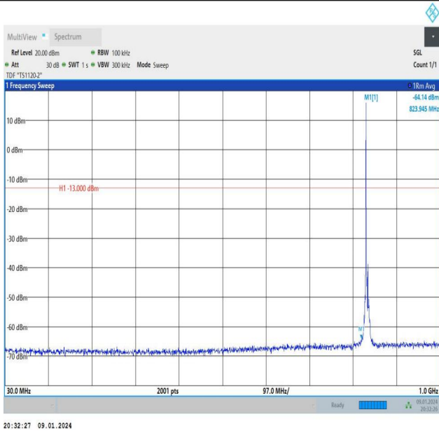
Band26_5MHz_QPSK_26915_1RB#0_30~1000_30~1000
