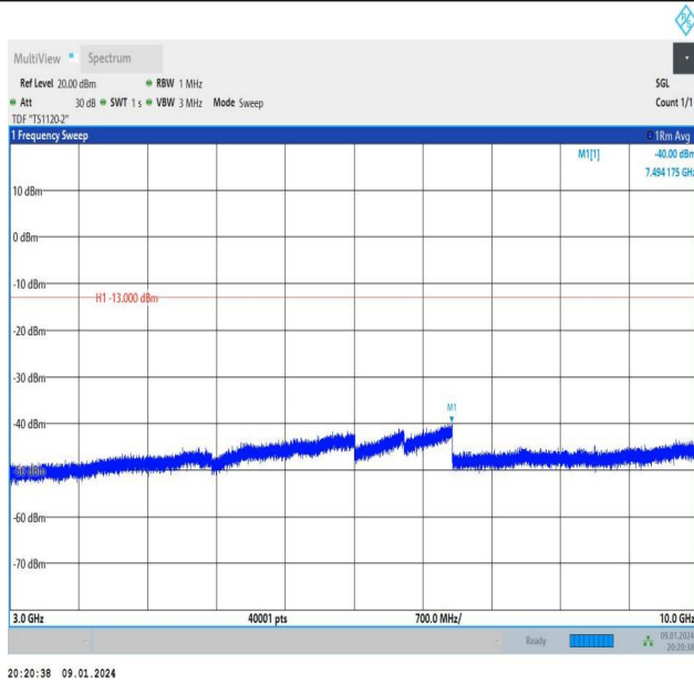
Band26_3MHz_QPSK_26915_1RB#0_3000~10000_3000~10000
