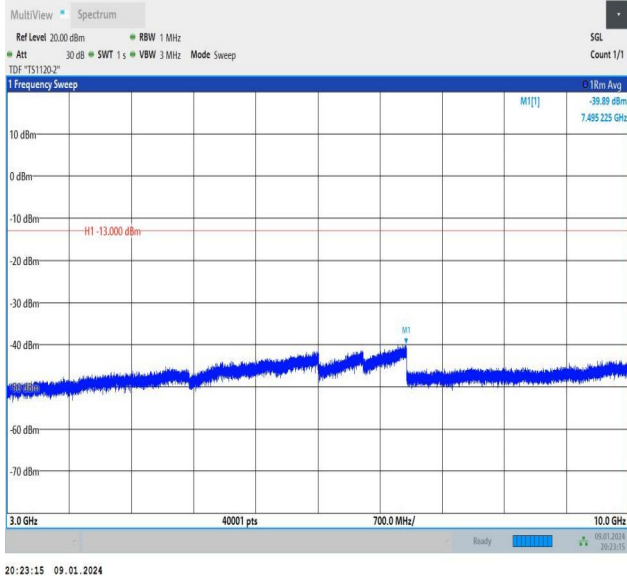
Band26_3MHz_QPSK_26915_15RB#0_3000~10000_3000~10000
