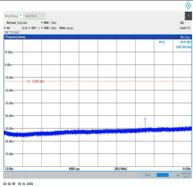
Band26_5MHz_QPSK_26915_1RB#0_1000~3000_1000~300
