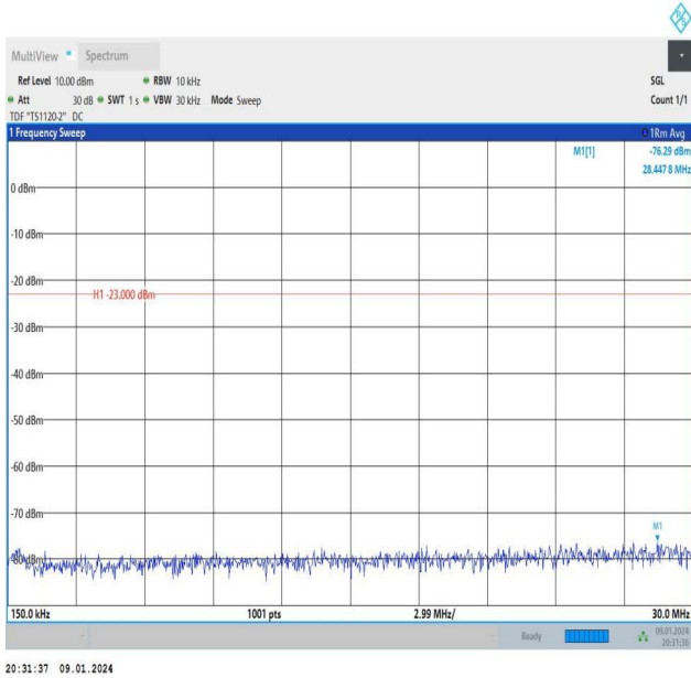
Band26_5MHz_16QAM_26815_25RB#0_0.15~30_0.15~30
