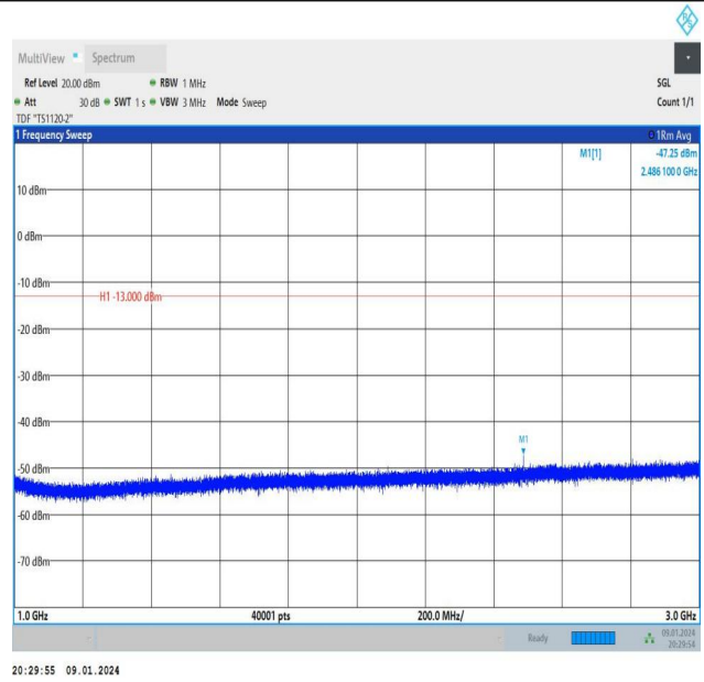
Band26_5MHz_QPSK_26815_1RB#24_1000~3000_1000~3000
