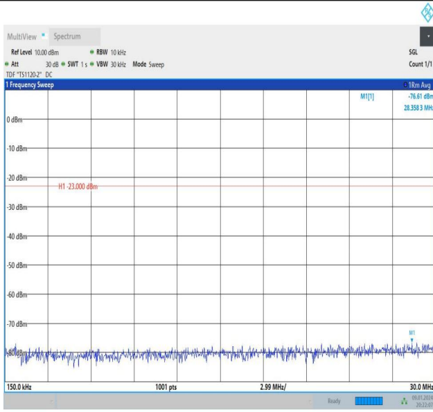
Band26_3MHz_16QAM_26915_1RB#14_0.15~30_0.15~30
