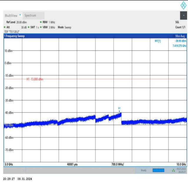
Band26_5MHz_16QAM_26815_1RB#0_3000~10000_3000~10000
