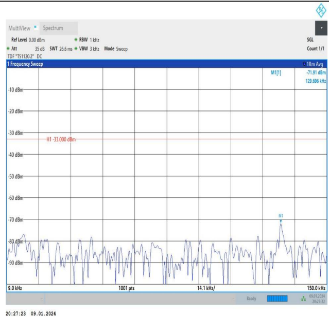
Band26_3MHz_16QAM_27025_15RB#0_0.009~0.15_0.009~0.15
