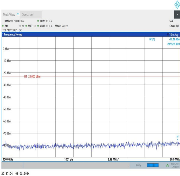
Band26_5MHz_16QAM_27015_1RB#0_0.15~30_0.15~30
