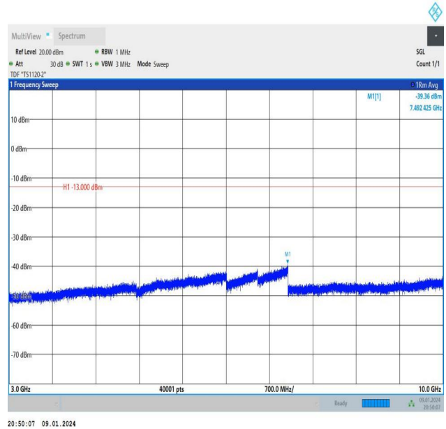
Band26_10MHz_QPSK_26915_50RB#0_3000~10000_3000~10000
