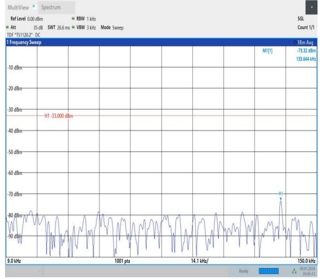
Band26_10MHz_16QAM_26915_1RB#49_0.009~0.15_0.009~0.15
