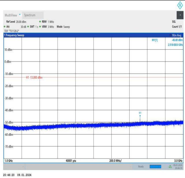
Band26_10MHz_QPSK_26990_1RB#0_1000~3000_1000~3000
