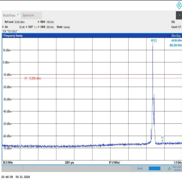
Band26_10MHz_QPSK_26990_1RB#0_30~1000_30~1000
