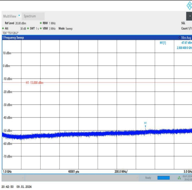
Band26_10MHz_16QAM_26840_1RB#49_1000~3000_1000~3000
