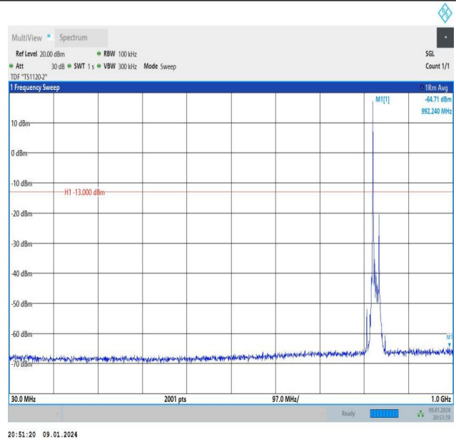
Band26_15MHz_QPSK_26865_1RB#0_30~1000_30~1000
