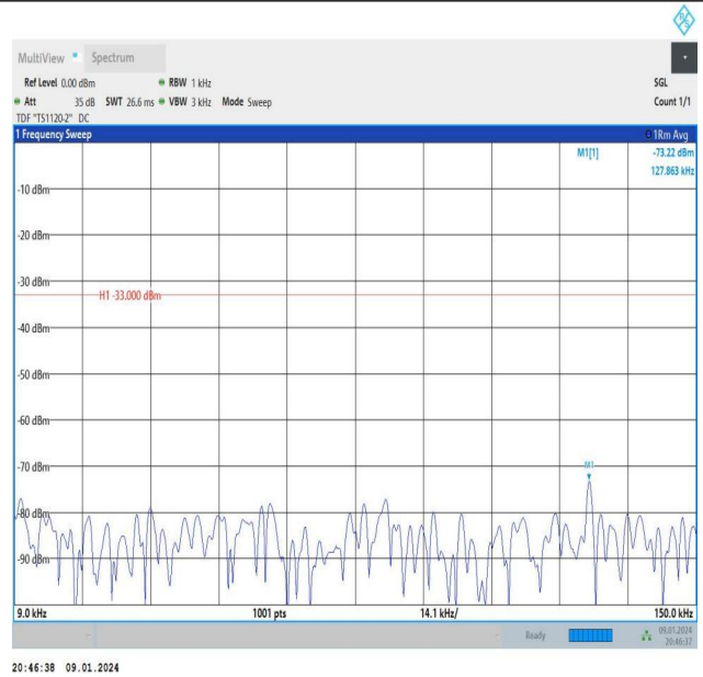
Band26_10MHz_16QAM_26990_1RB#0_0.009~0.15_0.009~0.15
