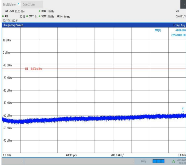
Band26_10MHz_16QAM_26990_1RB#49_1000~3000_1000~3000
