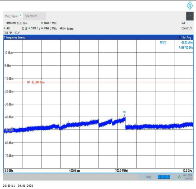
Band26_5MHz_16QAM_27015_25RB#0_3000~10000_3000~10000
