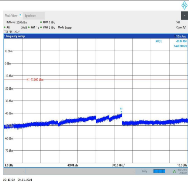
Band26_10MHz_16QAM_26840_1RB#49_3000~10000_3000~10000
