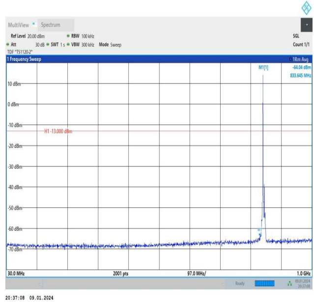
Band26_5MHz_16QAM_27015_1RB#0_30~1000_30~1000
