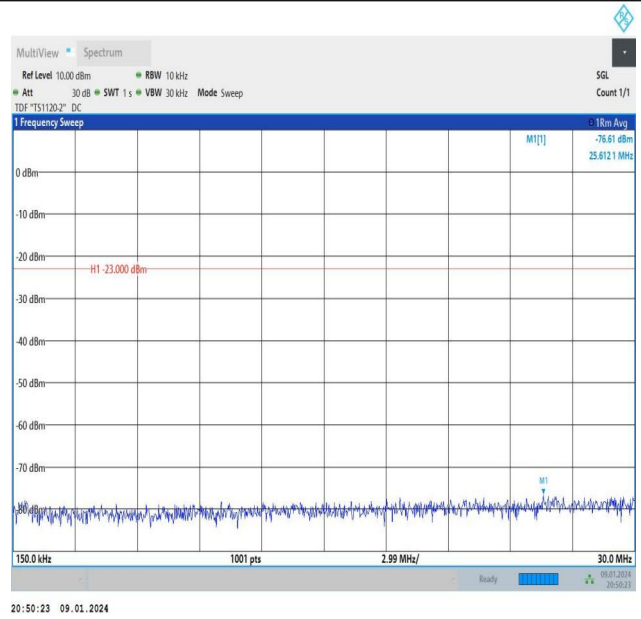
Band26_10MHz_QPSK_26990_50RB#0_0.15~30_0.15~30
