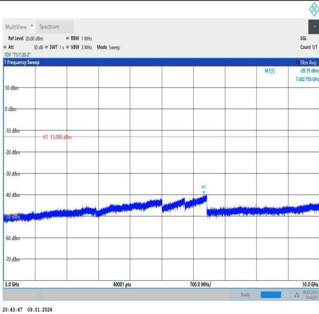
Band26_10MHz_QPSK_26915_1RB#0_3000~10000_3000~10000
