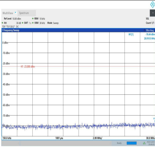
Band26_10MHz_16QAM_26990_1RB#0_0.15~30_0.15~30
