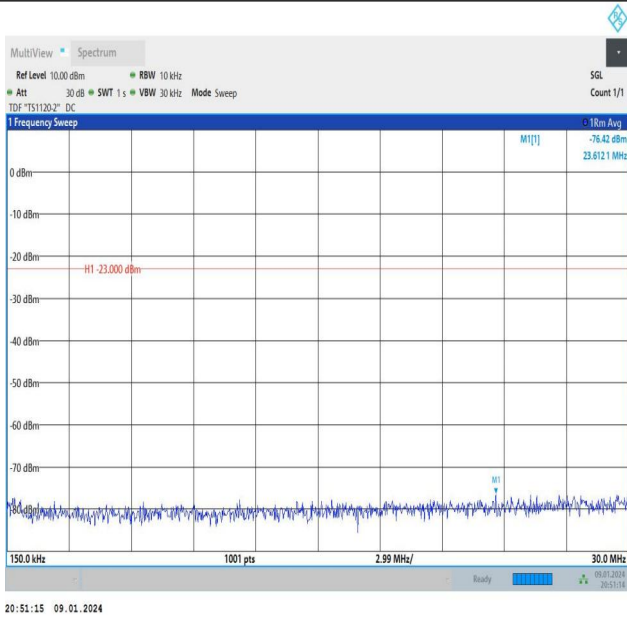
Band26_15MHz_QPSK_26865_1RB#0_0.15~30_0.15~30
