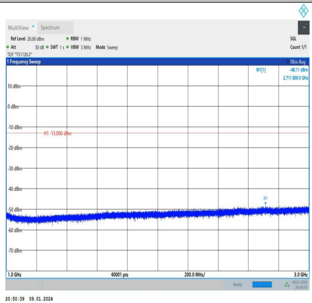
Band26_10MHz_QPSK_26990_50RB#0_1000~3000_1000~3000
