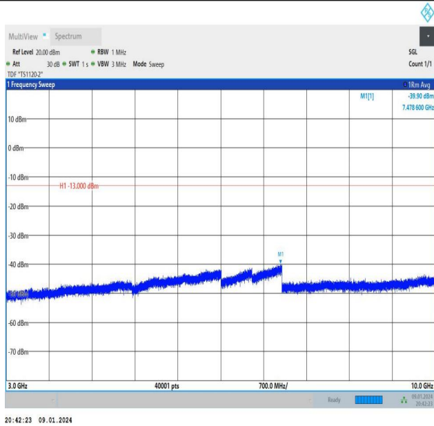
Band26_10MHz_QPSK_26840_1RB#49_3000~10000_3000~10000
