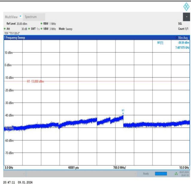
Band26_10MHz_16QAM_26990_1RB#0_3000~10000_3000~10000
