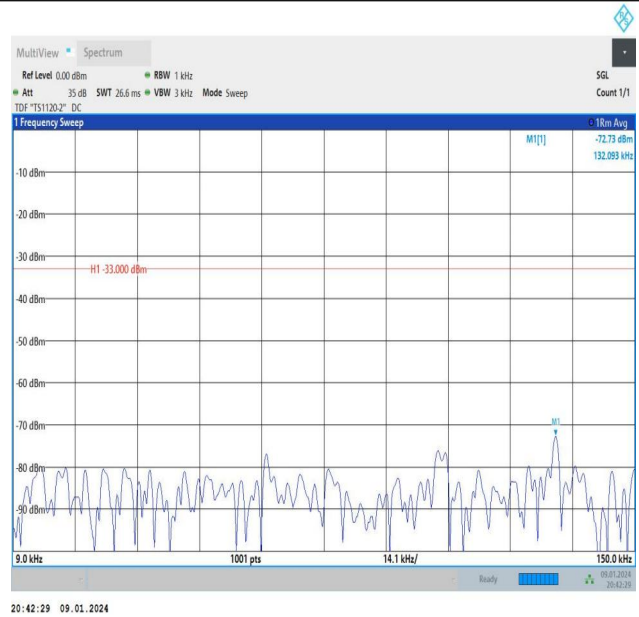
Band26_10MHz_16QAM_26840_1RB#49_0.009~0.15_0.009~0.15
