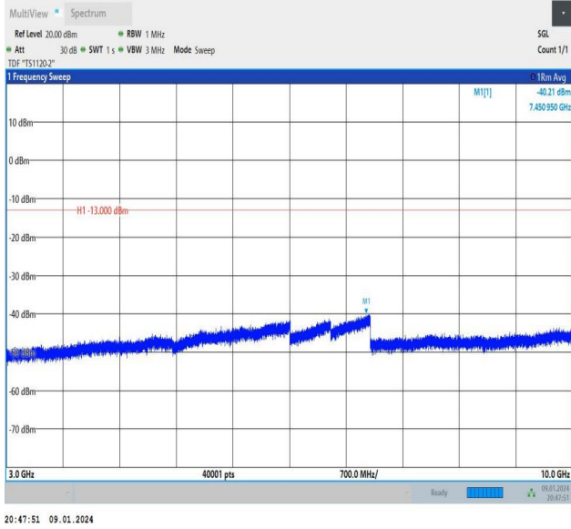
Band26_10MHz_QPSK_26990_1RB#49_3000~10000_3000~10000
