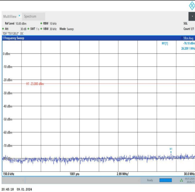
Band26_10MHz_16QAM_26915_1RB#49_0.15~30_0.15~30
