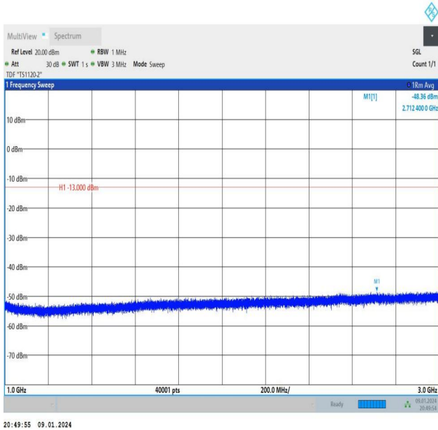
Band26_10MHz_QPSK_26915_50RB#0_1000~3000_1000~3000
