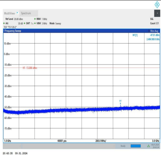
Band26_10MHz_QPSK_26915_1RB#0_1000~3000_1000~3000
