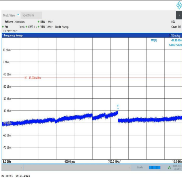
Band26_10MHz_QPSK_26990_50RB#0_3000~10000_3000~10000
