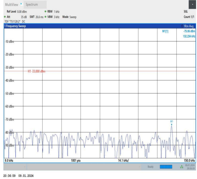
Band26_5MHz_16QAM_27015_1RB#0_0.009~0.15_0.009~0.15
