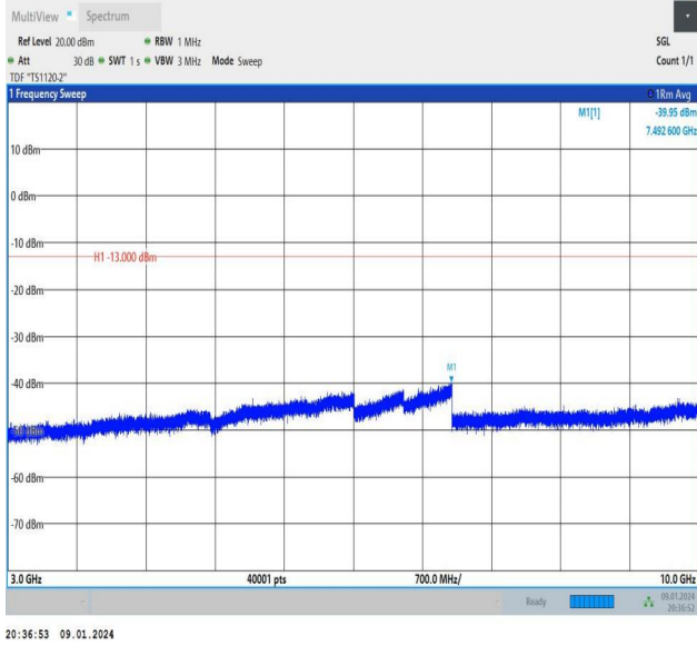
Band26_5MHz_QPSK_27015_1RB#0_3000~10000_3000~10000
