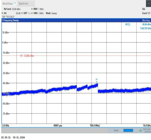
Band26_5MHz_QPSK_27015_25RB#0_3000~10000_3000~10000
