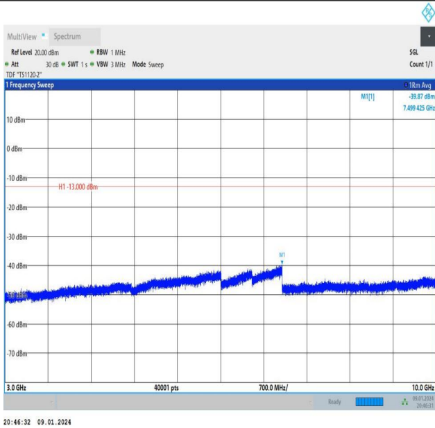
Band26_10MHz_QPSK_26990_1RB#0_3000~10000_3000~10000
