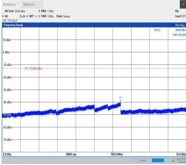
Band26_10MHz_QPSK_26915_1RB#49_3000~10000_3000~10000
