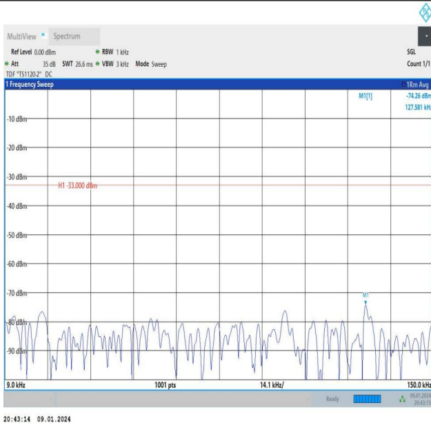
Band26_10MHz_QPSK_26915_1RB#0_0.009~0.15_0.009~0.15
