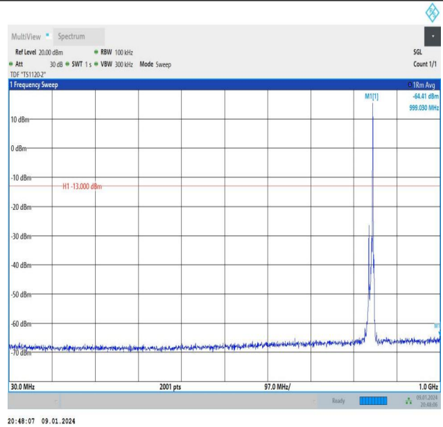
Band26_10MHz_16QAM_26990_1RB#49_30~1000_30~1000
