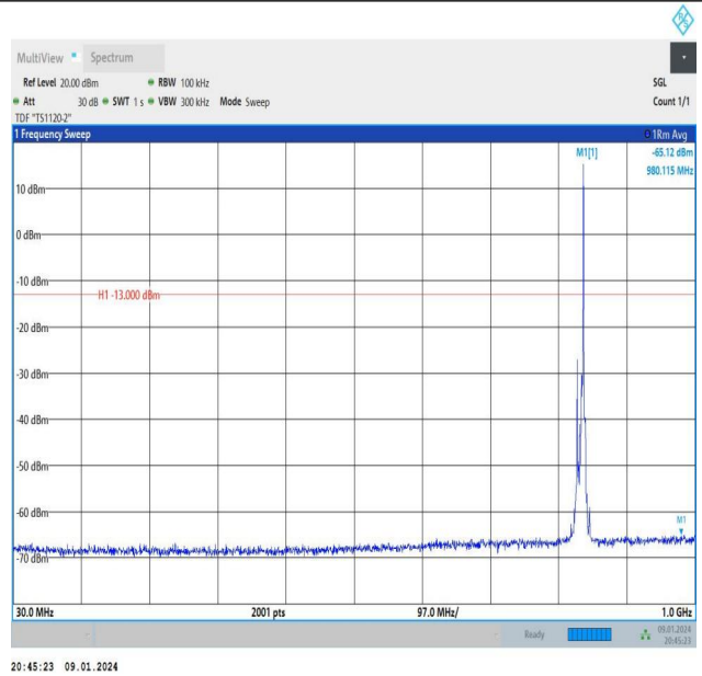
Band26_10MHz_16QAM_26915_1RB#49_30~1000_30~1000
