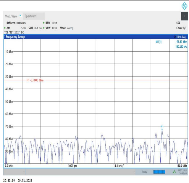
Band26_10MHz_16QAM_26840_1RB#0_0.009~0.15_0.009~0.15
