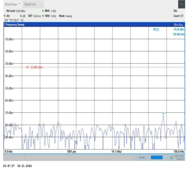
Band26_10MHz_16QAM_26990_1RB#49_0.009~0.15_0.009~0.15
