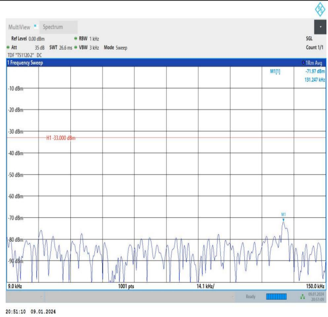
Band26_15MHz_QPSK_26865_1RB#0_0.009~0.15_0.009~0.15
