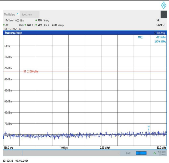
Band26_10MHz_QPSK_26840_1RB#0_0.15~30_0.15~30
