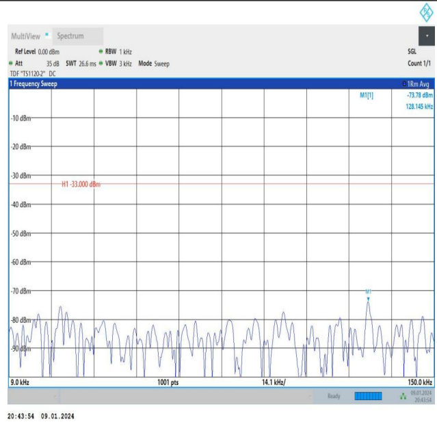
Band26_10MHz_16QAM_26915_1RB#0_0.009~0.15_0.009~0.15
