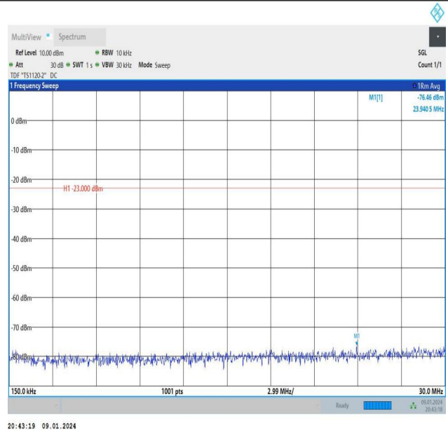
Band26_10MHz_QPSK_26915_1RB#0_0.15~30_0.15~30
