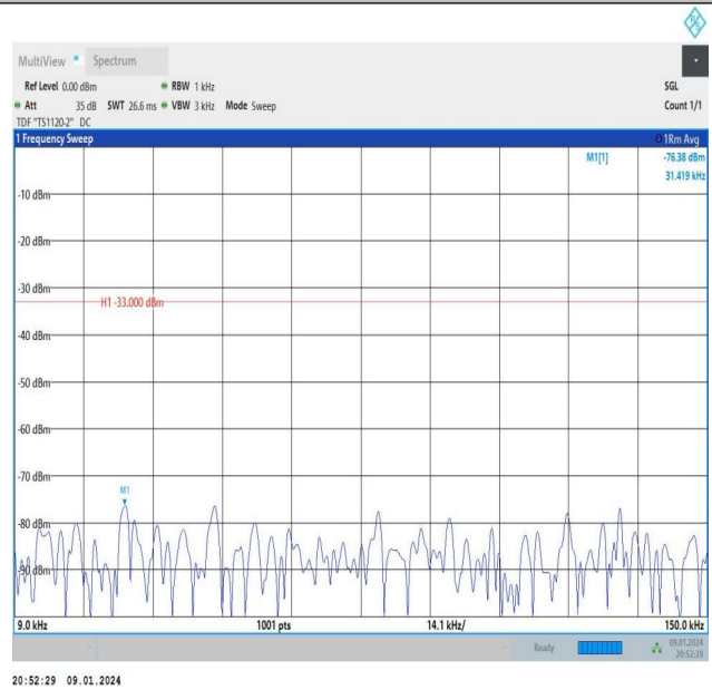
Band26_15MHz_QPSK_26865_1RB#74_0.009~0.15_0.009~0.15
