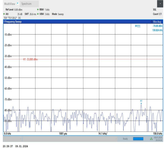
Band26_5MHz_16QAM_27015_25RB#0_0.009~0.15_0.009~0.15
