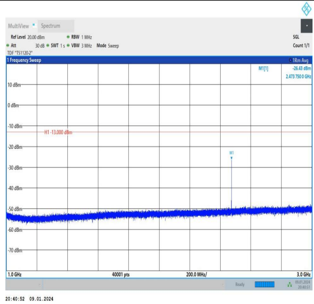
Band26_10MHz_QPSK_26840_1RB#0_1000~3000_1000~3000
