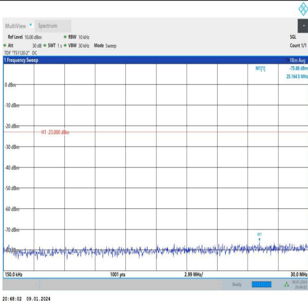
Band26_10MHz_16QAM_26990_1RB#49_0.15~30_0.15~30
