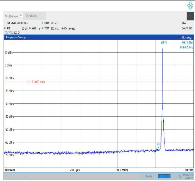
Band26_10MHz_16QAM_26990_1RB#0_30~1000_30~1000
