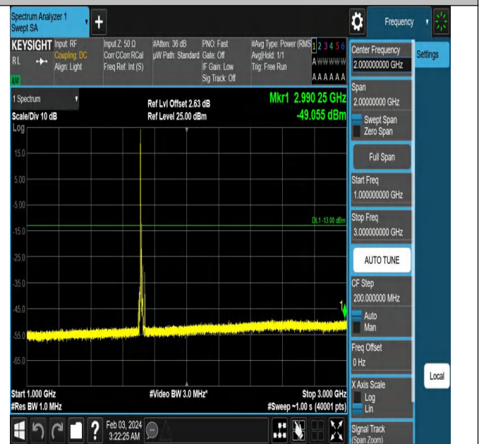
Band66_15MHz_QPSK_132047_1RB#0_1000~3000_1000~3000
