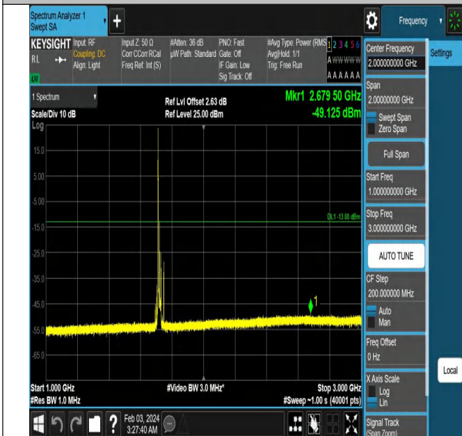
Band66_20MHz_QPSK_132072_1RB#0_1000~3000_1000~3000
