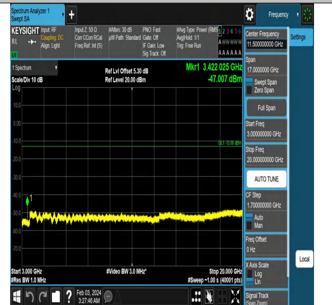
Band66_20MHz_QPSK_132072_1RB#0_3000~20000_3000~20000
