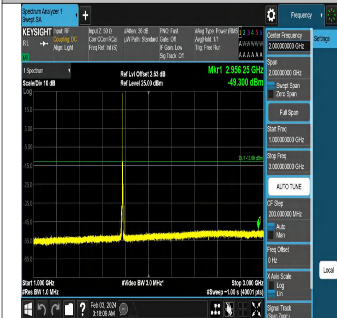
Band66_10MHz_QPSK_132622_1RB#0_1000~3000_1000~3000
