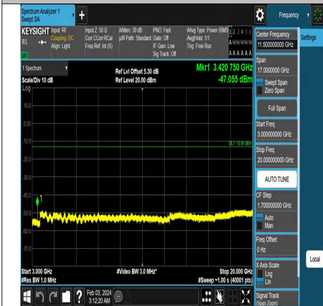
Band66_5MHz_QPSK_131997_1RB#0_3000~20000_3000~20000
