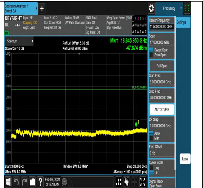
Band66_10MHz_QPSK_132022_1RB#0_3000~20000_3000~20000
