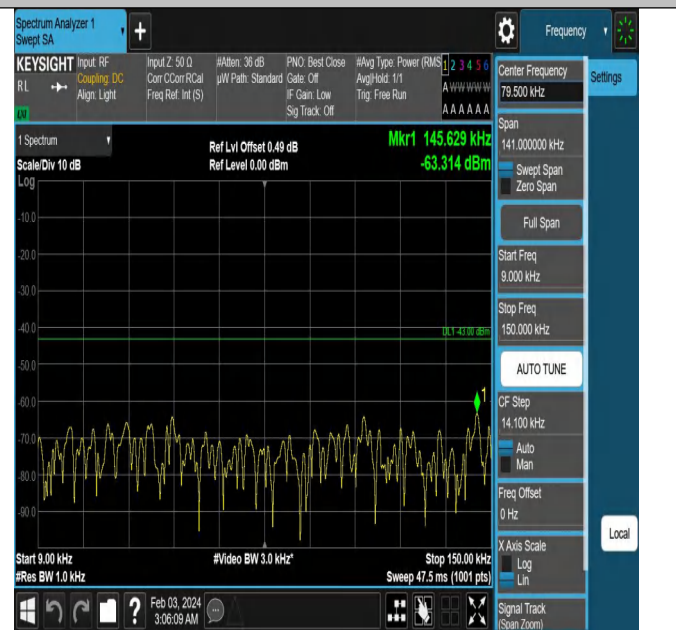
Band66_3MHz_QPSK_131987_1RB#0_0.009~0.15_0.009~0.15
