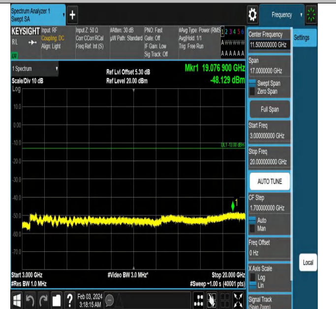
Band66_10MHz_QPSK_132622_1RB#0_3000~20000_3000~20000
