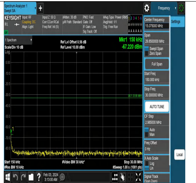
Band66_5MHz_QPSK_132647_1RB#0_0.15~30_0.15~30
