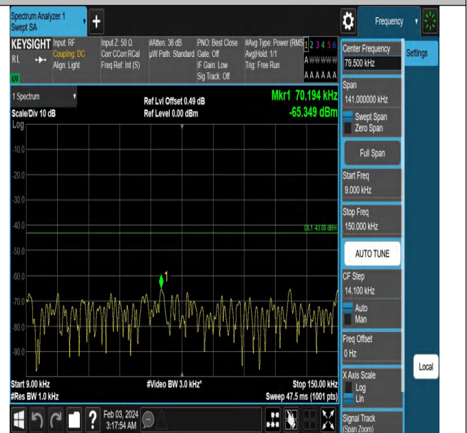
Band66_10MHz_QPSK_132622_1RB#0_0.009~0.15_0.009~0.15
