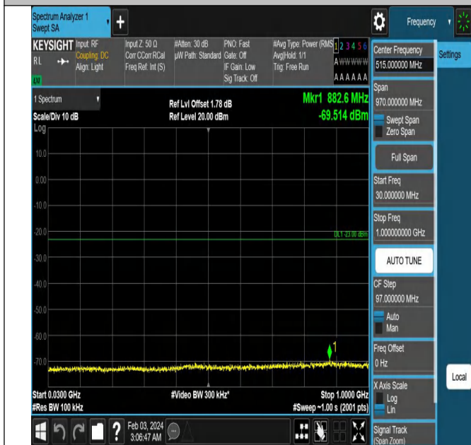
Band66_3MHz_QPSK_132322_1RB#0_30~1000_30~1000
