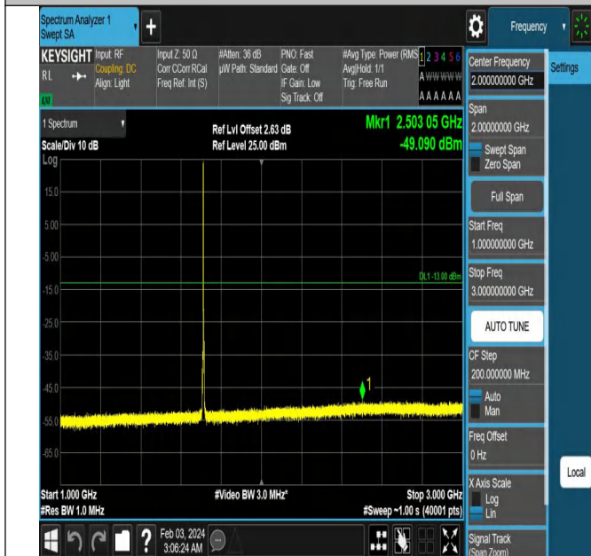
Band66_3MHz_QPSK_131987_1RB#0_1000~3000_1000~30
