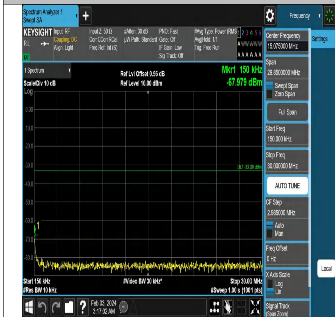
Band66_10MHz_QPSK_132022_1RB#0_0.15~30_0.15~30
