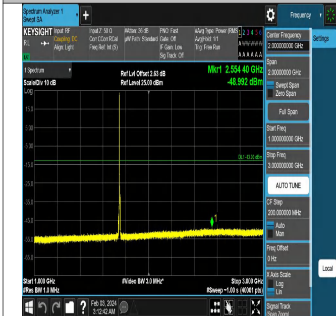
Band66_5MHz_QPSK_132322_1RB#0_1000~3000_1000~30
