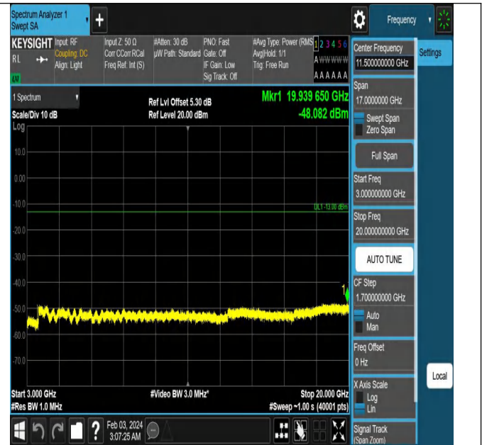
Band66_3MHz_QPSK_132657_1RB#0_3000~20000_3000~2
