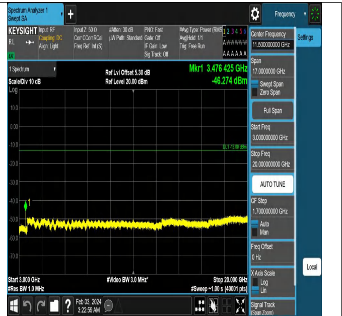
Band66_15MHz_QPSK_132322_1RB#0_3000~20000_3000~20000
