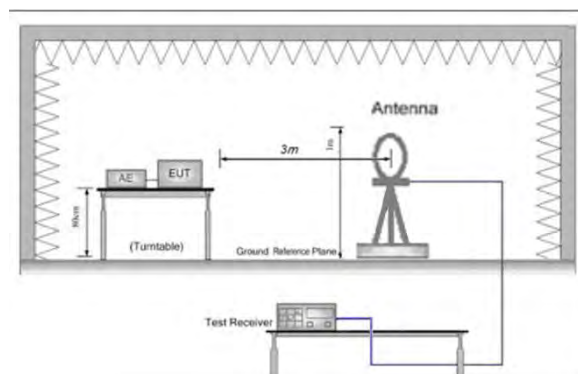
Figure 1. 9kHz to 30MHz
