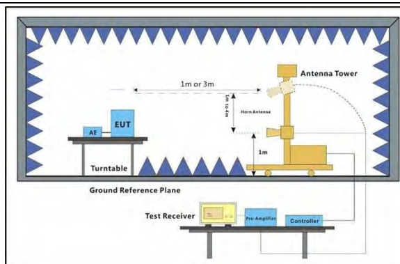
Figure 2. Above 1 GHz
