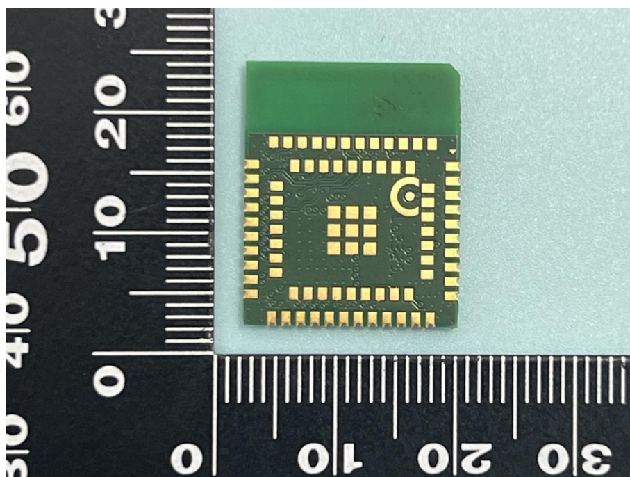
FCM561D-P_Bottom
