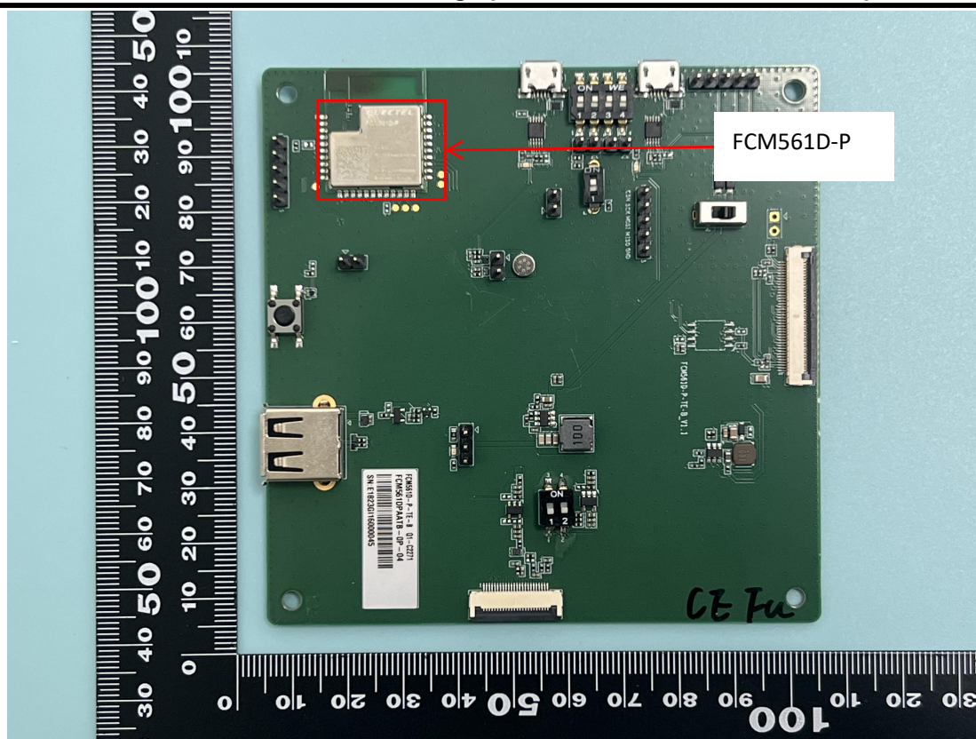
FCM561D-P + EVB _Top
