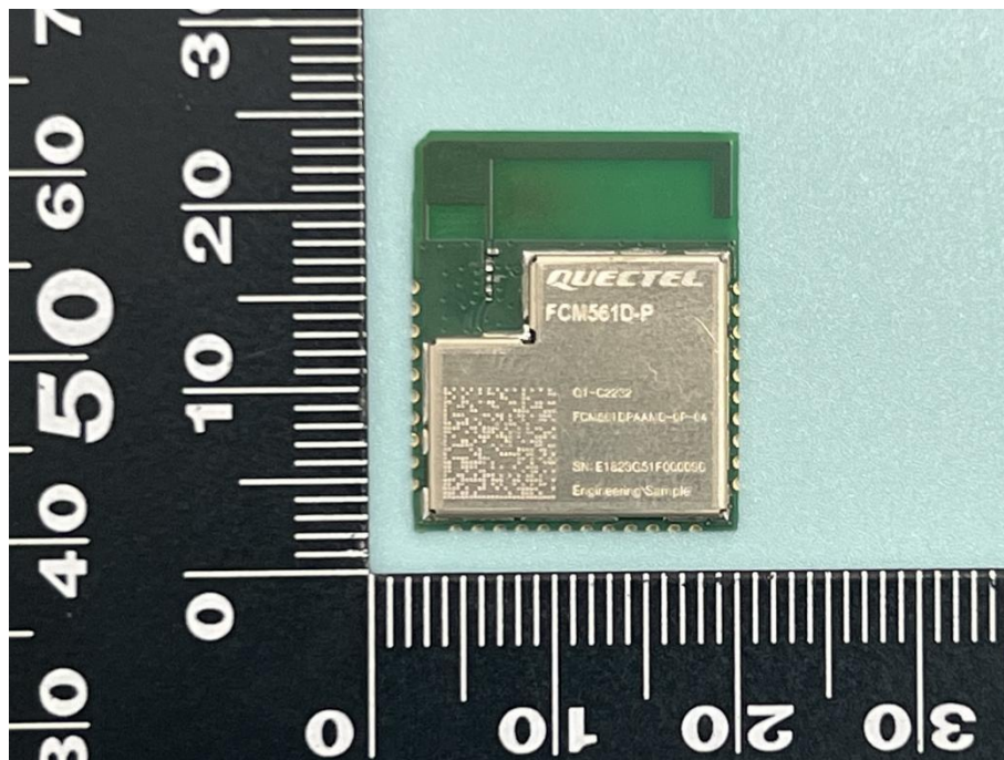
FCM561D-P_Top
