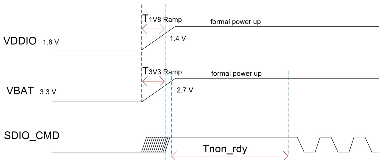
Figure 4: Power-up Timing
