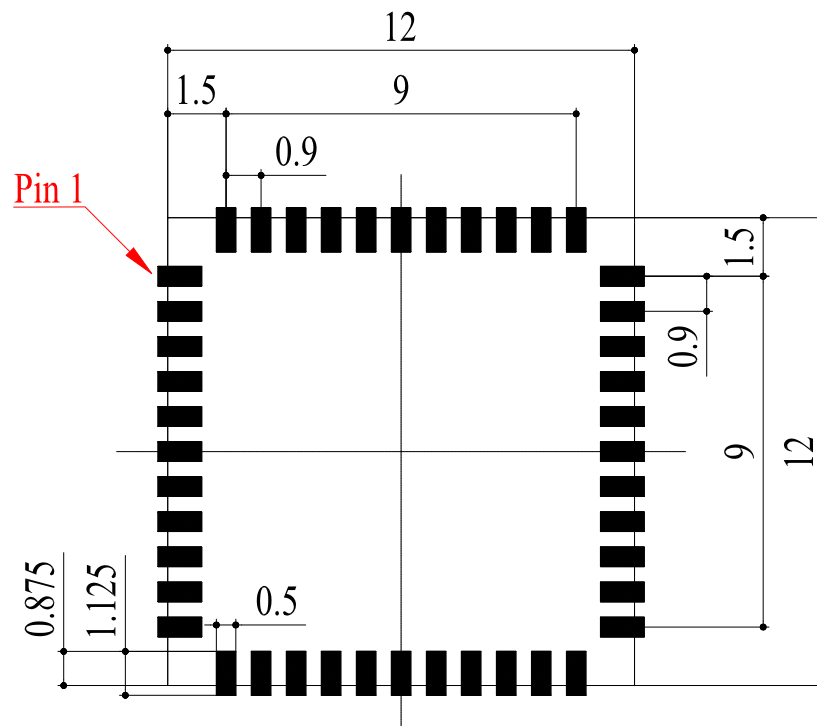
Figure 23: Recommended Footprint
