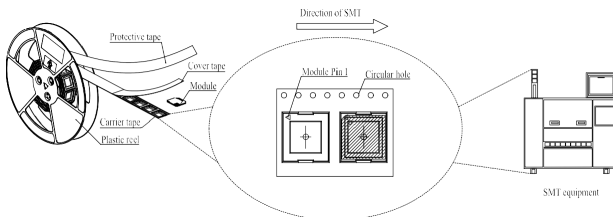
Figure 30: Mounting Direction
