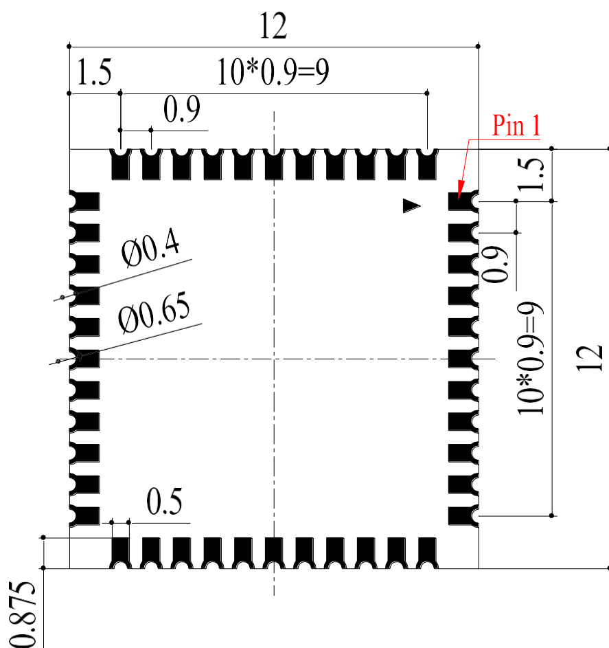
Figure 19: Bottom Dimension (Bottom View)
