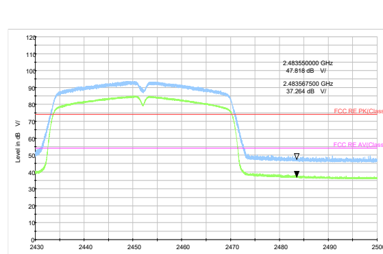
802.11n HT40 -Channel 9 Peak+ Average
