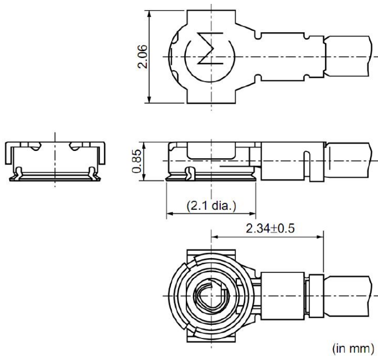
Figure 14: Dimensions of Mated Plugs ( \varnothing 0.81 mm Coaxial Cables) (Unit: mm)
