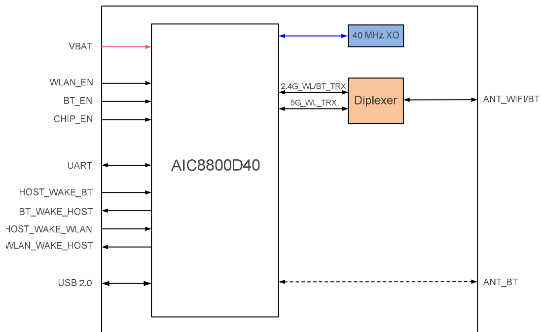
Figure 1: Functional Diagram
