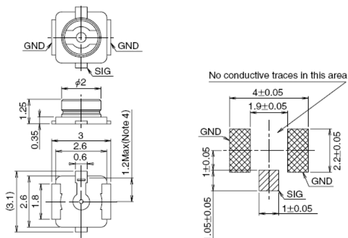
Figure 13: Dimensions of the Receptacle (Unit: mm)
