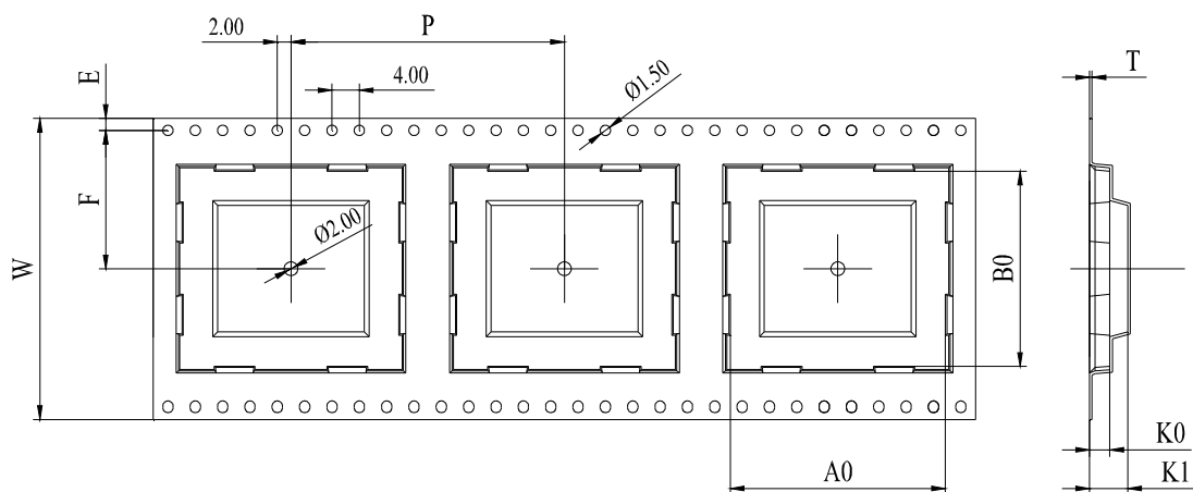
Figure 22: Carrier Tape Dimension Drawing
