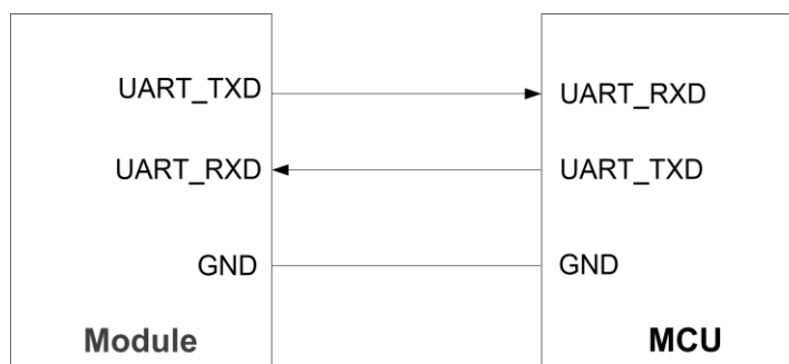
Figure 3: UART0 Connection
