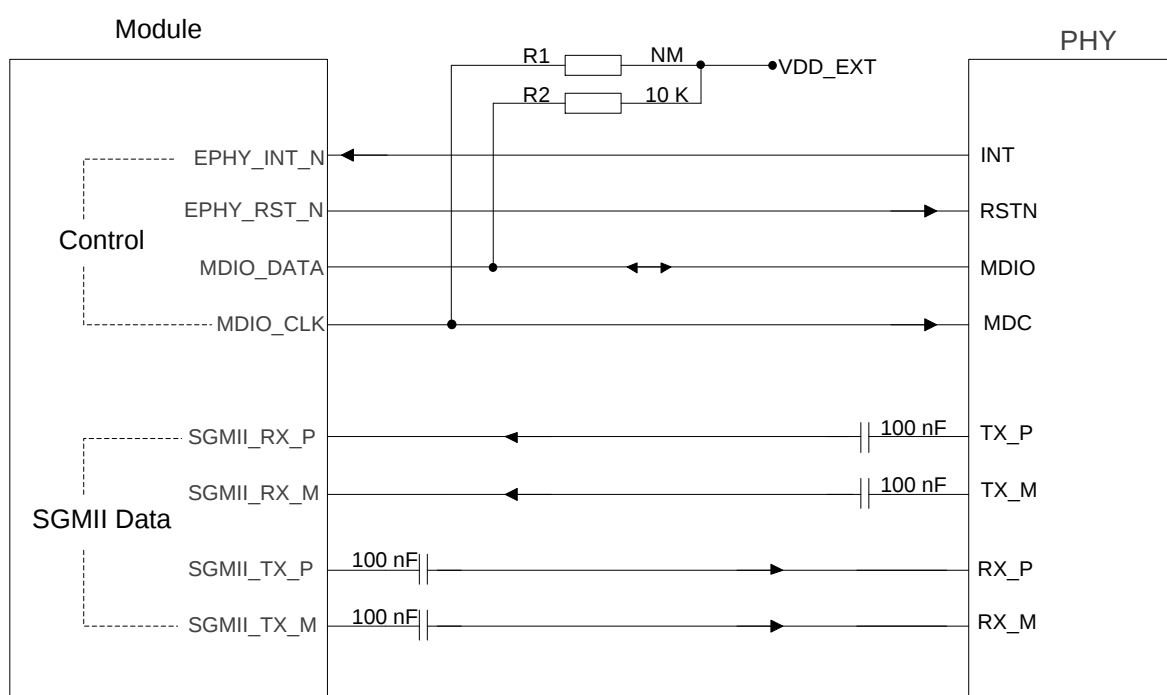
Figure 22: Reference Circuit of SGMII Interface with PHY Application
