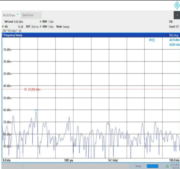
Band2_3MHz_16QAM_18900_1RB#0_0.009~0.15_0.009~0.1
