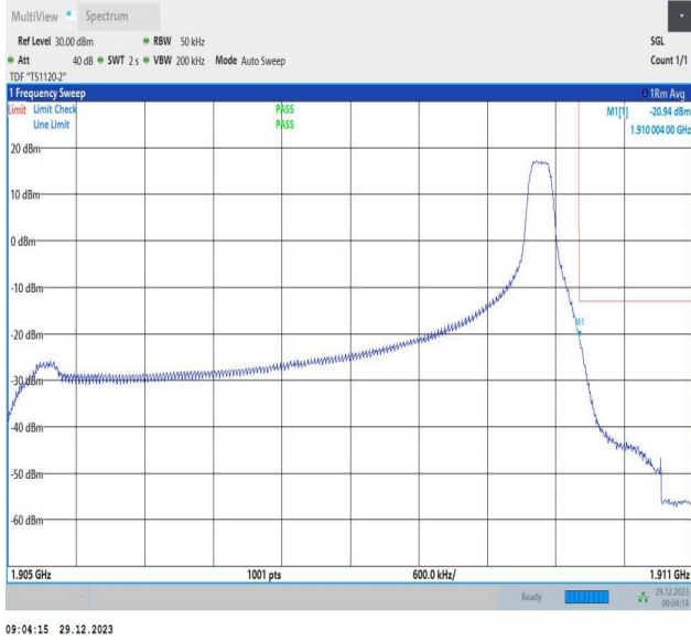
Band2_5MHz_64QAM_19175_1RB#24
