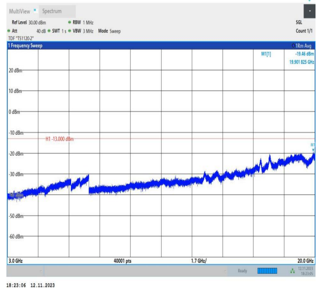
Band2_3MHz_QPSK_19185_1RB#0_3000~20000_3000~2000
