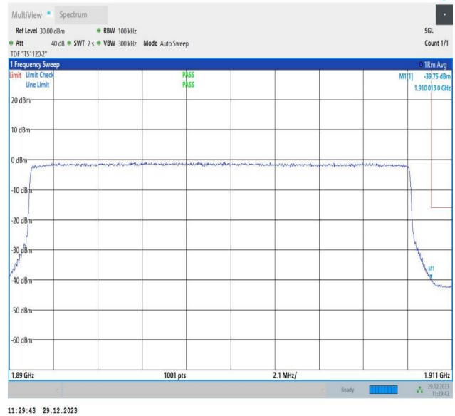
Band2_20MHz_64QAM_19100_100RB#0
