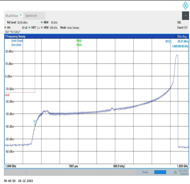
Band2_5MHz_64QAM_18625_1RB#24
