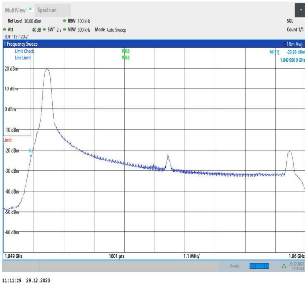
Band2_10MHz_64QAM_18650_1RB#0
