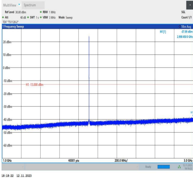
Band2_1.4MHz_16QAM_19193_1RB#0_1000~3000_1000~3000
