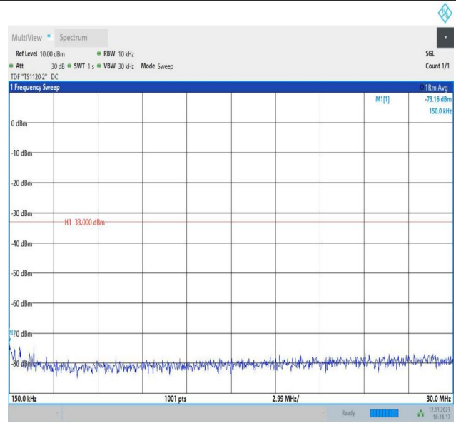
Band2_5MHz_QPSK_18625_1RB#0_0.15~30_0.15~30
