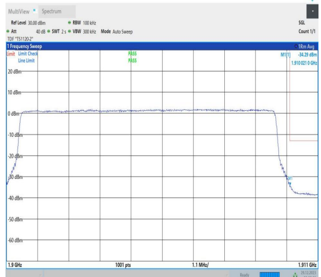
Band2_10MHz_64QAM_19150_50RB#0
