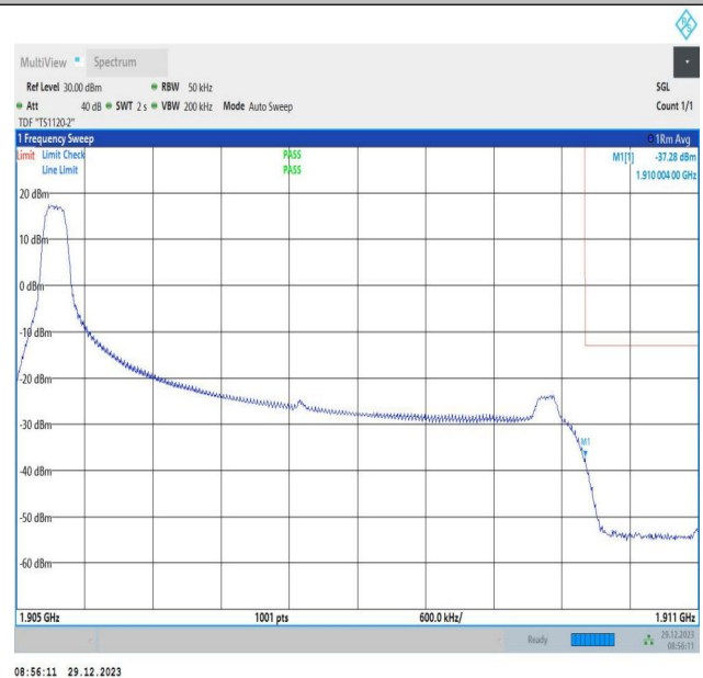
Band2_5MHz_64QAM_19175_1RB#0
