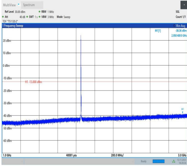
Band2_3MHz_16QAM_18615_1RB#0_1000~3000_1000~3000
