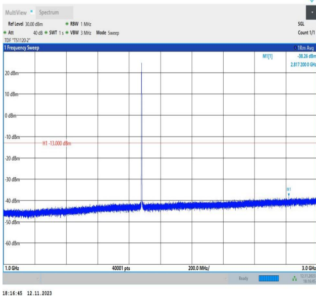
Band2_1.4MHz_16QAM_18900_1RB#0_1000~3000_1000~3000
