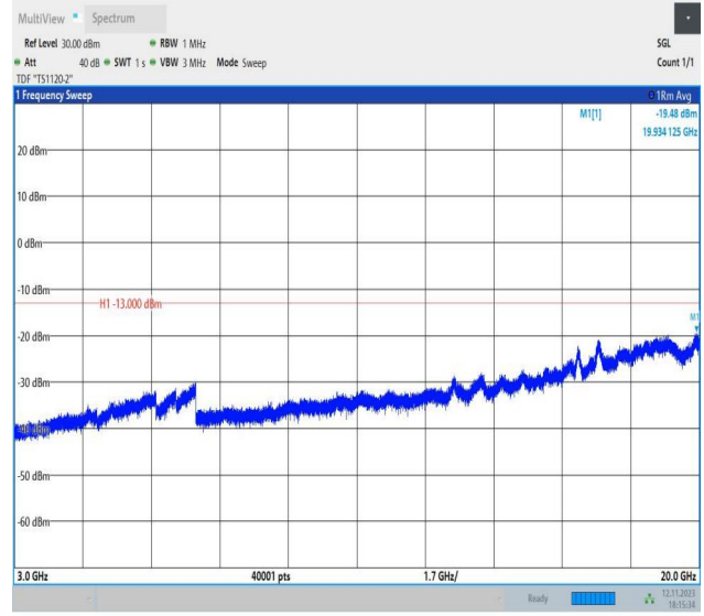
Band2_1.4MHz_16QAM_18607_1RB#0_3000~20000_3000~20000
