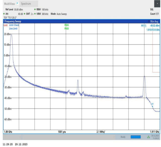
Band2_20MHz_64QAM_19100_1RB#0
