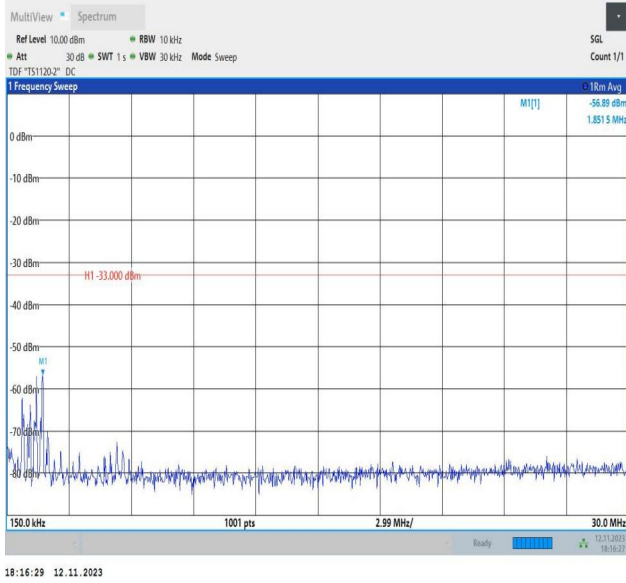
Band2_1.4MHz_16QAM_18900_1RB#0_0.15~30_0.15~30
