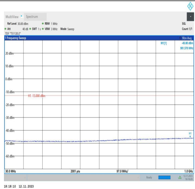
Band2_1.4MHz_16QAM_19193_1RB#0_30~1000_30~1000
