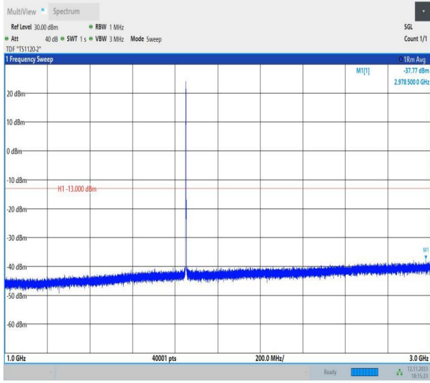
Band2_1.4MHz_16QAM_18607_1RB#0_1000~3000_1000~3000
