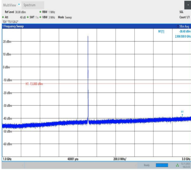
Band2_3MHz_16QAM_19185_1RB#0_1000~3000_1000~300
