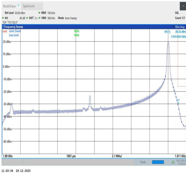
Band2_20MHz_64QAM_19100_1RB#99
