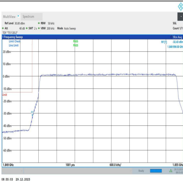
Band2_5MHz_64QAM_18625_25RB#0
