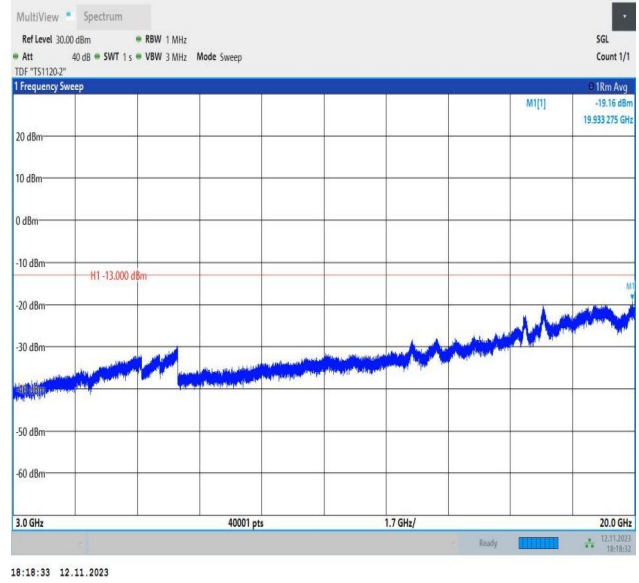
Band2_1.4MHz_16QAM_19193_1RB#0_3000~20000_3000~20000
