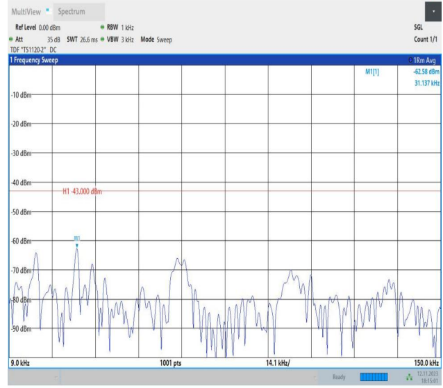
Band2_1.4MHz_16QAM_18607_1RB#0_0.009~0.15_0.009~0.15 15
