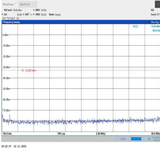
Band2_3MHz_QPSK_19185_1RB#0_0.15~30_0.15~30
