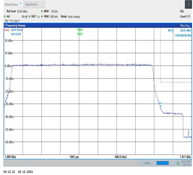
Band2_5MHz_64QAM_19175_25RB#0
