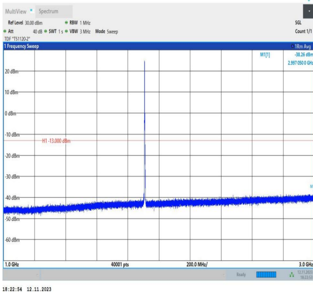
Band2_3MHz_QPSK_19185_1RB#0_1000~3000_1000~3000
