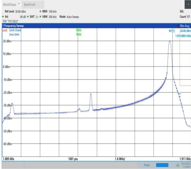
Band2_15MHz_64QAM_19125_1RB#74
