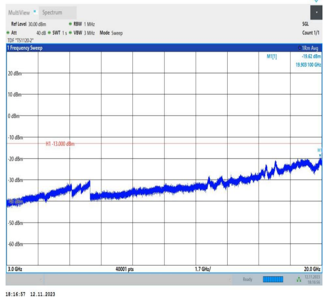
Band2_1.4MHz_16QAM_18900_1RB#0_3000~20000_3000~20000
