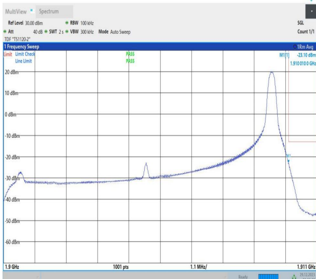
Band2_10MHz_64QAM_19150_1RB#49
