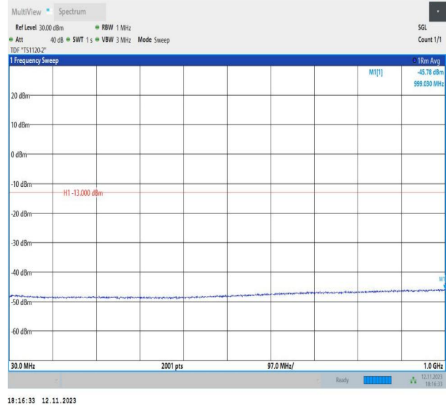
Band2_1.4MHz_16QAM_18900_1RB#0_30~1000_30~1000
