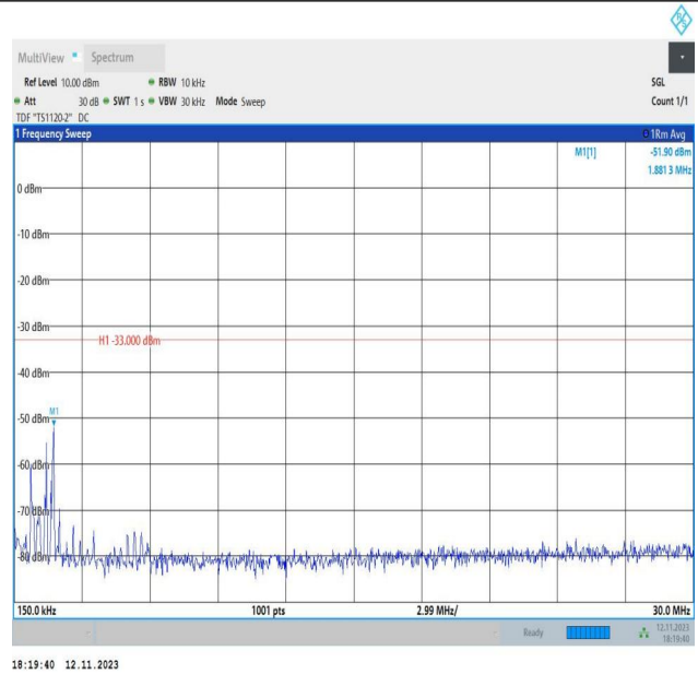
Band2_3MHz_QPSK_18615_1RB#0_0.15~30_0.15~30
