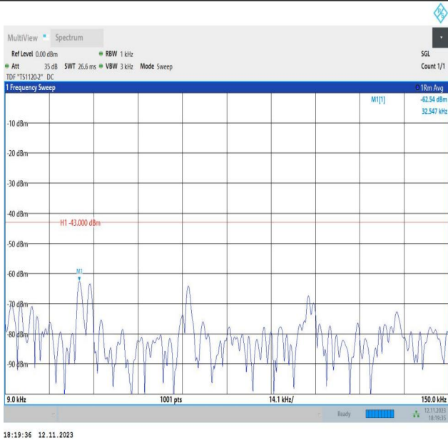
Band2_3MHz_QPSK_18615_1RB#0_0.009~0.15_0.009~0.15
