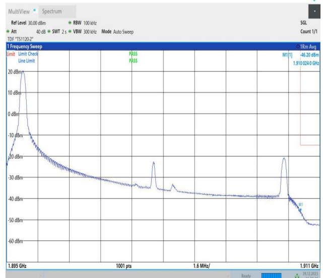
Band2_15MHz_64QAM_19125_1RB#0
