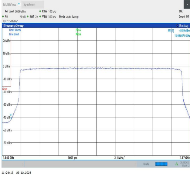
Band2_20MHz_64QAM_18700_100RB#0
