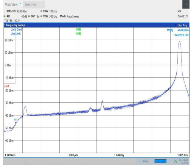
Band2_15MHz_64QAM_18675_1RB#74
