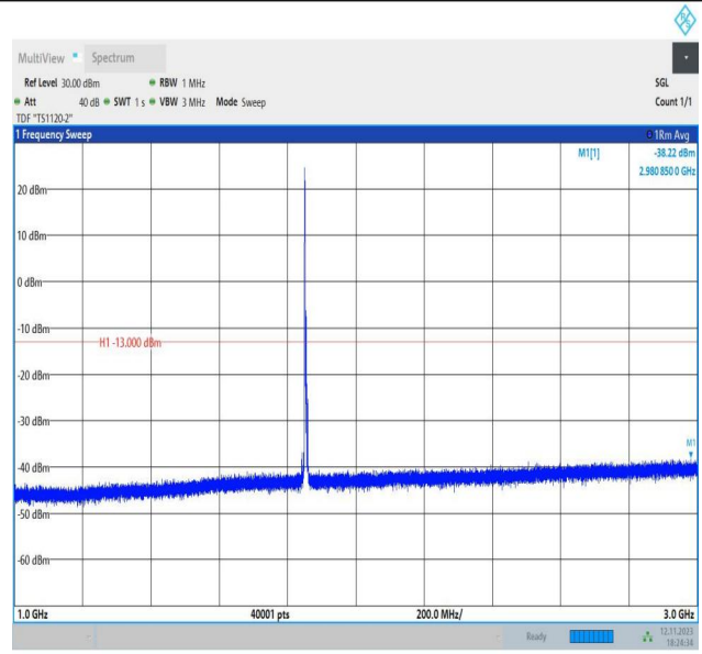
Band2_5MHz_QPSK_18625_1RB#0_1000~3000_1000~3000
