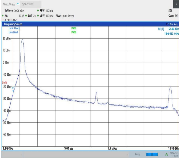
Band2_15MHz_64QAM_18675_1RB#0
