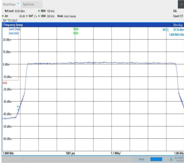
Band2_10MHz_64QAM_18650_50RB#0
