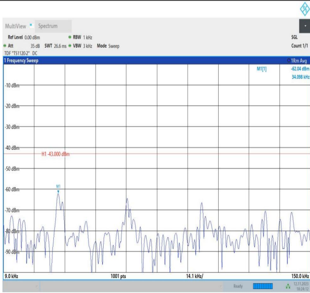
Band2_5MHz_QPSK_18625_1RB#0_0.009~0.15_0.009~0.15
