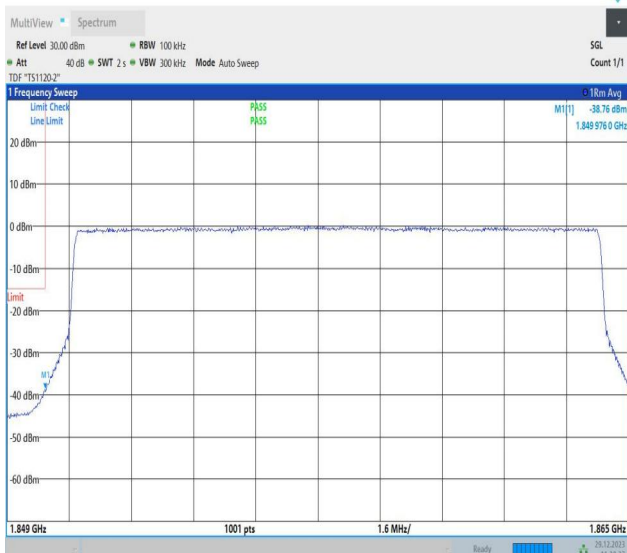
Band2_15MHz_64QAM_18675_75RB#0
