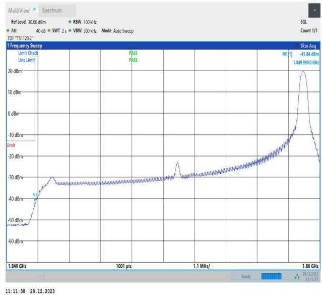
Band2_10MHz_64QAM_18650_1RB#49
