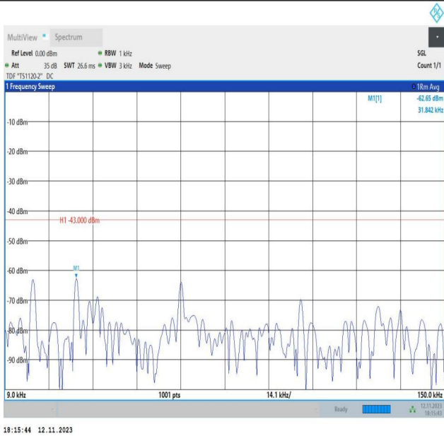
Band2_1.4MHz_QPSK_18900_1RB#0_0.009~0.15_0.009~0.15
