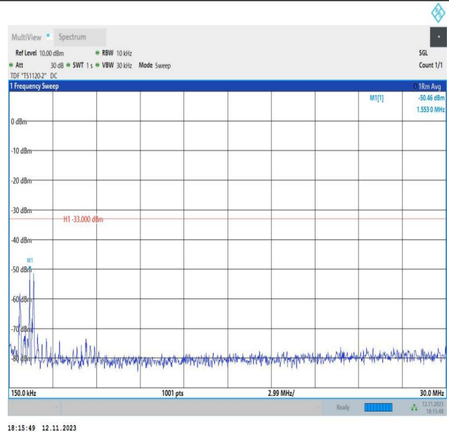
Band2_1.4MHz_QPSK_18900_1RB#0_0.15~30_0.15~30
