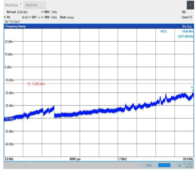
Band2_3MHz_16QAM_19185_1RB#0_3000~20000_3000~200
