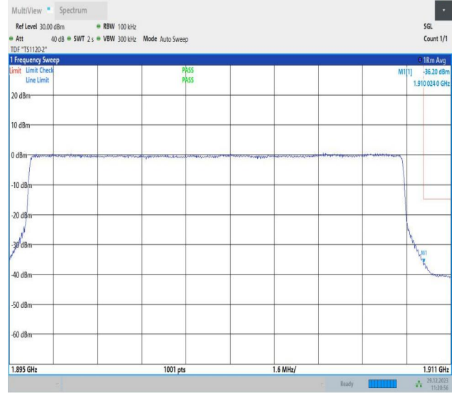
Band2_15MHz_64QAM_19125_75RB#0
