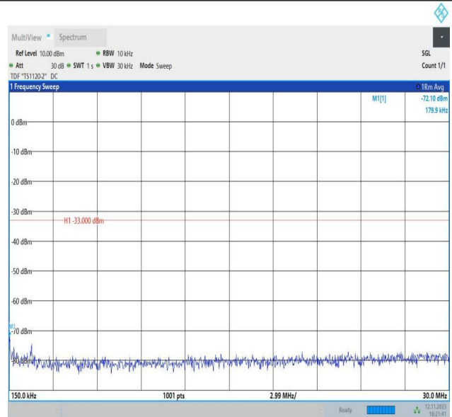
Band2_3MHz_16QAM_18900_1RB#0_0.15~30_0.15~30
