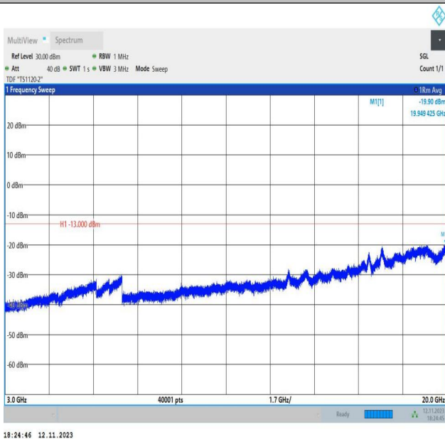
Band2_5MHz_QPSK_18625_1RB#0_3000~20000_3000~2000 00
