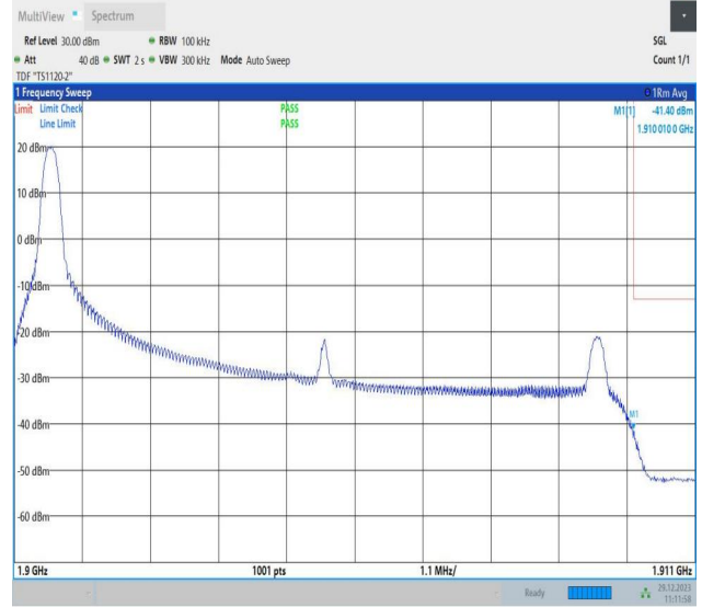
Band2_10MHz_64QAM_19150_1RB#0
