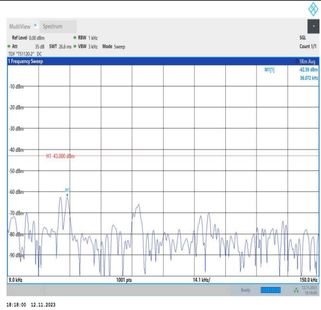
Band2_1.4MHz_16QAM_19193_1RB#0_0.009~0.15_0.009~0.15
