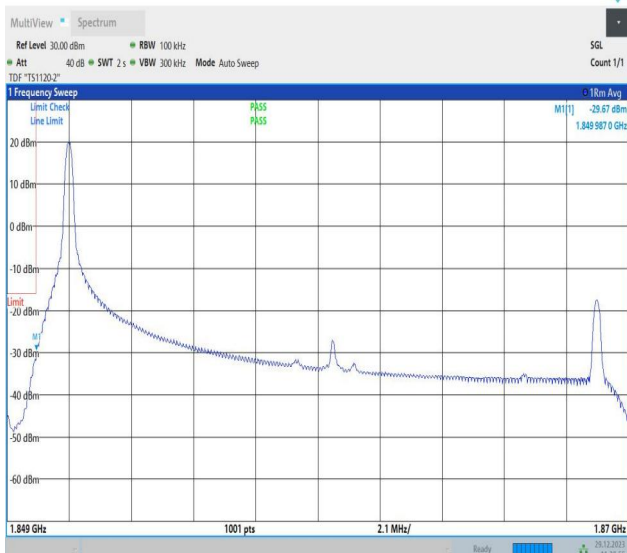
Band2_20MHz_64QAM_18700_1RB#0
