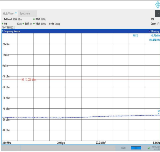
Band2_5MHz_QPSK_18625_1RB#0_30~1000_30~1000
