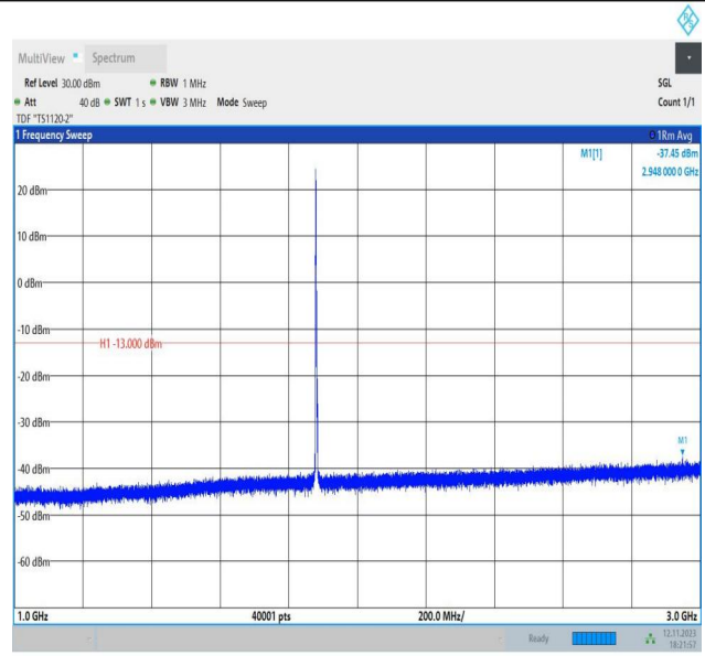
Band2_3MHz_16QAM_18900_1RB#0_1000~3000_1000~3000
