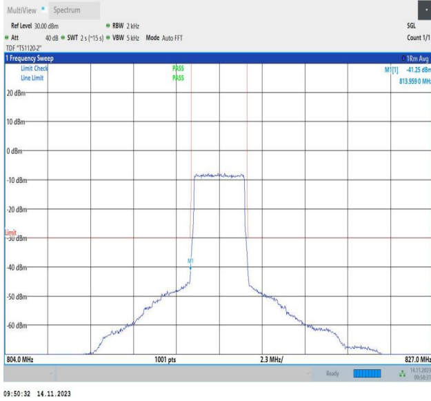
Band26_3MHz_QPSK_26705_15RB#0
