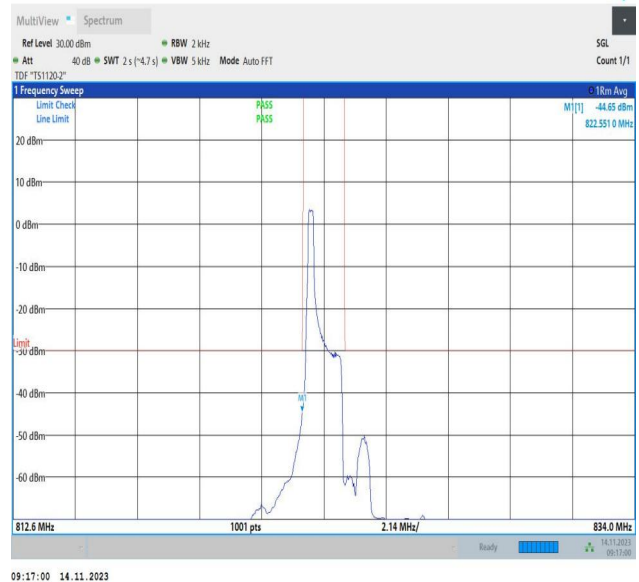
Band26_1.4MHz_16QAM_26783_1RB#0
