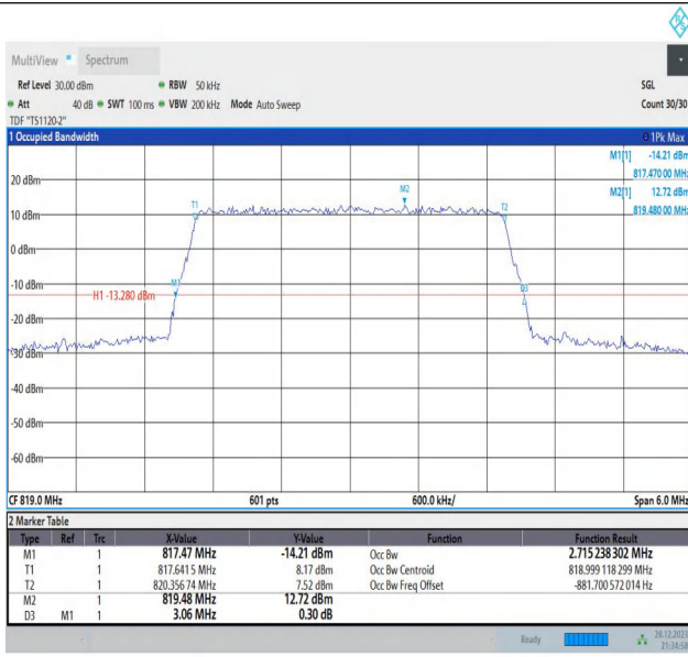
26(814-824)-3MHz-64QAM-26740-15RB#0-PASS
