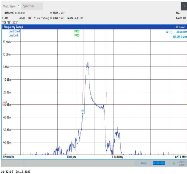
Band26_1.4MHz_64QAM_26697_1RB#0
