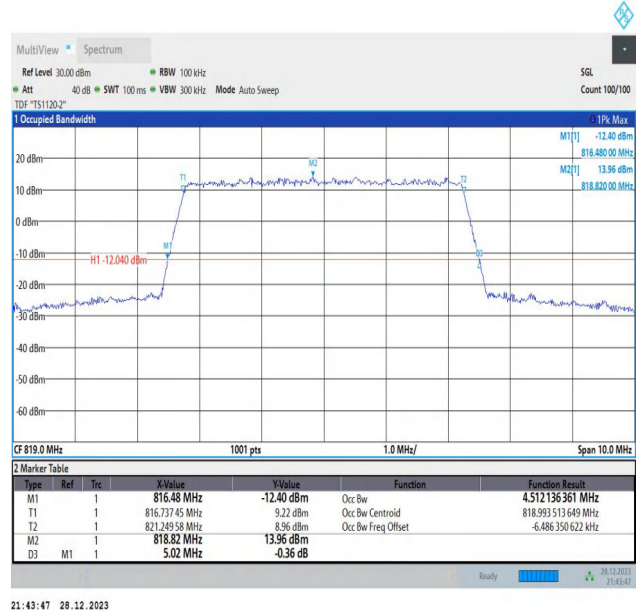
26(814-824)-5MHz-64QAM-26740-25RB#0-PASS
