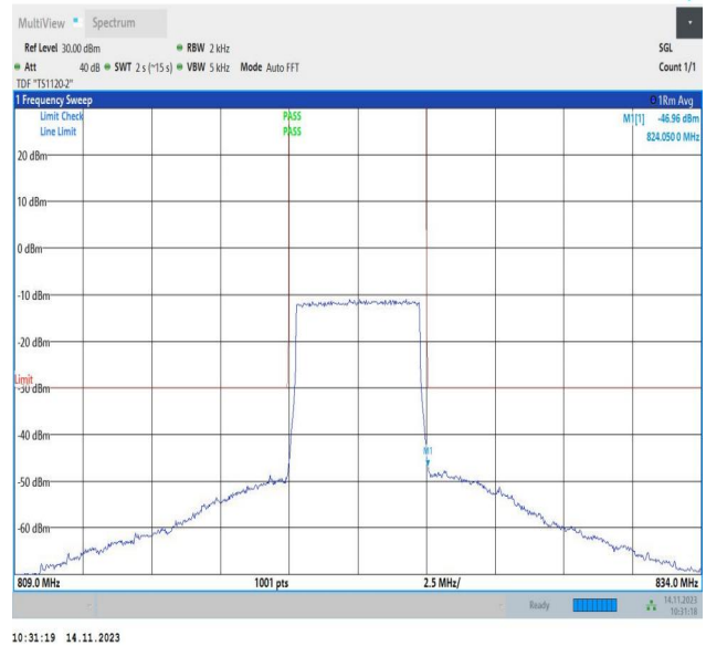
Band26_5MHz_16QAM_26765_25RB#0
