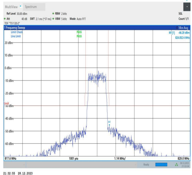
Band26_1.4MHz_64QAM_26783_6RB#0
