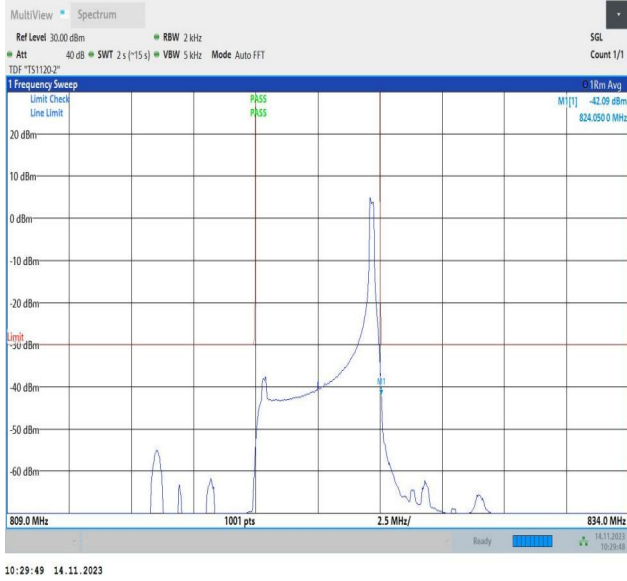
Band26_5MHz_QPSK_26765_1RB#24
