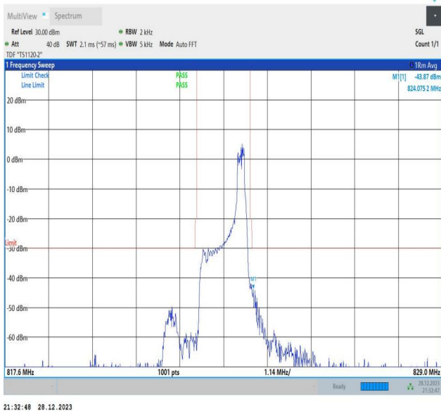
Band26_1.4MHz_64QAM_26783_1RB#5
