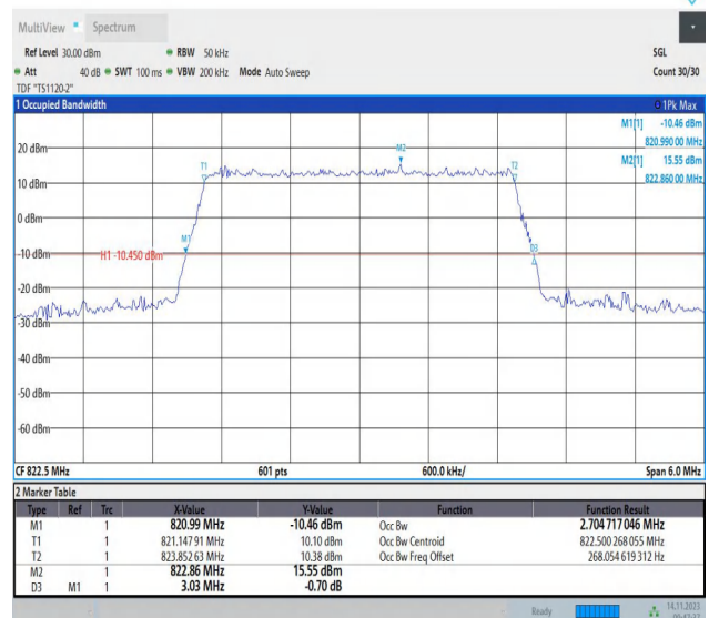
26(814-824)-3MHz-16QAM-26775-15RB#0-PASS
