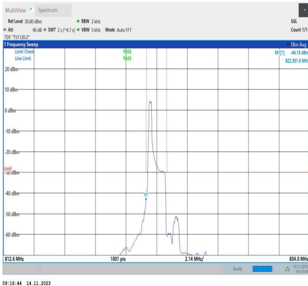
Band26_1.4MHz_QPSK_26783_1RB#0
