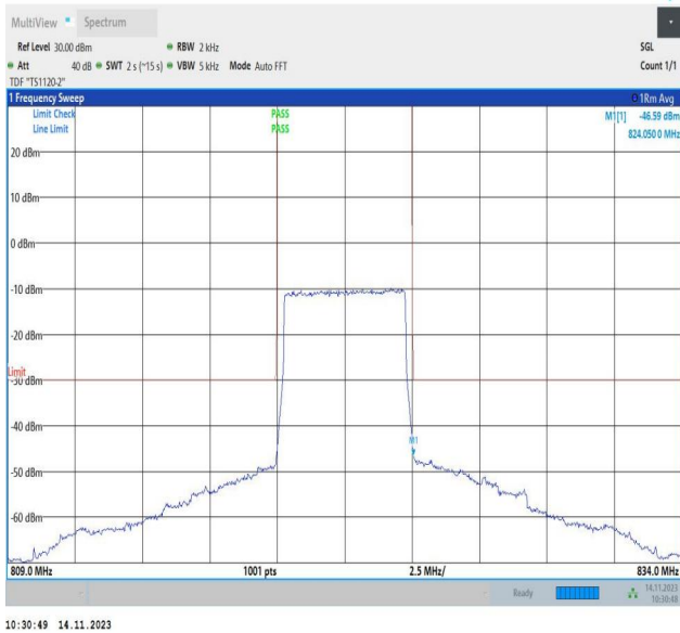
Band26_5MHz_QPSK_26765_25RB#0
