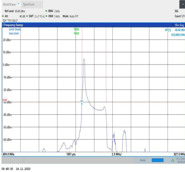
Band26_3MHz_QPSK_26705_1RB#0
