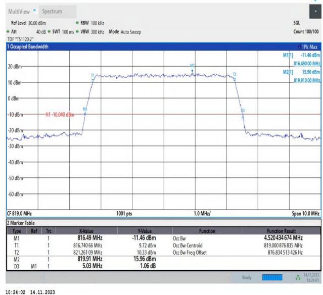
26(814-824)-5MHz-16QAM-26740-25RB#0-PASS
