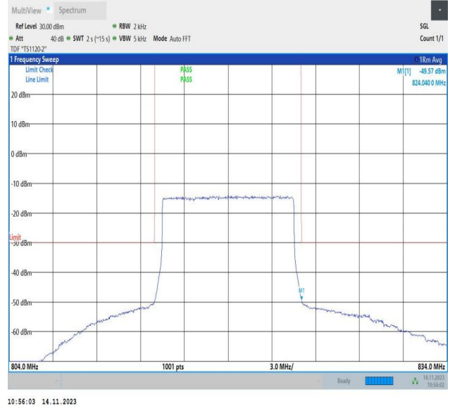
Band26_10MHz_16QAM_26740_50RB#0
