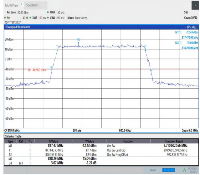
26(814-824)-3MHz-16QAM-26740-15RB#0-PASS
