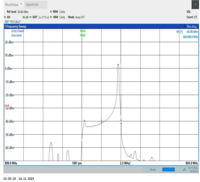
Band26_5MHz_16QAM_26765_1RB#24
