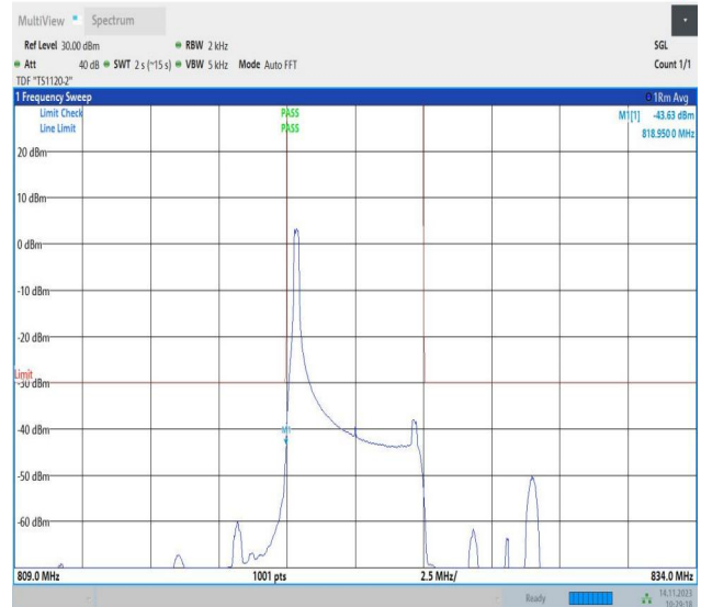
Band26_5MHz_16QAM_26765_1RB#0
