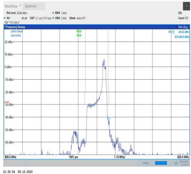
Band26_1.4MHz_64QAM_26697_1RB#5
