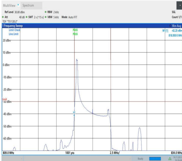
Band26_5MHz_QPSK_26765_1RB#0
