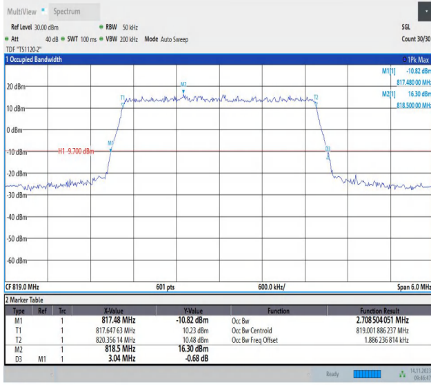
26(814-824)-3MHz-QPSK-26740-15RB#0-PASS
