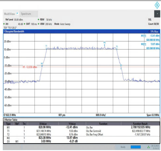
26(814-824)-3MHz-64QAM-26775-15RB#0-PASS
