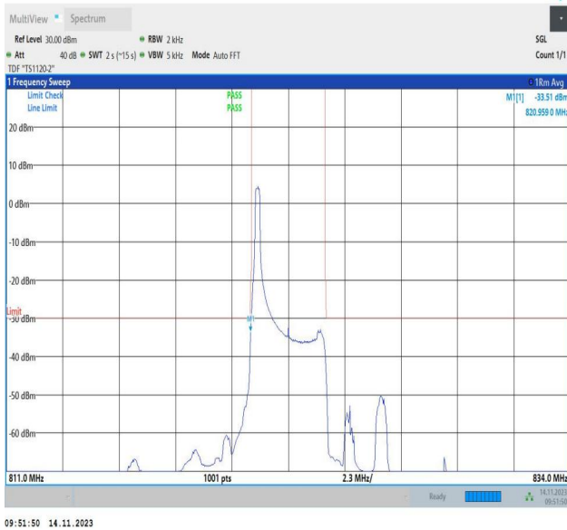
Band26_3MHz_QPSK_26775_1RB#0
