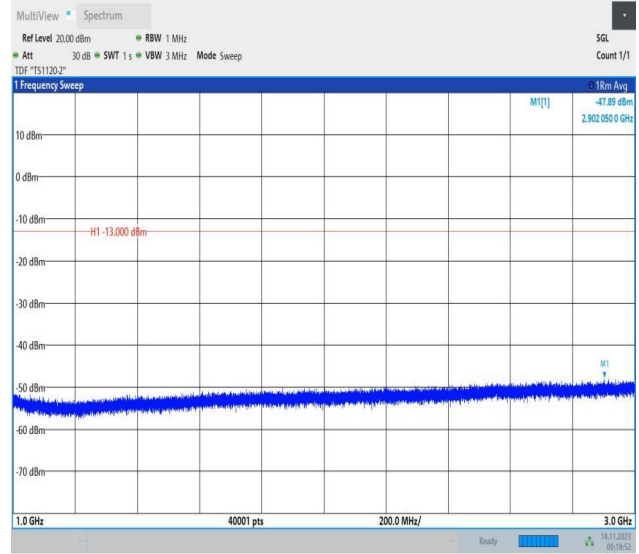
Band26_1.4MHz_QPSK_26697_1RB#0_1000~3000_1000~3000
