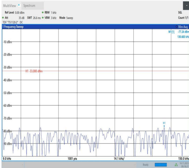
Band26_1.4MHz_QPSK_26697_1RB#0_0.009~0.15_0.009~0.15
