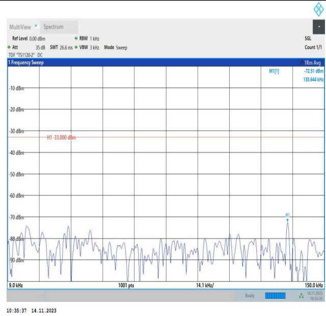
Band26_5MHz_16QAM_26765_1RB#0_0.009~0.15_0.009~0.15
