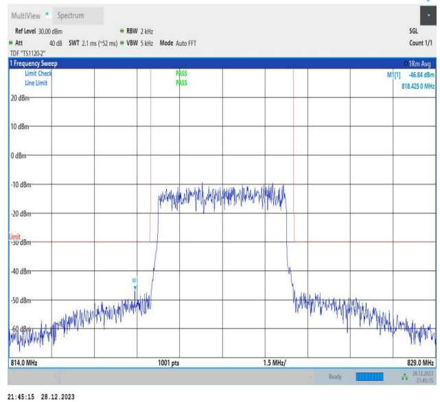
Band26_5MHz_64QAM_26765_25RB#0
