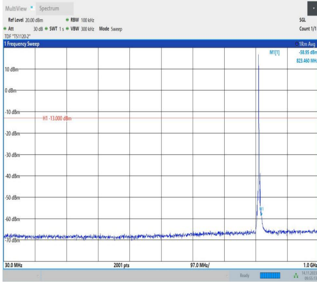
Band26_3MHz_QPSK_26705_1RB#0_30~1000_30~1000
