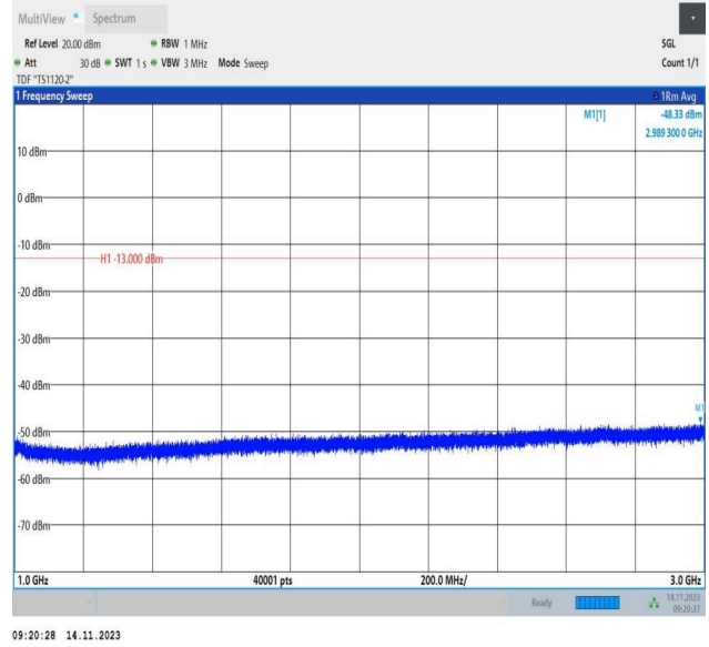
Band26_1.4MHz_QPSK_26740_1RB#0_1000~3000_1000~3000
