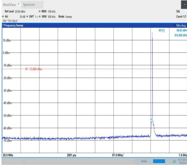
Band26_1.4MHz_QPSK_26697_1RB#0_30~1000_30~1000
