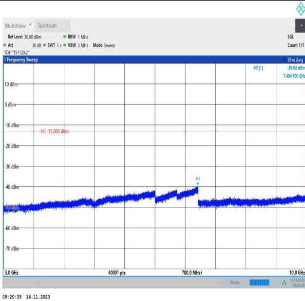
Band26_1.4MHz_QPSK_26740_1RB#0_3000~10000_3000~10000
