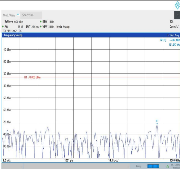
Band26_1.4MHz_16QAM_26783_1RB#0_1000~3000_1000~3000
