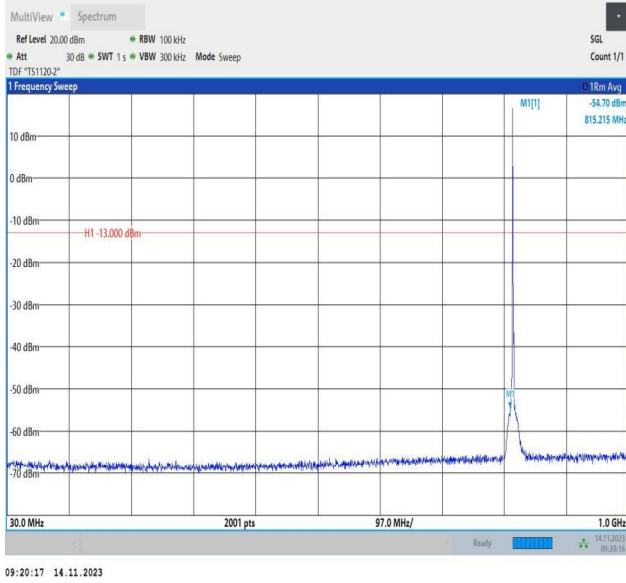
Band26_1.4MHz_QPSK_26740_1RB#0_30~1000_30~1000
