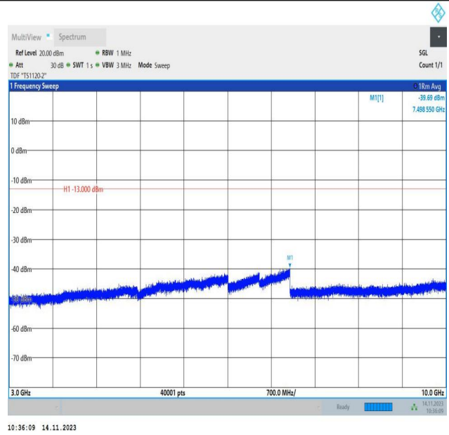
Band26_5MHz_16QAM_26765_1RB#0_3000~10000_3000~10000
