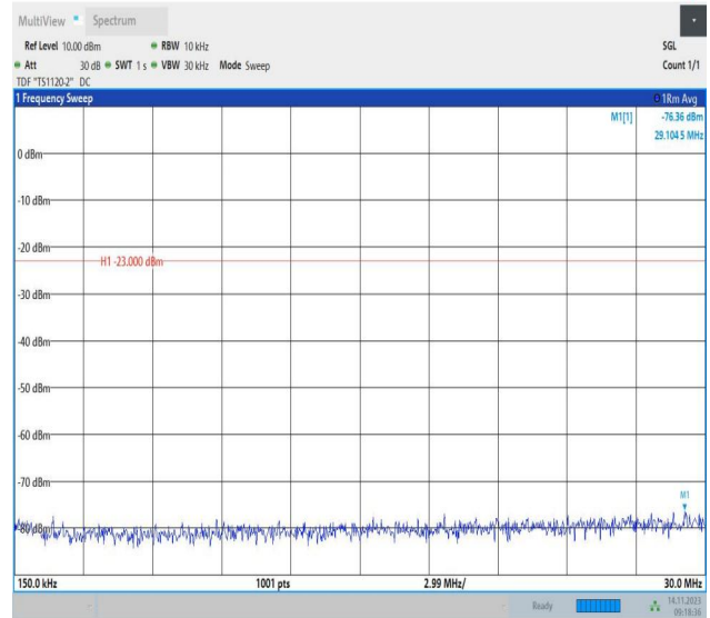
Band26_1.4MHz_QPSK_26697_1RB#0_0.15~30_0.15~30
