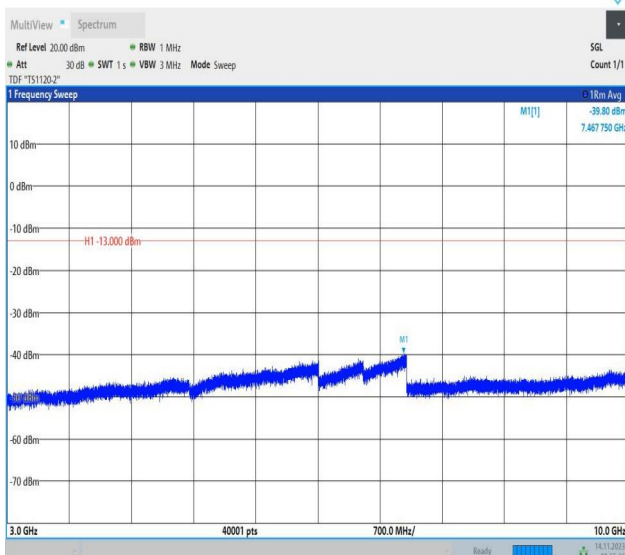
Band26_3MHz_QPSK_26705_1RB#0_3000~10000_3000~10000
