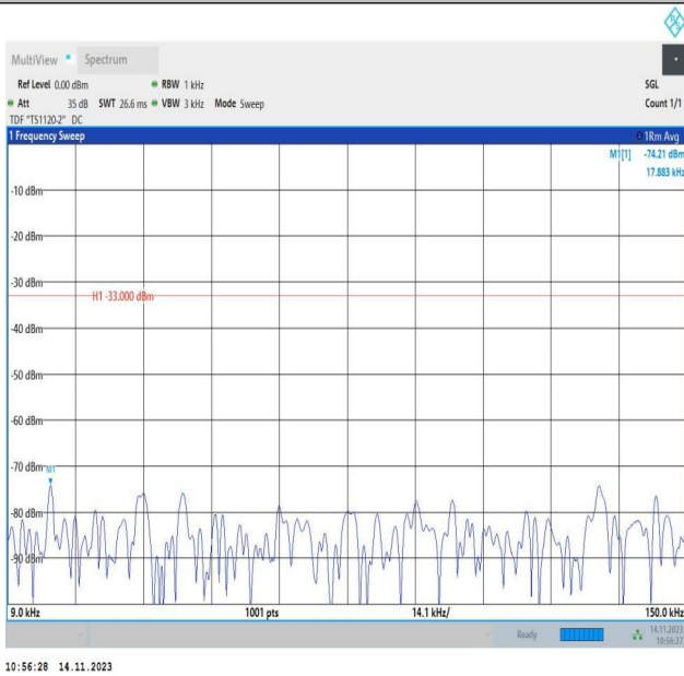
Band26_10MHz_QPSK_26740_1RB#0_0.009~0.15_0.009~0.15
