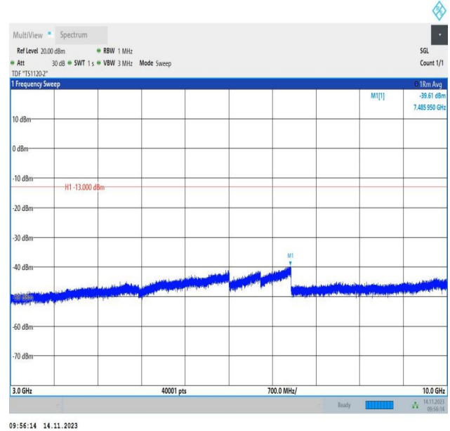
Band26_3MHz_16QAM_26705_1RB#0_3000~10000_3000~10
