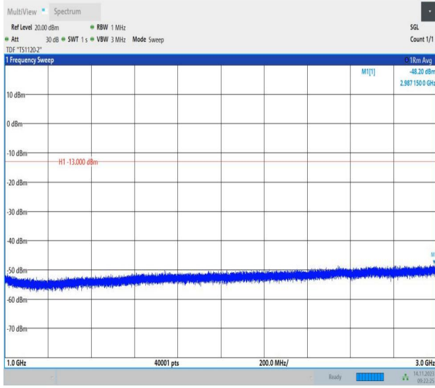
Band26_1.4MHz_16QAM_26783_1RB#0_1000~3000_1000~3000
