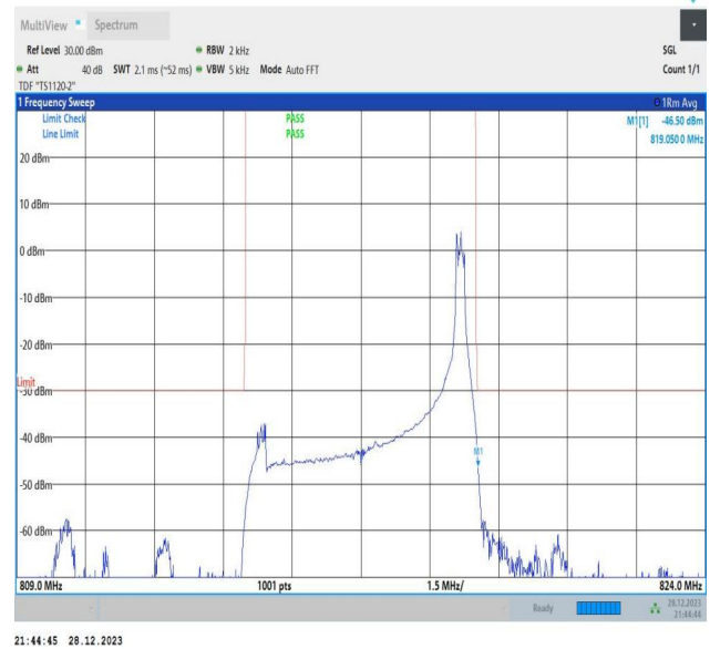
Band26_5MHz_64QAM_26715_1RB#24
