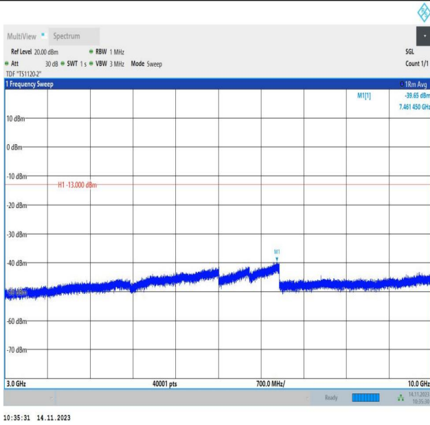
Band26_5MHz_QPSK_26765_1RB#0_3000~10000_3000~10000
