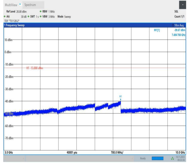
Band26_1.4MHz_16QAM_26783_1RB#0_3000~10000_3000~10000
