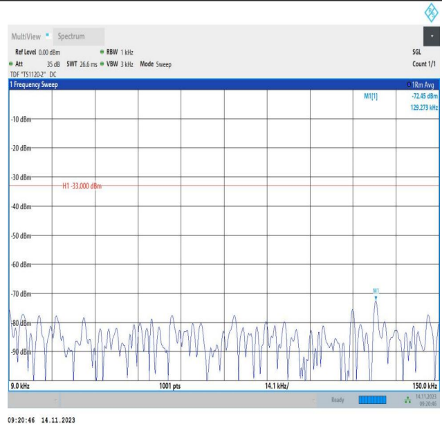
Band26_1.4MHz_16QAM_26740_1RB#0_0.009~0.15_0.009~0.15
