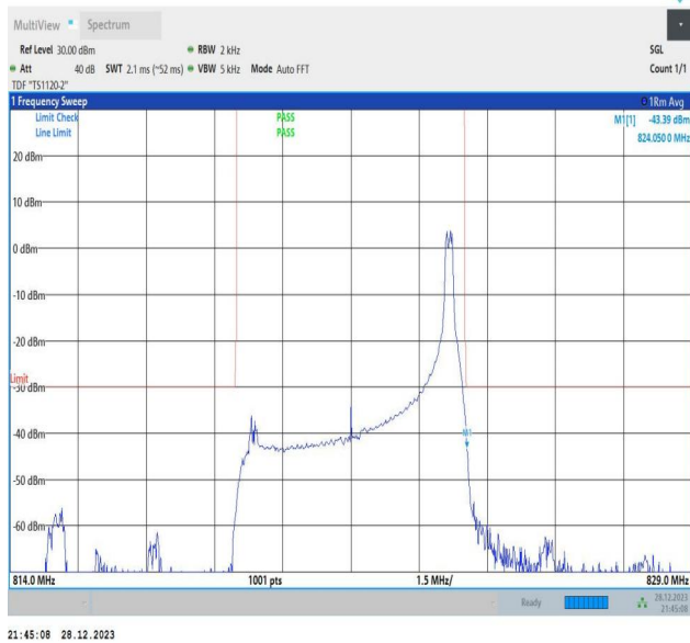
Band26_5MHz_64QAM_26765_1RB#24
