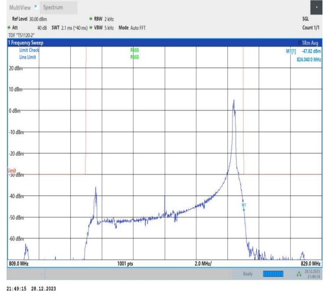
Band26_10MHz_64QAM_26740_1RB#49
