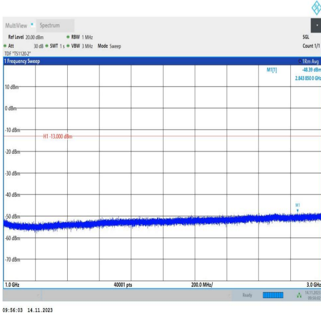
Band26_3MHz_16QAM_26705_1RB#0_1000~3000_1000~30
