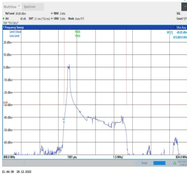
Band26_5MHz_64QAM_26715_1RB#0
