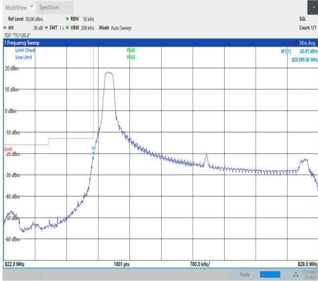
Band26_5MHz_QPSK_26815_1RB#0
