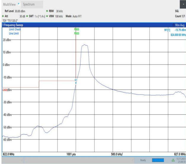
Band26_3MHz_QPSK_26805_1RB#0
