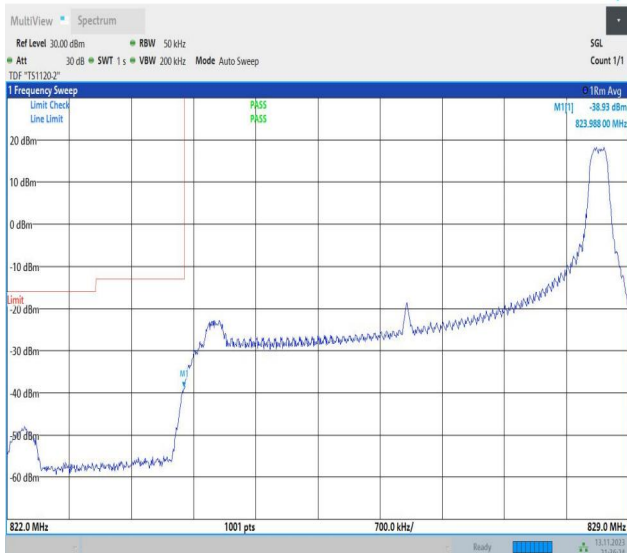
Band26_5MHz_QPSK_26815_1RB#24
