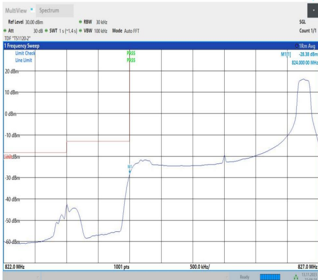
Band26_3MHz_QPSK_26805_1RB#14
