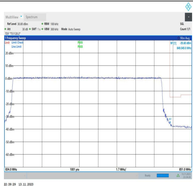
Band26_15MHz_16QAM_26965_75RB#0
