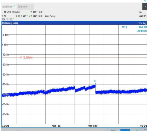
Band26_3MHz_QPSK_27025_1RB#0_3000~10000_3000~10000
