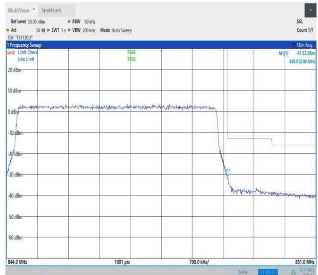
Band26_5MHz_16QAM_27015_25RB#0
