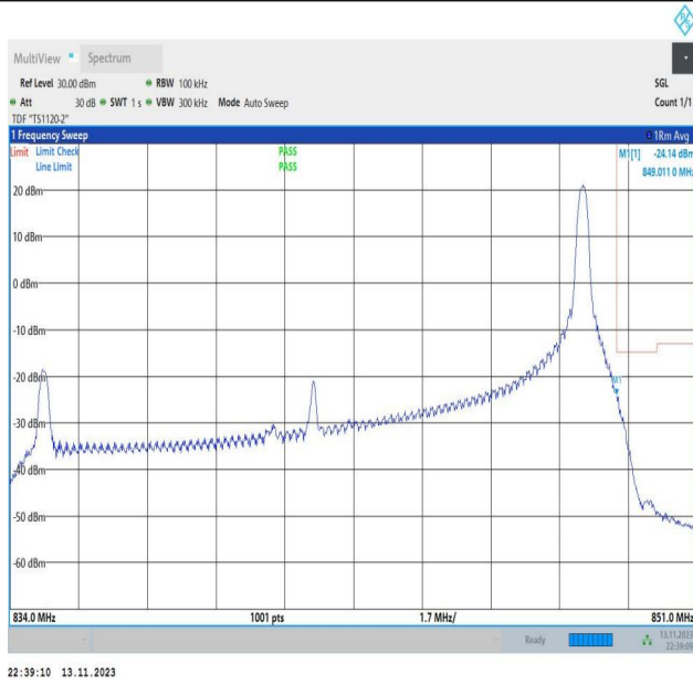
Band26_15MHz_QPSK_26965_1RB#74
