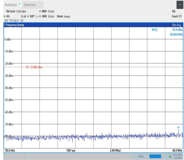
Band26_1.4MHz_QPSK_27033_1RB#0_0.15~30_0.15~30
