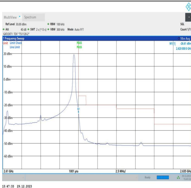
Band38_10MHz_64QAM_38200_1RB#49
