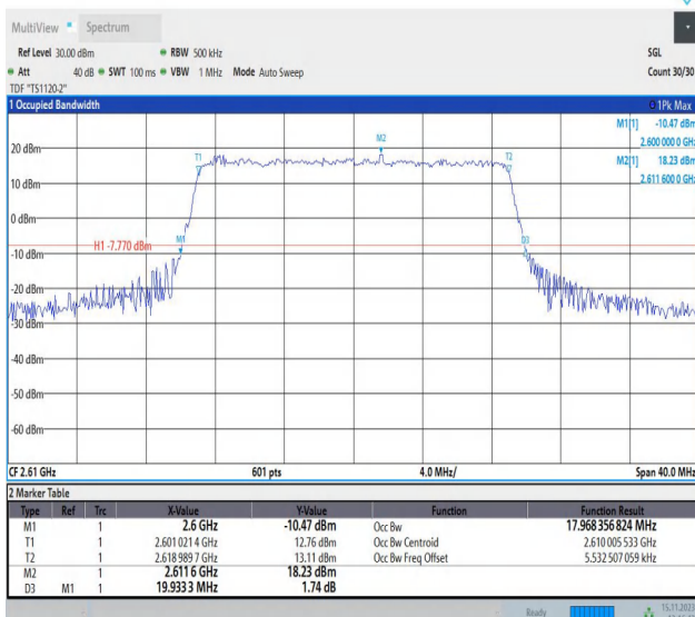
Band38-20MHz-QPSK-38150-100RB#0-PASS
