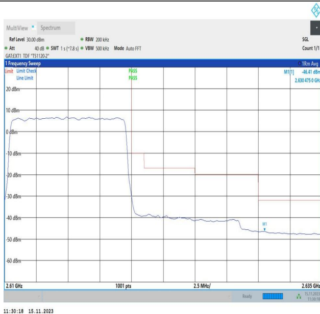
Band38_10MHz_QPSK_38200_50RB#0
