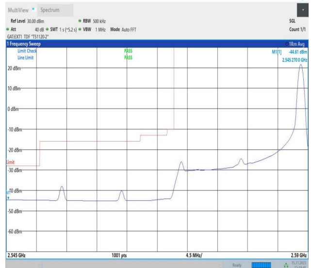
Band38_20MHz_16QAM_37850_1RB#99
