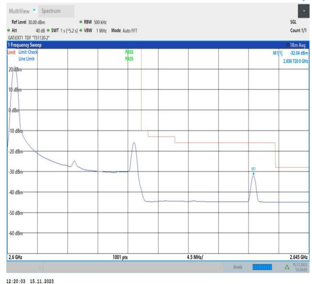
Band38_20MHz_16QAM_38150_1RB#0
