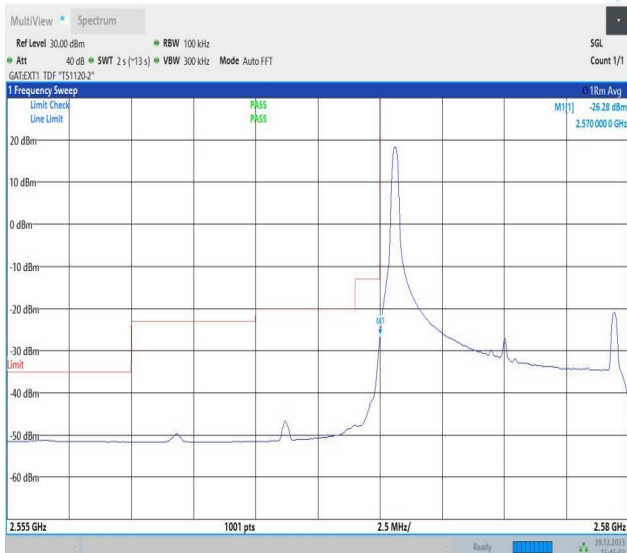
Band38_10MHz_64QAM_37800_1RB#0
