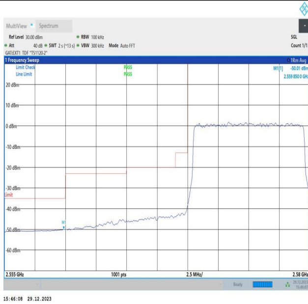
Band38_10MHz_64QAM_37800_50RB#0
