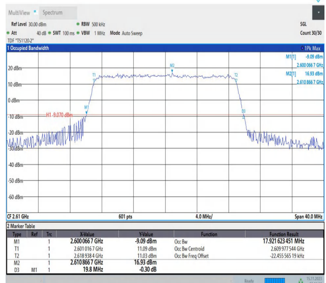
Band38-20MHz-16QAM-38150-100RB#0-PASS
