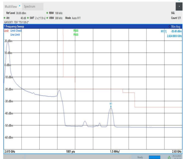
Band38_5MHz_64QAM_38225_1RB#0
