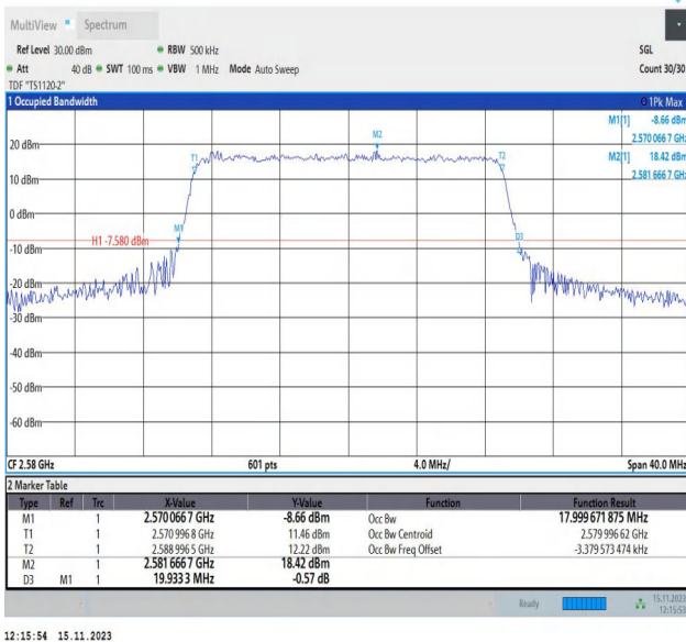
Band38-20MHz-QPSK-37850-100RB#0-PASS
