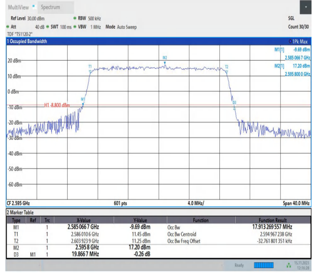
Band38-20MHz-16QAM-38000-100RB#0-PASS
