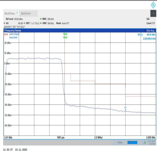
Band38_10MHz_16QAM_38200_50RB#0
