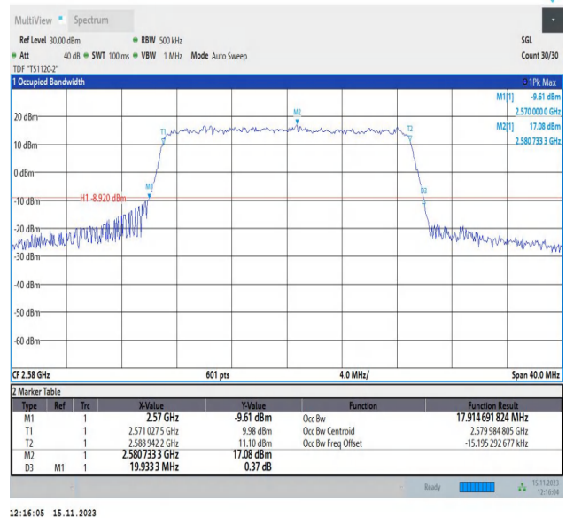
Band38-20MHz-16QAM-37850-100RB#0-PASS
