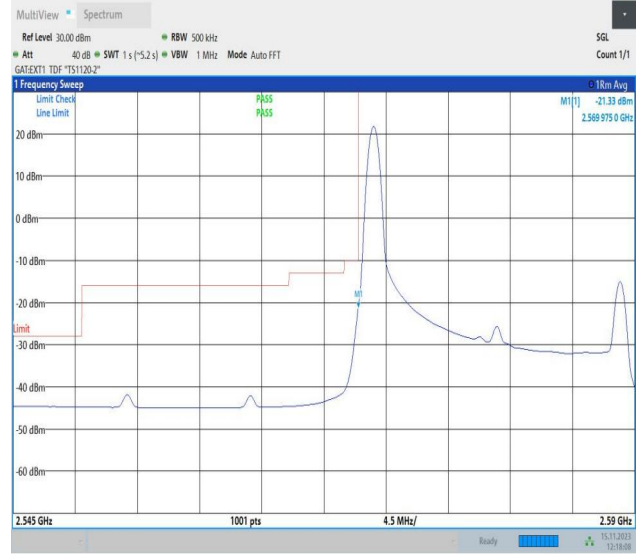
Band38_20MHz_16QAM_37850_1RB#0
