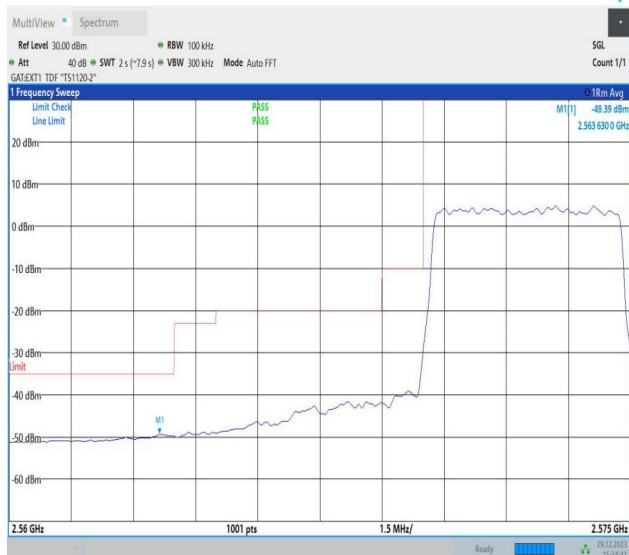
Band38_5MHz_64QAM_37775_25RB#0
