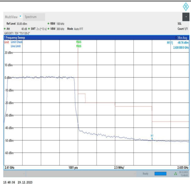
Band38_10MHz_64QAM_38200_50RB#0
