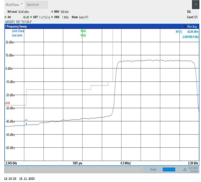
Band38_20MHz_16QAM_37850_100RB#0
