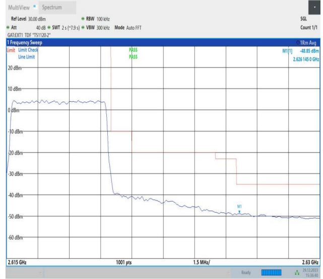
Band38_5MHz_64QAM_38225_25RB#0
