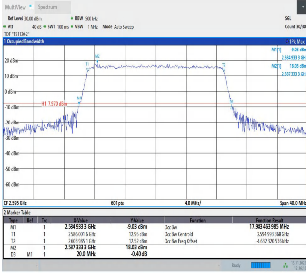
Band38-20MHz-QPSK-38000-100RB#0-PASS
