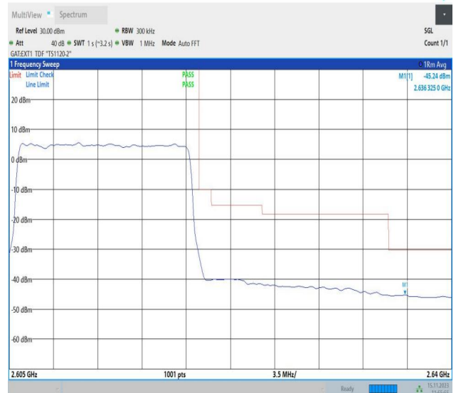
Band38_15MHz_16QAM_38175_75RB#0
