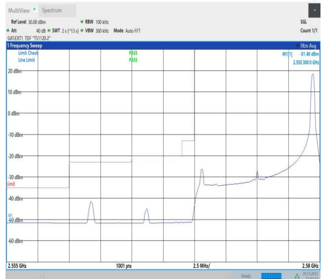
Band38_10MHz_64QAM_37800_1RB#49
