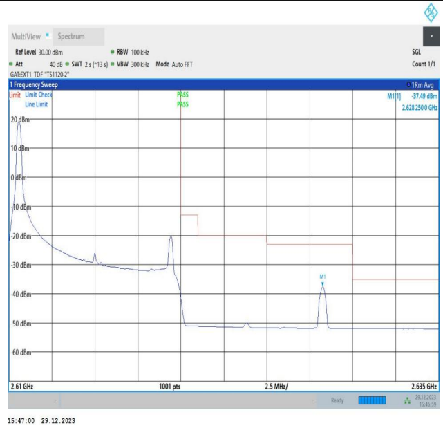
Band38_10MHz_64QAM_38200_1RB#0
