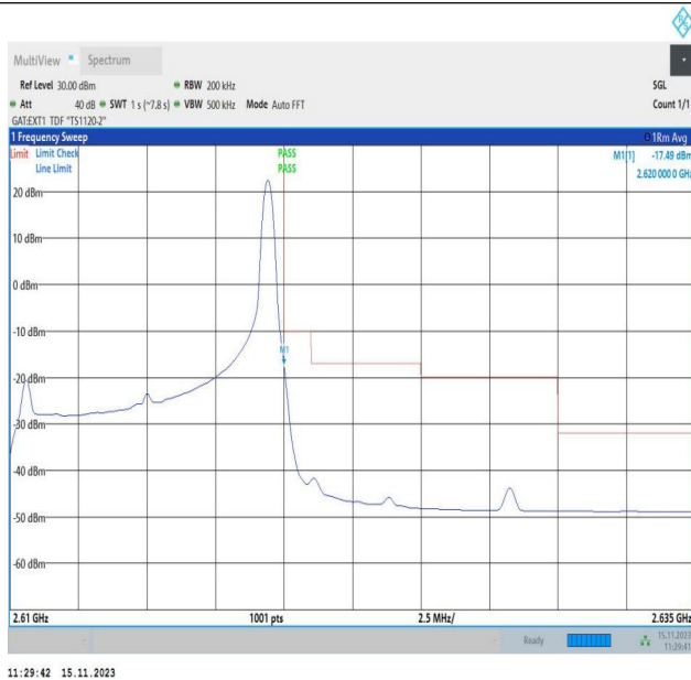
Band38_10MHz_QPSK_38200_1RB#49
