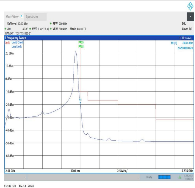
Band38_10MHz_16QAM_38200_1RB#49
