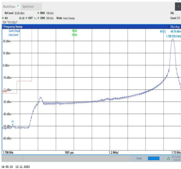
Band4_10MHz_QPSK_20000_1RB#49
