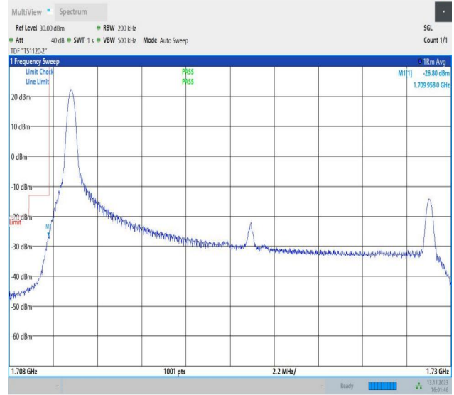
Band4_20MHz_16QAM_20050_1RB#0
