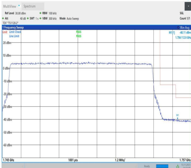
Band4_10MHz_QPSK_20350_50RB#0
