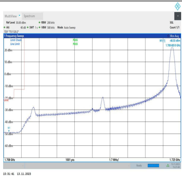
Band4_15MHz_16QAM_20025_1RB#74
