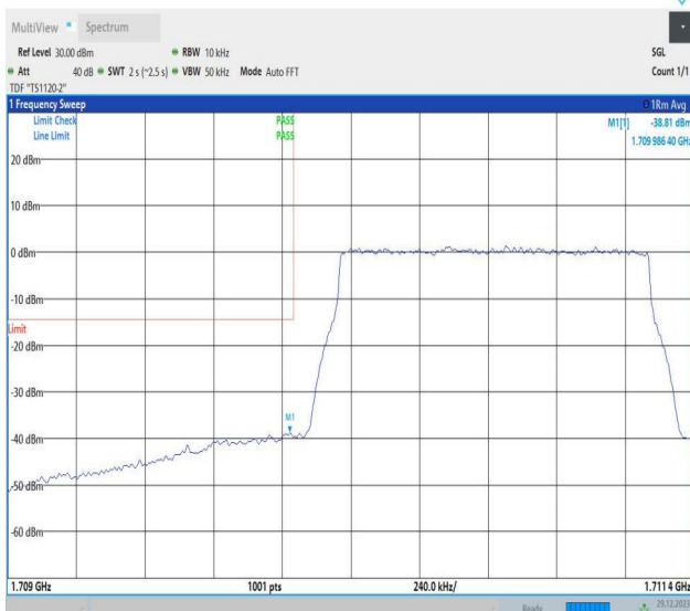
Band4_1.4MHz_64QAM_19957_6RB#0
