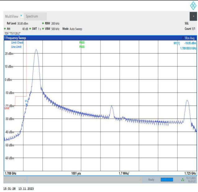
Band4_15MHz_16QAM_20025_1RB#0
