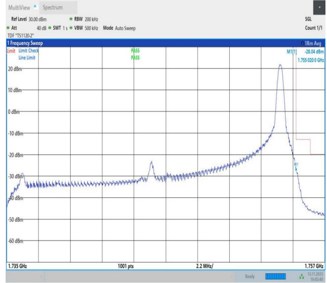
Band4_20MHz_16QAM_20300_1RB#99
