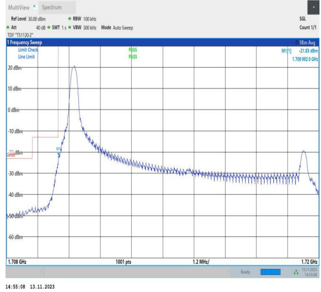
Band4_10MHz_16QAM_20000_1RB#0
