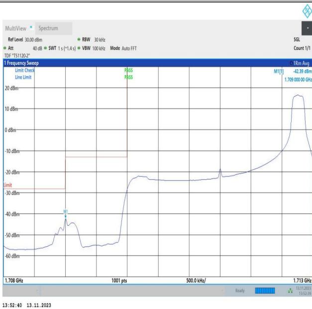
Band4_3MHz_QPSK_19965_1RB#14
