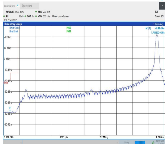
Band4_20MHz_16QAM_20050_1RB#99
