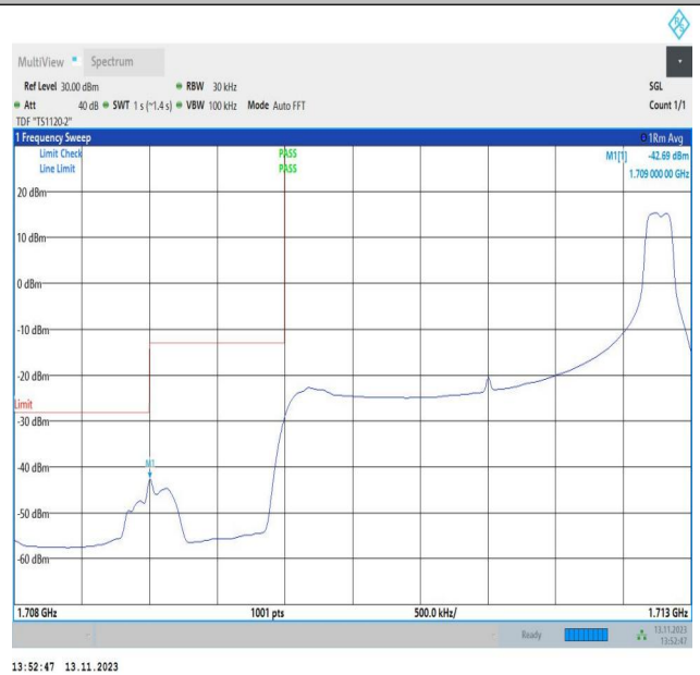
Band4_3MHz_16QAM_19965_1RB#14
