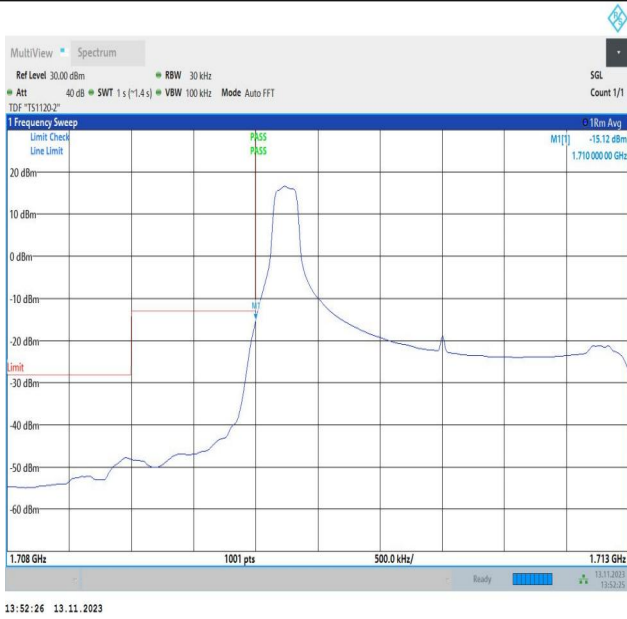
Band4_3MHz_QPSK_19965_1RB#0
