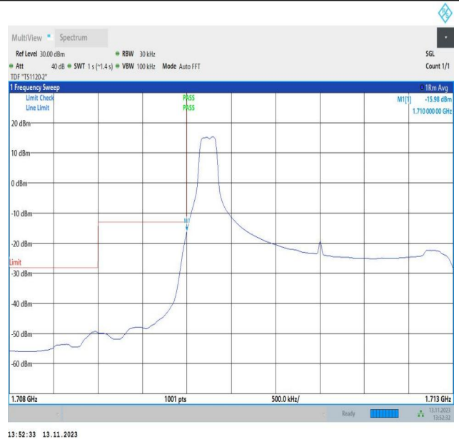
Band4_3MHz_16QAM_19965_1RB#0
