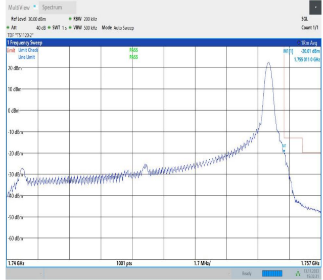
Band4_15MHz_16QAM_20325_1RB#74
