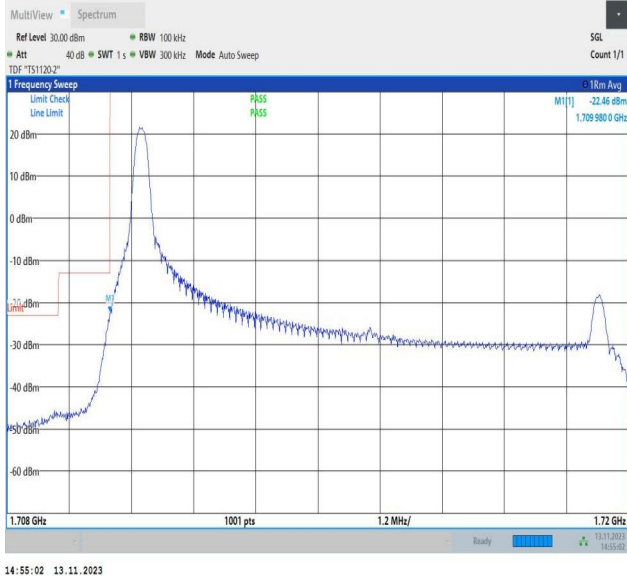
Band4_10MHz_QPSK_20000_1RB#0
