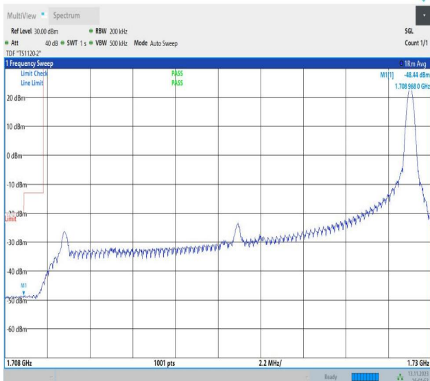
Band4_20MHz_QPSK_20050_1RB#99
