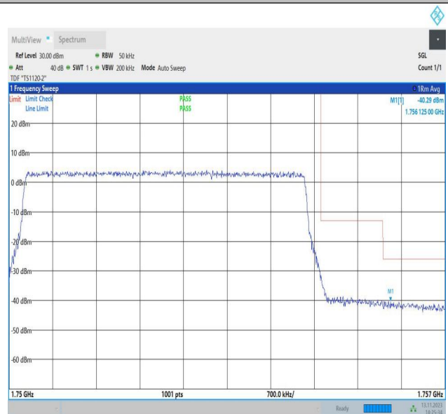
Band4_5MHz_16QAM_20375_1RB#24
