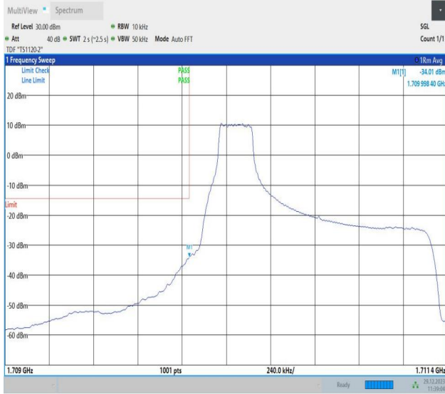
Band4_1.4MHz_64QAM_19957_1RB#0
