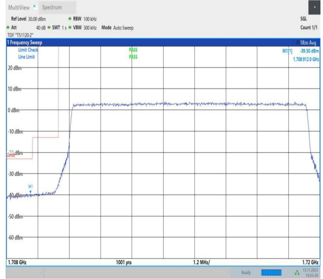
Band4_10MHz_16QAM_20000_50RB#0
