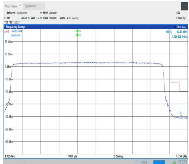
Band4_20MHz_16QAM_20300_100RB#0
