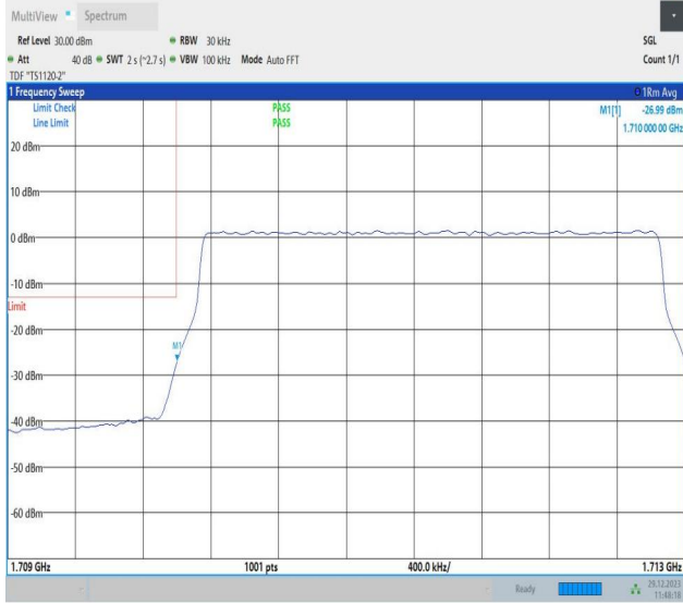
Band4_3MHz_64QAM_19965_15RB#0
