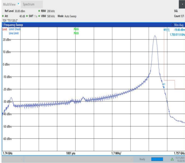
Band4_15MHz_QPSK_20325_1RB#74
