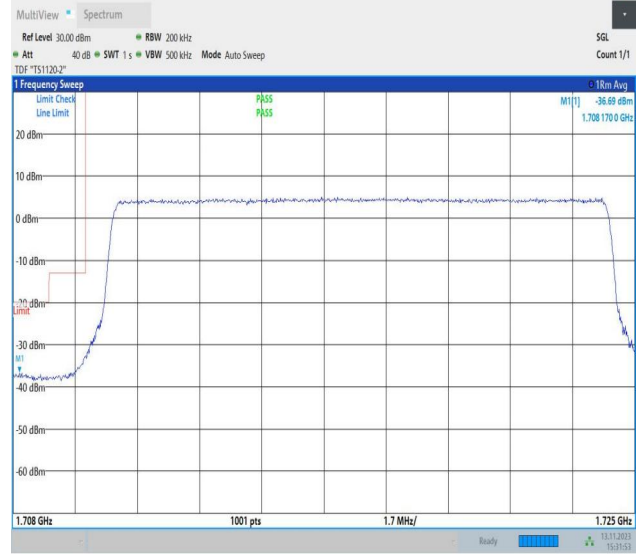
Band4_15MHz_16QAM_20025_75RB#0
