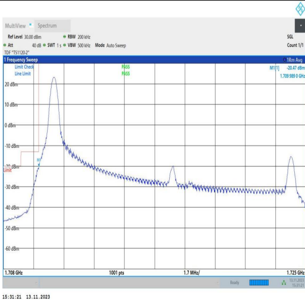
Band4_15MHz_QPSK_20025_1RB#0
