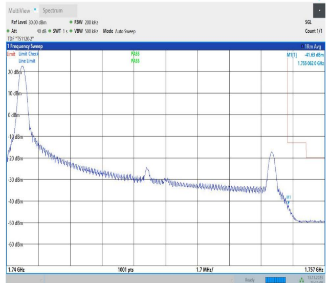
Band4_15MHz_16QAM_20325_1RB#0
