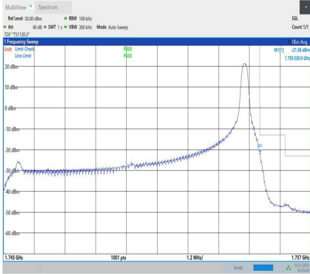
Band4_10MHz_QPSK_20350_1RB#49
