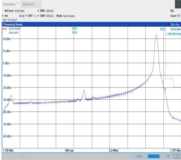
Band4_20MHz_QPSK_20300_1RB#99
