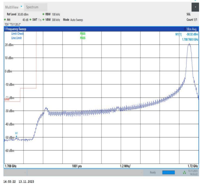
Band4_10MHz_16QAM_20000_1RB#49
