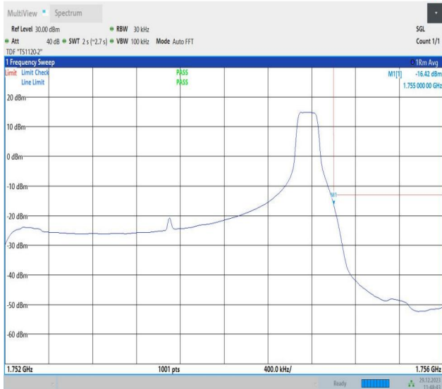
Band4_3MHz_64QAM_20385_1RB#14
