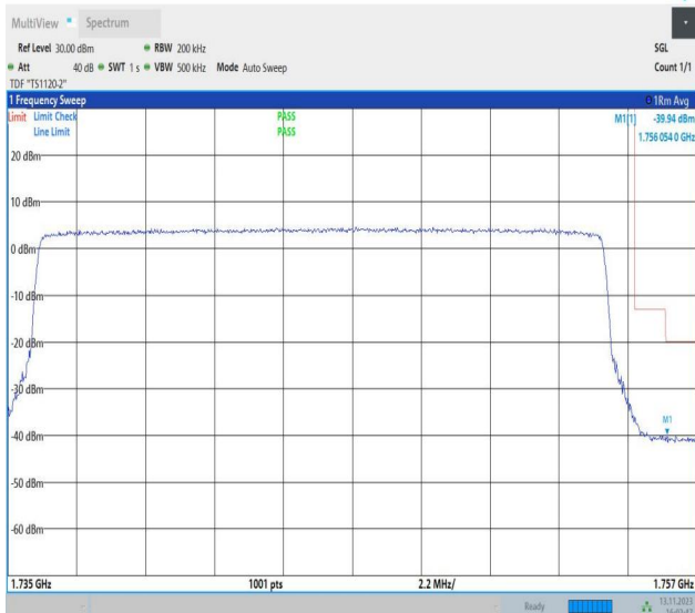
Band4_20MHz_QPSK_20300_100RB#0
