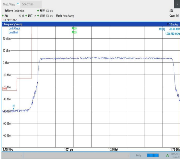
Band4_10MHz_QPSK_20000_50RB#0
