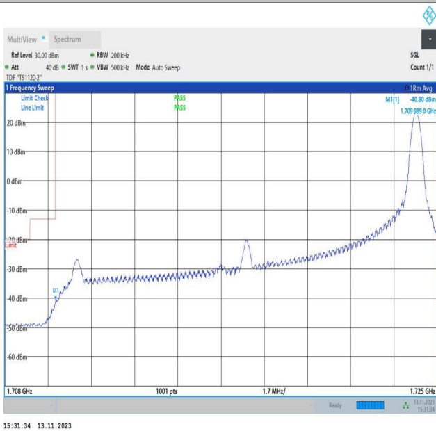
Band4_15MHz_QPSK_20025_1RB#74
