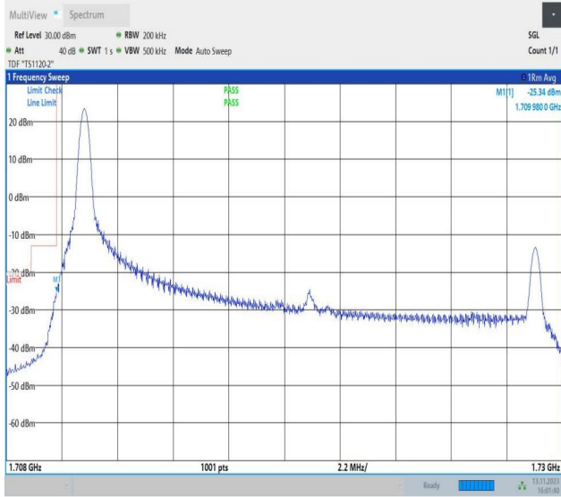
Band4_20MHz_QPSK_20050_1RB#0
