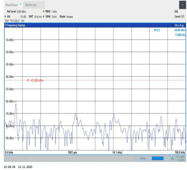
Band4_1.4MHz_16QAM_19957_1RB#0_0.009~0.15_0.009~0.15
