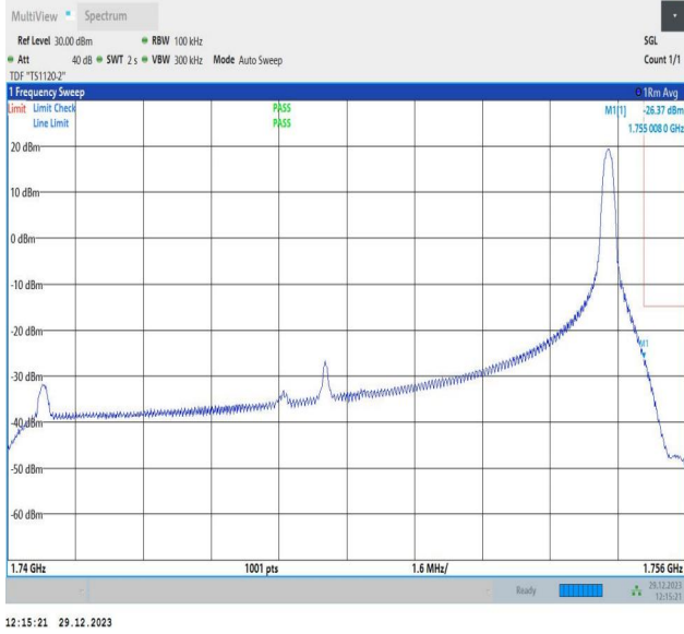
Band4_15MHz_64QAM_20325_1RB#74
