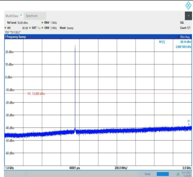
Band4_1.4MHz_QPSK_20393_1RB#0_1000~3000_1000~3000
