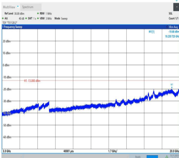
Band4_3MHz_QPSK_19965_1RB#0_3000~20000_3000~20000
