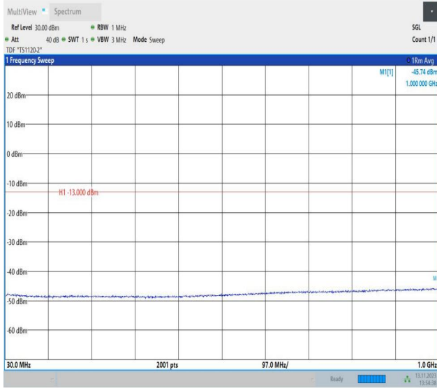
Band4_3MHz_QPSK_19965_1RB#0_30~1000_30~1000
