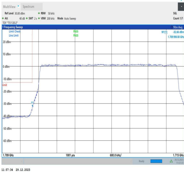
Band4_5MHz_64QAM_19975_25RB#0
