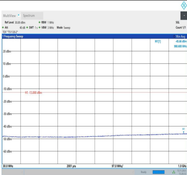
Band4_1.4MHz_QPSK_20393_1RB#0_30~1000_30~1000
