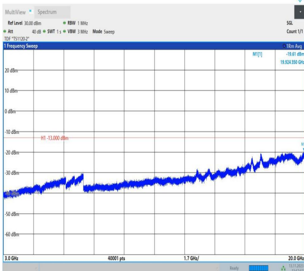
Band4_3MHz_QPSK_20385_1RB#0_3000~20000_3000~2000 00
