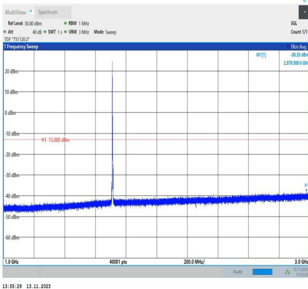
Band4_3MHz_16QAM_19965_1RB#0_1000~3000_1000~3000 0
