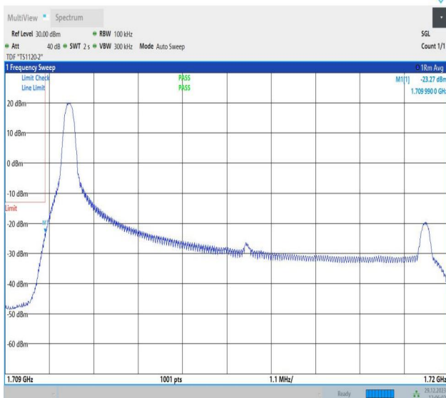
Band4_10MHz_64QAM_20000_1RB#0
