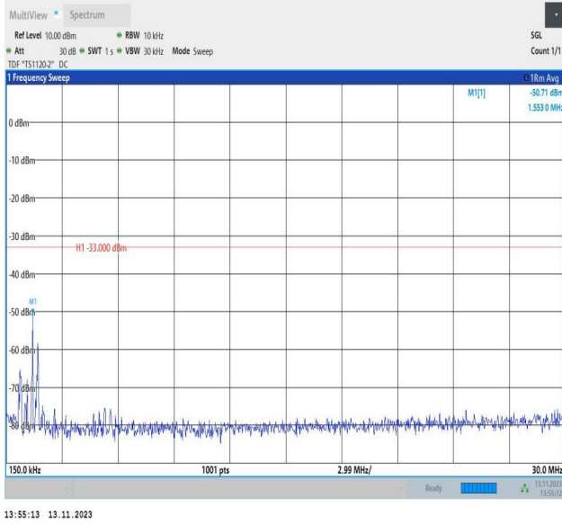
Band4_3MHz_16QAM_19965_1RB#0_0.15~30_0.15~30
