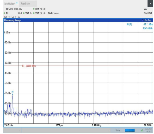
Band4_1.4MHz_QPSK_20393_1RB#0_0.15~30_0.15~30
