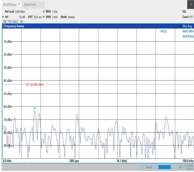
Band4_1.4MHz_QPSK_20393_1RB#0_0.009~0.15_0.009~0.15
