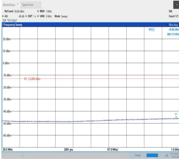
Band4_3MHz_QPSK_20385_1RB#0_30~1000_30~1000
