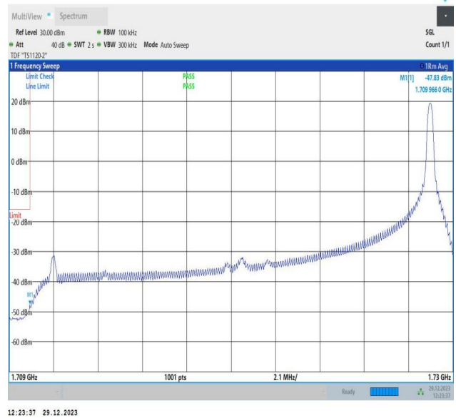
Band4_20MHz_64QAM_20050_1RB#99
