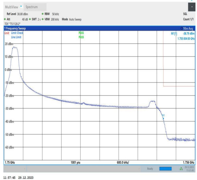
Band4_5MHz_64QAM_20375_1RB#0
