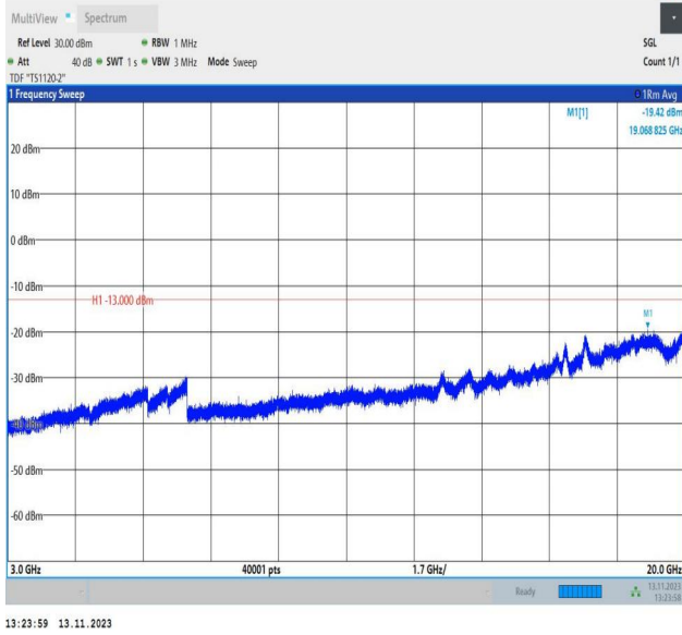
Band4_1.4MHz_QPSK_19957_1RB#0_3000~20000_3000~20000
