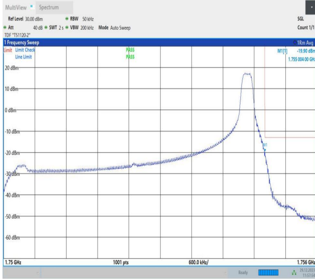
Band4_5MHz_64QAM_20375_1RB#24
