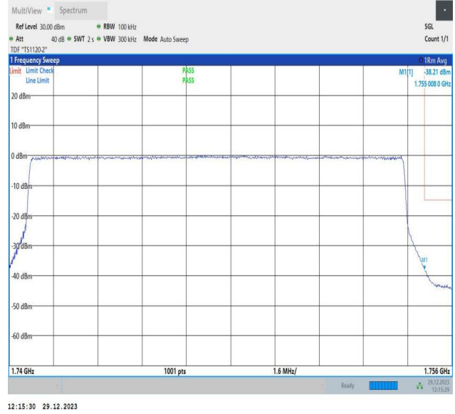
Band4_15MHz_64QAM_20325_75RB#0
