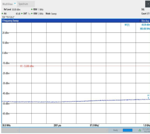
Band4_5MHz_QPSK_20175_1RB#0_30~1000_30~1000
