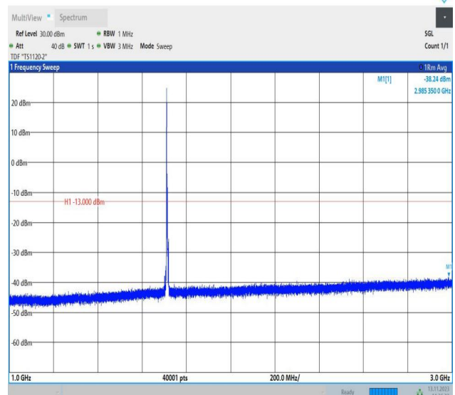
Band4_5MHz_QPSK_19975_1RB#0_1000~3000_1000~3000
