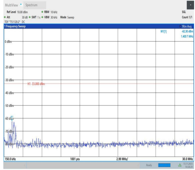
Band4_10MHz_QPSK_20175_1RB#0_0.15~30_0.15~30
