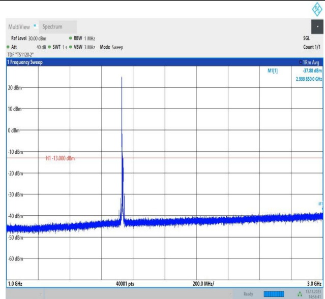
Band4_10MHz_QPSK_20175_1RB#0_1000~3000_1000~3000
