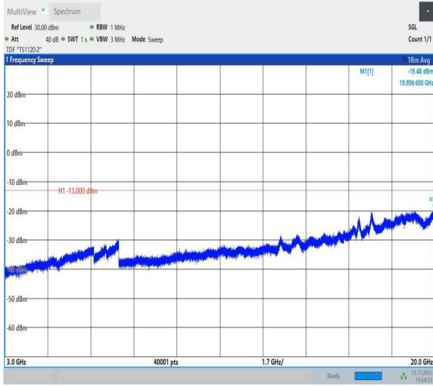
Band4_10MHz_QPSK_20175_1RB#0_3000~20000_3000~20000
