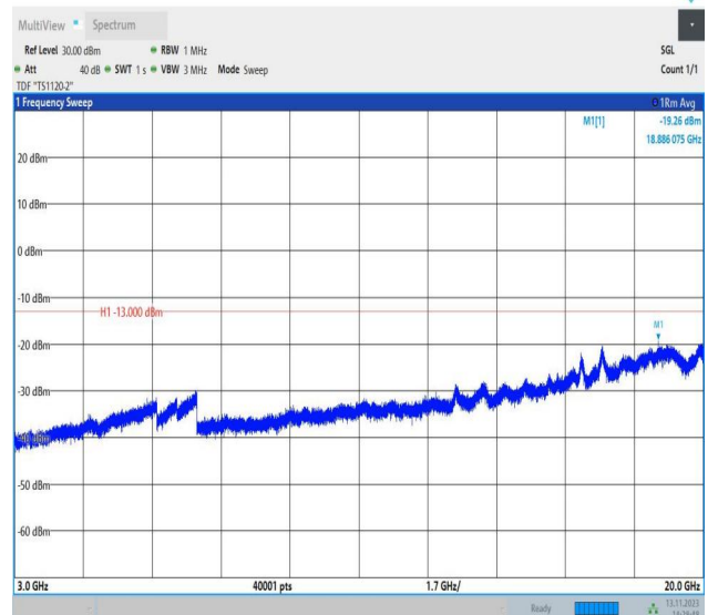
Band4_5MHz_16QAM_20175_1RB#0_3000~20000_3000~2000 00
