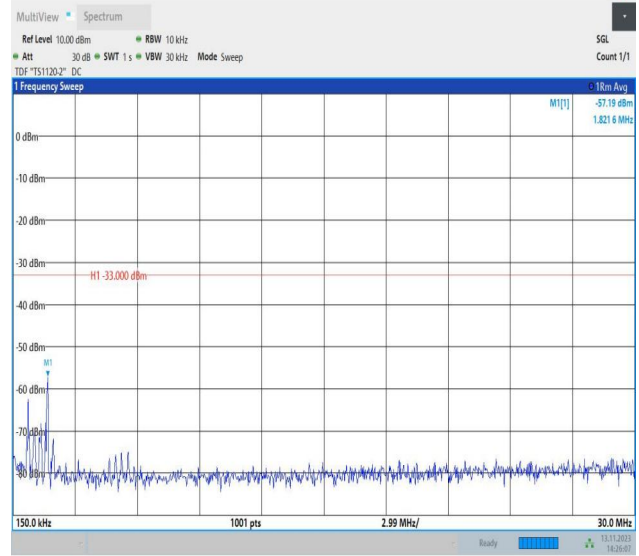
Band4_5MHz_QPSK_19975_1RB#0_0.15~30_0.15~30
