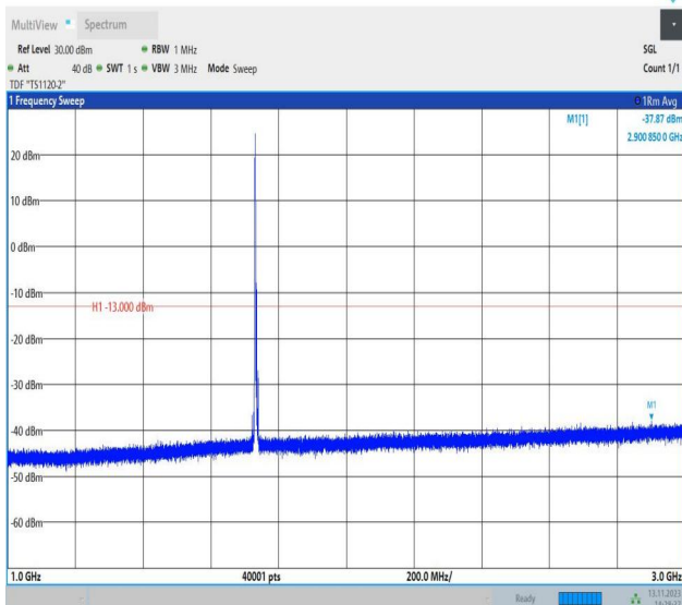
Band4_5MHz_16QAM_20175_1RB#0_1000~3000_1000~3000 0
