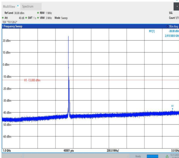
Band4_10MHz_16QAM_20350_1RB#0_1000~3000_1000~30 00
