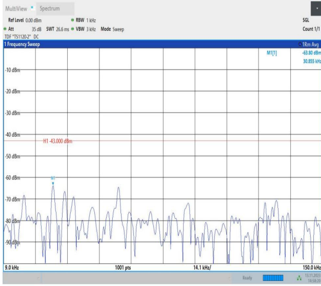
Band4_10MHz_QPSK_20175_1RB#0_0.009~0.15_0.009~0.1
