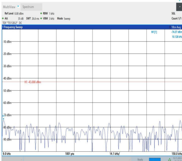
Band4_15MHz_QPSK_20175_1RB#0_0.009~0.15_0.009~0.15
