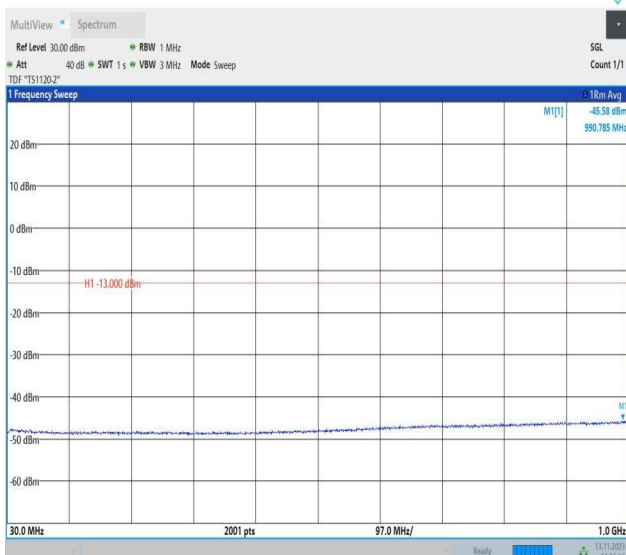
Band4_5MHz_QPSK_19975_1RB#0_30~1000_30~1000
