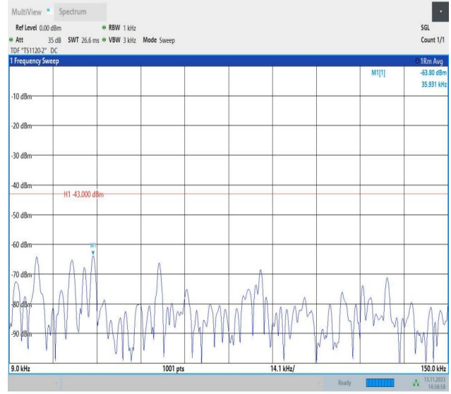
Band4_10MHz_16QAM_20175_1RB#0_0.009~0.15_0.009~0.15
