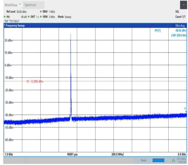
Band4_5MHz_QPSK_20175_1RB#0_1000~3000_1000~3000
