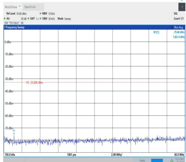
Band4_15MHz_QPSK_20175_1RB#0_0.15~30_0.15~30
