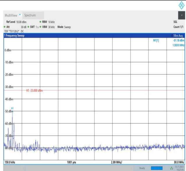
Band4_5MHz_QPSK_20175_1RB#0_0.15~30_0.15~30
