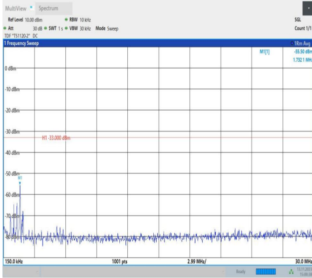
Band4_10MHz_16QAM_20350_1RB#0_0.15~30_0.15~30
