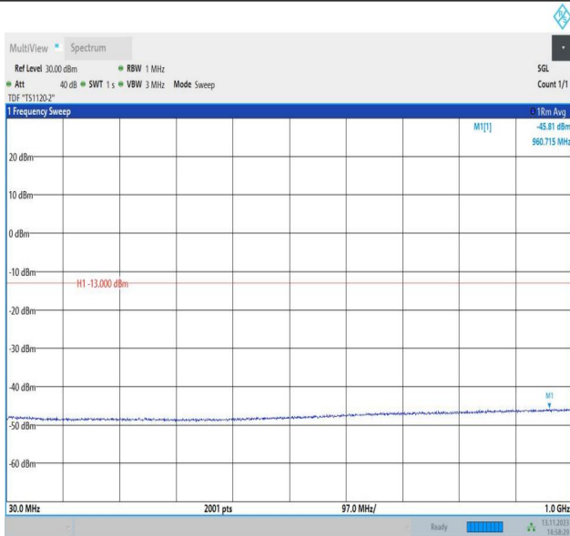
Band4_10MHz_QPSK_20175_1RB#0_30~1000_30~1000
