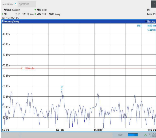
Band4_5MHz_QPSK_19975_1RB#0_0.009~0.15_0.009~0.15
