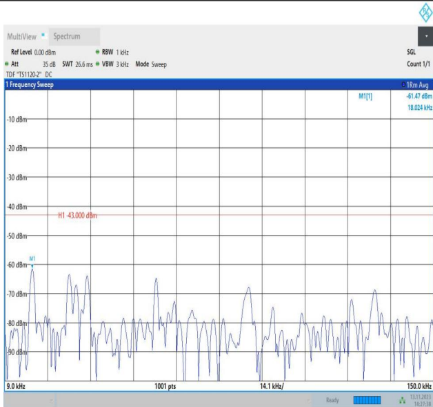
Band4_5MHz_QPSK_20175_1RB#0_0.009~0.15_0.009~0.15
