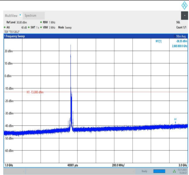
Band4_15MHz_QPSK_20175_1RB#0_1000~3000_1000~3000
