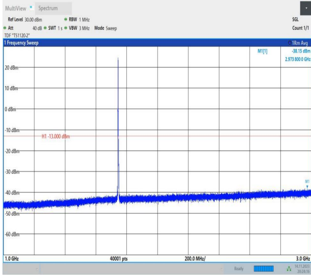
Band66_3MHz_16QAM_132322_1RB#0_1000~3000_1000~3000
