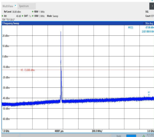
Band66_10MHz_16QAM_132622_1RB#0_1000~3000_1000~3000
