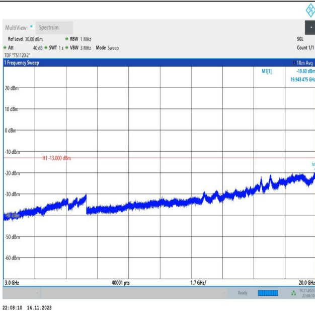
Band66_15MHz_QPSK_132322_1RB#0_3000~20000_3000~20000
