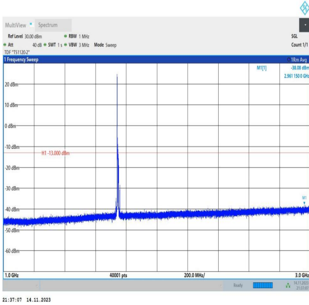
Band66_10MHz_16QAM_132322_1RB#0_1000~3000_1000~3000
