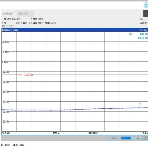
Band66_5MHz_QPSK_131997_1RB#0_30~1000_30~1000
