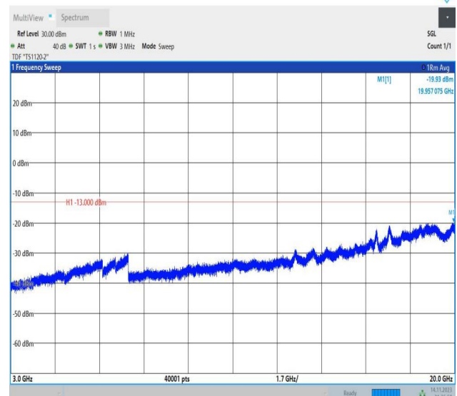
Band66_10MHz_16QAM_132022_1RB#0_3000~20000_3000~20000
