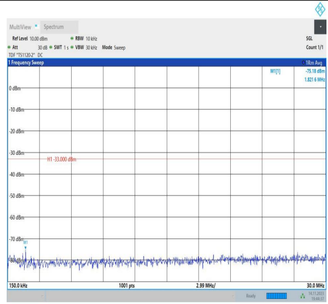
Band66_1.4MHz_QPSK_132665_1RB#0_0.15~30_0.15~30
