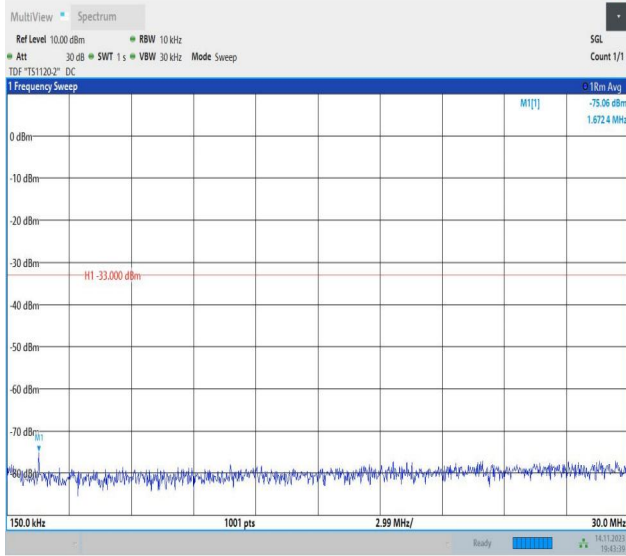
Band66_1.4MHz_16QAM_132322_1RB#0_0.15~30_0.15~30
