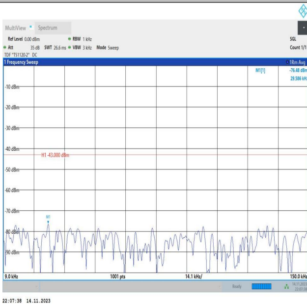
Band66_15MHz_QPSK_132322_1RB#0_0.009~0.15_0.009~0.15
