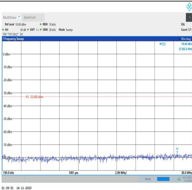
Band66_10MHz_16QAM_132322_1RB#0_0.15~30_0.15~30
