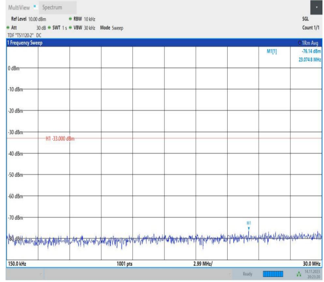
Band66_3MHz_QPSK_132322_1RB#0_0.15~30_0.15~30
