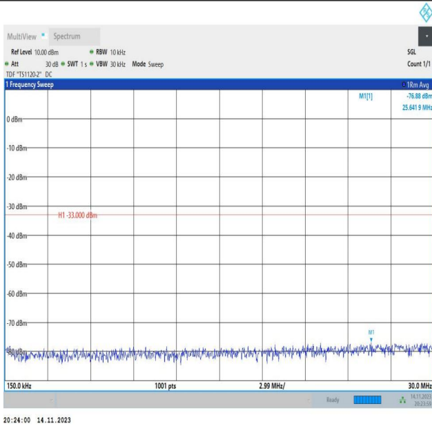
Band66_3MHz_16QAM_132322_1RB#0_0.15~30_0.15~30
