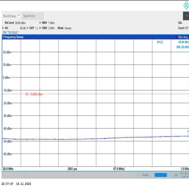
Band66_15MHz_QPSK_132322_1RB#0_30~1000_30~1000
