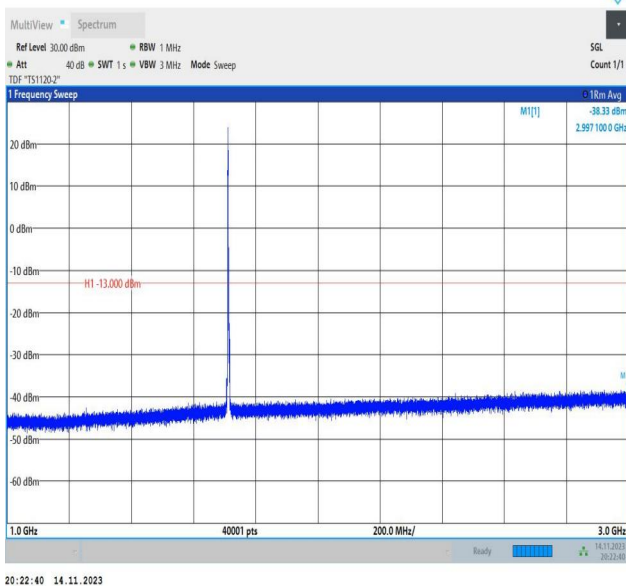
Band66_3MHz_16QAM_131987_1RB#0_1000~3000_1000~3000
