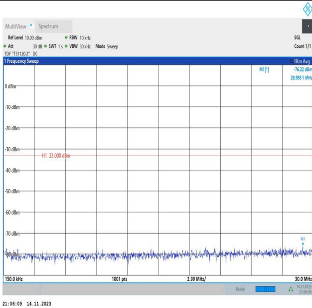
Band66_5MHz_16QAM_132647_1RB#0_0.15~30_0.15~30
