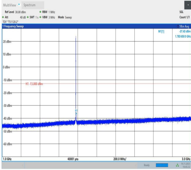
Band66_1.4MHz_16QAM_132665_1RB#0_1000~3000_1000 ~3000
