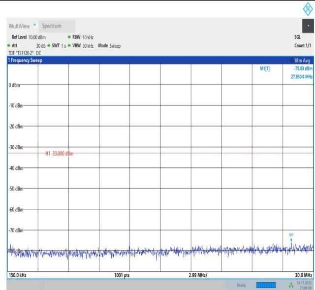
Band66_5MHz_16QAM_131997_1RB#0_3000~20000_3000~20000
