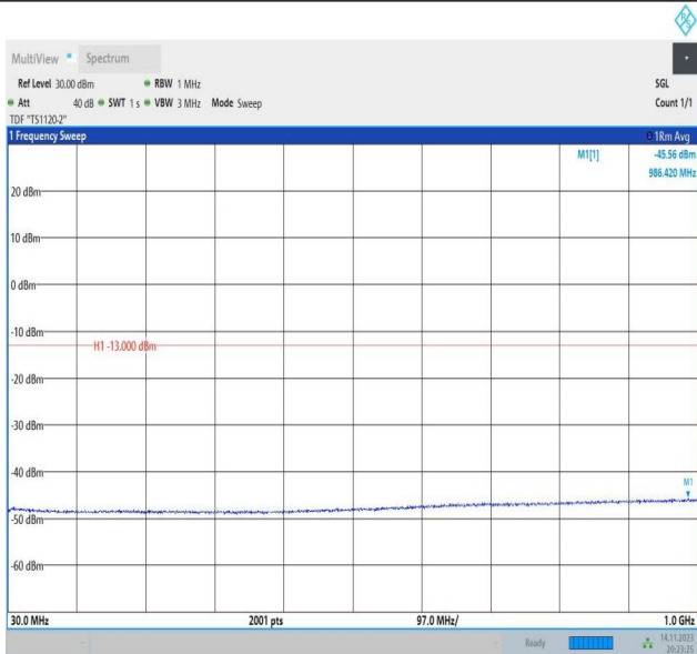
Band66_3MHz_QPSK_132322_1RB#0_30~1000_30~1000
