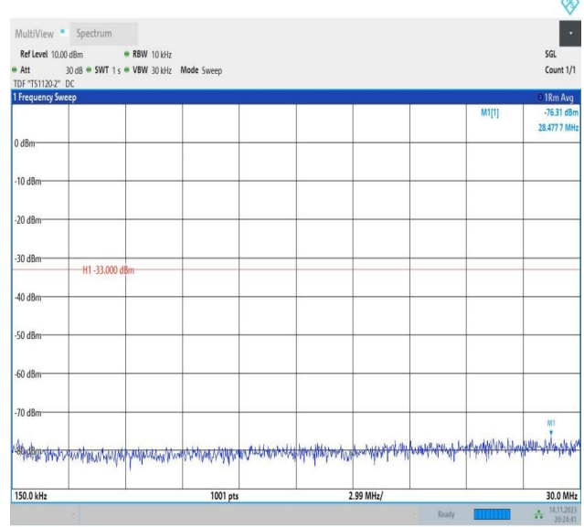
Band66_3MHz_QPSK_132657_1RB#0_0.15~30_0.15~30
