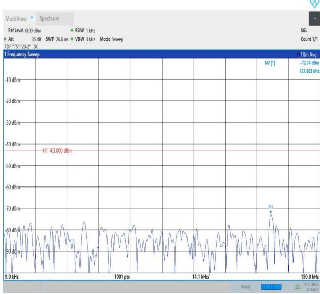
Band66_3MHz_QPSK_132657_1RB#0_0.009~0.15_0.009~0.15
