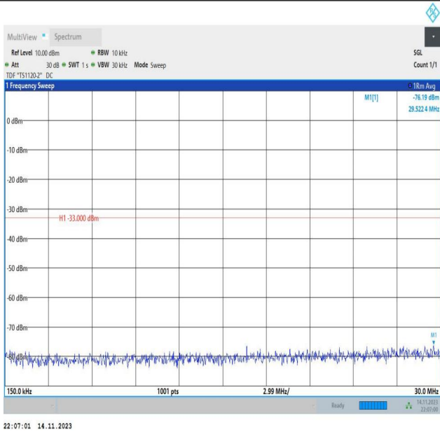
Band66_15MHz_16QAM_132047_1RB#0_0.15~30_0.15~30
