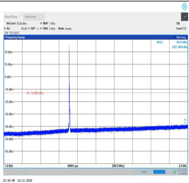
Band66_5MHz_QPSK_131997_1RB#0_1000~3000_1000~300
