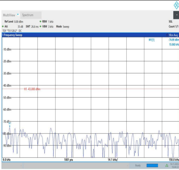
Band66_1.4MHz_QPSK_132665_1RB#0_0.009~0.15_0.009~0.15
