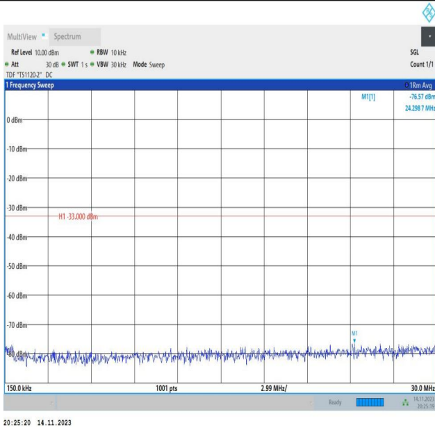
Band66_3MHz_16QAM_132657_1RB#0_0.15~30_0.15~30
