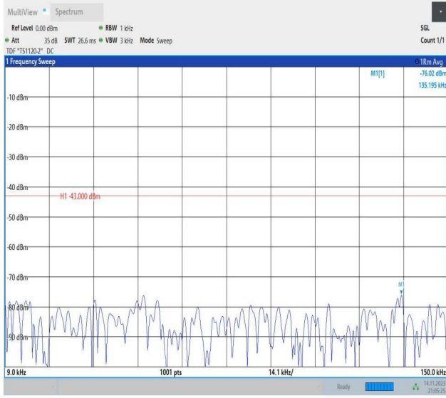
Band66_5MHz_QPSK_132647_1RB#0_0.009~0.15_0.009~0.
