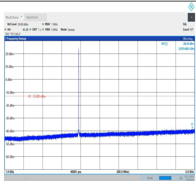
Band66_1.4MHz_QPSK_132665_1RB#0_1000~3000_1000~3000
