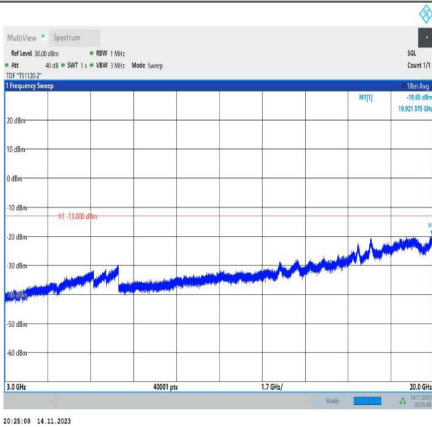
Band66_3MHz_QPSK_132657_1RB#0_3000~20000_3000~2 0000
