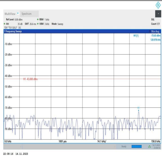
Band66_15MHz_16QAM_132322_1RB#0_0.009~0.15_0.009~0.15
