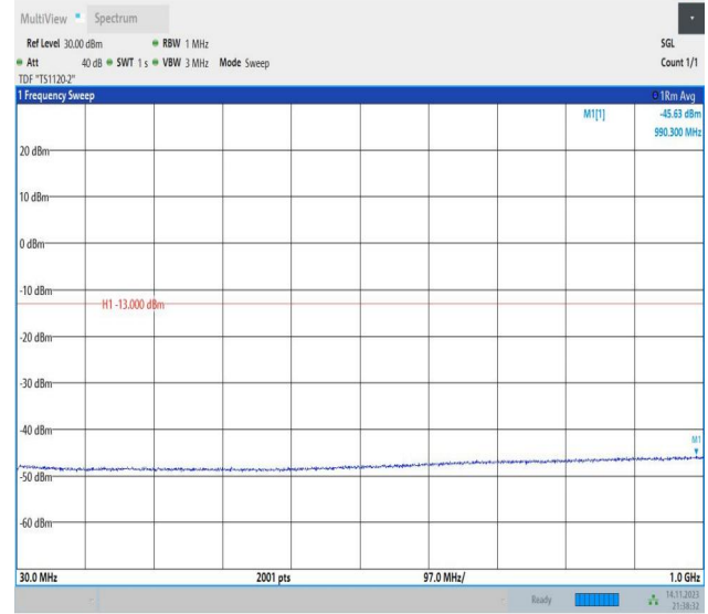
Band66_10MHz_16QAM_132622_1RB#0_30~1000_30~1000
