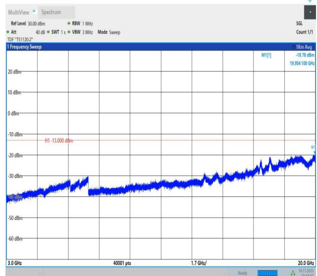
Band66_1.4MHz_16QAM_132322_1RB#0_3000~20000_3000~20000
