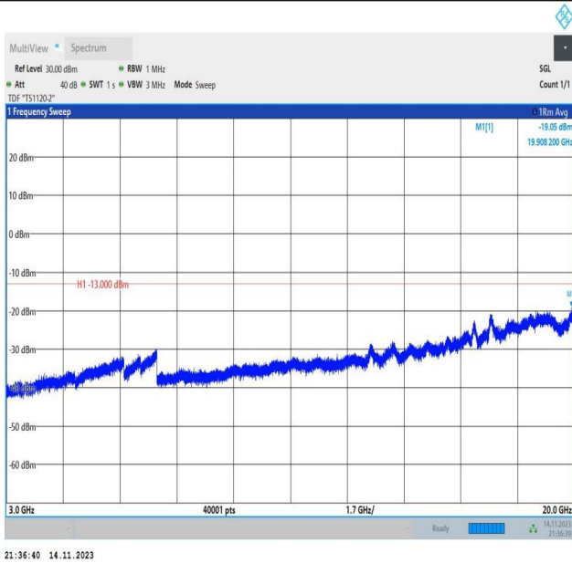
Band66_10MHz_QPSK_132322_1RB#0_3000~20000_3000~20000
