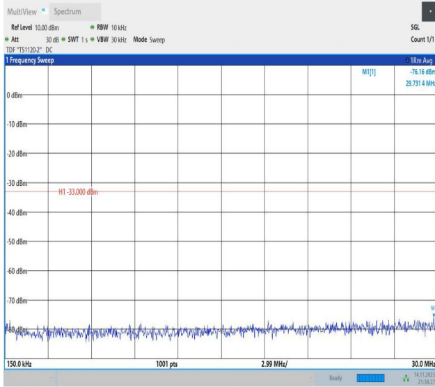
Band66_10MHz_16QAM_132622_1RB#0_0.15~30_0.15~30
