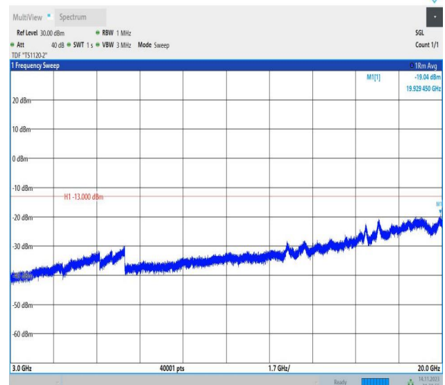
Band66_10MHz_16QAM_132622_1RB#0_3000~20000_3000~20000
