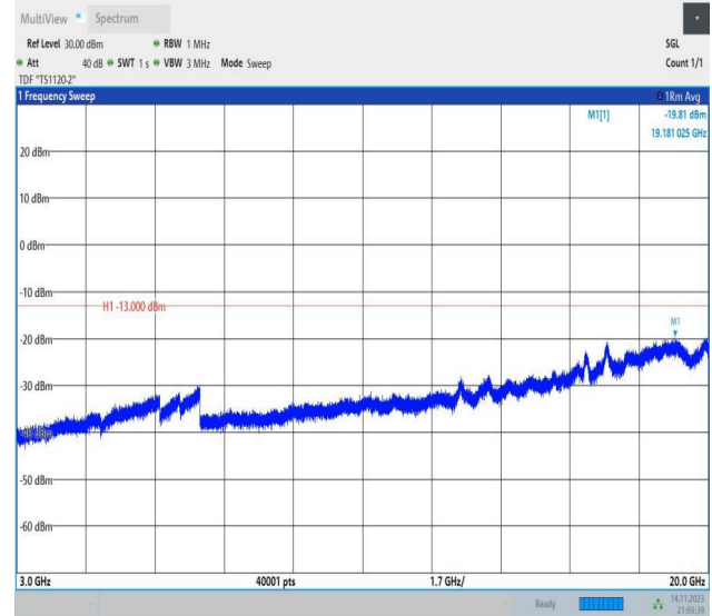
Band66_5MHz_16QAM_131997_1RB#0_3000~20000_3000~20000
