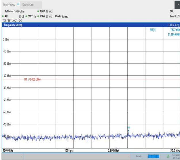
Band66_10MHz_16QAM_132022_1RB#0_0.15~30_0.15~30
