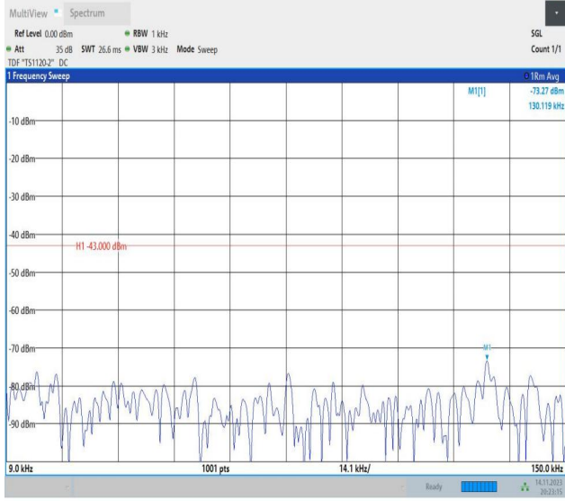
Band66_3MHz_QPSK_132322_1RB#0_0.009~0.15_0.009~0.
