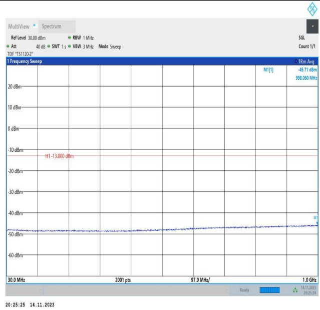
Band66_3MHz_16QAM_132657_1RB#0_30~1000_30~1000
