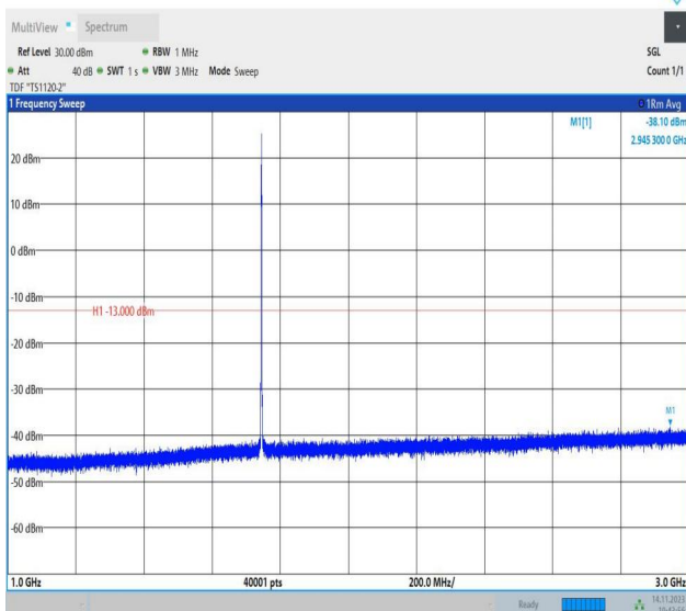
Band66_1.4MHz_16QAM_132322_1RB#0_1000~3000_1000~3000
