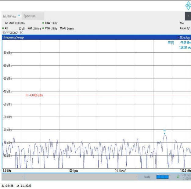
Band66_5MHz_QPSK_131997_1RB#0_0.009~0.15_0.009~0.
