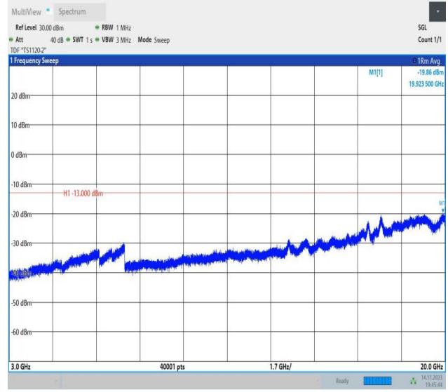
Band66_1.4MHz_16QAM_132665_1RB#0_3000~20000_3000 ~20000
