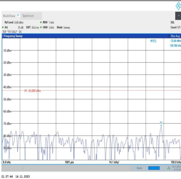
Band66_10MHz_QPSK_132622_1RB#0_0.009~0.15_0.009~0.15
