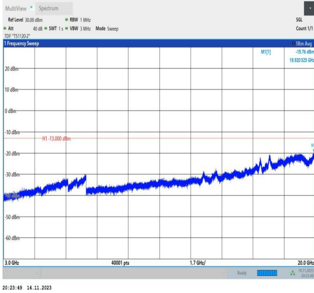
Band66_3MHz_QPSK_132322_1RB#0_3000~20000_3000~20000
