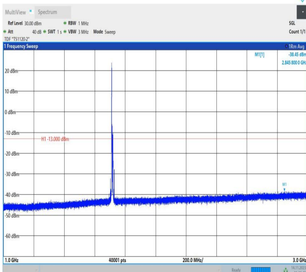
Band66_10MHz_16QAM_132022_1RB#0_1000~3000_1000~3000
