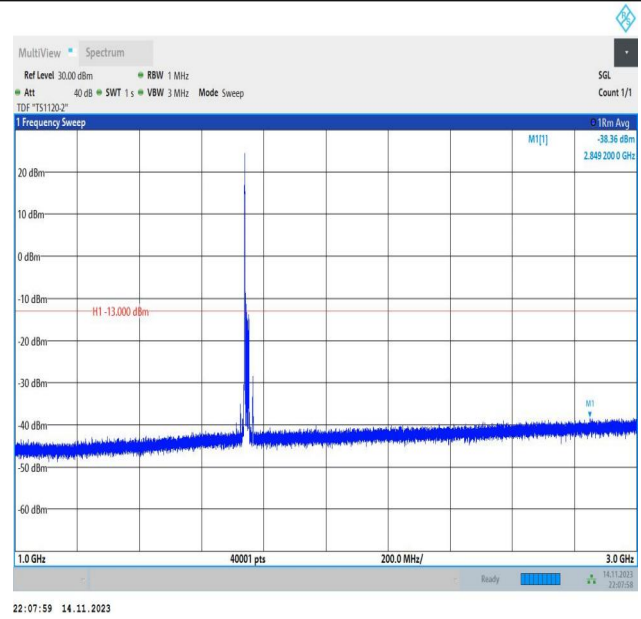
Band66_15MHz_QPSK_132322_1RB#0_1000~3000_1000~3000 00
