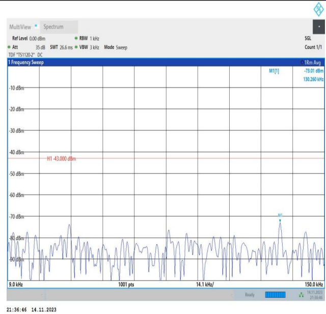
Band66_10MHz_16QAM_132322_1RB#0_0.009~0.15_0.009~0.15
