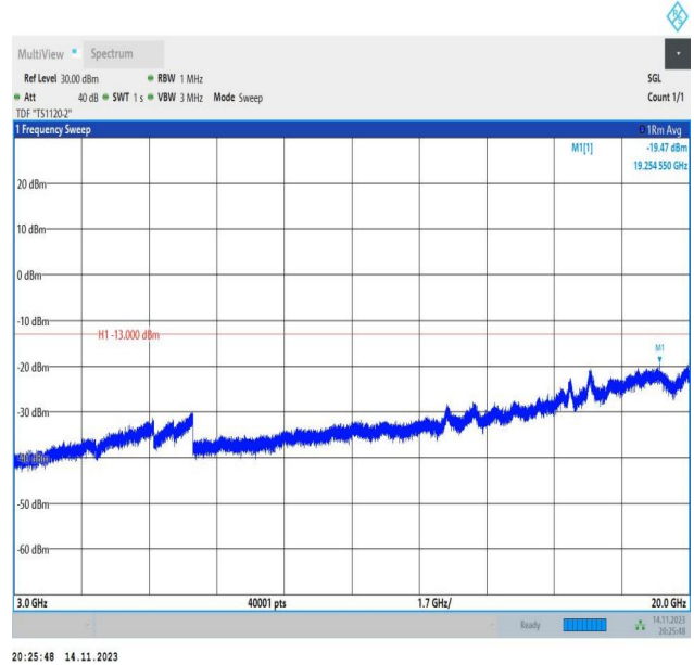
Band66_3MHz_16QAM_132657_1RB#0_3000~20000_3000~20000
