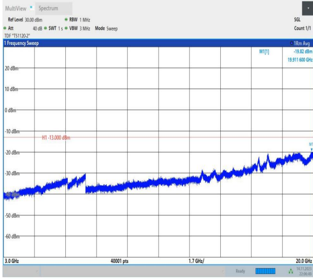
Band66_15MHz_QPSK_132047_1RB#0_3000~20000_3000~20000
