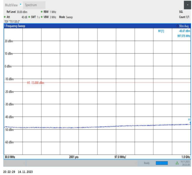
Band66_3MHz_16QAM_131987_1RB#0_30~1000_30~1000
