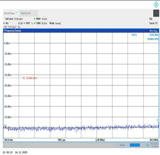
Band66_10MHz_QPSK_132322_1RB#0_0.15~30_0.15~30
