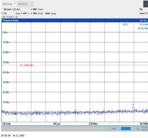
Band66_3MHz_16QAM_131987_1RB#0_0.15~30_0.15~30
