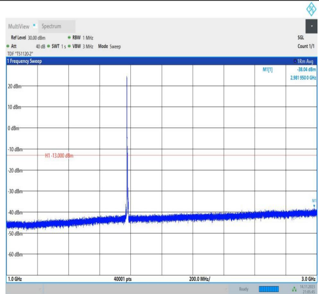
Band66_5MHz_QPSK_132647_1RB#0_1000~3000_1000~300
