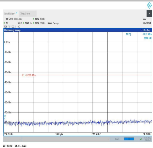
Band66_15MHz_QPSK_132322_1RB#0_0.15~30_0.15~30
