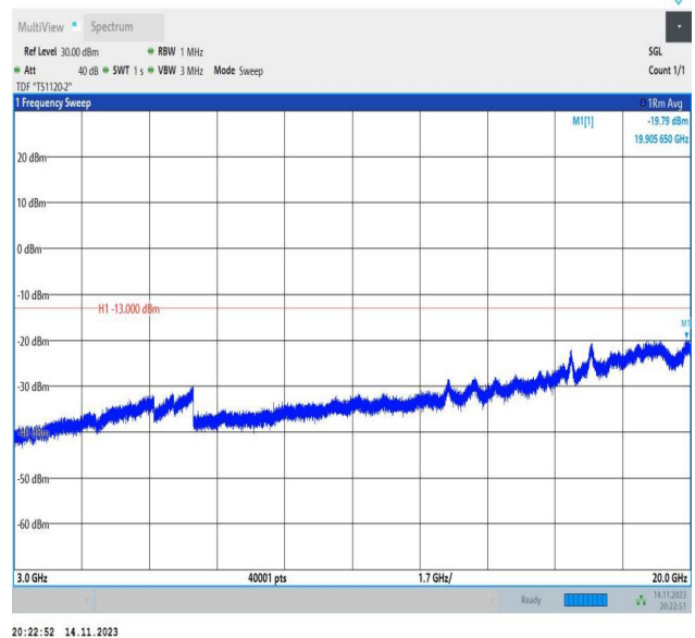
Band66_3MHz_16QAM_131987_1RB#0_3000~20000_3000~20000
