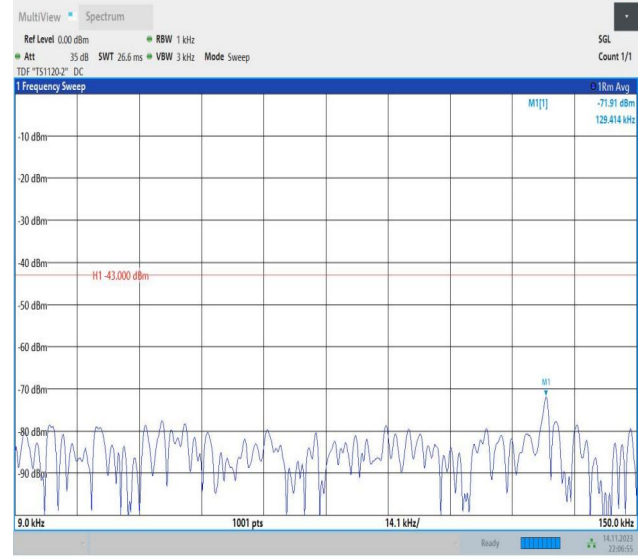
Band66_15MHz_16QAM_132047_1RB#0_0.009~0.15_0.009~0.15
