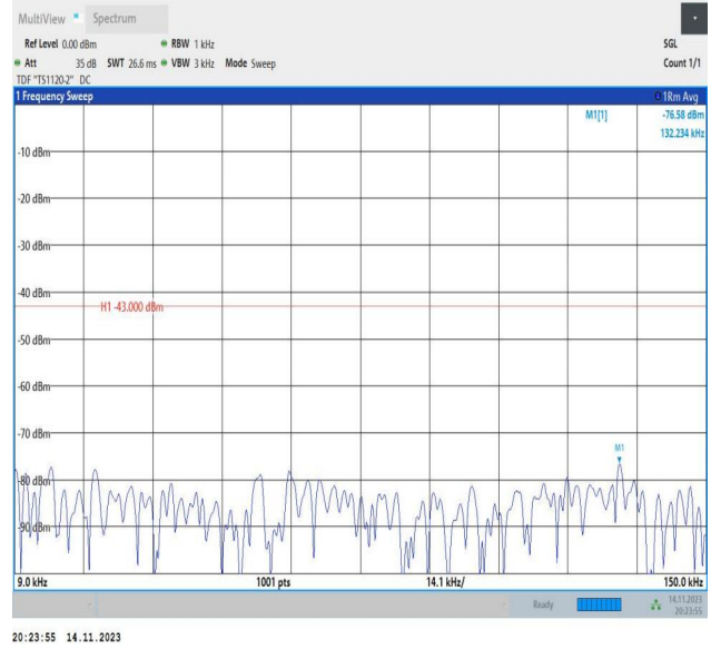
Band66_3MHz_16QAM_132322_1RB#0_0.009~0.15_0.009~0.15
