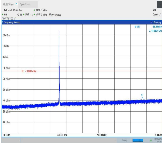
Band66_5MHz_16QAM_131997_1RB#0_1000~3000_1000~3000
