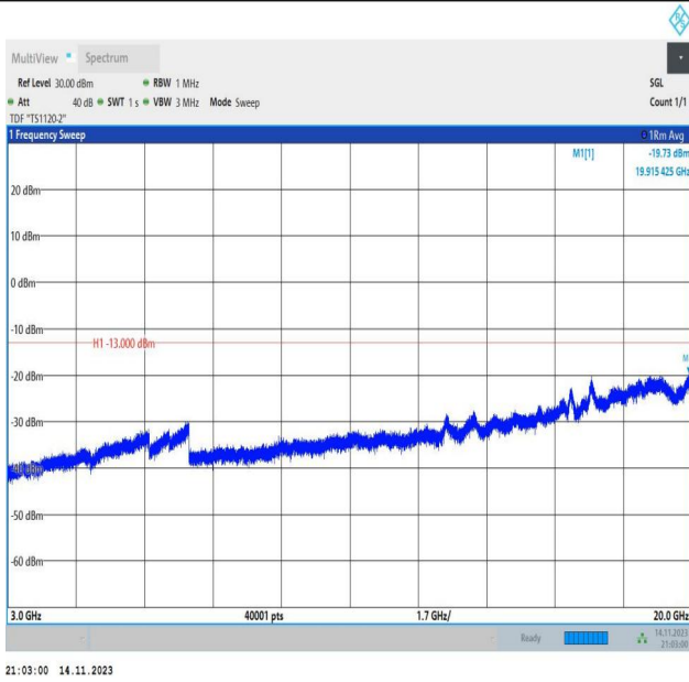
Band66_5MHz_QPSK_131997_1RB#0_3000~20000_3000~20000
