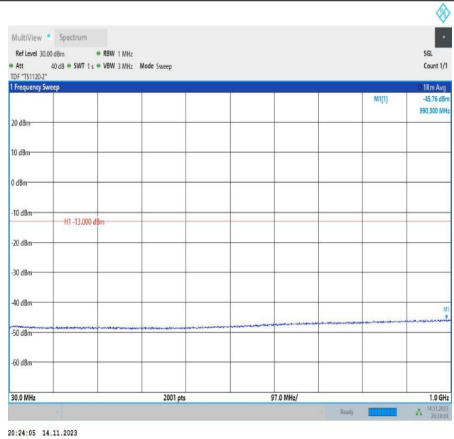
Band66_3MHz_16QAM_132322_1RB#0_30~1000_30~1000
