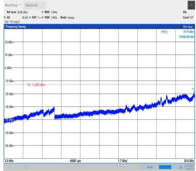
Band66_3MHz_16QAM_132322_1RB#0_3000~20000_3000~20000
