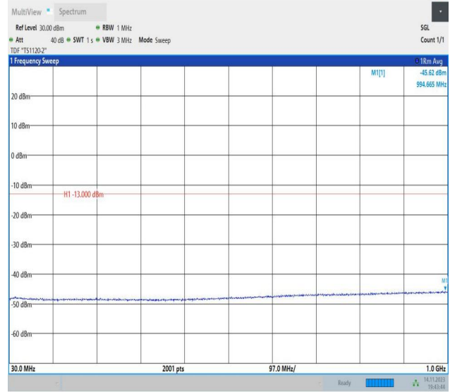
Band66_1.4MHz_16QAM_132322_1RB#0_30~1000_30~1000
