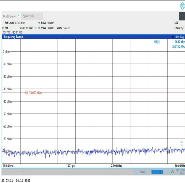
Band66_5MHz_16QAM_131997_1RB#0_0.15~30_0.15~30
