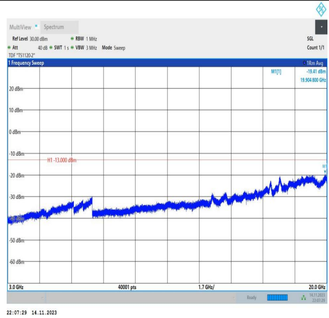
Band66_15MHz_16QAM_132047_1RB#0_3000~20000_3000~20000
