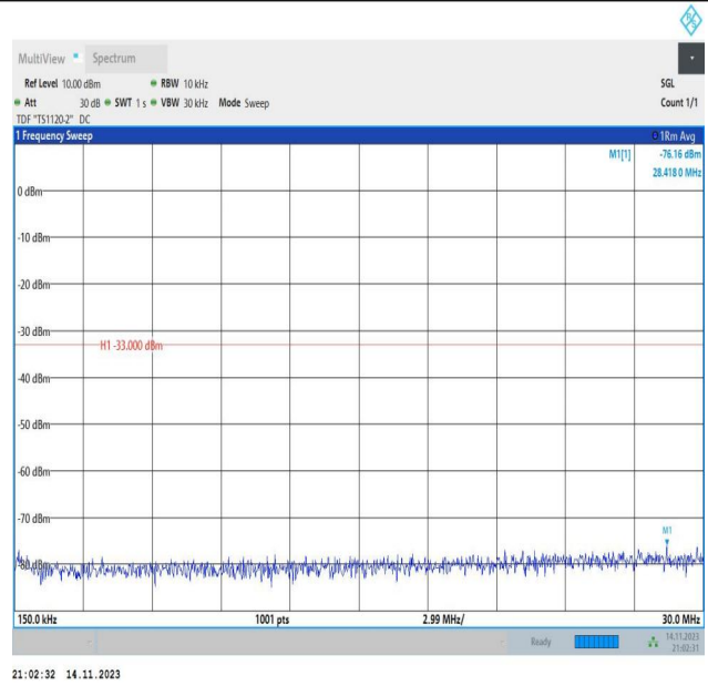
Band66_5MHz_QPSK_131997_1RB#0_0.15~30_0.15~30
