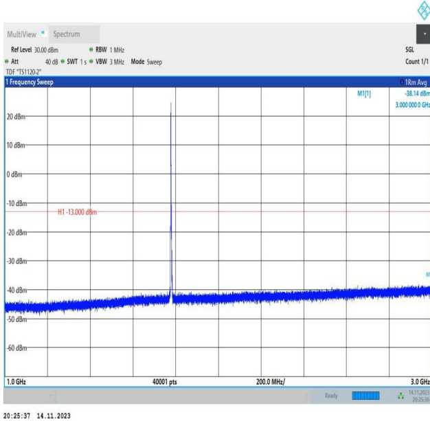
Band66_3MHz_16QAM_132657_1RB#0_1000~3000_1000~3000
