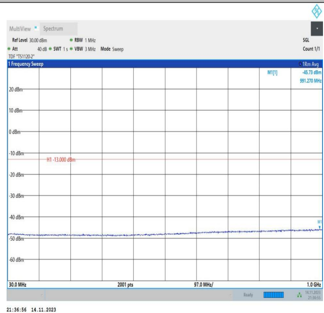
Band66_10MHz_16QAM_132322_1RB#0_30~1000_30~1000
