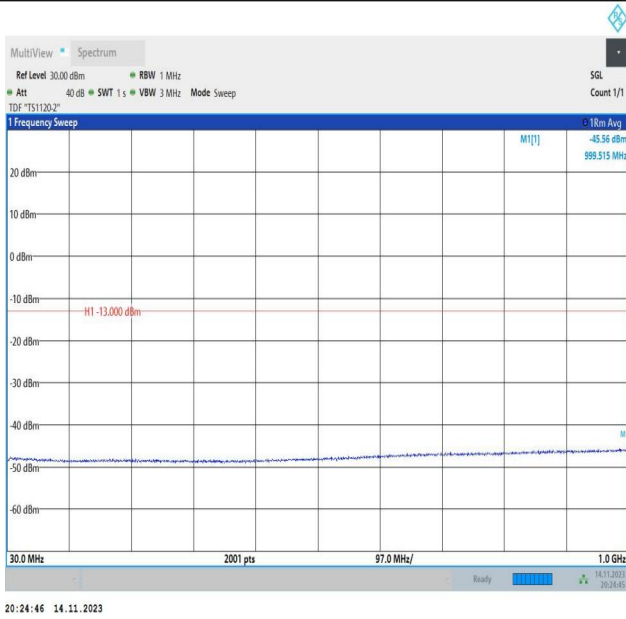
Band66_3MHz_QPSK_132657_1RB#0_30~1000_30~1000
