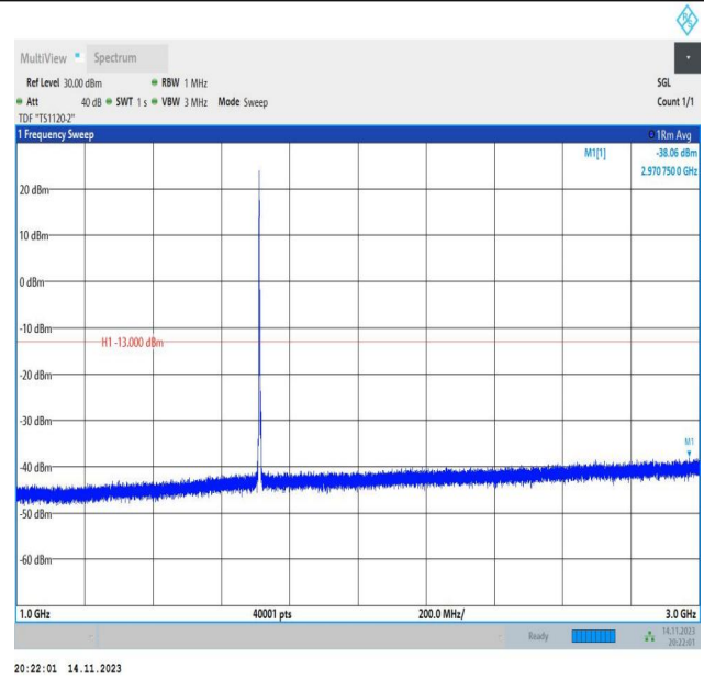
Band66_3MHz_QPSK_131987_1RB#0_1000~3000_1000~300 0
