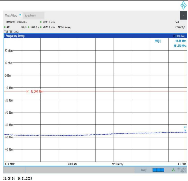
Band66_5MHz_16QAM_132647_1RB#0_30~1000_30~1000
