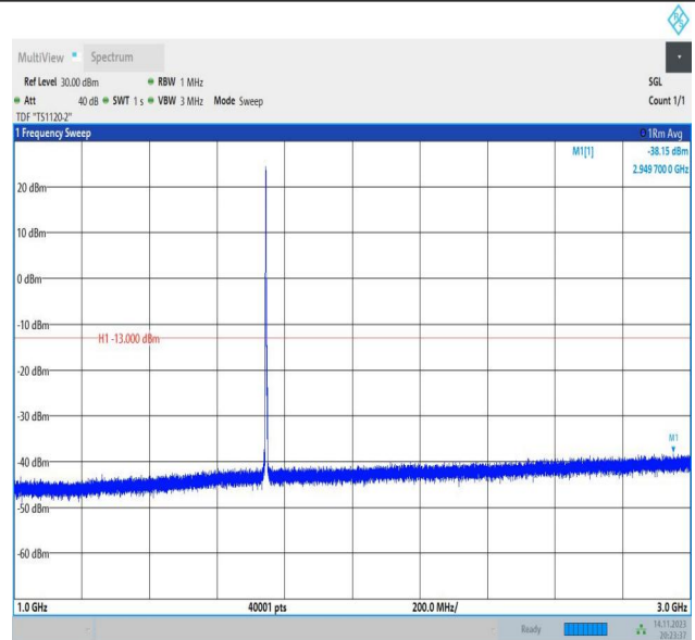
Band66_3MHz_QPSK_132322_1RB#0_1000~3000_1000~300
