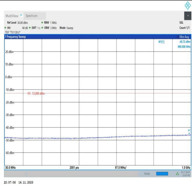
Band66_15MHz_16QAM_132047_1RB#0_30~1000_30~1000
