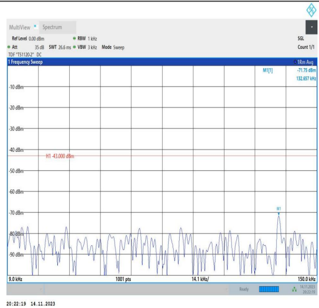
Band66_3MHz_16QAM_131987_1RB#0_0.009~0.15_0.009~0. 15
