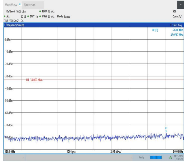
Band66_5MHz_QPSK_132647_1RB#0_0.15~30_0.15~30
