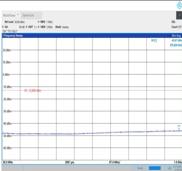
Band66_5MHz_QPSK_132647_1RB#0_30~1000_30~1000
