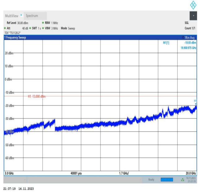
Band66_10MHz_16QAM_132322_1RB#0_3000~20000_3000~20000
