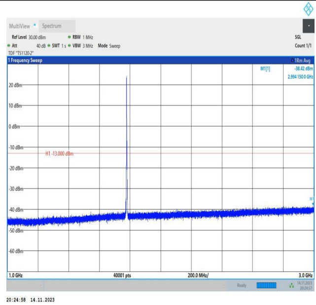
Band66_3MHz_QPSK_132657_1RB#0_1000~3000_1000~300 0
