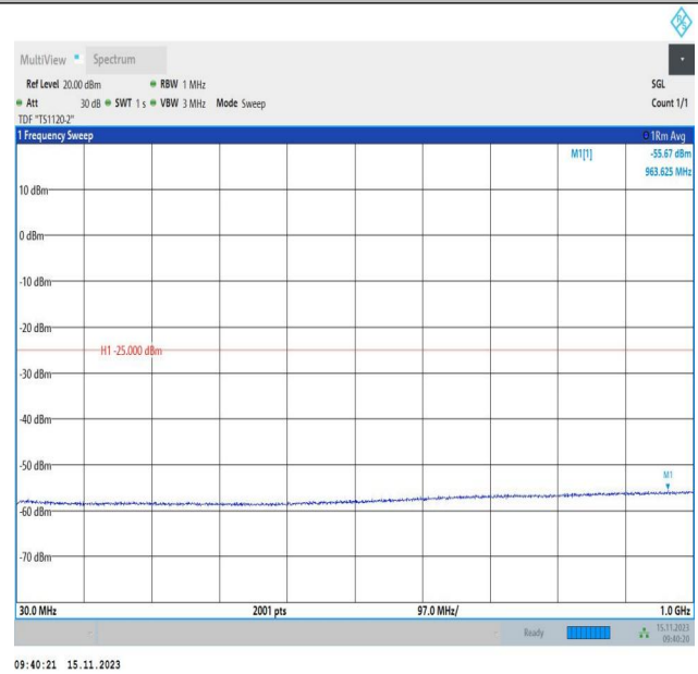
Band7_10MHz_16QAM_21100_1RB#0_30~1000_30~1000
