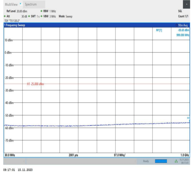
Band7_5MHz_16QAM_21100_1RB#0_30~1000_30~1000
