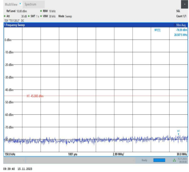
Band7_10MHz_QPSK_21100_1RB#0_0.15~30_0.15~30
