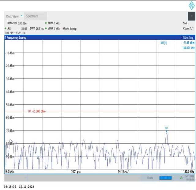
Band7_5MHz_16QAM_21425_1RB#0_0.009~0.15_0.009~0.15
