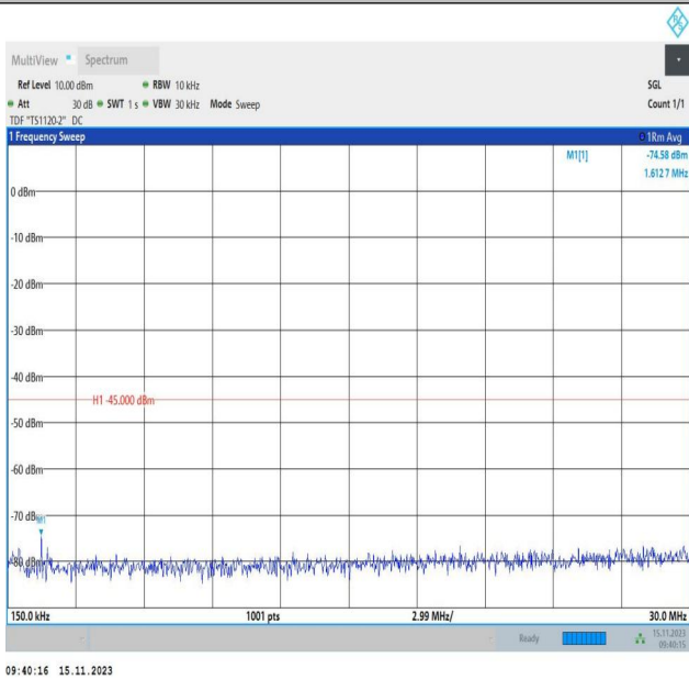
Band7_10MHz_16QAM_21100_1RB#0_0.15~30_0.15~30
