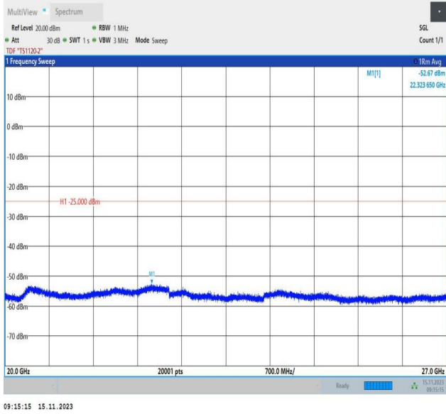
Band7_5MHz_QPSK_20775_1RB#0_20000~27000_20000~27000
