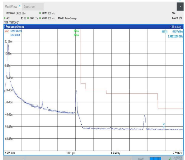
Band7_15MHz_64QAM_21375_1RB#0
