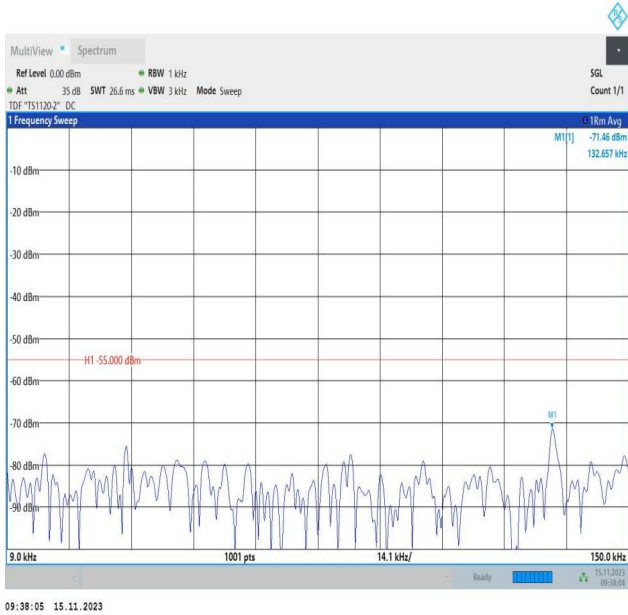
Band7_10MHz_QPSK_20800_1RB#0_0.009~0.15_0.009~0.15
