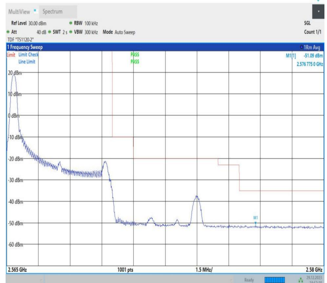
Band7_5MHz_64QAM_21425_1RB#0
