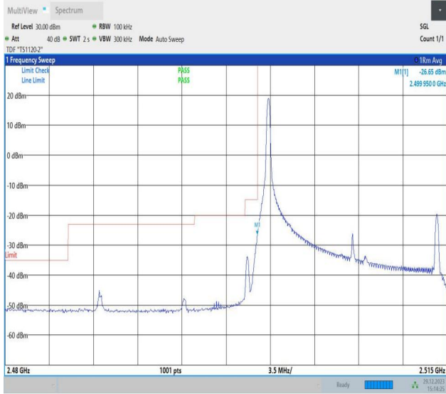
Band7_15MHz_64QAM_20825_1RB#0
