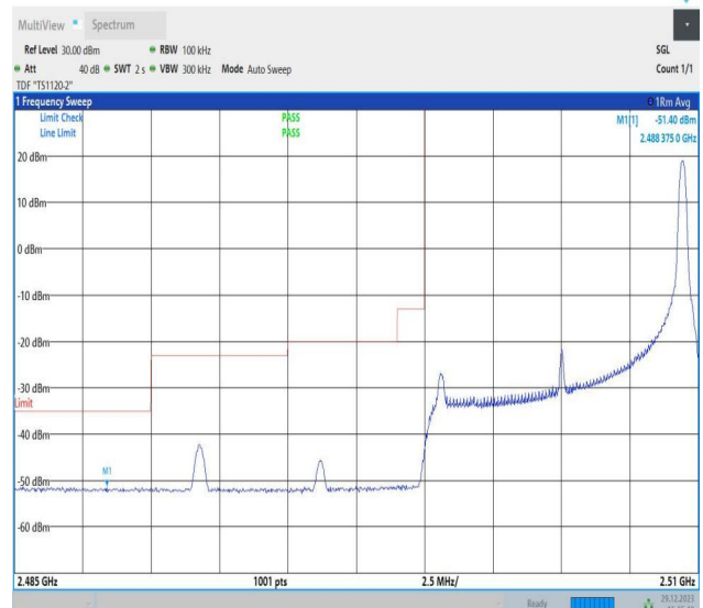
Band7_10MHz_64QAM_20800_1RB#49
