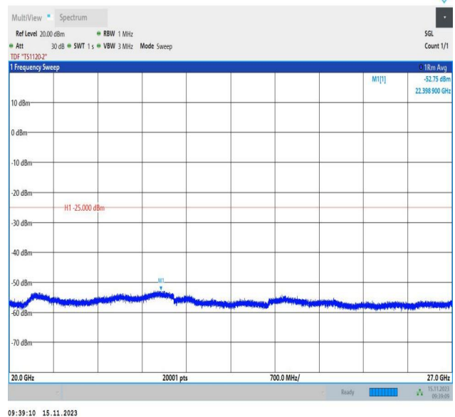
Band7_10MHz_16QAM_20800_1RB#0_20000~27000_20000~27000
