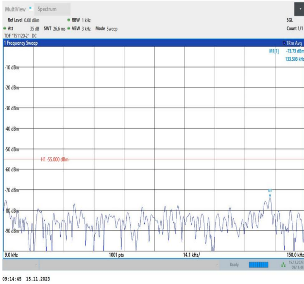
Band7_5MHz_QPSK_20775_1RB#0_0.009~0.15_0.009~0.15
