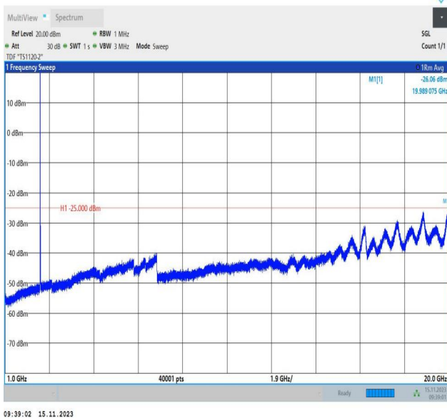
Band7_10MHz_16QAM_20800_1RB#0_1000~20000_1000~20000
