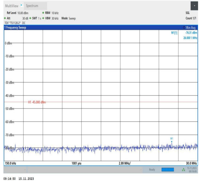
Band7_5MHz_QPSK_20775_1RB#0_0.15~30_0.15~30
