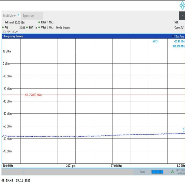
Band7_10MHz_QPSK_21100_1RB#0_30~1000_30~1000
