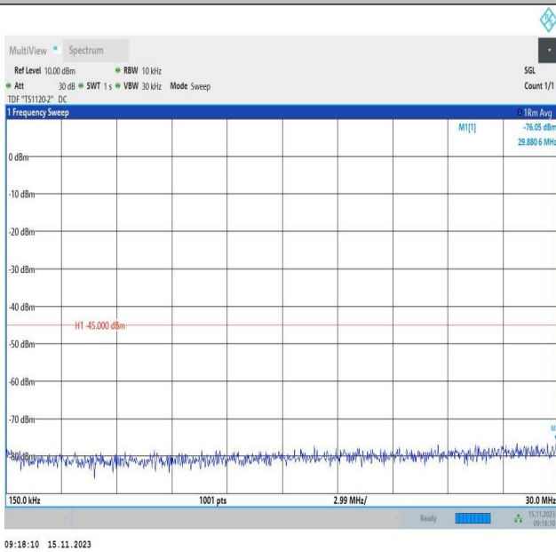
Band7_5MHz_16QAM_21425_1RB#0_0.15~30_0.15~30
