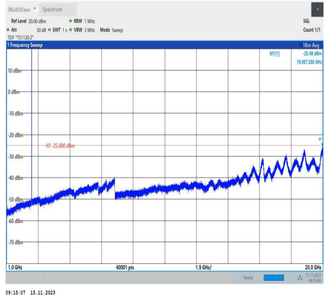
Band7_5MHz_QPSK_20775_1RB#0_1000~20000_1000~20000
