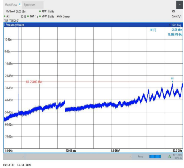
Band7_5MHz_QPSK_21100_1RB#0_1000~20000_1000~2000 0
