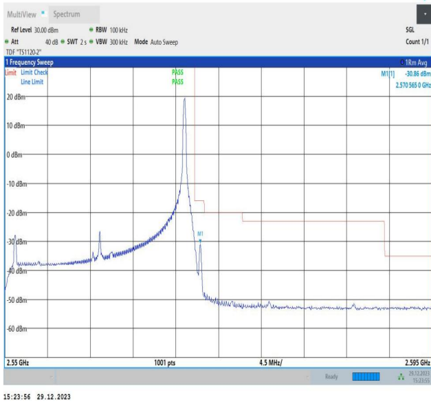
Band7_20MHz_64QAM_21350_1RB#99
