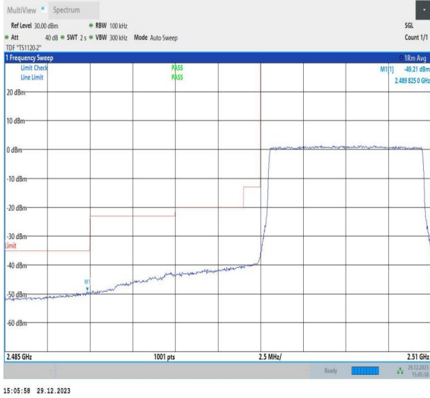
Band7_10MHz_64QAM_20800_50RB#0
