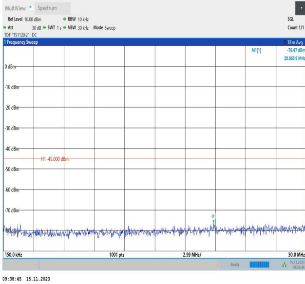
Band7_10MHz_16QAM_20800_1RB#0_0.15~30_0.15~30
