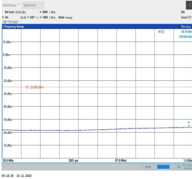
Band7_5MHz_QPSK_21100_1RB#0_30~1000_30~1000
