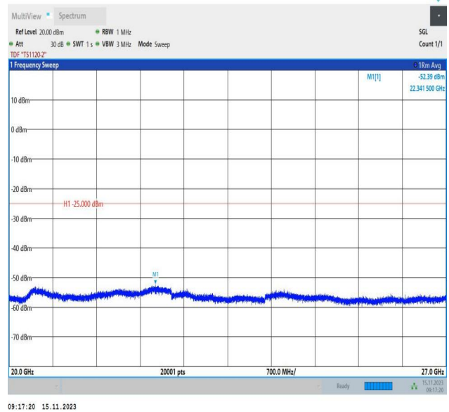
Band7_5MHz_16QAM_21100_1RB#0_20000~27000_20000~27000
