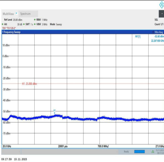
Band7_5MHz_QPSK_21425_1RB#0_20000~27000_20000~27000
