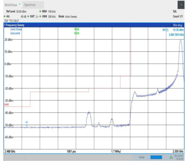
Band7_5MHz_64QAM_20775_1RB#24
