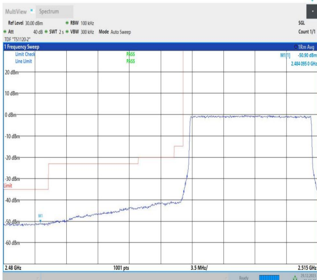
Band7_15MHz_64QAM_20825_75RB#0
