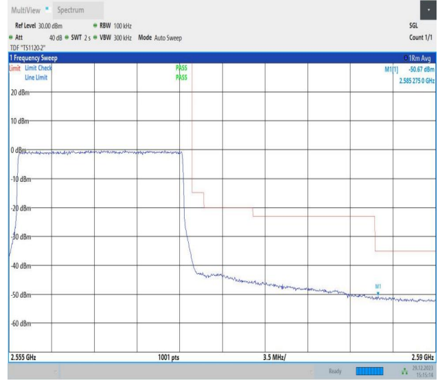
Band7_15MHz_64QAM_21375_75RB#0
