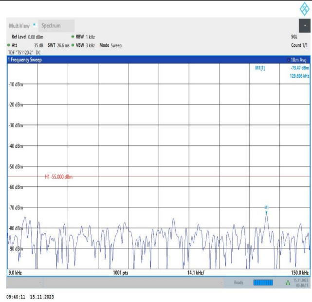
Band7_10MHz_16QAM_21100_1RB#0_0.009~0.15_0.009~0.1
