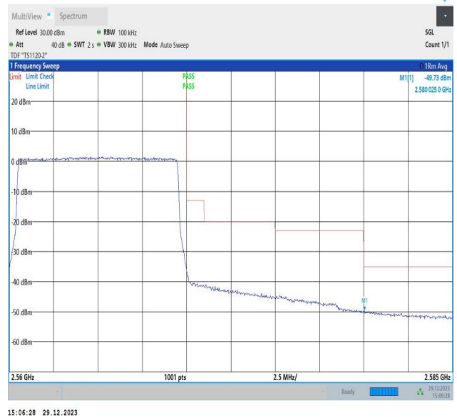
Band7_10MHz_64QAM_21400_50RB#0
