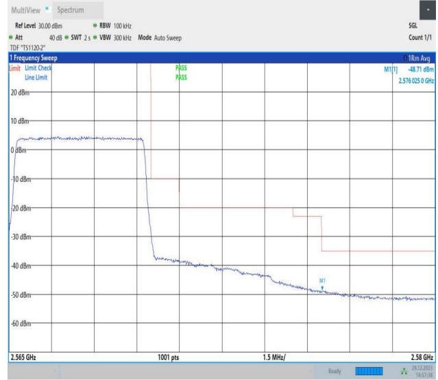
Band7_5MHz_64QAM_21425_25RB#0
