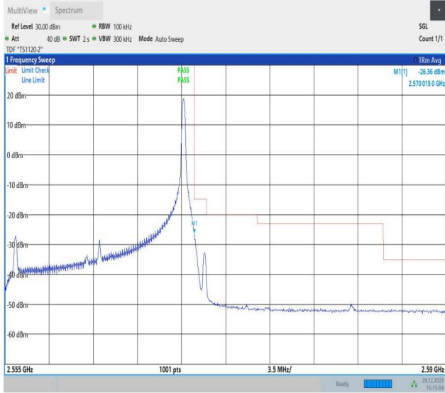
Band7_15MHz_64QAM_21375_1RB#74
