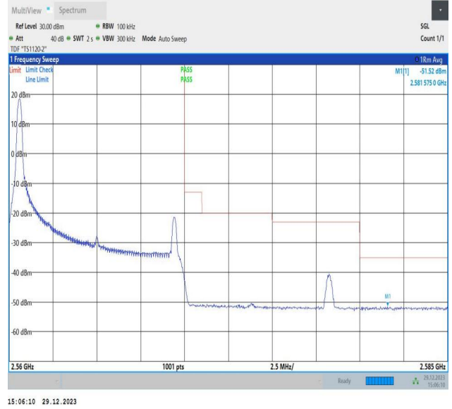
Band7_10MHz_64QAM_21400_1RB#0
