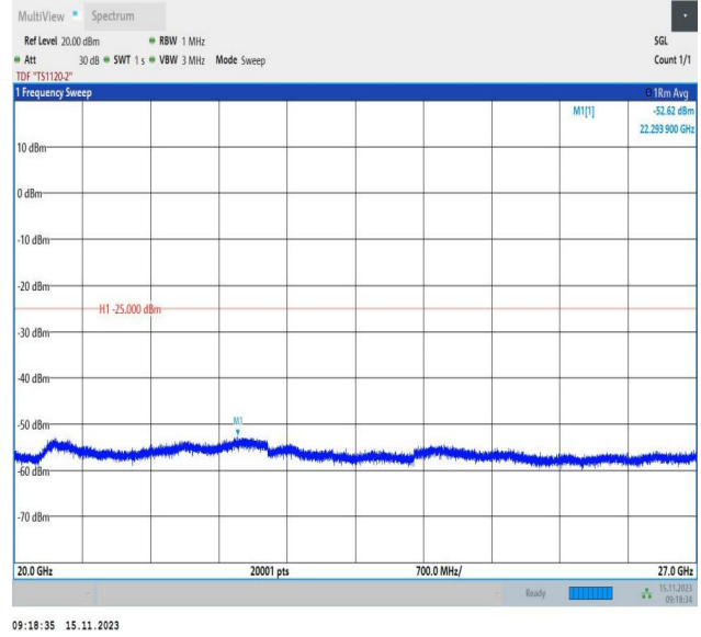
Band7_5MHz_16QAM_21425_1RB#0_20000~27000_20000~27000
