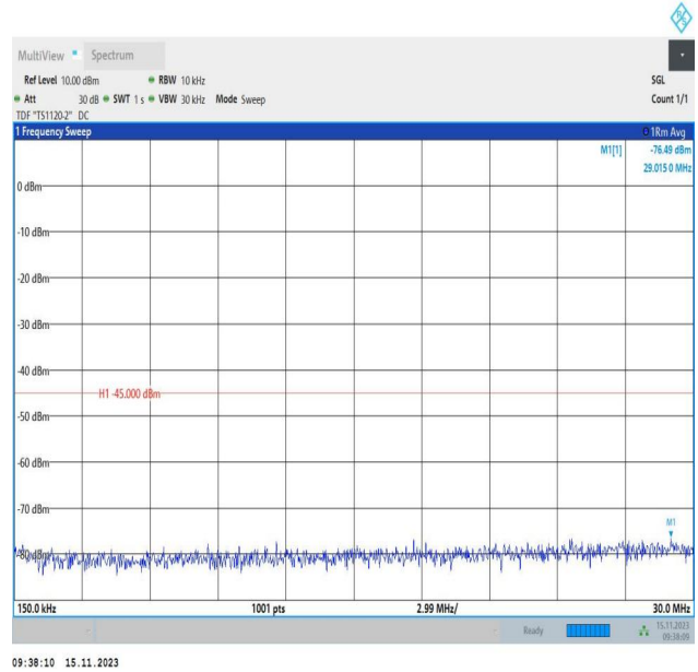
Band7_10MHz_QPSK_20800_1RB#0_0.15~30_0.15~30
