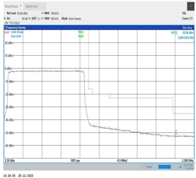
Band7_20MHz_64QAM_21350_100RB#0
