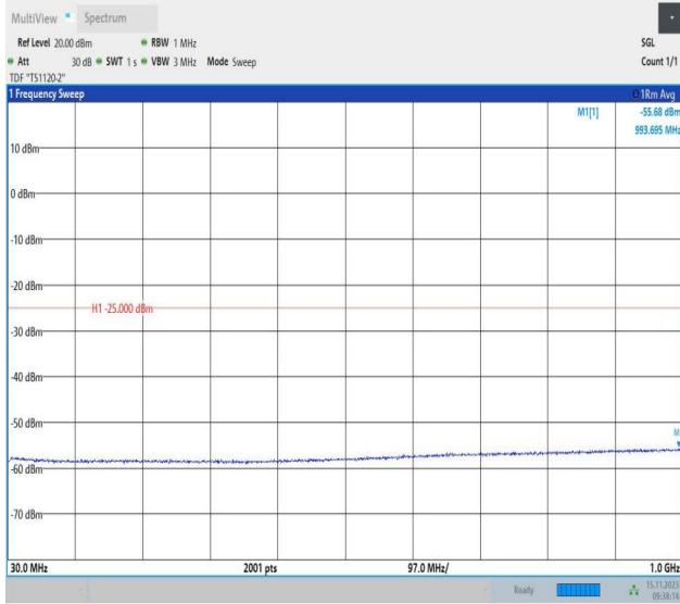
Band7_10MHz_QPSK_20800_1RB#0_30~1000_30~1000
