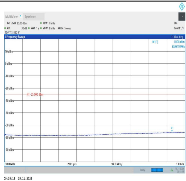
Band7_5MHz_16QAM_21425_1RB#0_30~1000_30~1000
