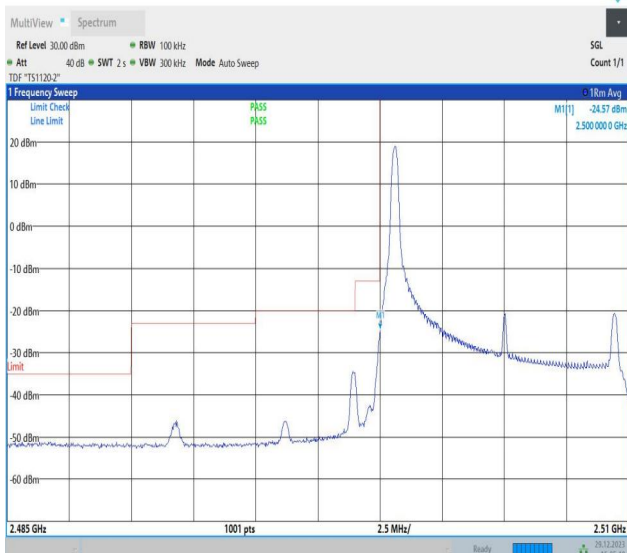
Band7_10MHz_64QAM_20800_1RB#0
