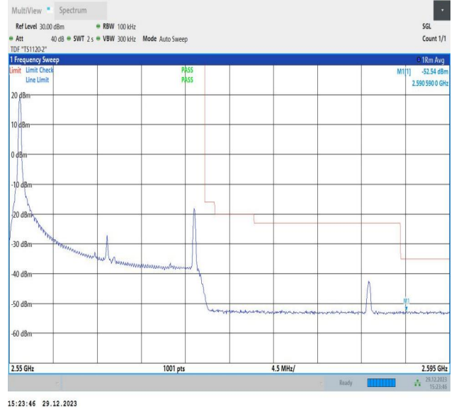
Band7_20MHz_64QAM_21350_1RB#0
