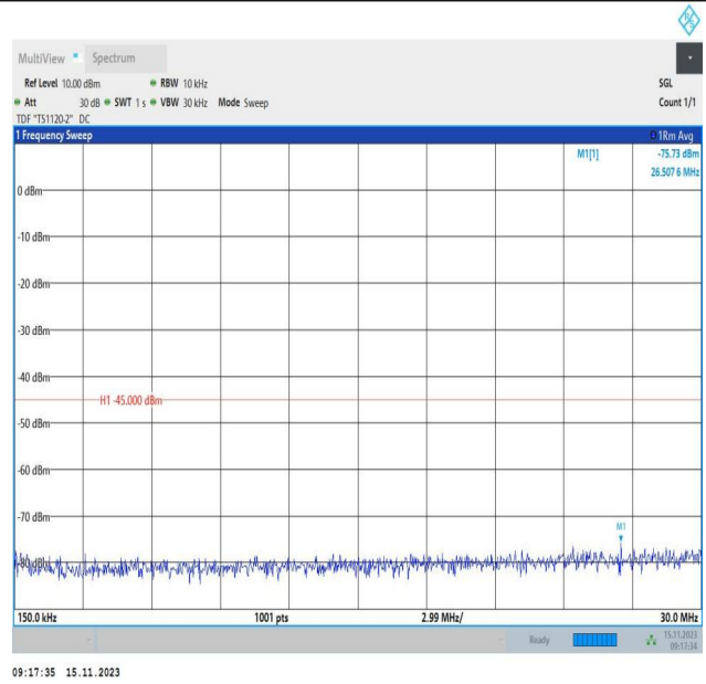
Band7_5MHz_QPSK_21425_1RB#0_0.15~30_0.15~30
