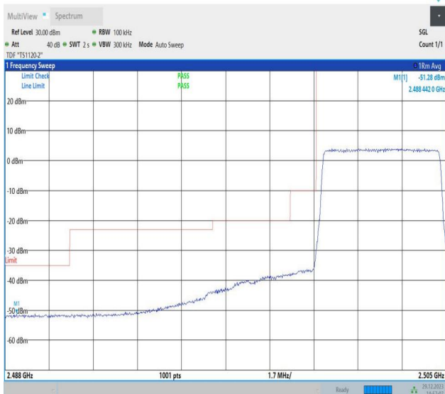
Band7_5MHz_64QAM_20775_25RB#0
