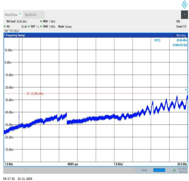
Band7_5MHz_QPSK_21425_1RB#0_1000~20000_1000~2000
