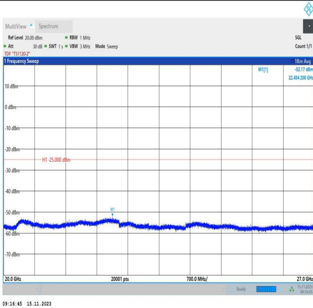
Band7_5MHz_QPSK_21100_1RB#0_20000~27000_20000~27000
