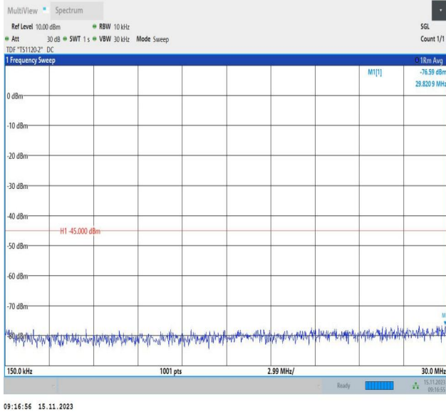
Band7_5MHz_16QAM_21100_1RB#0_0.15~30_0.15~30
