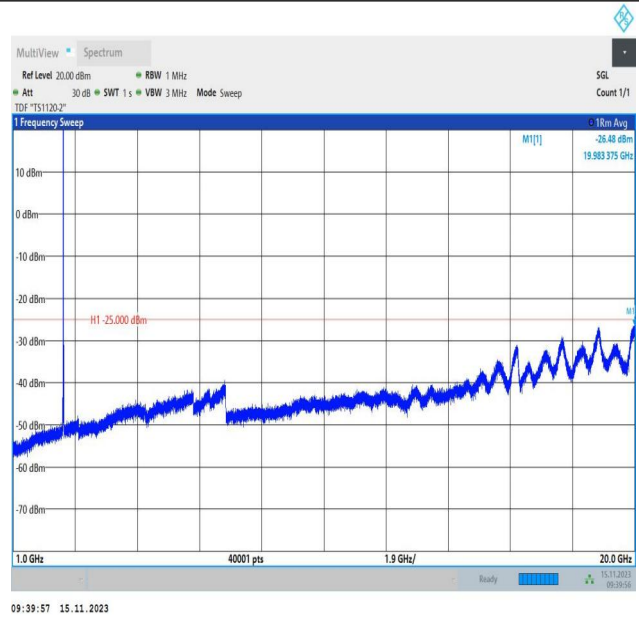
Band7_10MHz_QPSK_21100_1RB#0_1000~20000_1000~200
