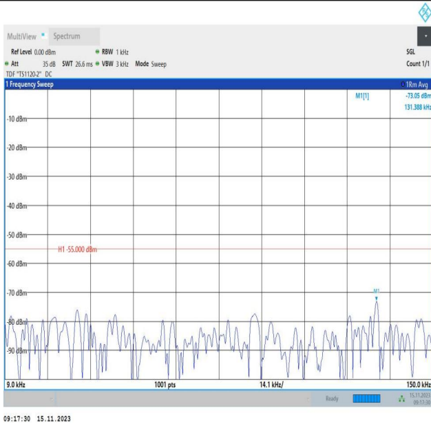
Band7_5MHz_QPSK_21425_1RB#0_0.009~0.15_0.009~0.15
