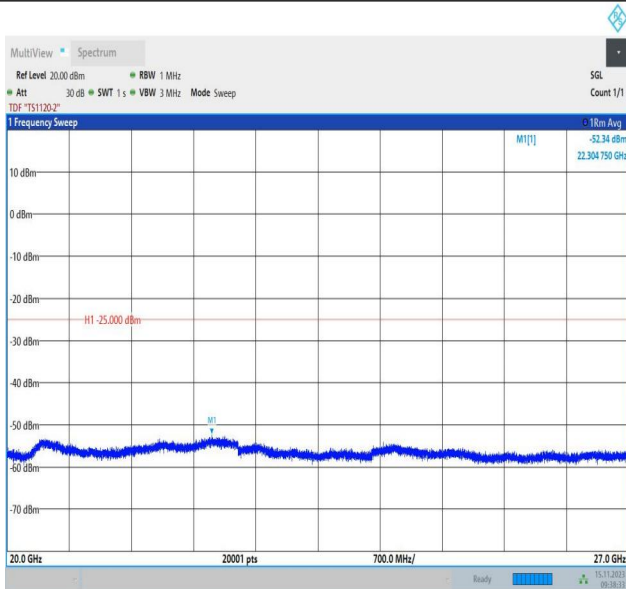
Band7_10MHz_QPSK_20800_1RB#0_20000~27000_20000~ 27000
