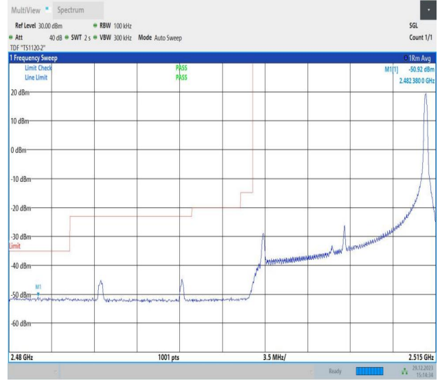
Band7_15MHz_64QAM_20825_1RB#74
