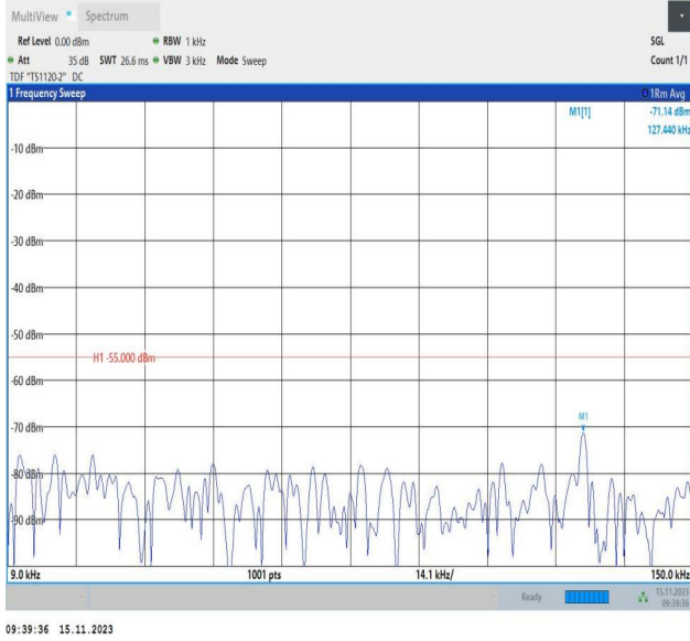
Band7_10MHz_QPSK_21100_1RB#0_0.009~0.15_0.009~0.1
