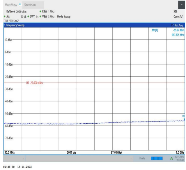
Band7_10MHz_16QAM_20800_1RB#0_30~1000_30~1000
