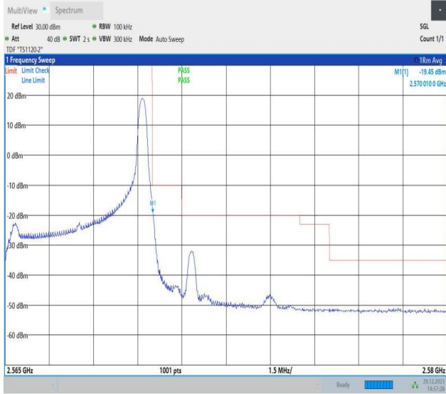
Band7_5MHz_64QAM_21425_1RB#24
