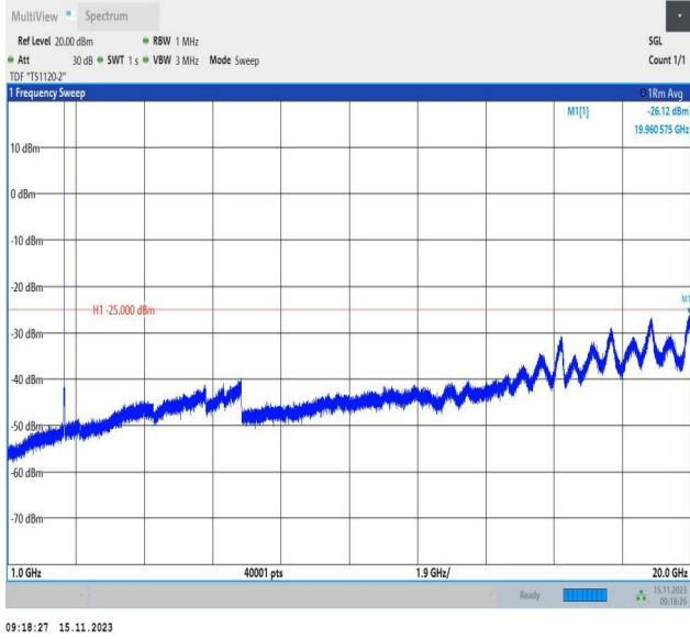
Band7_5MHz_16QAM_21425_1RB#0_1000~20000_1000~20000
