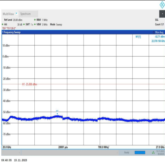
Band7_10MHz_QPSK_21100_1RB#0_20000~27000_20000~27000
