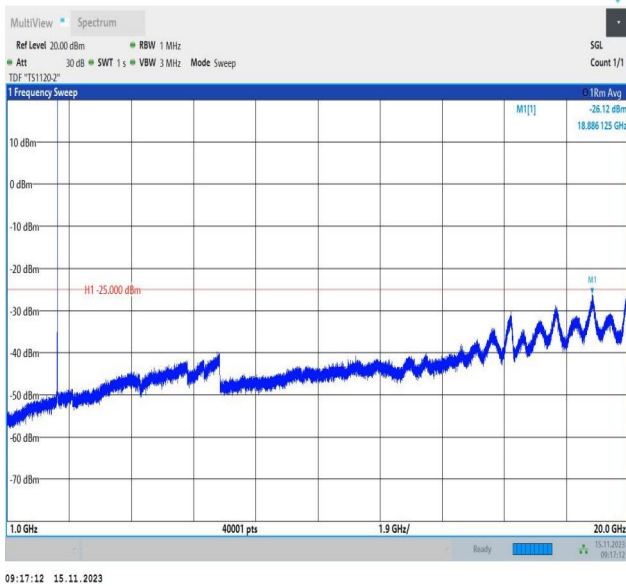
Band7_5MHz_16QAM_21100_1RB#0_1000~20000_1000~20000
