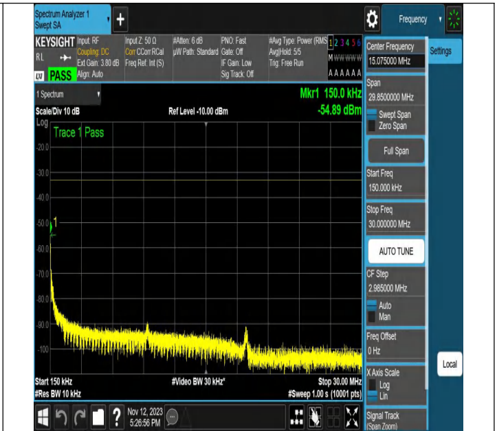
NTNV-N2-PC3-15-20-L-CP-64QAM-Edge_1RB_Left-Ant1-PASS
