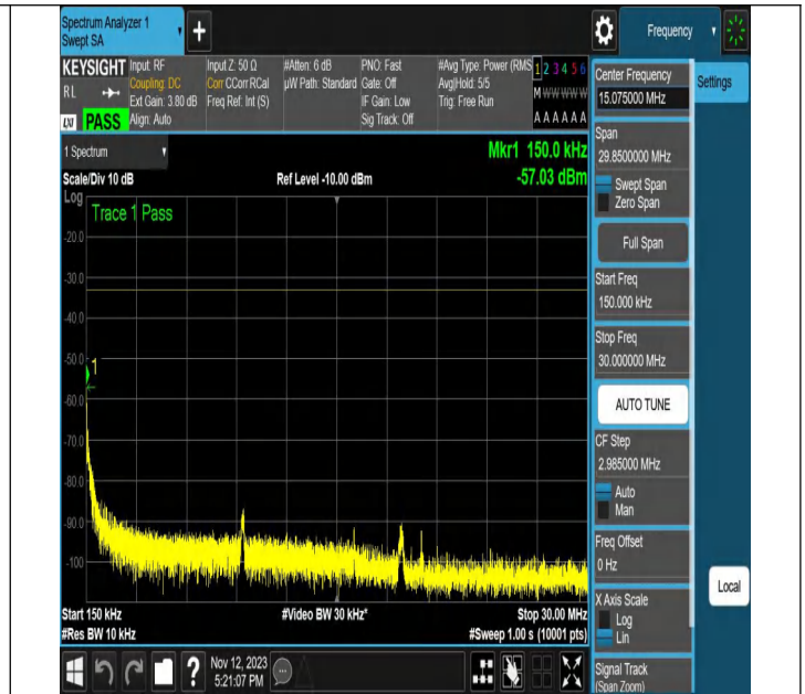
NTNV-N2-PC3-15-20-L-CP-QPSK-Edge_1RB_Left-Ant1-PASS
