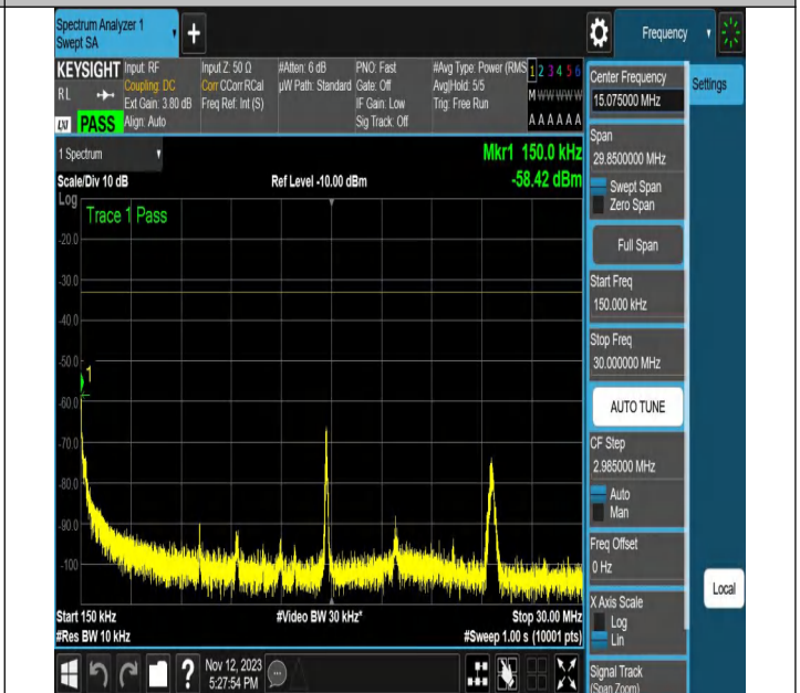
NTNV-N2-PC3-15-20-L-CP-64QAM-Edge_1RB_Right-Ant1-PAS
