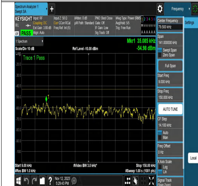
NTNV-N2-PC3-15-20-L-CP-256QAM-Edge_1RB_Left-Ant1-PAS
