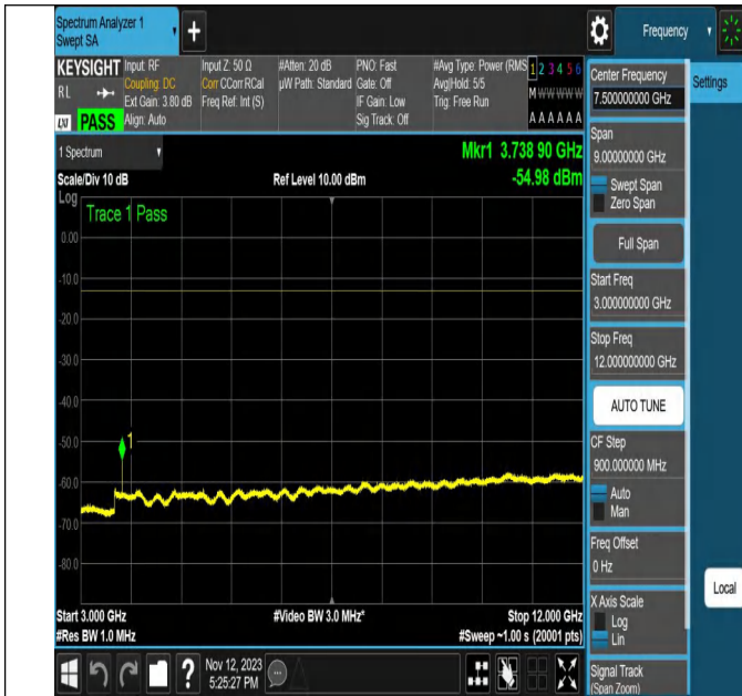
NTVN-N2-PC3-15-20-L-CP-16QAM-Edge_1RB_Right-Ant1-PAS
