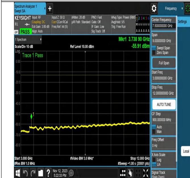
NTNV-N2-PC3-15-20-L-CP-QPSK-Edge_1RB_Right-Ant1-PASS
