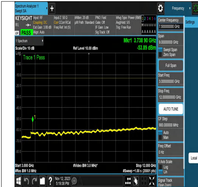
NTNV-N2-PC3-15-20-L-DFT-256QAM-Edge_1RB_Right-Ant1-P
