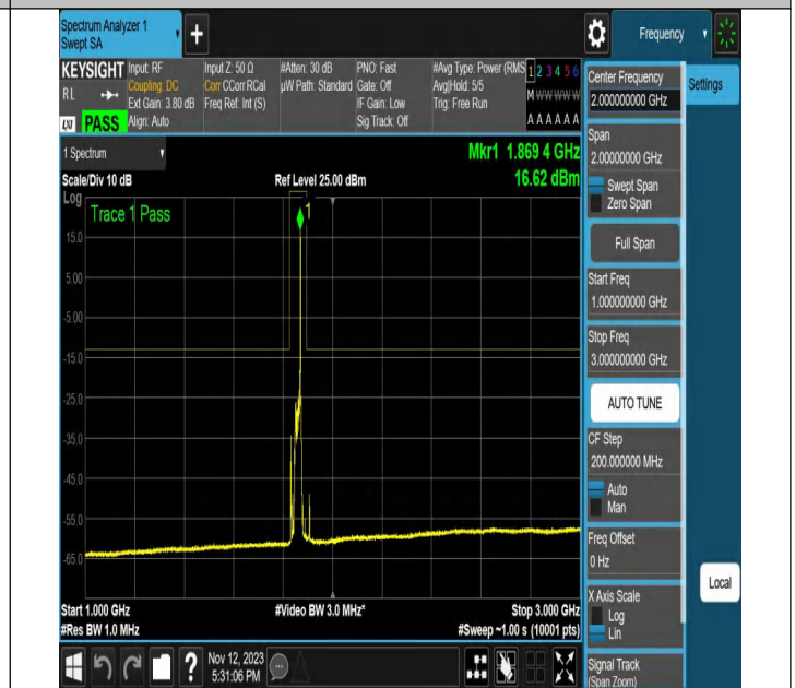
NTNV-N2-PC3-15-20-L-CP-256QAM-Edge_1RB_Right-Ant1-PA
