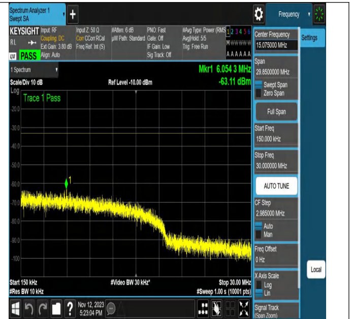
NTNV-N2-PC3-15-20-L-CP-16QAM-Outer_Full-Ant1-PASS
