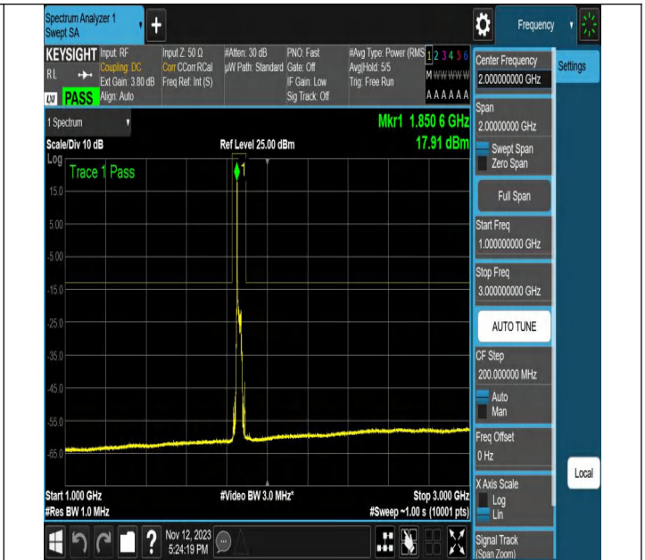
NTNV-N2-PC3-15-20-L-CP-16QAM-Edge_1RB_Left-Ant1-PASS
