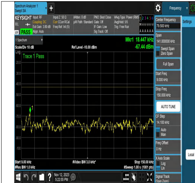
NTNV-N2-PC3-15-20-L-CP-16QAM-Outer_Full-Ant1-PASS
