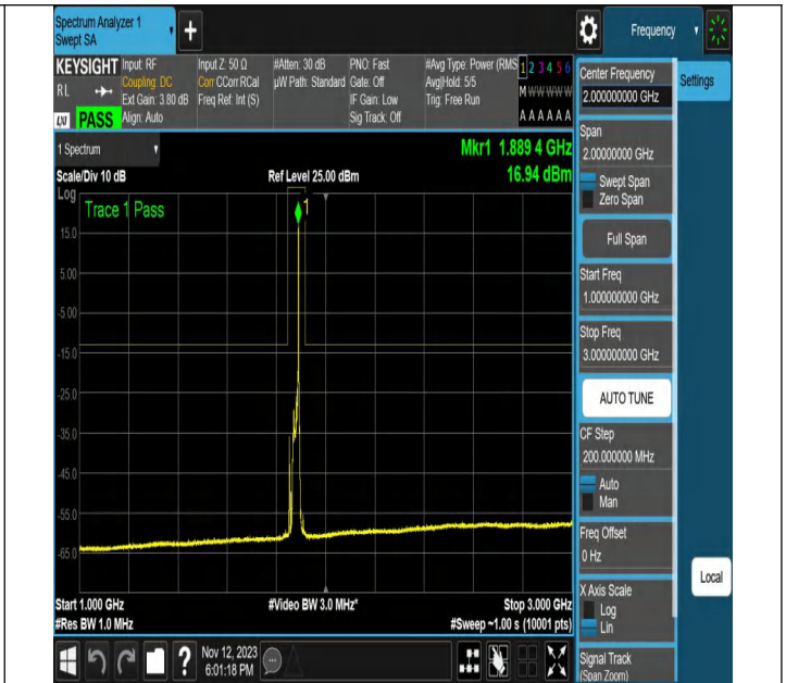
NTNV-N2-PC3-15-20-L-CP-QPSK-Edge_1RB_Right-Ant1-PASS
