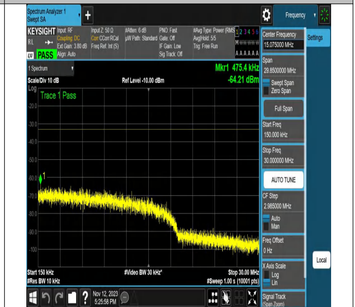
NTVN-N2-PC3-15-20-L-CP-64QAM-Outer_Full-Ant1-PASS
