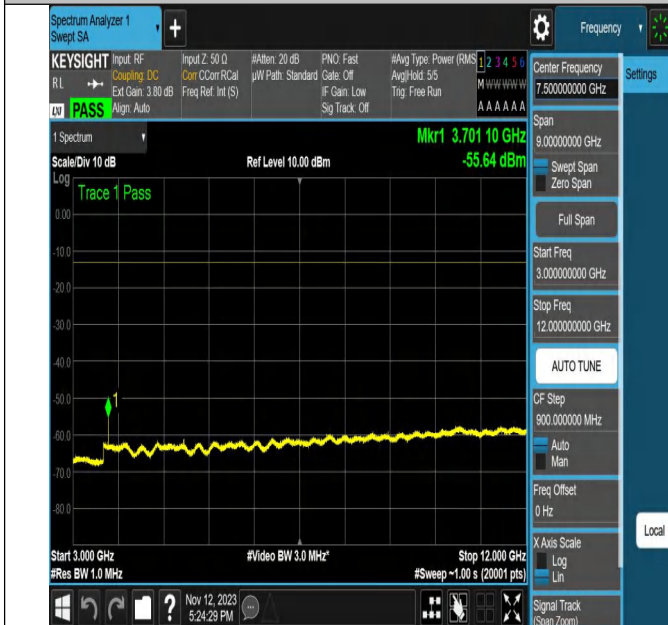
NTNV-N2-PC3-15-20-L-CP-16QAM-Edge_1RB_Left-Ant1-PASS
