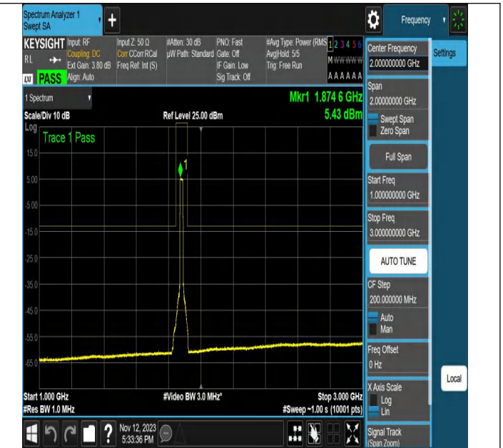
NTNV-N2-PC3-15-20-M-DFT-PI2BPSK-Outter_Full-Ant1-PASS
