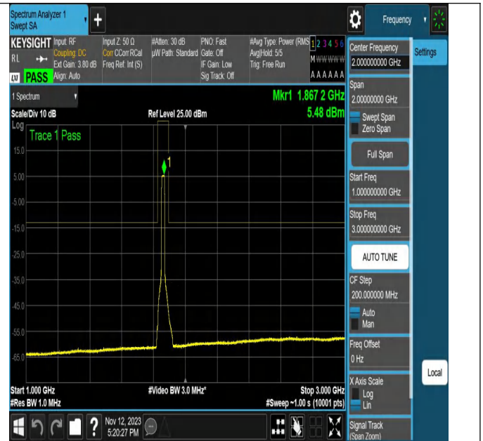
NTNV-N2-PC3-15-20-L-CP-QPSK-Outer_Full-Ant1-PASS
