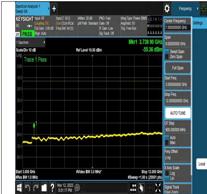
NTNV-N2-PC3-15-20-L-CP-256QAM-Edge_1RB_Right-Ant1-PA
