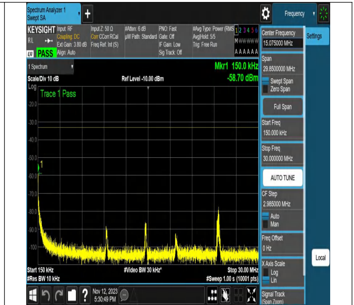
NTNV-N2-PC3-15-20-L-CP-256QAM-Edge_1RB_Right-Ant1-PA
