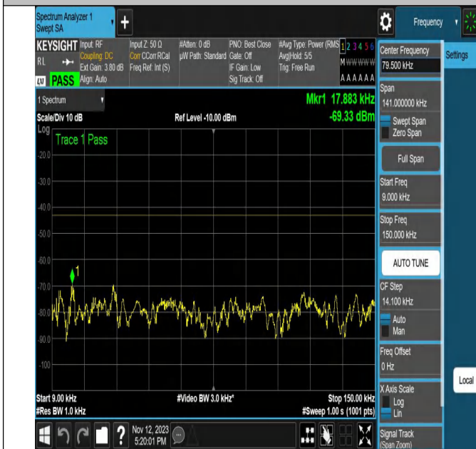
NTNV-N2-PC3-15-20-L-CP-QPSK-Outer_Full-Ant1-PASS
