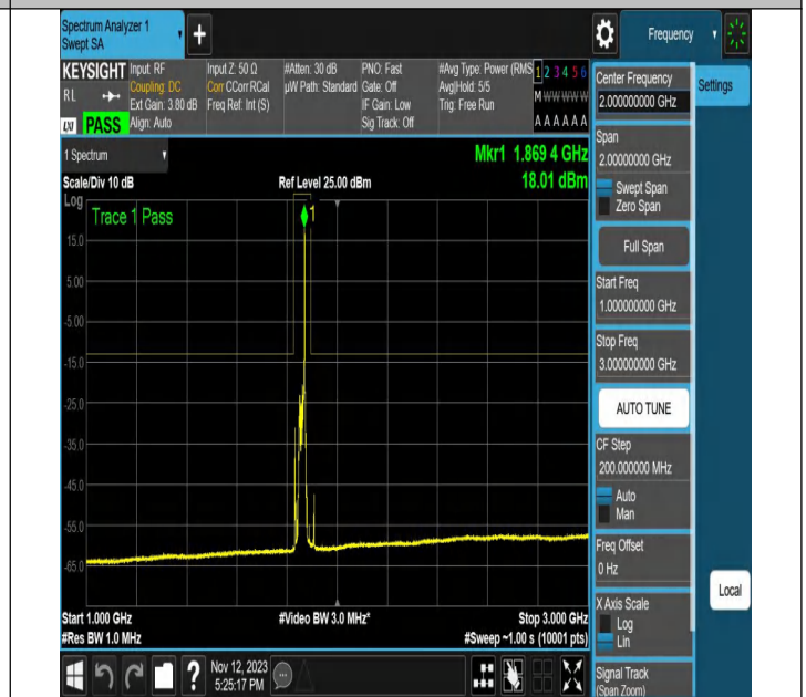
NTVN-N2-PC3-15-20-L-CP-16QAM-Edge_1RB_Right-Ant1-PAS
