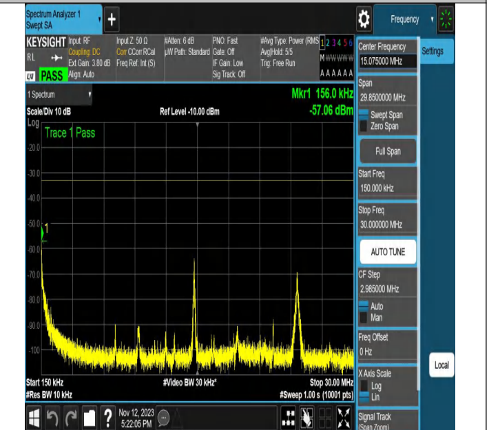
NTNV-N2-PC3-15-20-L-CP-QPSK-Edge_1RB_Right-Ant1-PASS
