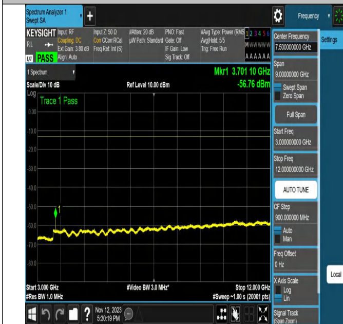
NTNV-N2-PC3-15-20-L-CP-256QAM-Edge_1RB_Left-Ant1-PAS
