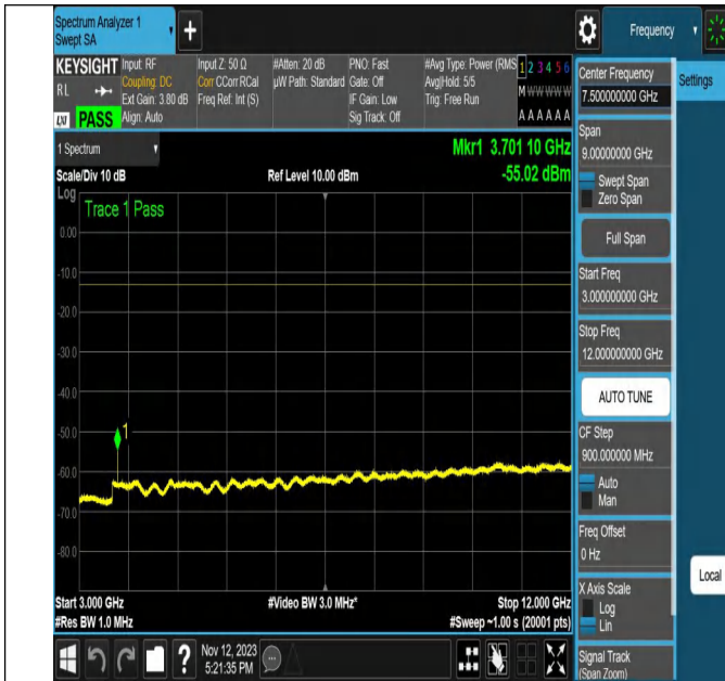
NTNV-N2-PC3-15-20-L-CP-QPSK-Edge_1RB_Left-Ant1-PASS
