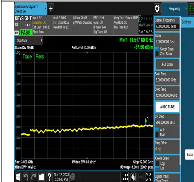
NTNV-N2-PC3-15-20-M-DFT-PI2BPSK-Outter_Full-Ant1-PASS
