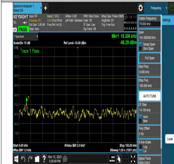
NTVN-N2-PC3-15-20-L-CP-64QAM-Outer_Full-Ant1-PASS
