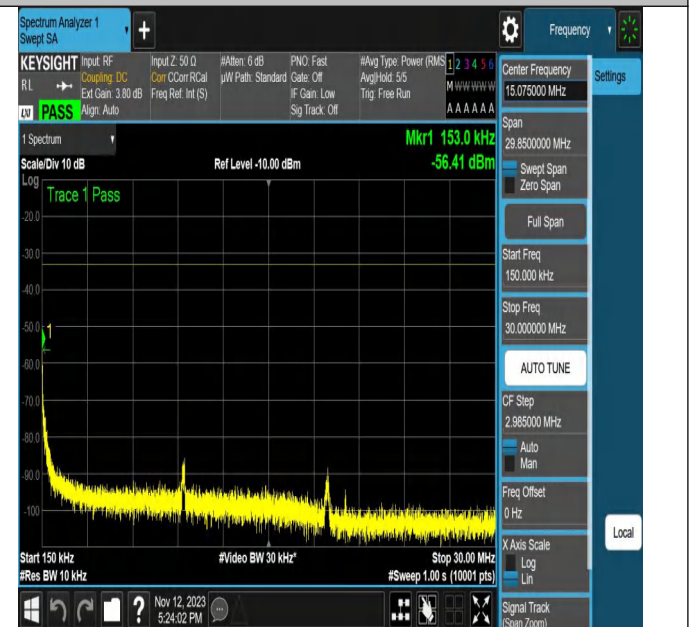
NTNV-N2-PC3-15-20-L-CP-16QAM-Edge_1RB_Left-Ant1-PASS
