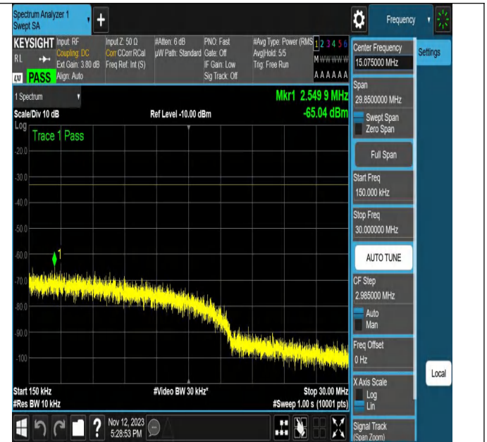
NTNV-N2-PC3-15-20-L-CP-256QAM-Outer_Full-Ant1-PASS
