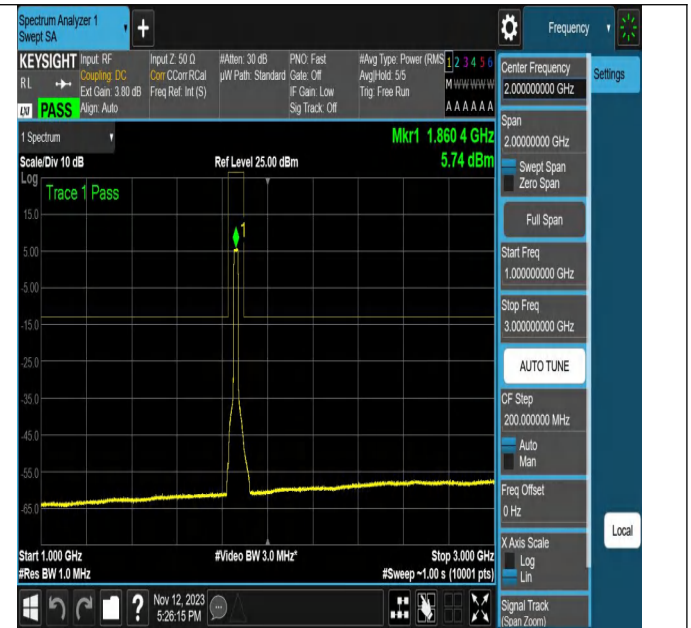
NTNV-N2-PC3-15-20-L-CP-64QAM-Outer_Full-Ant1-PASS
