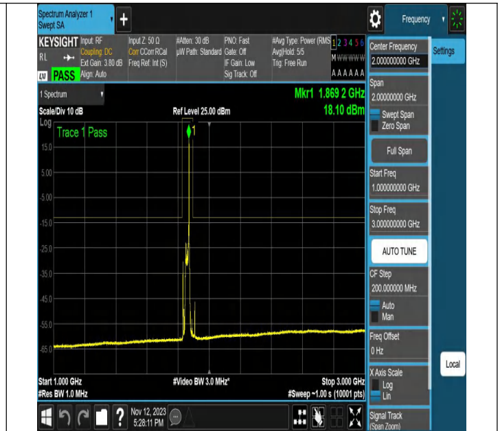
NTVN-N2-PC3-15-20-L-CP-64QAM-Edge_1RB_Right-Ant1-PAS
