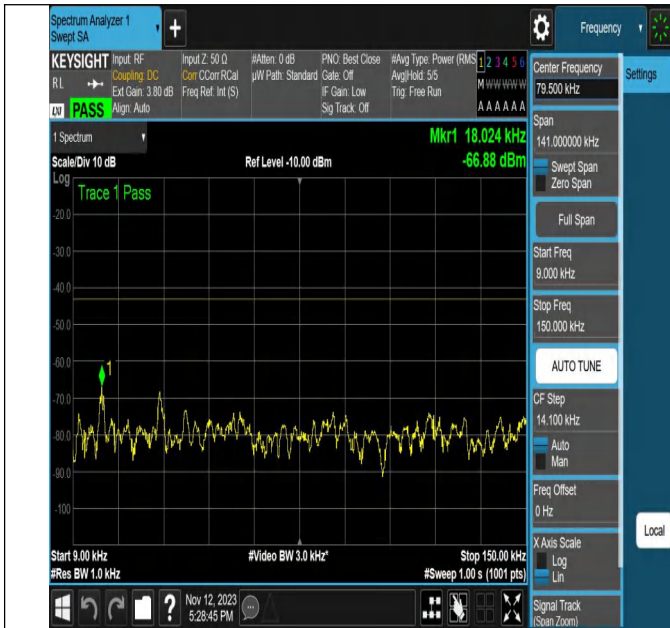
NTNV-N2-PC3-15-20-L-CP-256QAM-Outer_Full-Ant1-PASS
