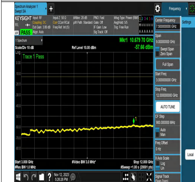
NTNV-N2-PC3-15-20-L-CP-64QAM-Outer_Full-Ant1-PASS
