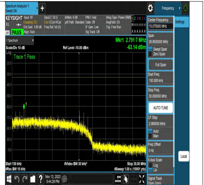
NTNV-N2-PC3-15-20-M-DFT-64QAM-Outer_Full-Ant1-PASS
