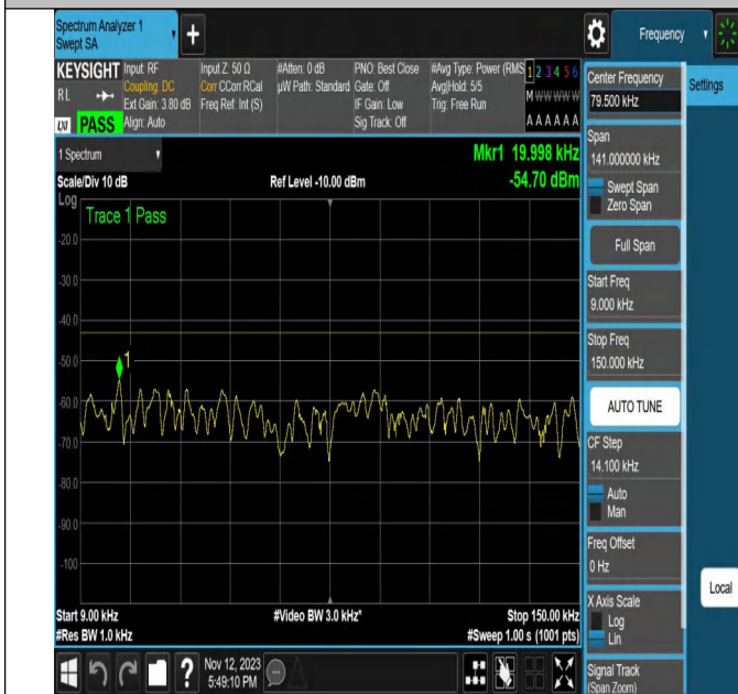
NTVN-N2-PC3-15-20-M-DFT-256QAM-Edge_1RB_Right-Ant1-P
