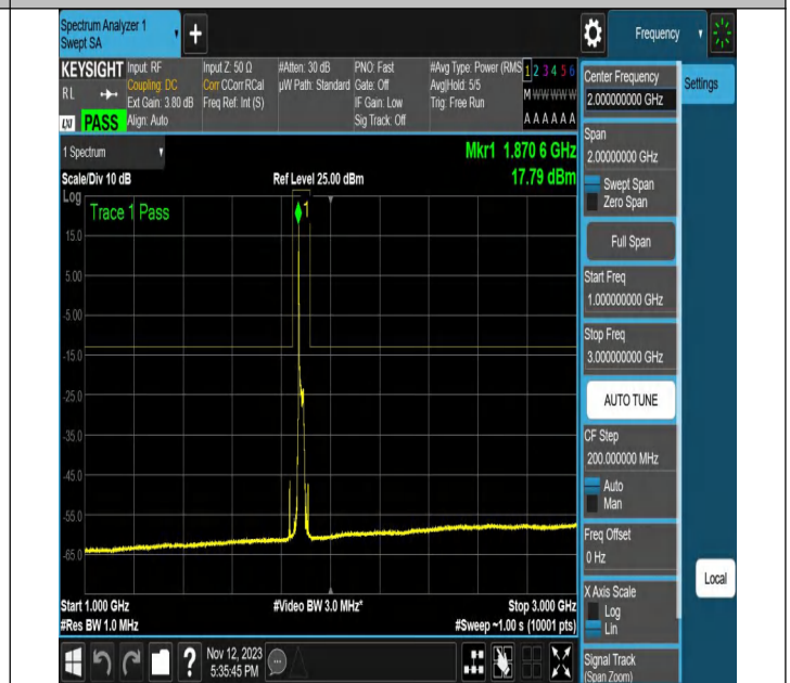
NTNV-N2-PC3-15-20-M-DFT-PI2BPSK-Edge_1RB_Left-Ant1-P
