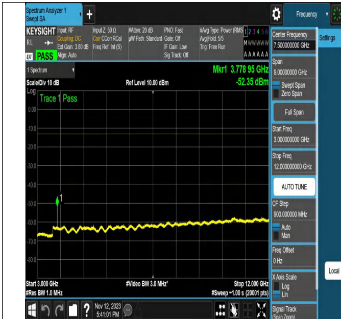
NTNV-N2-PC3-15-20-M-DFT-QPSK-Edge_1RB_Right-Ant1-PA SS
