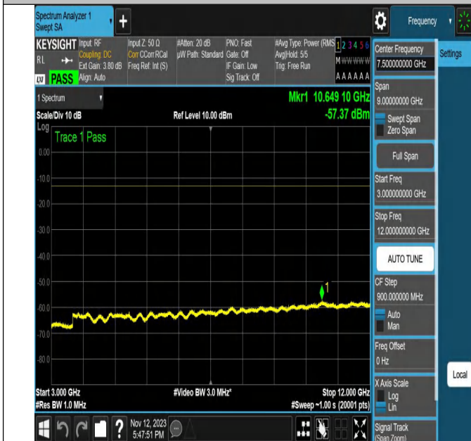
NTNV-N2-PC3-15-20-M-DFT-256QAM-Outer_Full-Ant1-PASS
