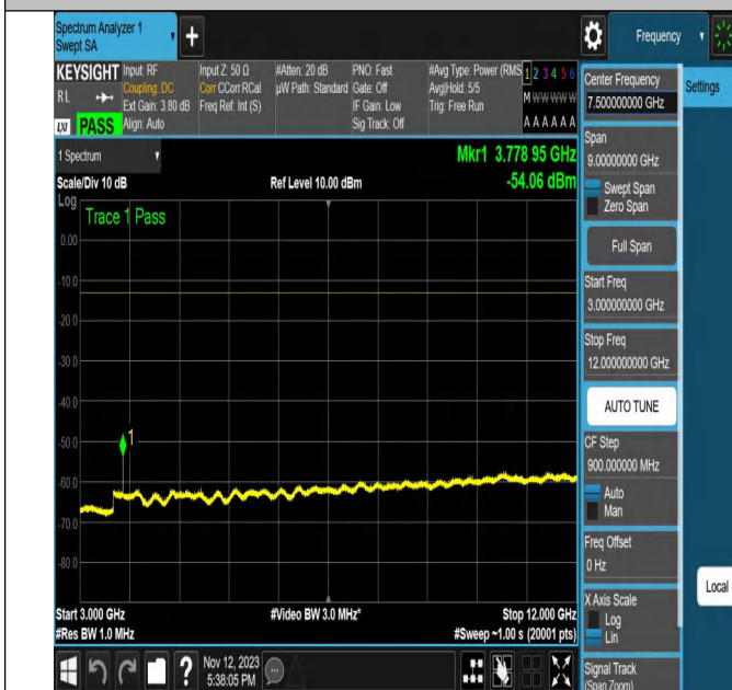
NTNV-N2-PC3-15-20-M-DFT-PI2BPSK-Edge_1RB_Right-Ant1- PASS
