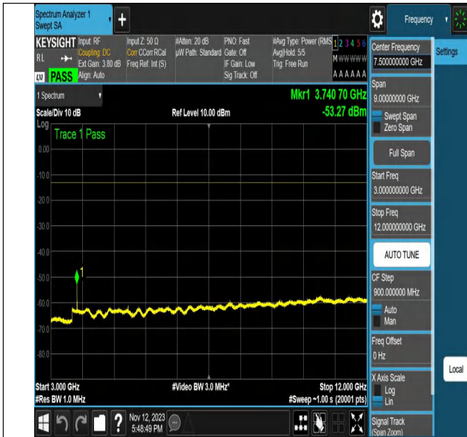
NTVN-N2-PC3-15-20-M-DFT-256QAM-Edge_1RB_Left-Ant1-PA
