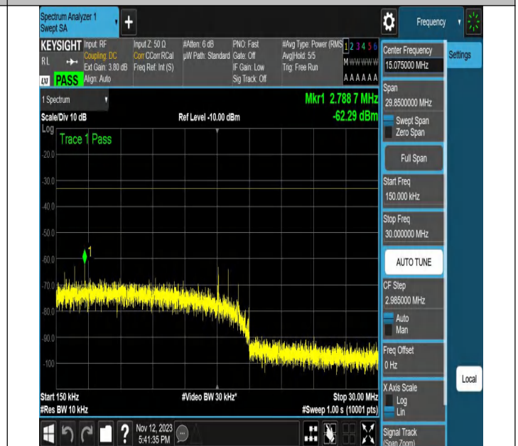
NTNV-N2-PC3-15-20-M-DFT-16QAM-Outer_Full-Ant1-PASS
