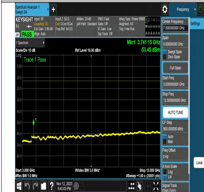
NTNV-N2-PC3-15-20-M-DFT-QPSK-Edge_1RB_Left-Ant1-PAS
