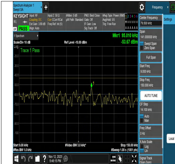
NTNV-N2-PC3-15-20-M-DFT-64QAM-Edge_1RB_Right-Ant1-P
