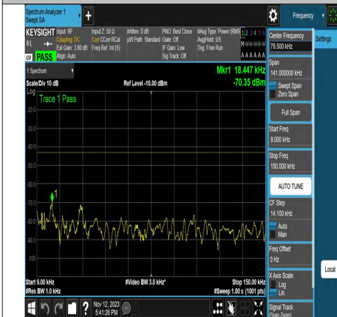
NTNV-N2-PC3-15-20-M-DFT-16QAM-Outer_Full-Ant1-PASS
