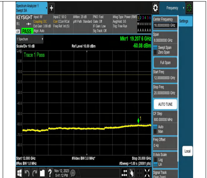
NTNV-N2-PC3-15-20-M-DFT-QPSK-Edge_1RB_Right-Ant1-PA SS
