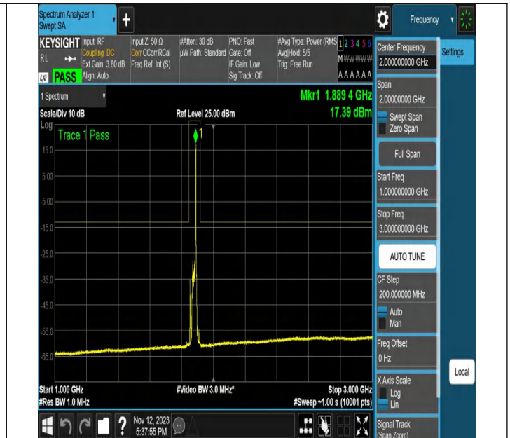
NTNV-N2-PC3-15-20-M-DFT-PI2BPSK-Edge_1RB_Right-Ant1- PASS
