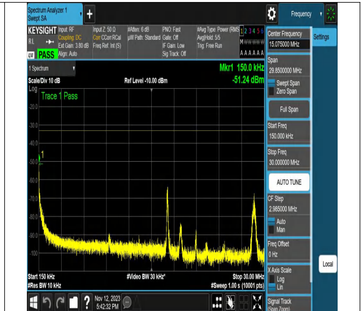
NTNV-N2-PC3-15-20-M-DFT-16QAM-Edge_1RB_Left-Ant1-PA
