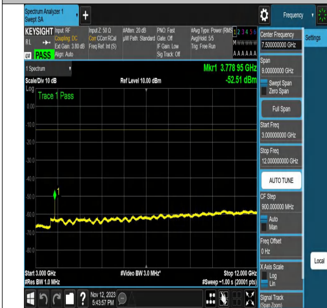
NTNV-N2-PC3-15-20-M-DFT-16QAM-Edge_1RB_Right-Ant1-P
