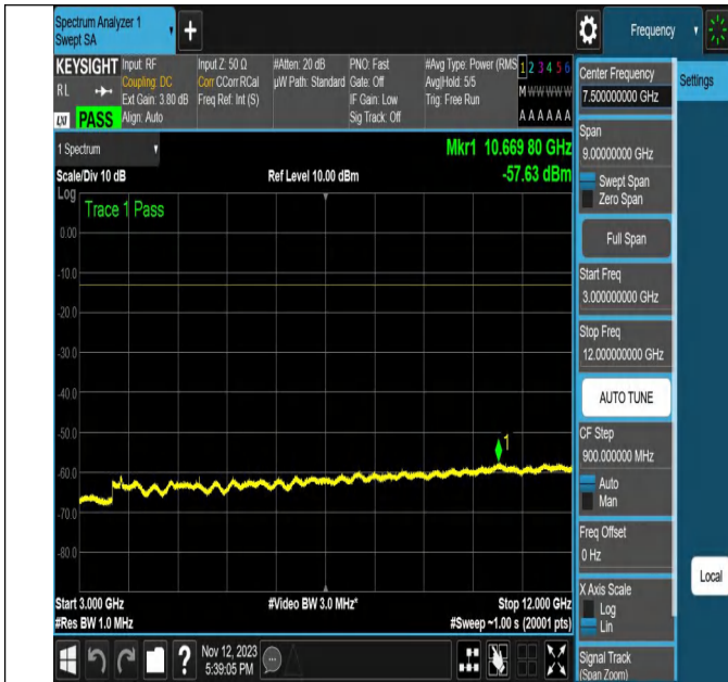
NTNV-N2-PC3-15-20-M-DFT-QPSK-Outter_Full-Ant1-PASS
