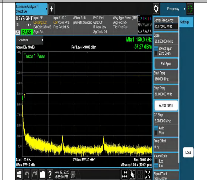
NTNV-N2-PC3-15-20-M-CP-16QAM-Edge_1RB_Right-Ant1-PA
