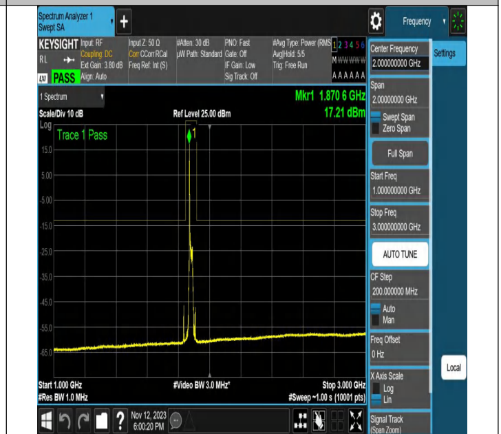
NTNV-N2-PC3-15-20-M-CP-256QAM-Edge_1RB_Left-Ant1-PA
