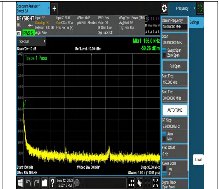
NTNV-N2-PC3-15-20-M-CP-QPSK-Edge_1RB_Right-Ant1-PAS
