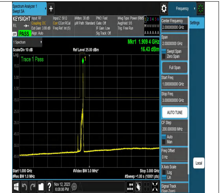
NTNV-N2-PC3-15-20-M-CP-QPSK-Edge_1RB_Left-Ant1-PASS
