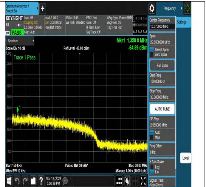
NTNV-N2-PC3-15-20-M-CP-QPSK-Outer_Full-Ant1-PASS
