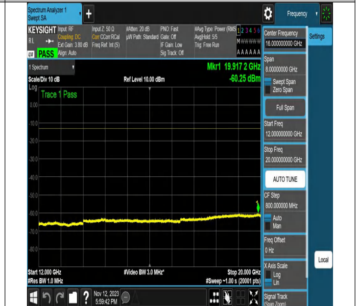
NTNV-N2-PC3-15-20-M-CP-256QAM-Outer_Full-Ant1-PASS
