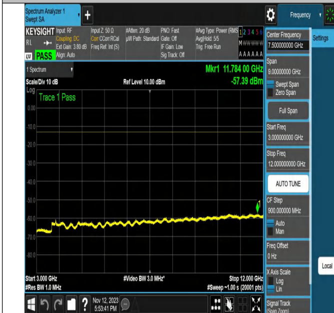
NTNV-N2-PC3-15-20-M-CP-16QAM-Outer_Full-Ant1-PASS
