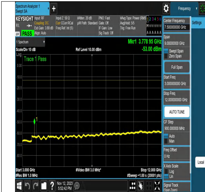
NTNV-N2-PC3-15-20-M-CP-QPSK-Edge_1RB_Right-Ant1-PAS
