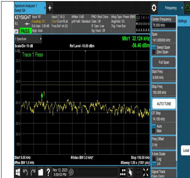
NTNV-N2-PC3-15-20-M-CP-256QAM-Edge_1RB_Left-Ant1-PA
