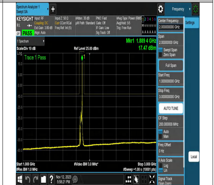
NTNV-N2-PC3-15-20-M-CP-64QAM-Edge_1RB_Right-Ant1-PA
