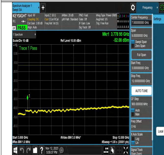
NTNV-N2-PC3-15-20-M-CP-16QAM-Edge_1RB_Right-Ant1-PA
