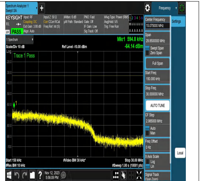
NTNV-N2-PC3-15-20-M-CP-64QAM-Outer_Full-Ant1-PASS
