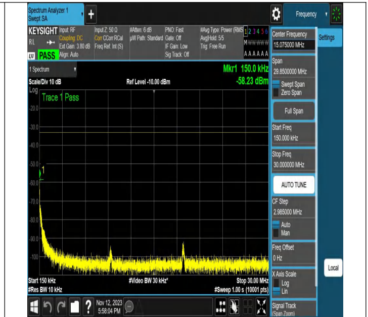
NTNV-N2-PC3-15-20-M-CP-64QAM-Edge_1RB_Right-Ant1-PA
