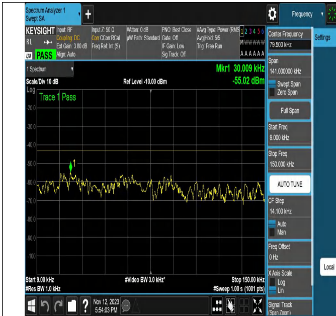
NTNV-N2-PC3-15-20-M-CP-16QAM-Edge_1RB_Left-Ant1-PAS
