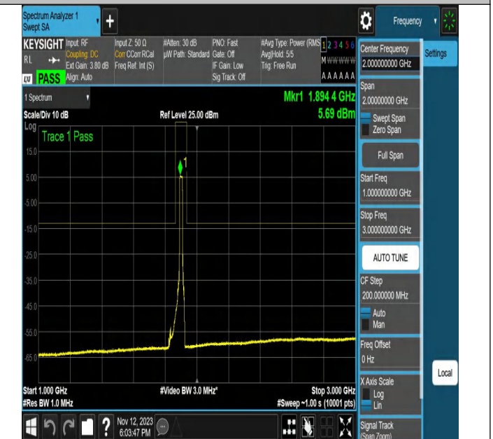
NTNV-N2-PC3-15-20-H-DFT-PI2BPSK-Outter_Full-Ant1-PASS
