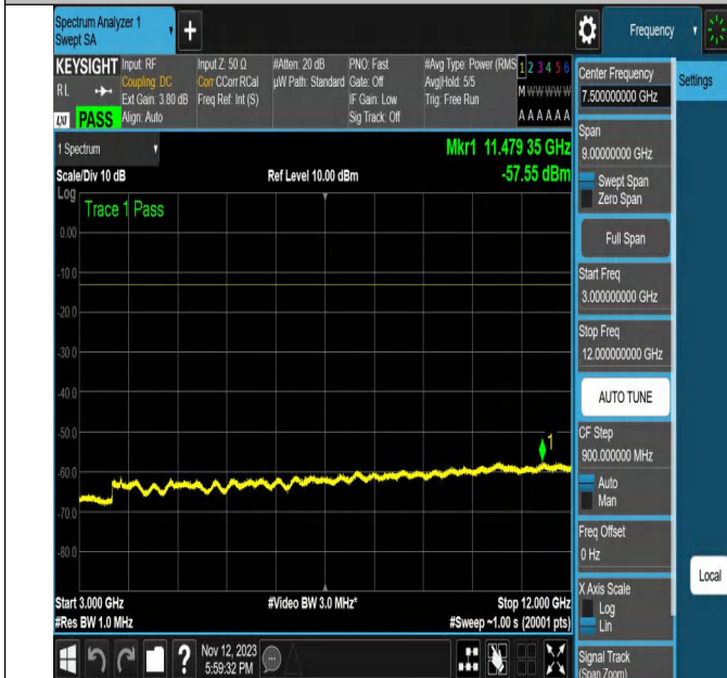
NTNV-N2-PC3-15-20-M-CP-256QAM-Outer_Full-Ant1-PASS
