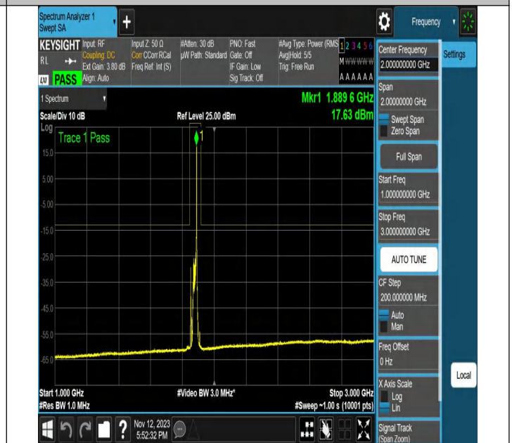
NTNV-N2-PC3-15-20-M-CP-QPSK-Edge_1RB_Right-Ant1-PAS
