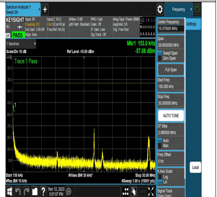
NTNV-N2-PC3-15-20-M-CP-64QAM-Edge_1RB_Left-Ant1-PAS
