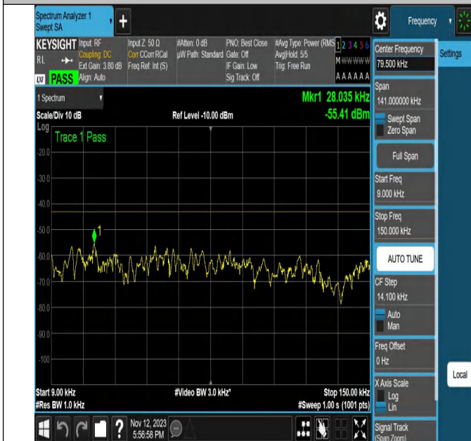
NTNV-N2-PC3-15-20-M-CP-64QAM-Edge_1RB_Left-Ant1-PAS
