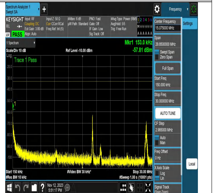
NTNV-N2-PC3-15-20-M-CP-QPSK-Edge_1RB_Left-Ant1-PASS
