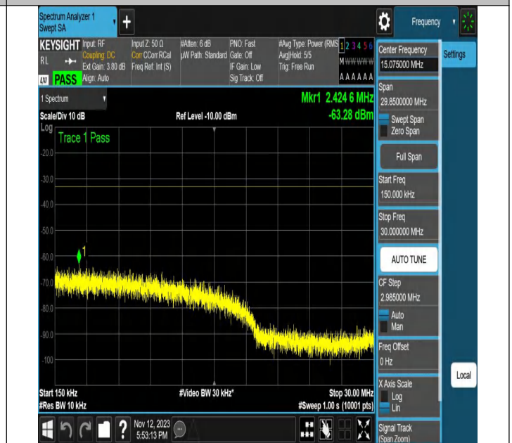
NTNV-N2-PC3-15-20-M-CP-16QAM-Outer_Full-Ant1-PASS
