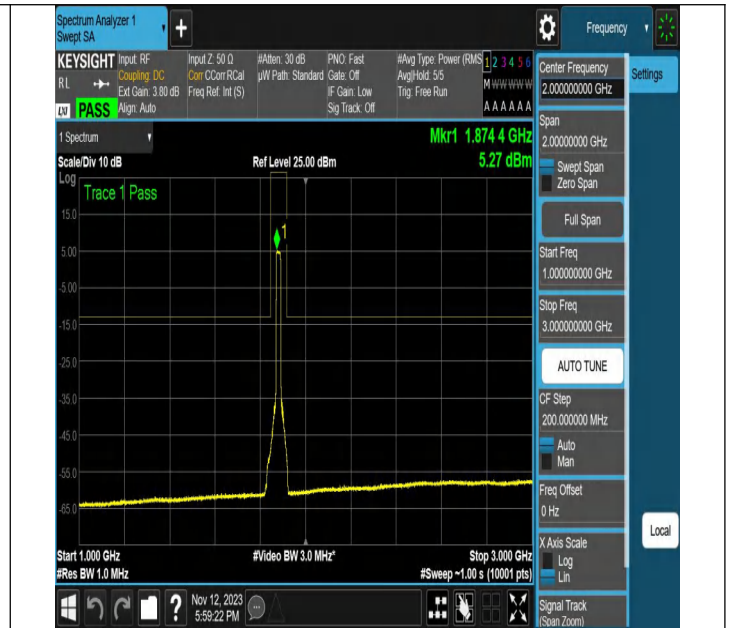
NTNV-N2-PC3-15-20-M-CP-256QAM-Outer_Full-Ant1-PASS
