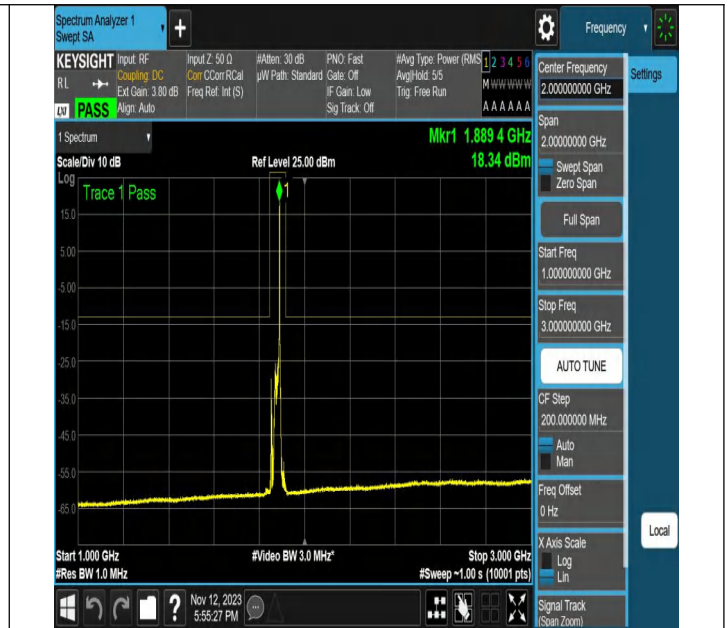
NTNV-N2-PC3-15-20-M-CP-16QAM-Edge_1RB_Right-Ant1-PA
