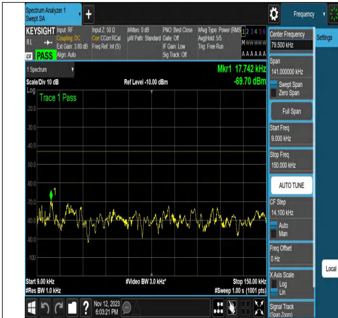
NTNV-N2-PC3-15-20-H-DFT-PI2BPSK-Outter_Full-Ant1-PASS
