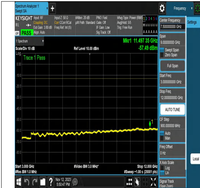
NTNV-N2-PC3-15-20-M-CP-QPSK-Outer_Full-Ant1-PASS
