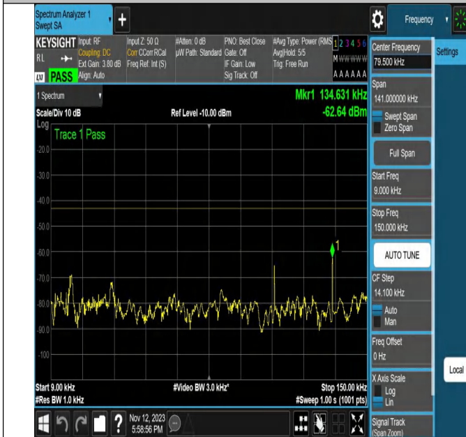
NTNV-N2-PC3-15-20-M-CP-256QAM-Outer_Full-Ant1-PASS
