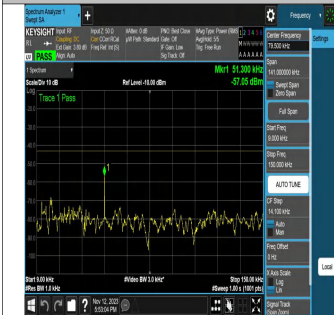
NTNV-N2-PC3-15-20-M-CP-16QAM-Outer_Full-Ant1-PASS
