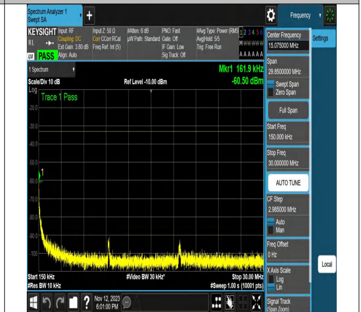
NTNV-N2-PC3-15-20-M-CP-256QAM-Edge_1RB_Right-Ant1-P
