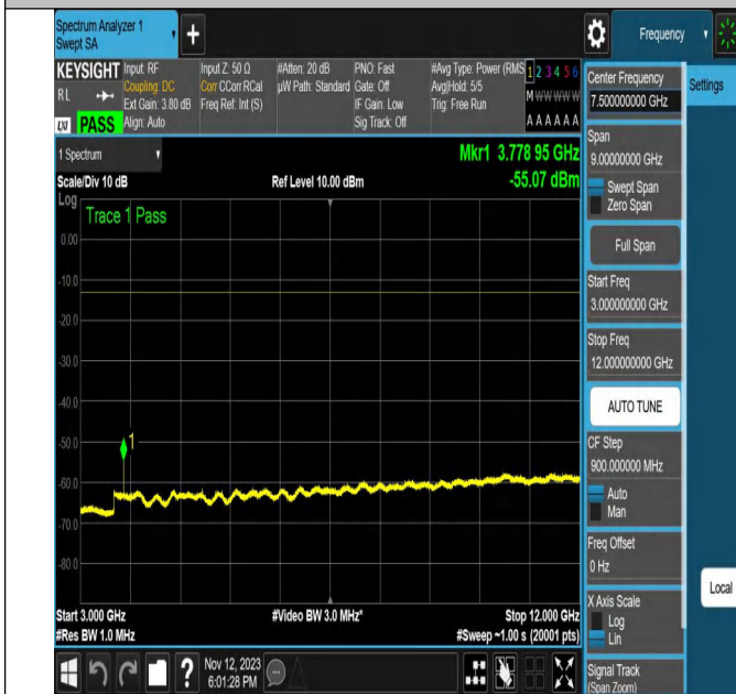
NTNV-N2-PC3-15-20-M-CP-256QAM-Edge_1RB_Right-Ant1-P
