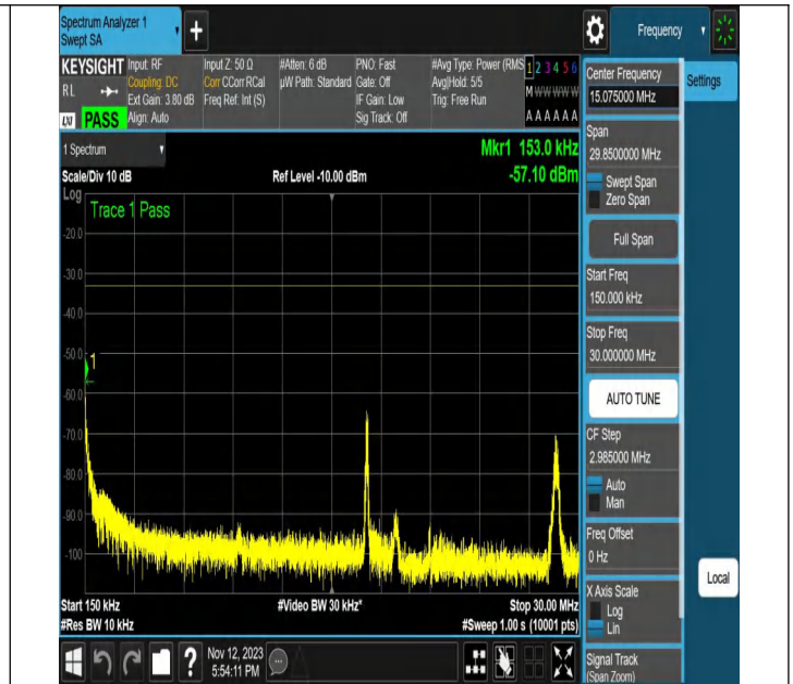
NTNV-N2-PC3-15-20-M-CP-16QAM-Edge_1RB_Left-Ant1-PAS
