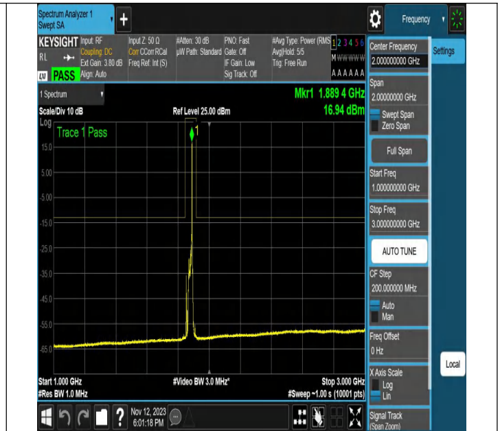
NTNV-N2-PC3-15-20-M-CP-256QAM-Edge_1RB_Right-Ant1-P
