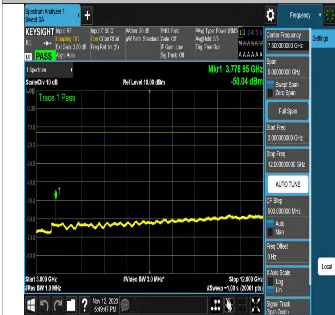
NTVN-N2-PC3-15-20-M-DFT-256QAM-Edge_1RB_Right-Ant1-P ASS
