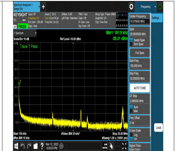
NTNV-N2-PC3-15-20-M-CP-256QAM-Edge_1RB_Left-Ant1-PA
