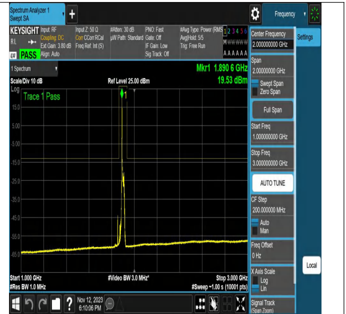
NTNV-N2-PC3-15-20-M-CP-16QAM-Outer_Full-Ant1-PASS
