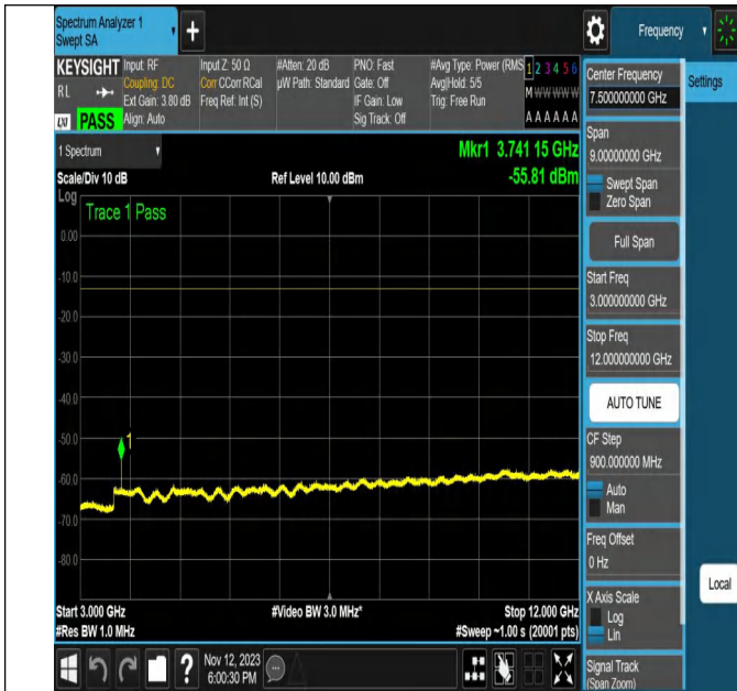
NTNV-N2-PC3-15-20-M-CP-256QAM-Edge_1RB_Left-Ant1-PA
