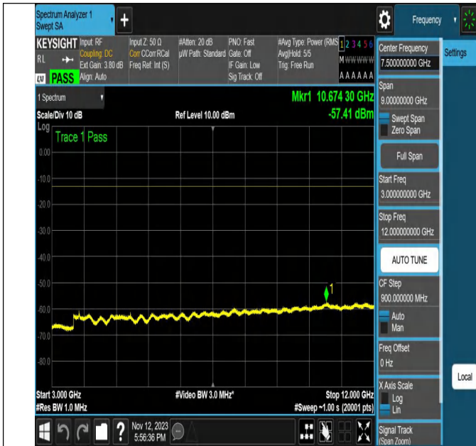
NTNV-N2-PC3-15-20-M-CP-64QAM-Outer_Full-Ant1-PASS
