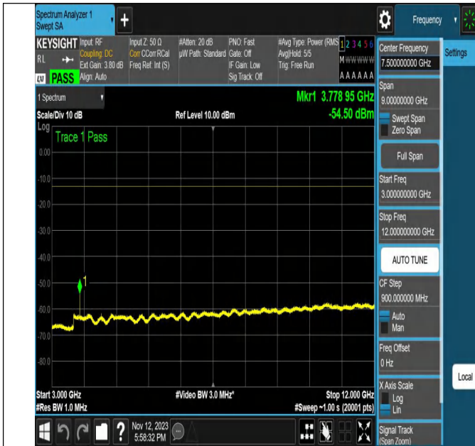
NTNV-N2-PC3-15-20-M-CP-64QAM-Edge_1RB_Right-Ant1-PA
