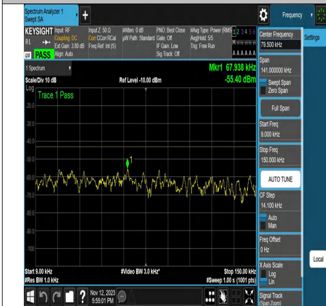
NTNV-N2-PC3-15-20-M-CP-16QAM-Edge_1RB_Right-Ant1-PA
