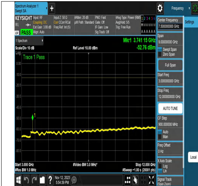
NTNV-N2-PC3-15-20-M-CP-16QAM-Edge_1RB_Left-Ant1-PAS
