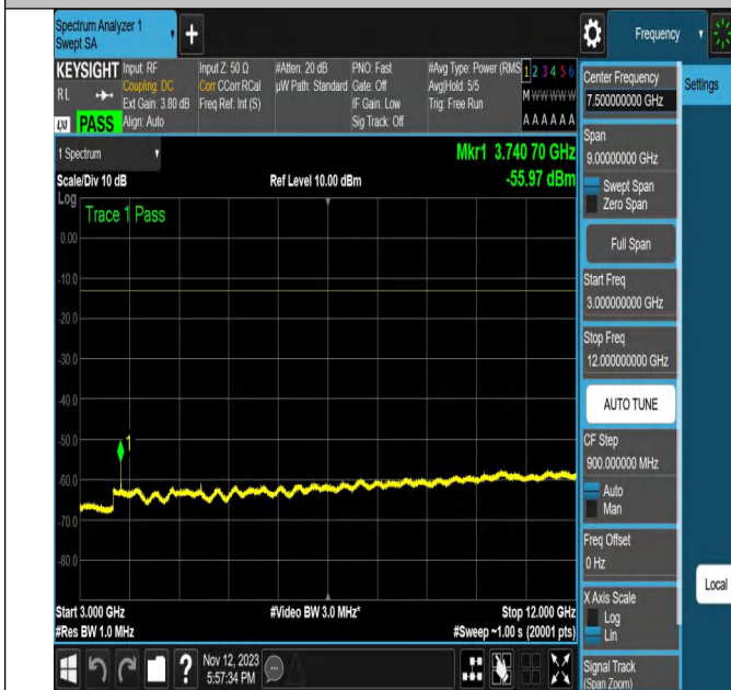
NTNV-N2-PC3-15-20-M-CP-64QAM-Edge_1RB_Left-Ant1-PAS
