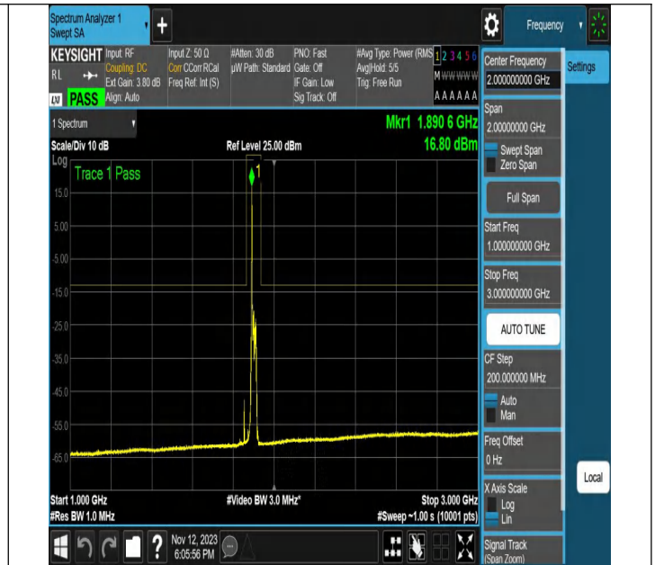
NTNV-N2-PC3-15-20-H-DFT-PI2BPSK-Edge_1RB_Left-Ant1-P
