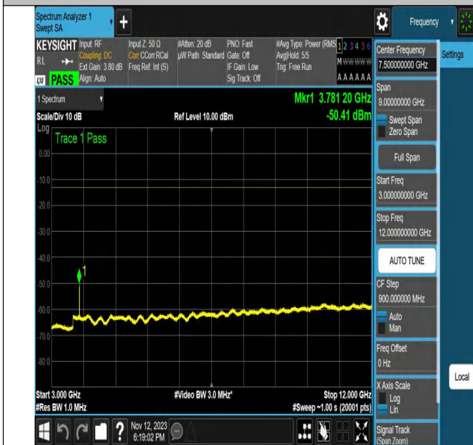
NTNV-N2-PC3-15-20-H-DFT-256QAM-Edge_1RB_Left-Ant1-PA
