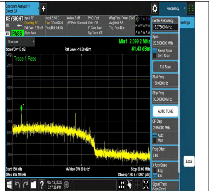
NTNV-N2-PC3-15-20-H-DFT-256QAM-Outer_Full-Ant1-PASS
