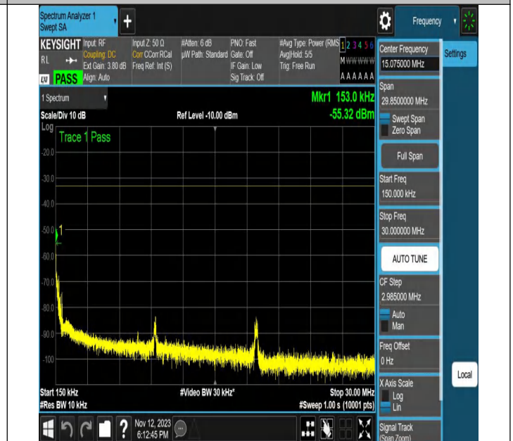
NTNV-N2-PC3-15-20-H-DFT-16QAM-Edge_1RB_Left-Ant1-PAS
