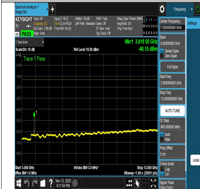
NTVN-N2-PC3-15-20-H-DFT-64QAM-Edge_1RB_Right-Ant1-PA
