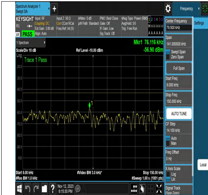
NTNV-N2-PC3-15-20-H-DFT-64QAM-Edge_1RB_Left-Ant1-PAS
