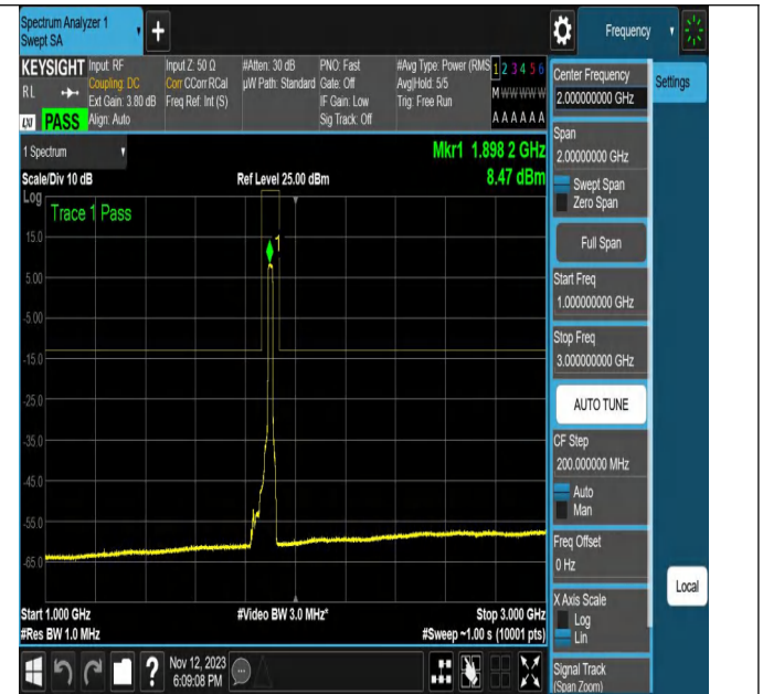
NTNV-N2-PC3-15-20-H-DFT-QPSK-Outer_Full-Ant1-PASS
