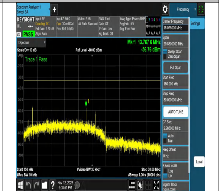
NTNV-N2-PC3-15-20-H-DFT-QPSK-Outer_Full-Ant1-PASS
