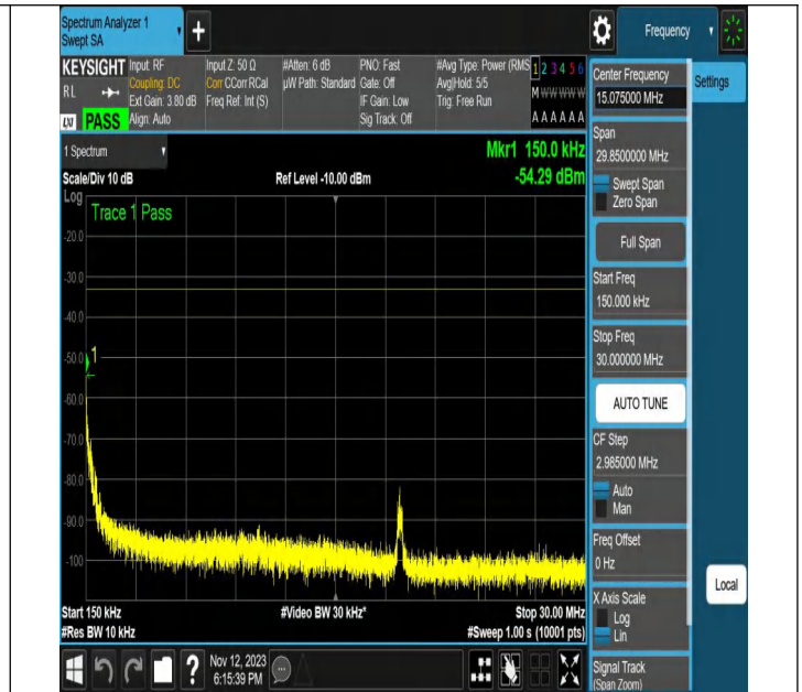
NTNV-N2-PC3-15-20-H-DFT-64QAM-Edge_1RB_Left-Ant1-PAS
