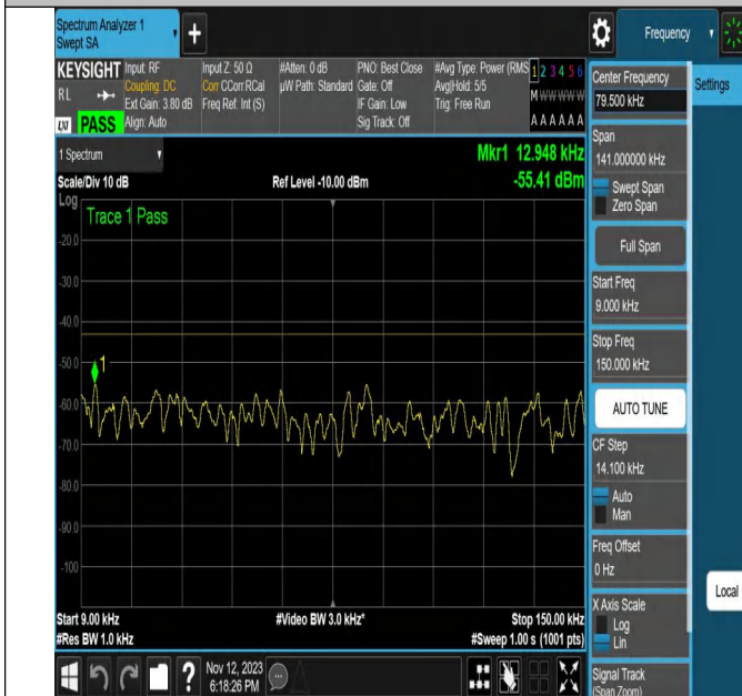
NTNV-N2-PC3-15-20-H-DFT-256QAM-Edge_1RB_Left-Ant1-PA
