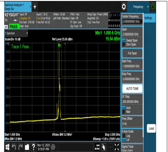
NTNV-N2-PC3-15-20-H-DFT-256QAM-Edge_1RB_Left-Ant1-PA
