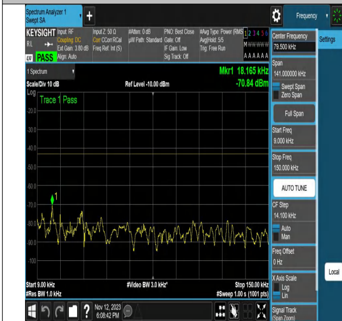
NTNV-N2-PC3-15-20-H-DFT-QPSK-Outer_Full-Ant1-PASS
