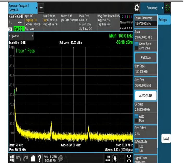
NTNV-N2-PC3-15-20-H-DFT-PI2BPSK-Edge_1RB_Left-Ant1-P
