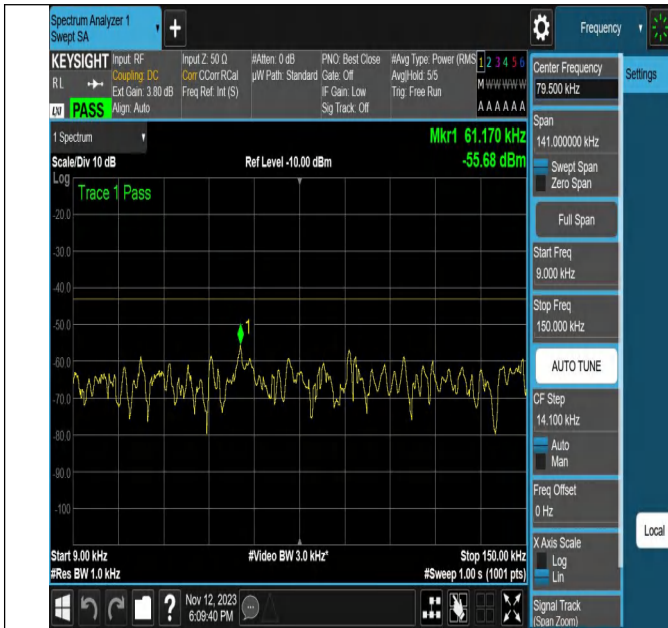
NTNV-N2-PC3-15-20-H-DFT-QPSK-Edge_1RB_Left-Ant1-PASS
