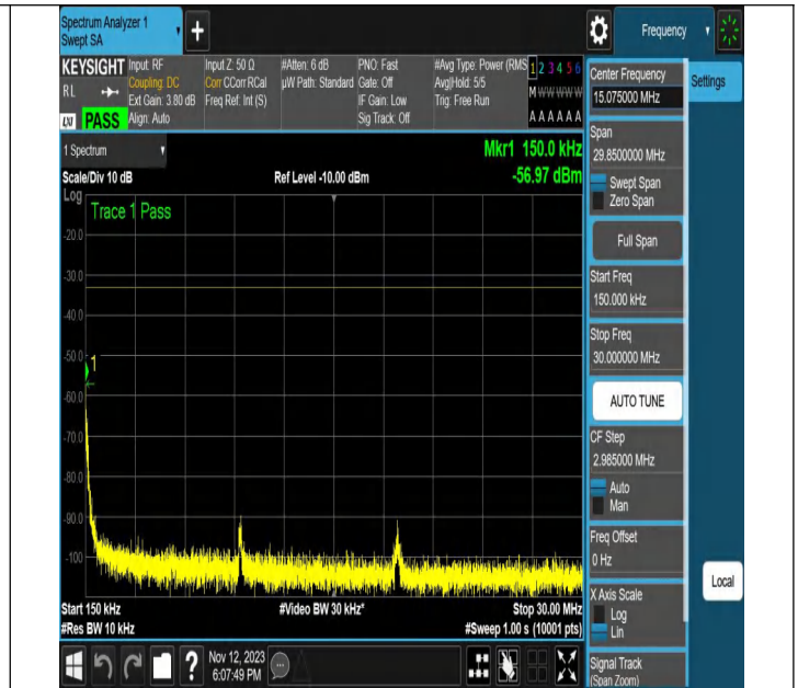
NTNV-N2-PC3-15-20-H-DFT-PI2BPSK-Edge_1RB_Right-Ant1- PASS
