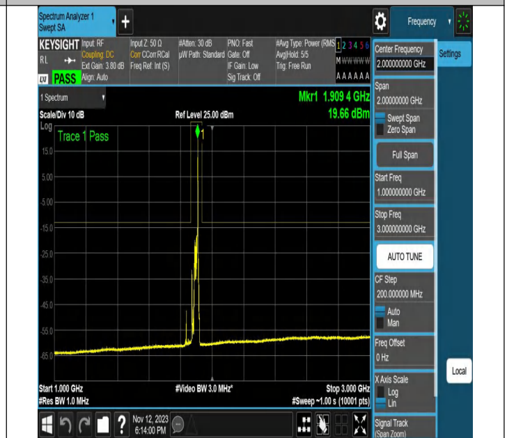
NTNV-N2-PC3-15-20-H-DFT-16QAM-Edge_1RB_Right-Ant1-PA
