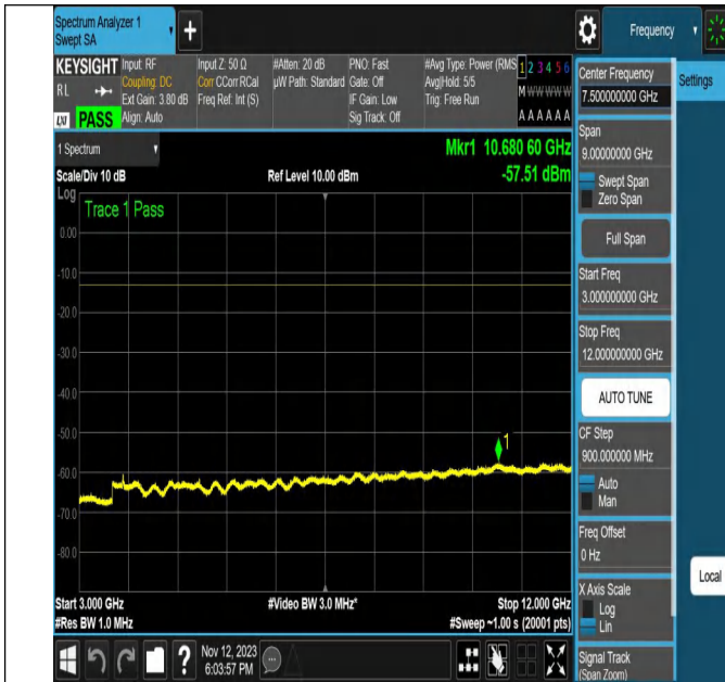
NTNV-N2-PC3-15-20-H-DFT-PI2BPSK-Outer_Full-Ant1-PASS
