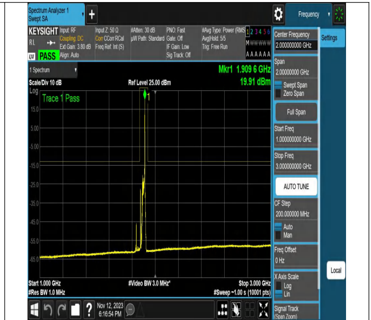
NTVN-N2-PC3-15-20-H-DFT-64QAM-Edge_1RB_Right-Ant1-PA
