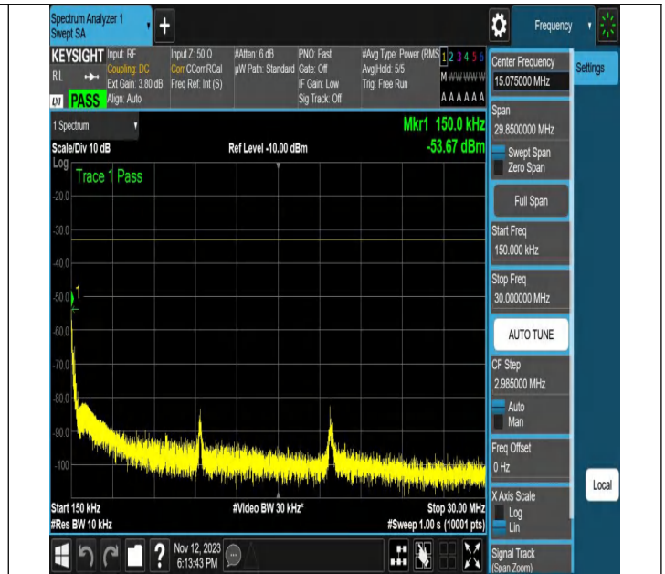
NTNV-N2-PC3-15-20-H-DFT-16QAM-Edge_1RB_Right-Ant1-PA
