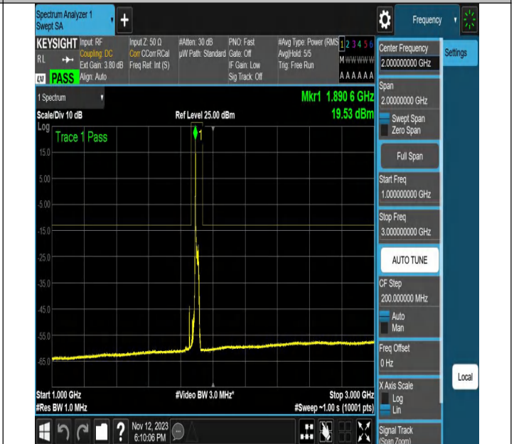
NTNV-N2-PC3-15-20-H-DFT-QPSK-Edge_1RB_Left-Ant1-PASS
