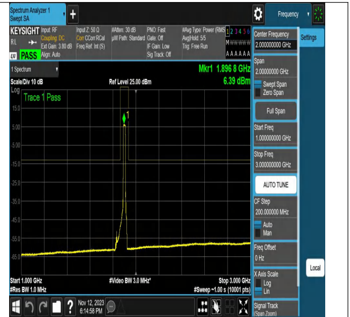
NTNV-N2-PC3-15-20-H-DFT-64QAM-Outer_Full-Ant1-PASS
