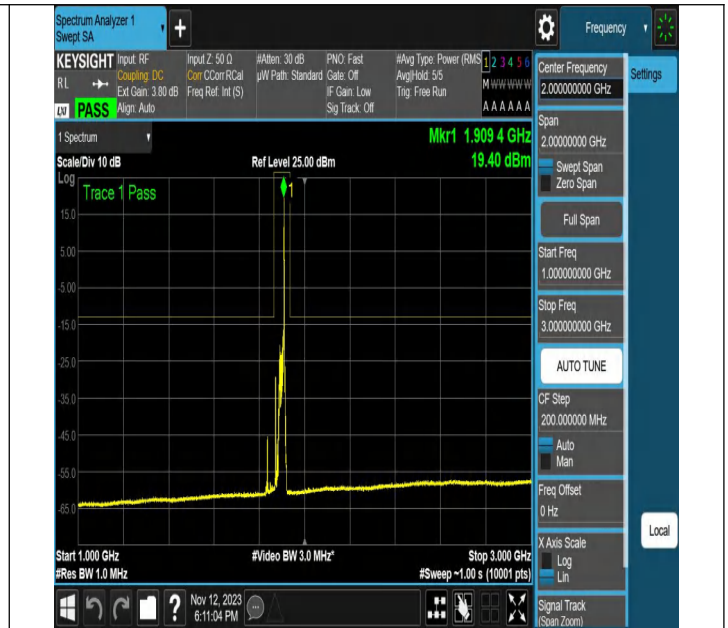
NTVN-N2-PC3-15-20-H-DFT-QPSK-Edge_1RB_Right-Ant1-PAS
