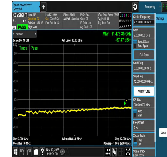
NTNV-N2-PC3-15-20-H-DFT-256QAM-Outer_Full-Ant1-PASS
