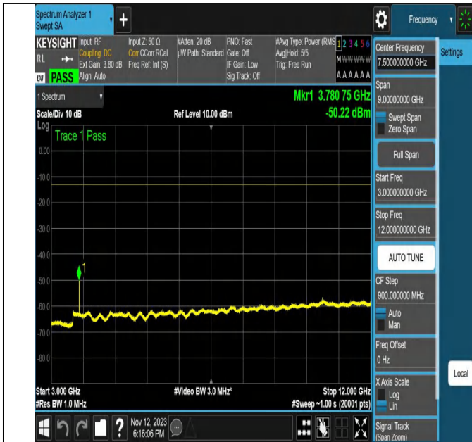
NTVN-N2-PC3-15-20-H-DFT-64QAM-Edge_1RB_Left-Ant1-PAS
