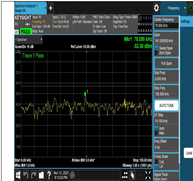
NTNV-N2-PC3-15-20-H-DFT-16QAM-Edge_1RB_Right-Ant1-PA
