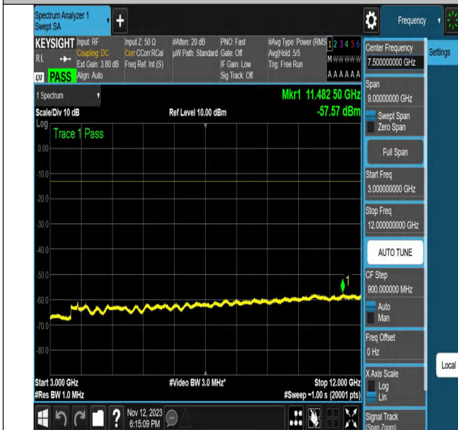
NTNV-N2-PC3-15-20-H-DFT-64QAM-Outer_Full-Ant1-PASS
