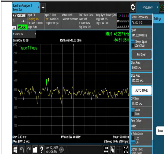
NTNV-N2-PC3-15-20-H-DFT-16QAM-Edge_1RB_Left-Ant1-PAS
