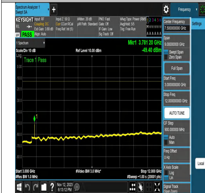
NTVN-N2-PC3-15-20-H-DFT-16QAM-Edge_1RB_Left-Ant1-PAS
