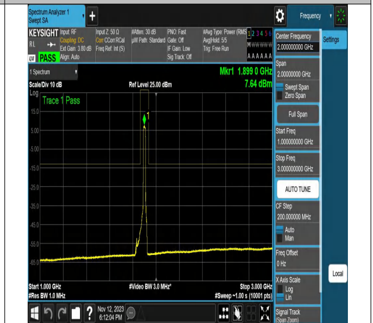
NTNV-N2-PC3-15-20-H-DFT-64QAM-Edge_1RB_Left-Ant1-PAS
