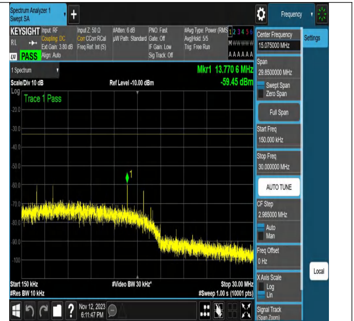
NTNV-N2-PC3-15-20-H-DFT-16QAM-Outer_Full-Ant1-PASS
