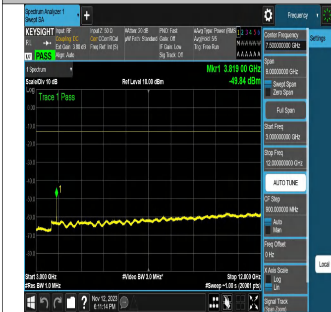
NTVN-N2-PC3-15-20-H-DFT-QPSK-Edge_1RB_Right-Ant1-PAS
