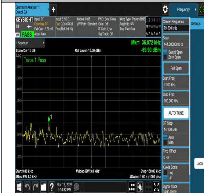
NTVN-N2-PC3-15-20-H-DFT-64QAM-Outer_Full-Ant1-PASS
