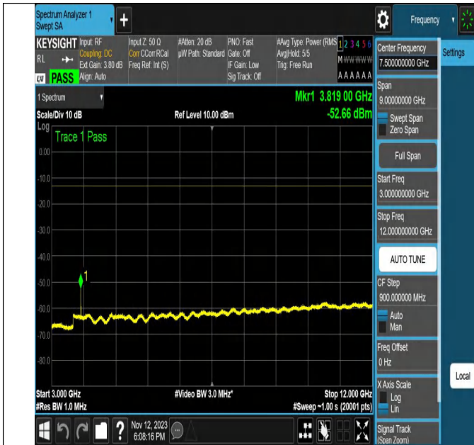
NTNV-N2-PC3-15-20-H-DFT-PI2BPSK-Edge_1RB_Right-Ant1-PASS
