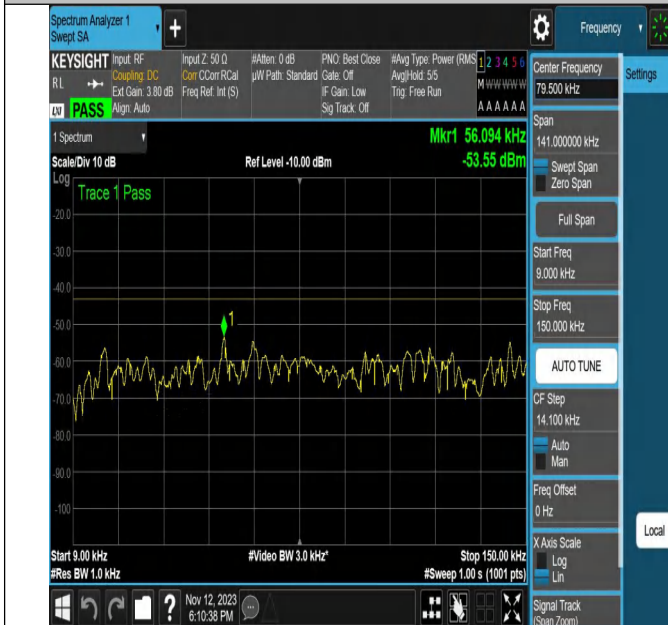
NTNV-N2-PC3-15-20-H-DFT-QPSK-Edge_1RB_Right-Ant1-PAS
