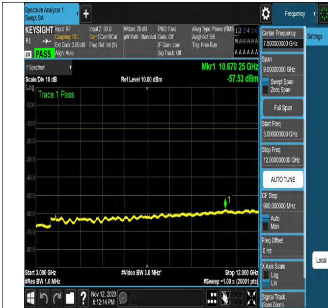
NTNV-N2-PC3-15-20-H-DFT-16QAM-Outer_Full-Ant1-PASS
