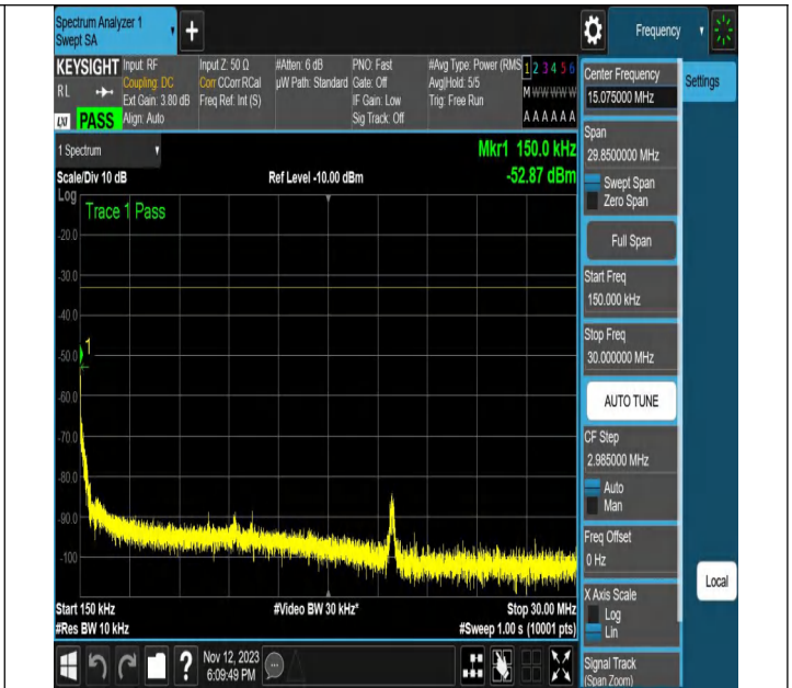
NTNV-N2-PC3-15-20-H-DFT-QPSK-Edge_1RB_Left-Ant1-PASS
