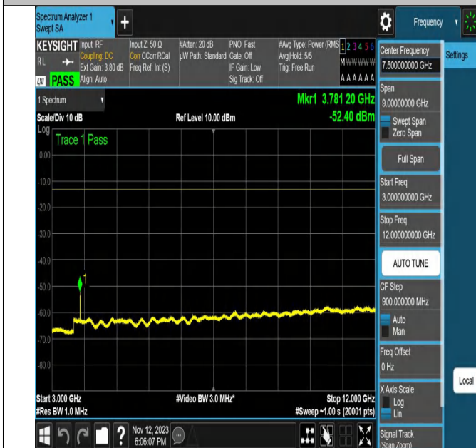
NTNV-N2-PC3-15-20-H-DFT-PI2BPSK-Edge_1RB_Left-Ant1-P
