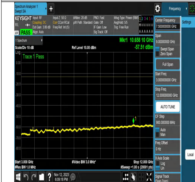
NTNV-N2-PC3-15-20-H-DFT-QPSK-Outer_Full-Ant1-PASS
