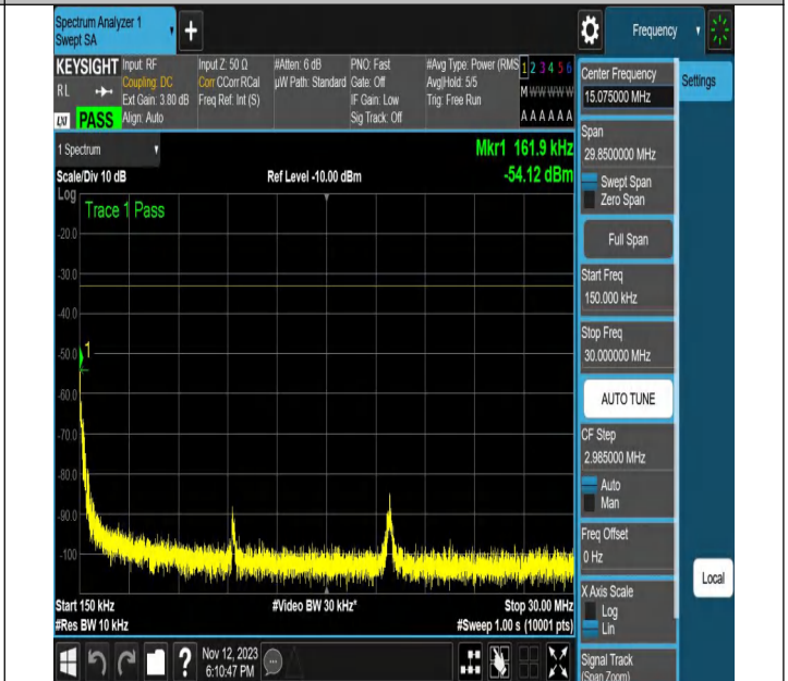
NTNV-N2-PC3-15-20-H-DFT-QPSK-Edge_1RB_Right-Ant1-PAS
