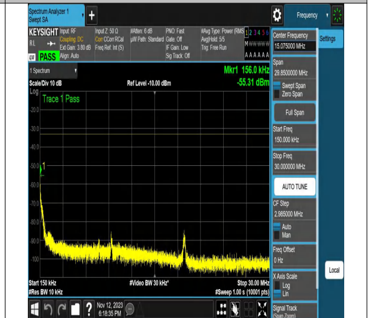
NTNV-N2-PC3-15-20-H-DFT-256QAM-Edge_1RB_Left-Ant1-PA
