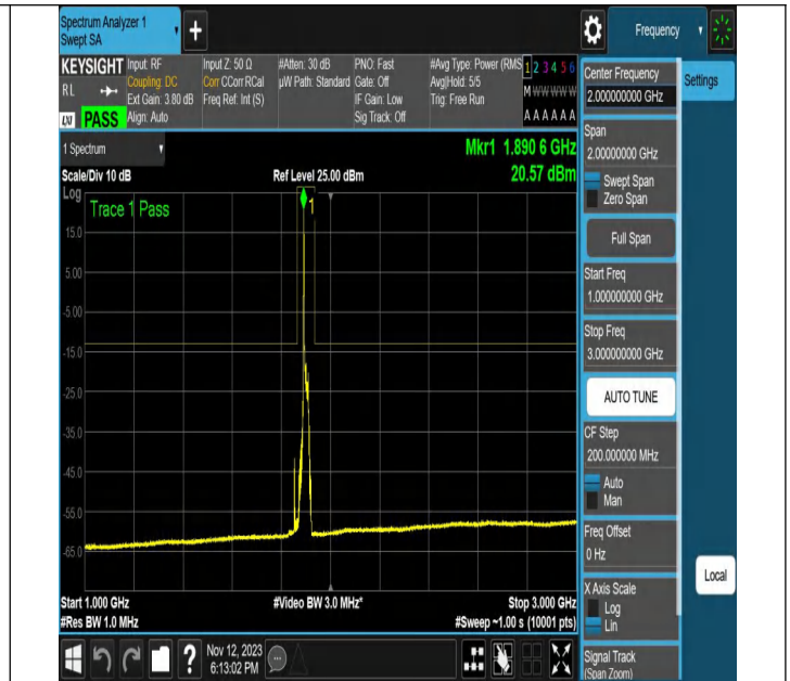
NTVN-N2-PC3-15-20-H-DFT-16QAM-Edge_1RB_Left-Ant1-PAS
